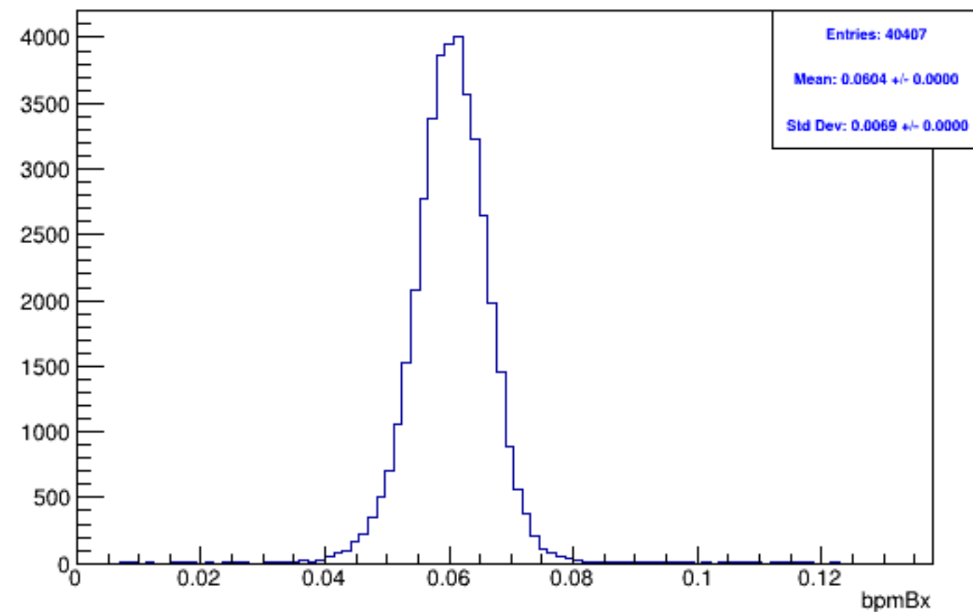
Run 5731, mpwise, bpmBx: Beam ON, Laser OFF
