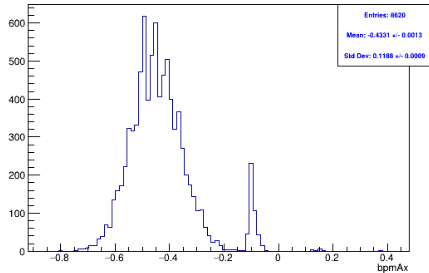
Run 5731 mpwise, bpmAx: Beam OFF
