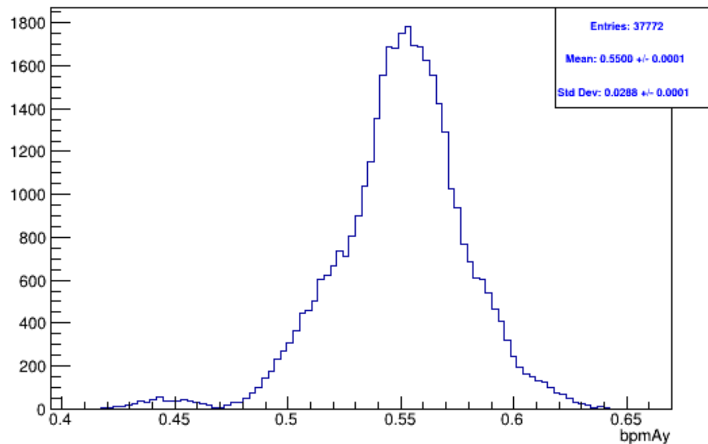
Run 5731, mpwise, bpmAy: Beam ON, Laser ON
