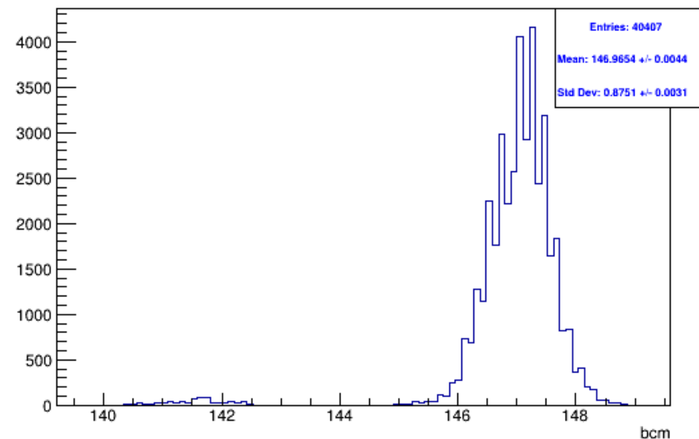
Run 5731, mpwise, BCM: Beam ON, Laser OFF
