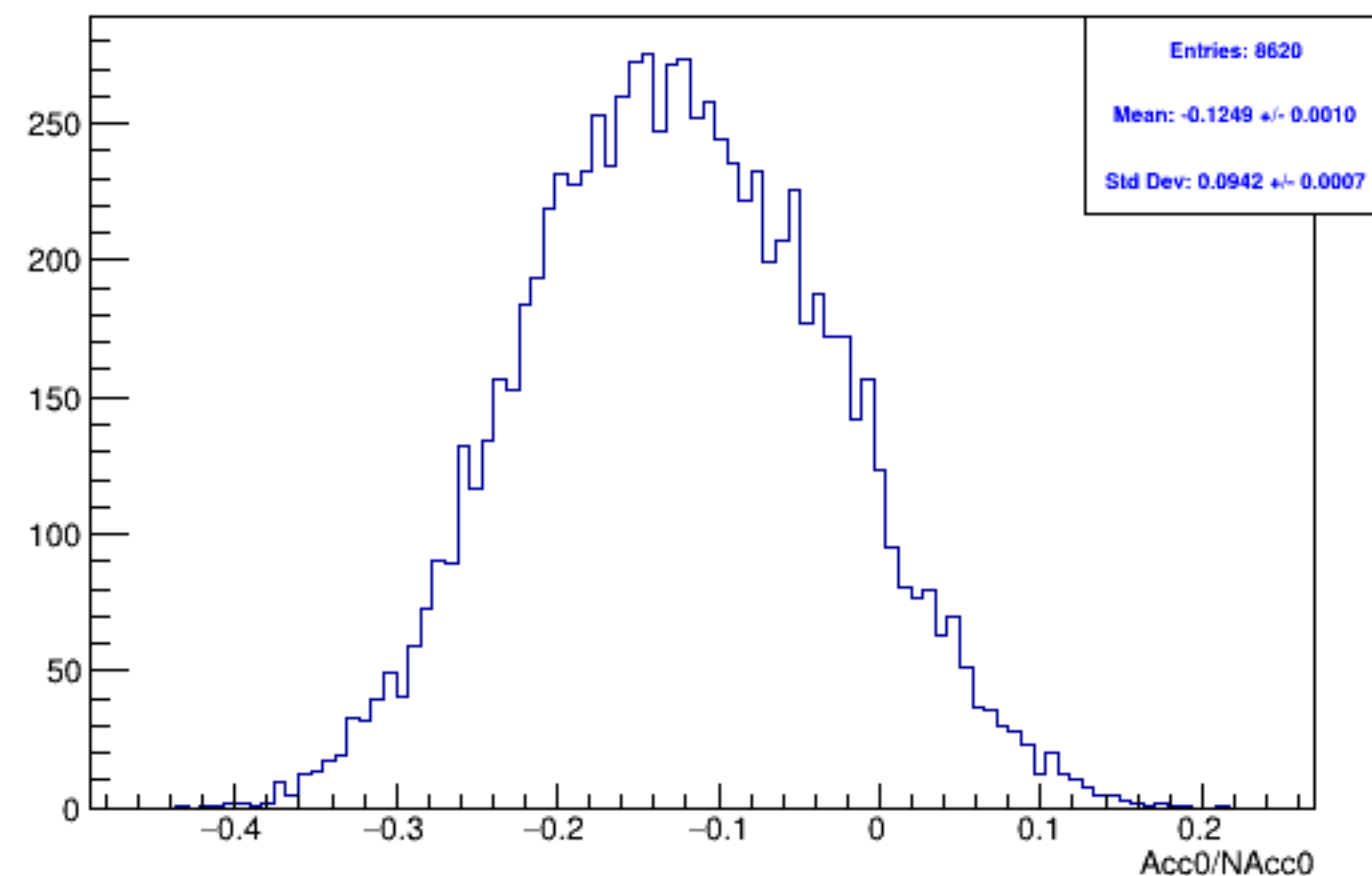
Run 5731 mpwise, acc0: Beam OFF
