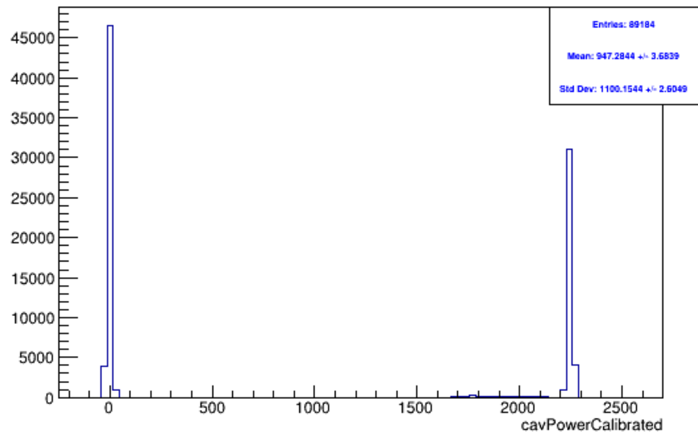
Run 5731 mpwise, lasPow: All
