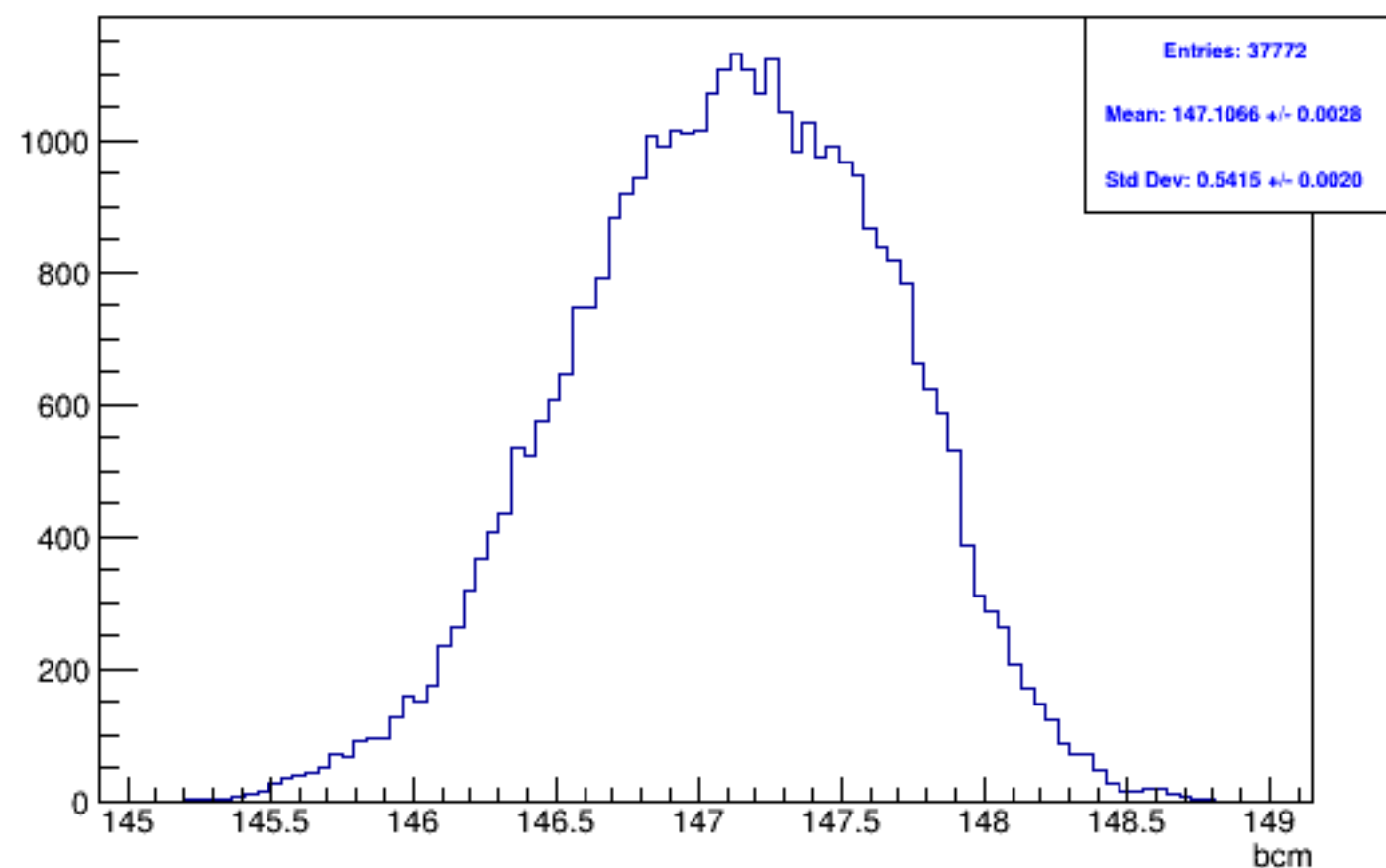
Run 5731, mpwise, BCM: Beam ON, Laser ON
