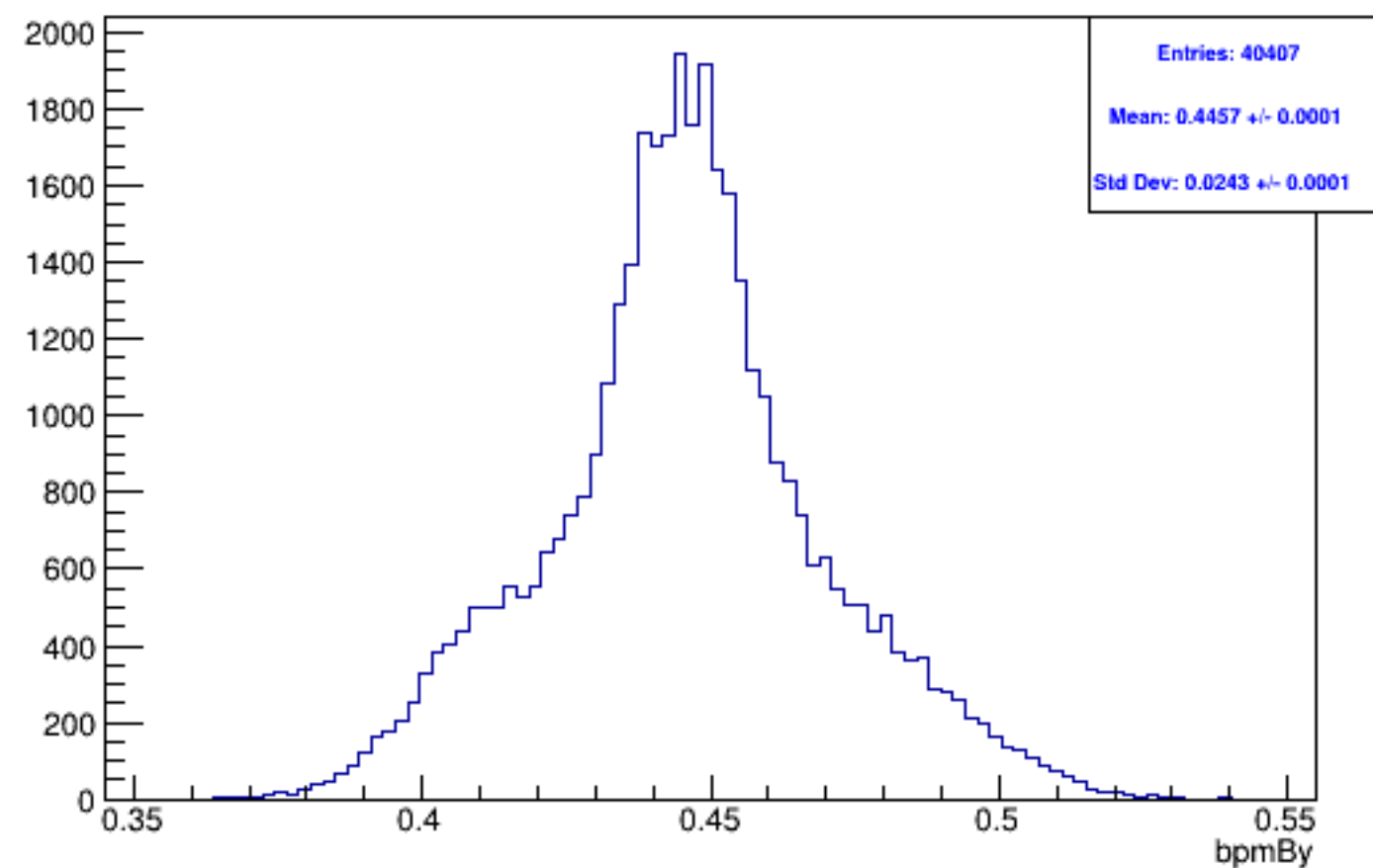
Run 5731, mpswise, bpmBy: Beam ON, Laser OFF
