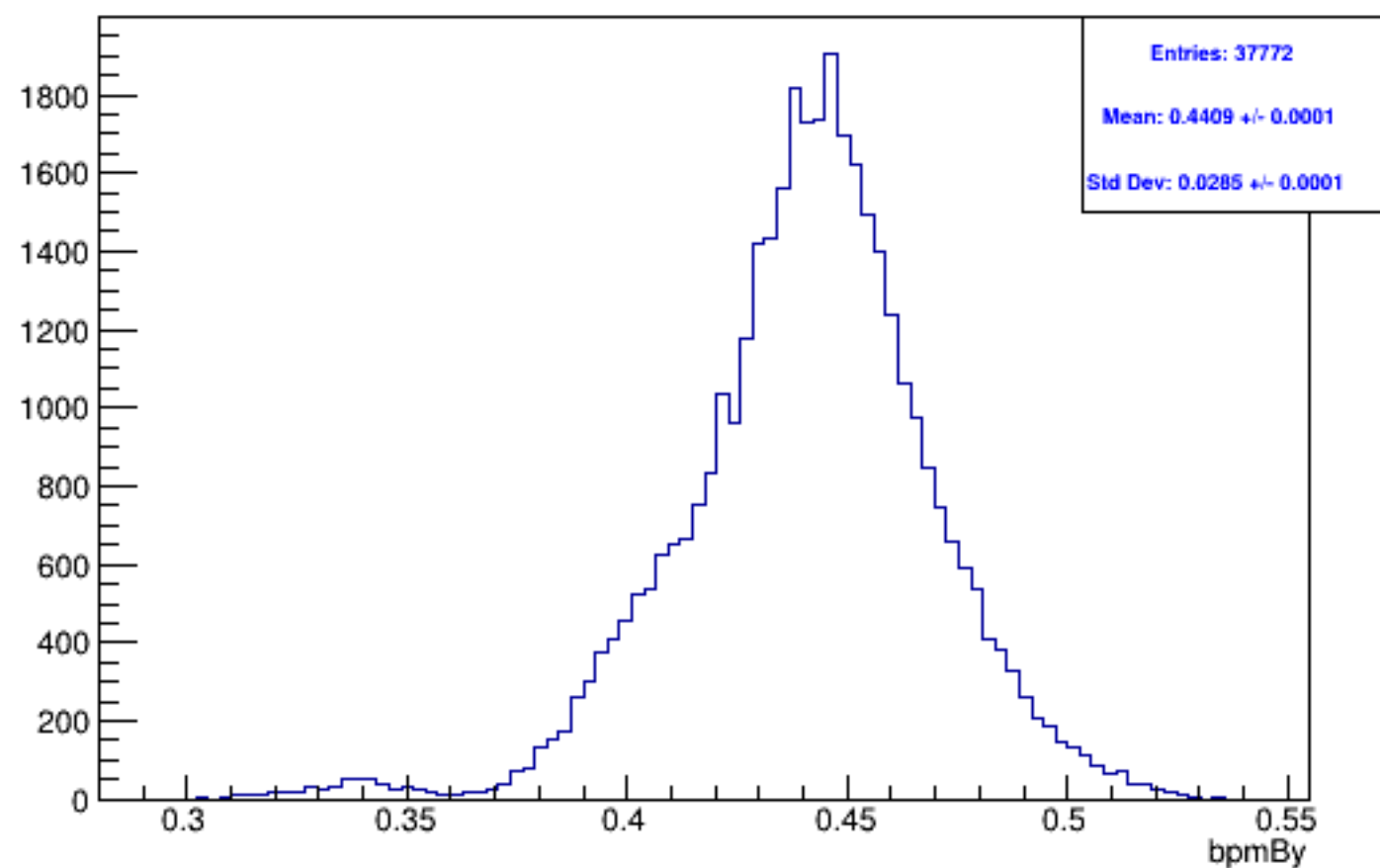
Run 5731, mpswise, bpmBy: Beam ON, Laser ON
