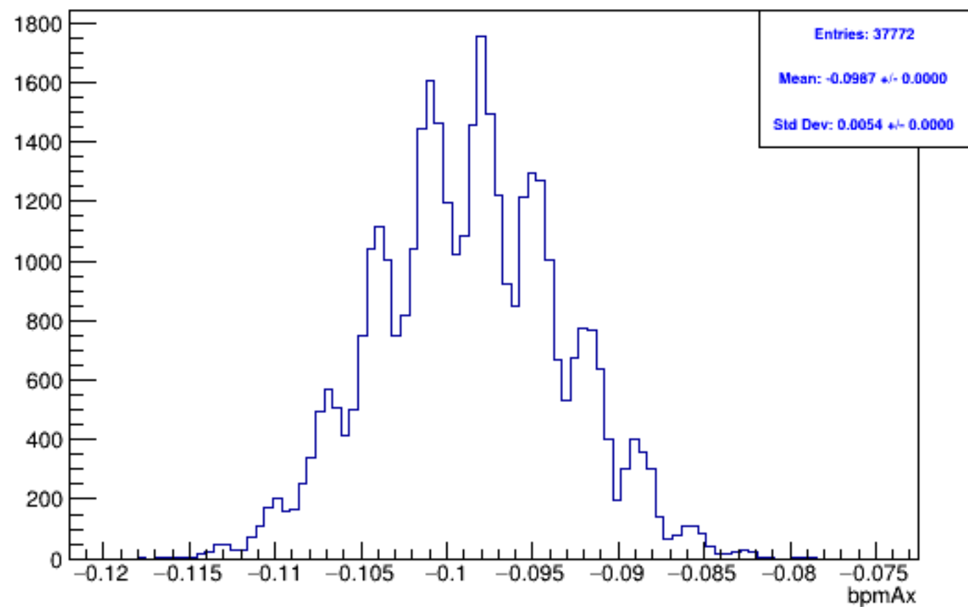
Run 5731, mpwise, bpmAx: Beam ON, Laser ON
