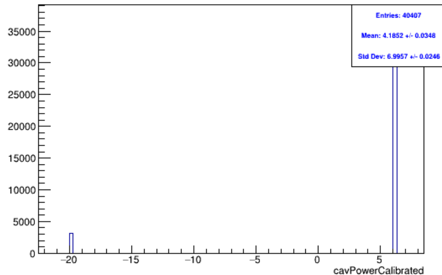
Run 5731, mpwise, lasPow: Beam ON, Laser OFF
