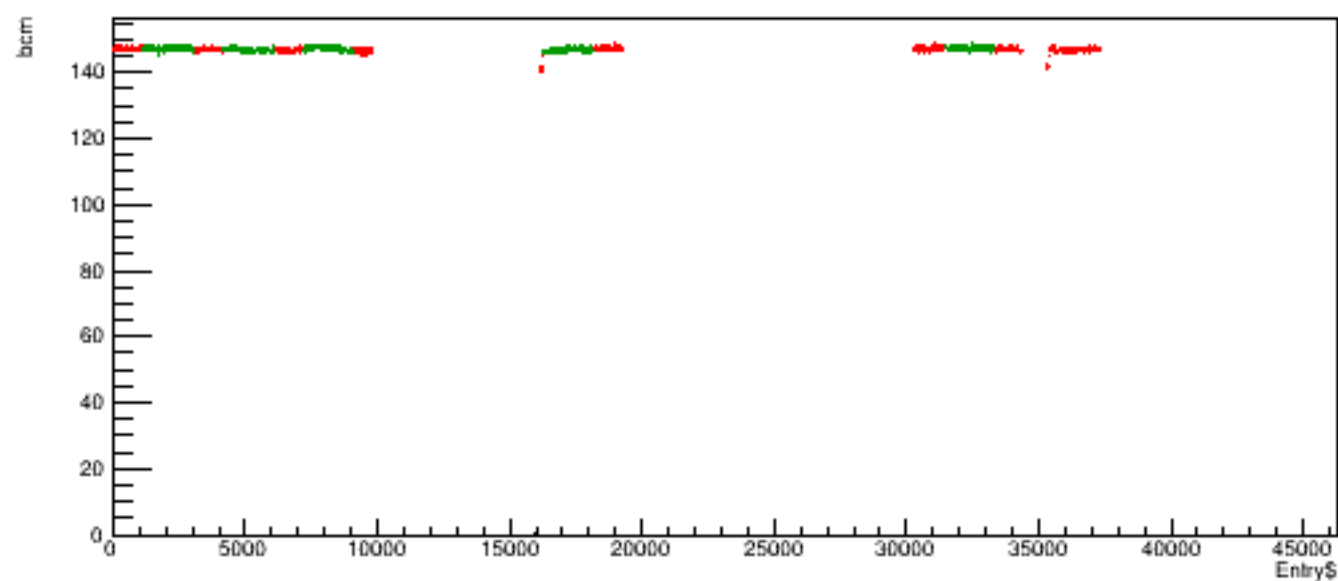
Run 5731 quartetwise, posH4 vs time
