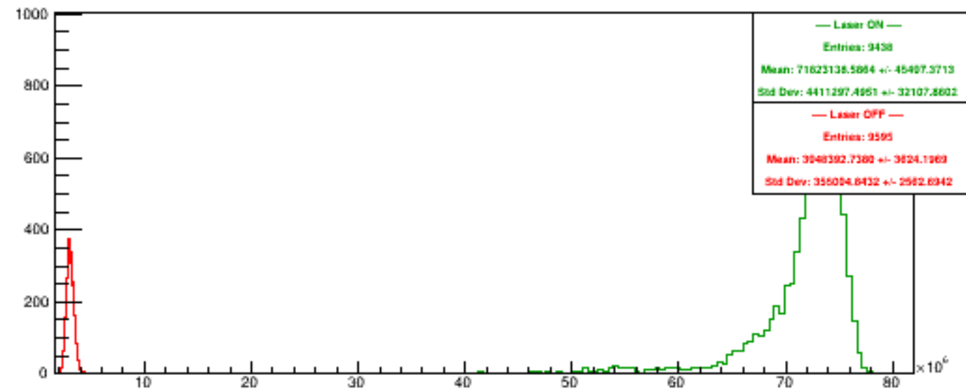
Run 5731 quartetwise, Sums4
