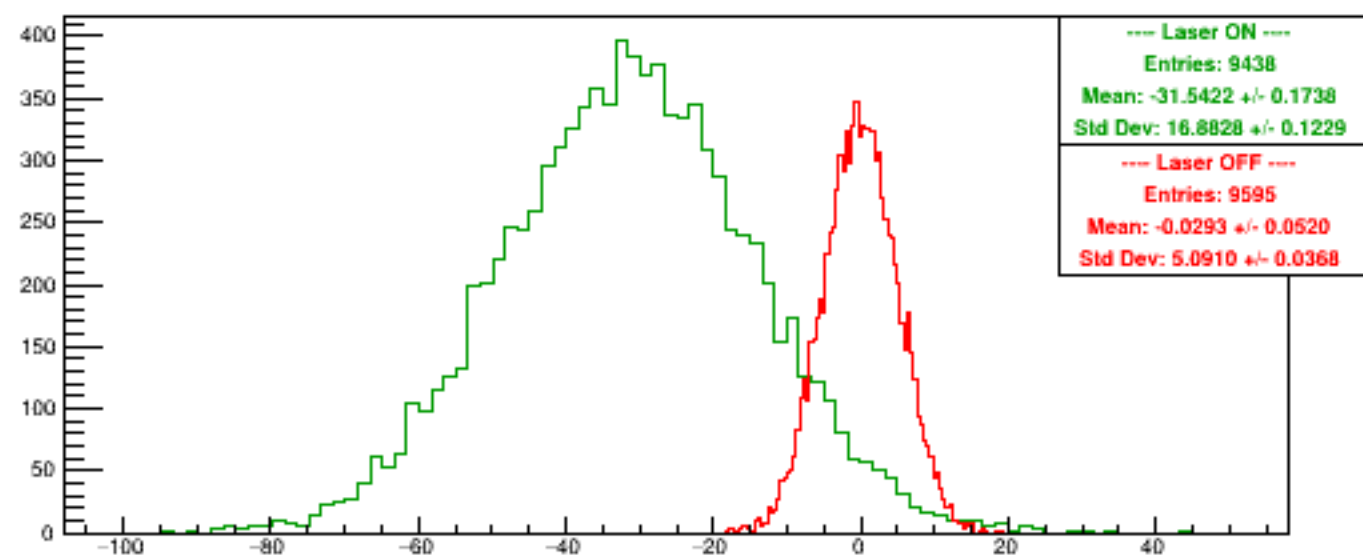
Run 5731 quartetwise, Asyms4
