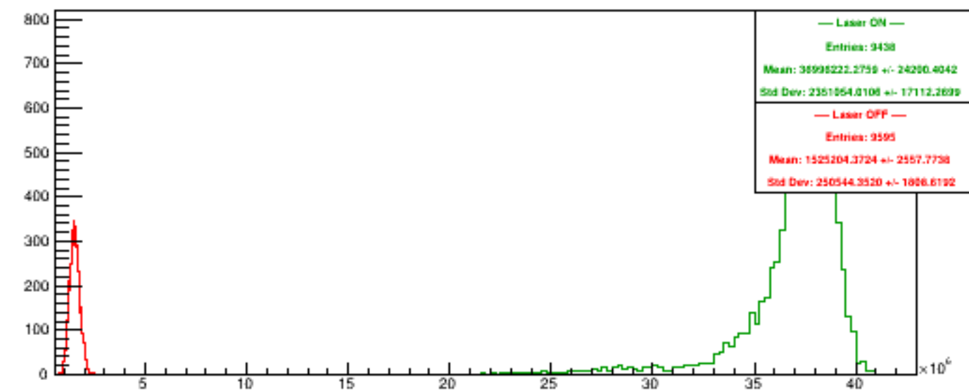
Run 5731 quartetwise, NegHelAcc4
