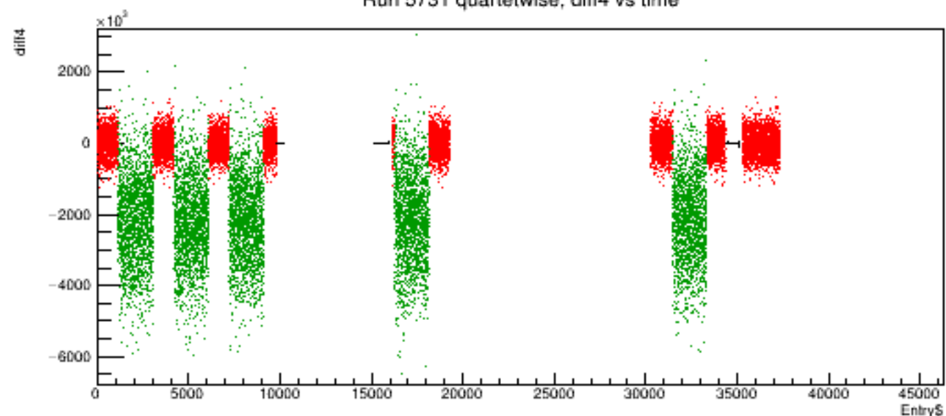
Run 5731 quartetwise, diff4 vs time
