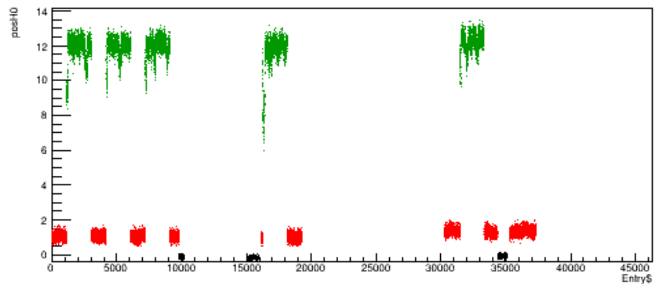
Run 5731 quartetwise, posH0 vs time
