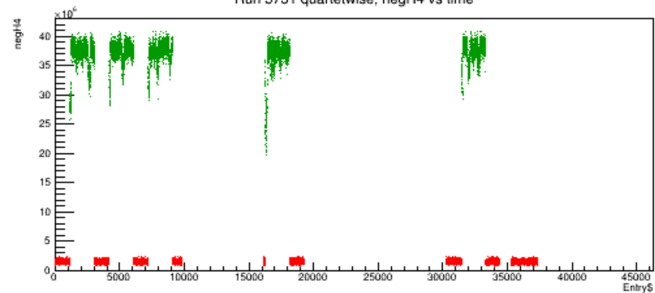
Run 5731 quartetwise, negH4 vs time
