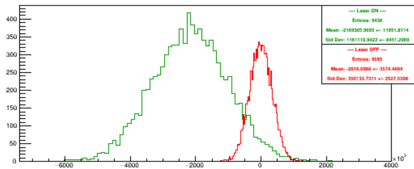
Run 5731 quartetwise, Diffs4
