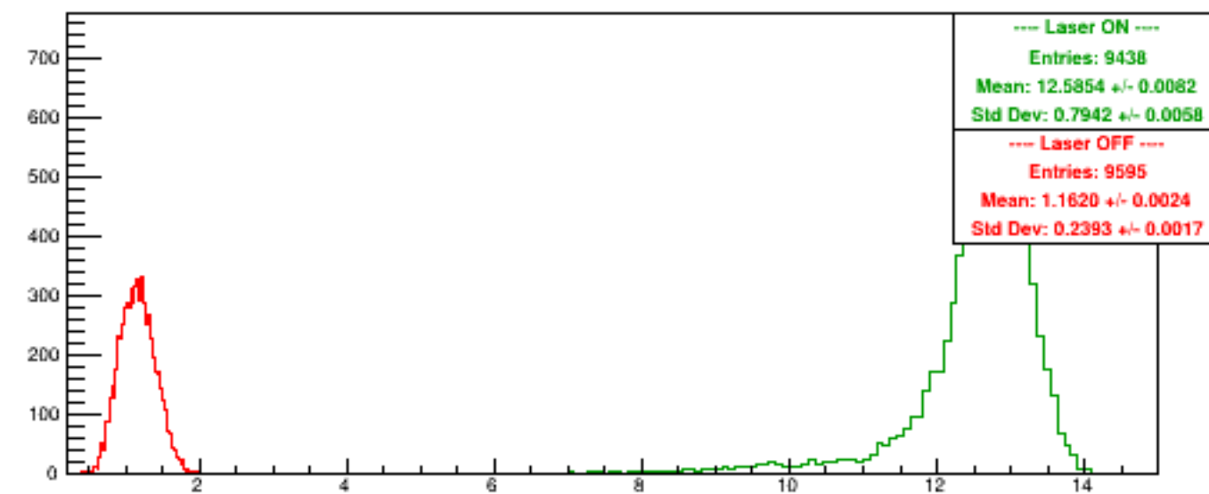
Run 5731 quartetwise, NegHelAcc0/NSamples0
