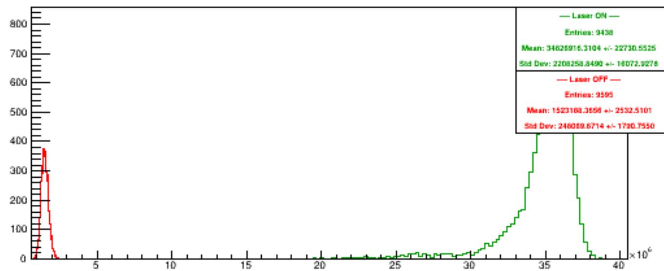
Run 5731 quartetwise, PosHelAcc4
