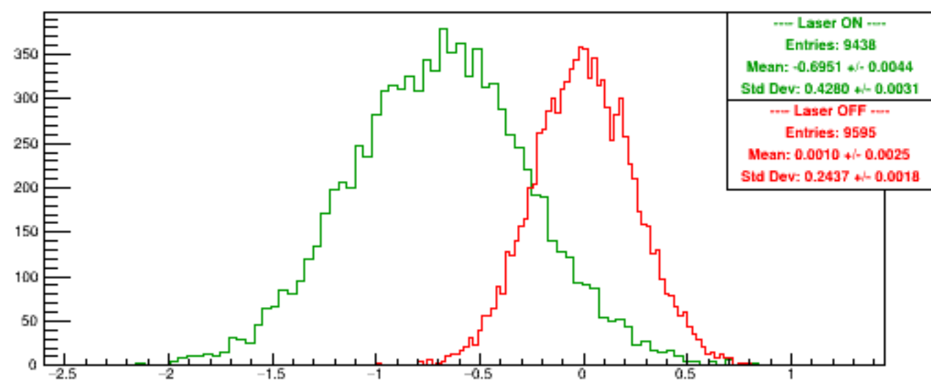
Run 5731 quartetwise, Diffs0
