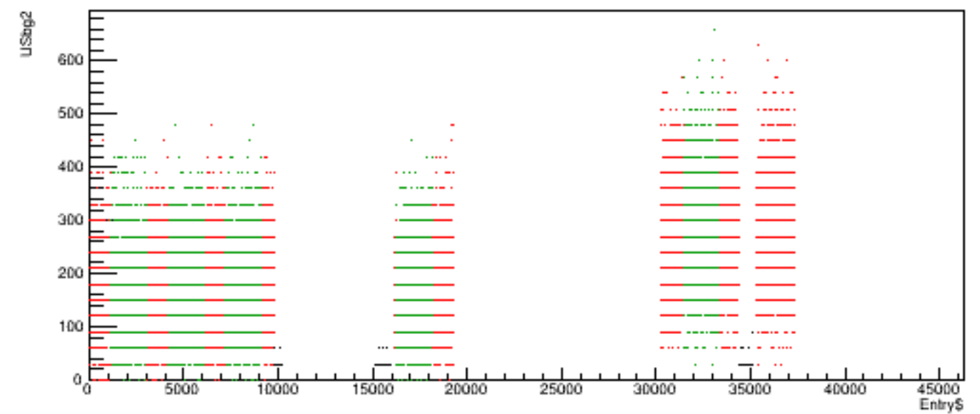
Run 5731 quartetwise, USbg2 vs time
