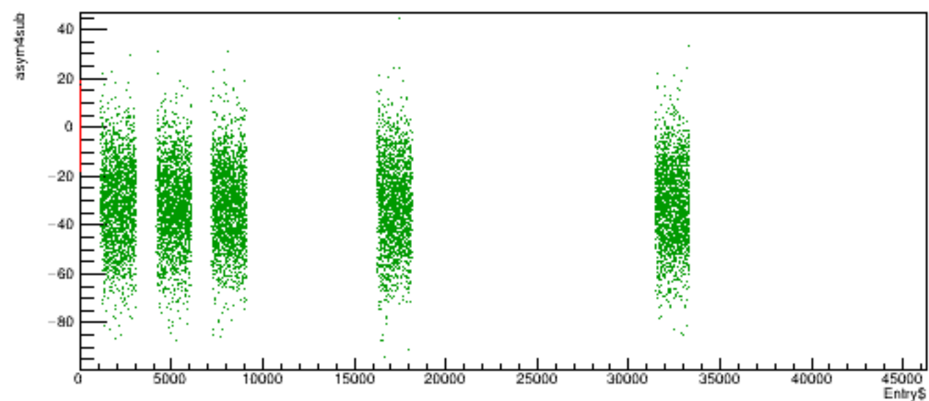
Run 5731 quartetwise, asym4sub vs time
