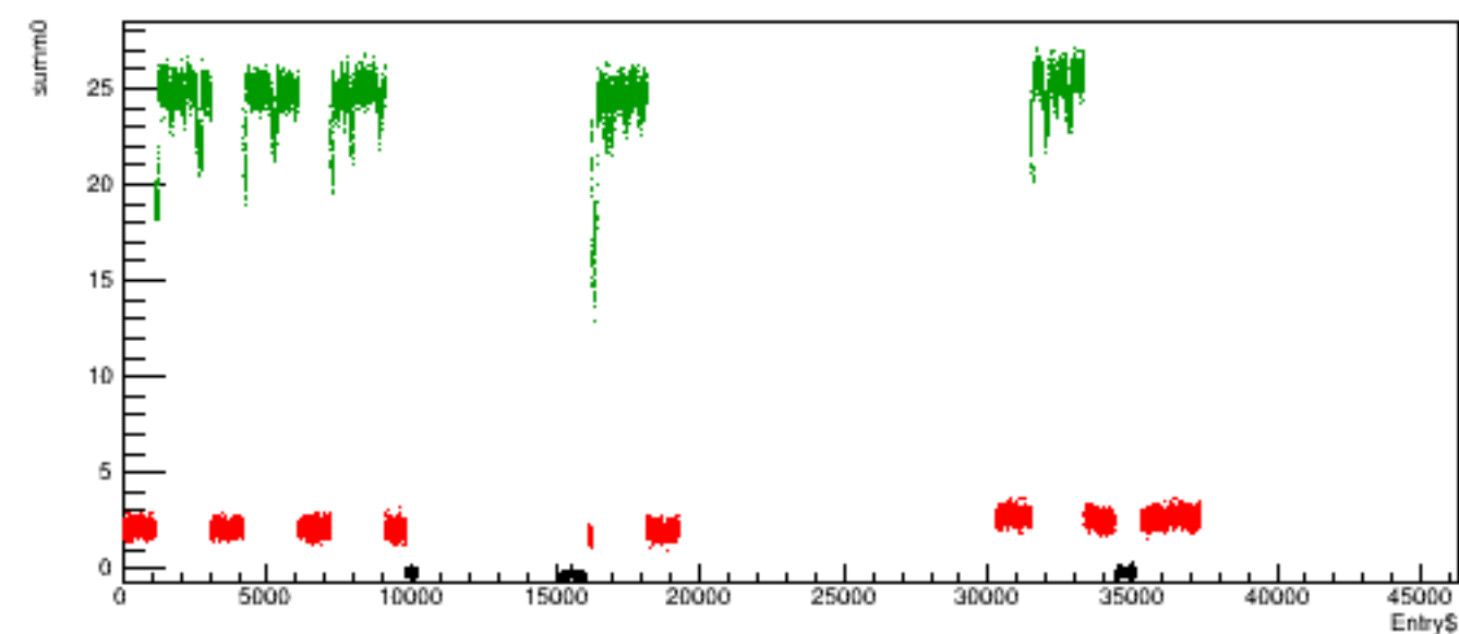
Run 5731 quartetwise, summ0 vs time
