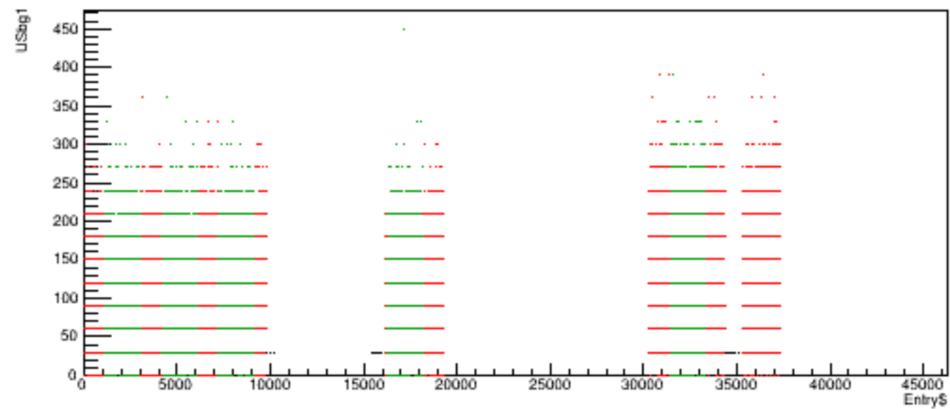
Run 5731 quartetwise, USbg1 vs time
