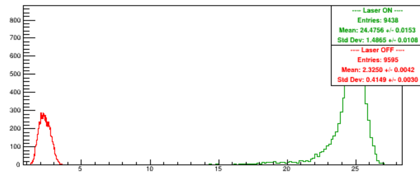
Run 5731 quartetwise, Sums0
