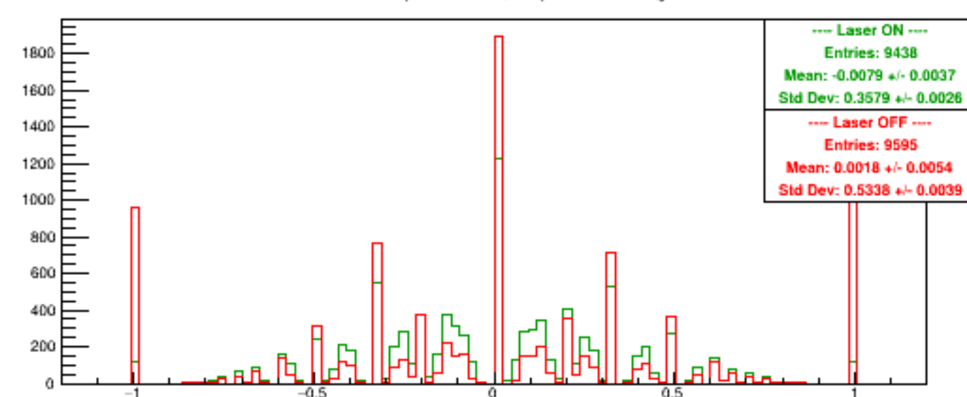
Run 5731 quartetwise, Asyms Vert Finger
