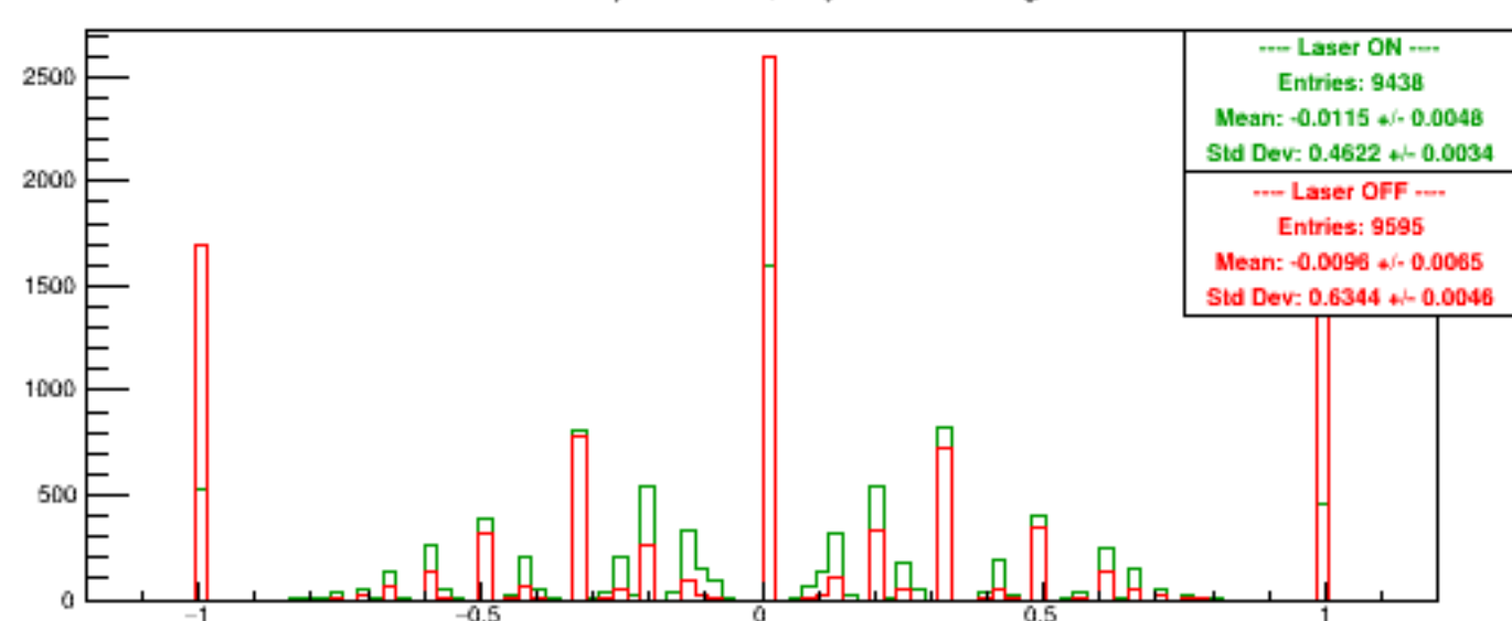
Run 5731 quartetwise, Asyms Horiz Finger
