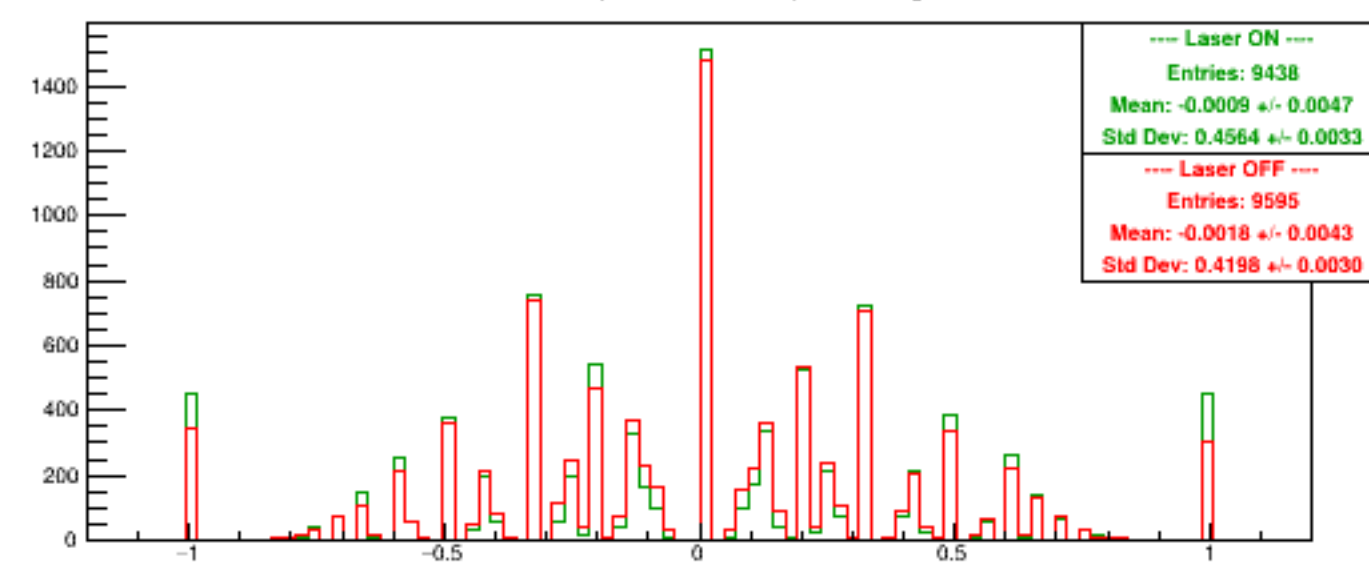
Run 5731 quartetwise, Asyms USbg2
