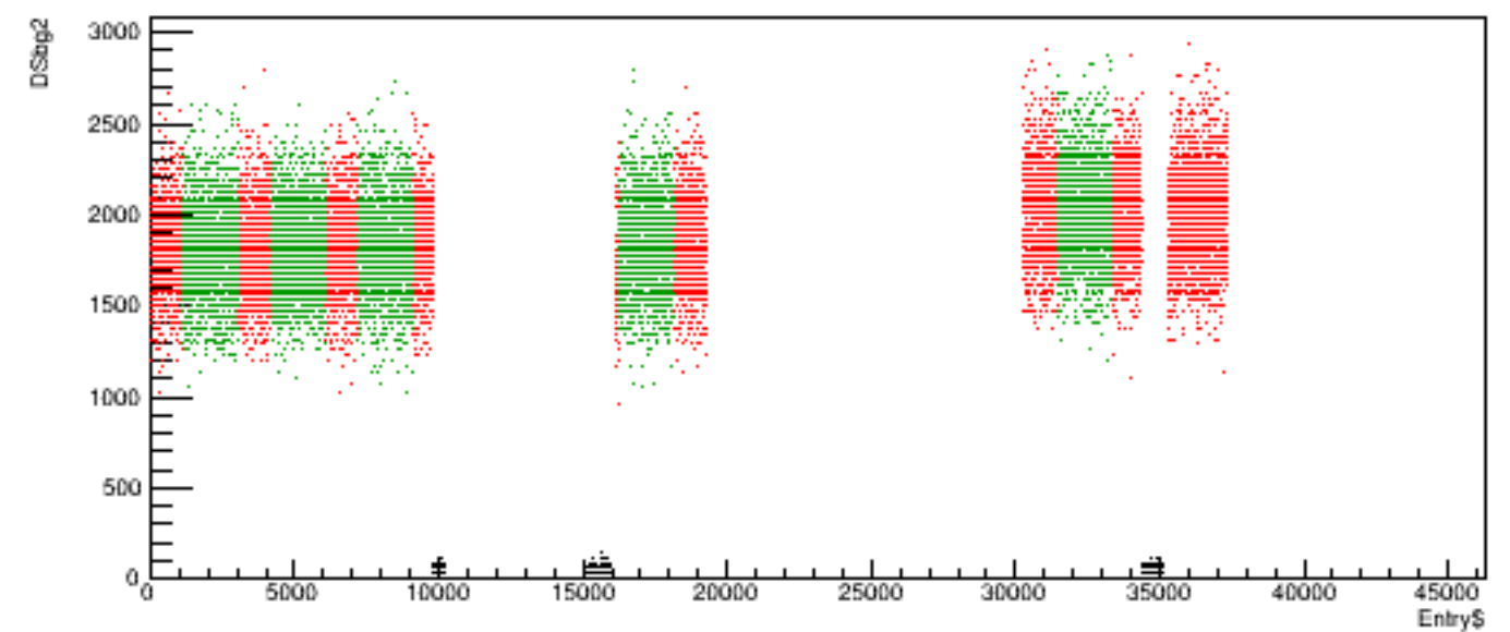
Run 5731 quartetwise, DSbg2 vs time
