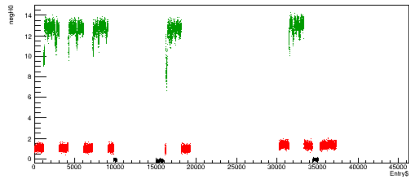
Run 5731 quartetwise, negH0 vs time
