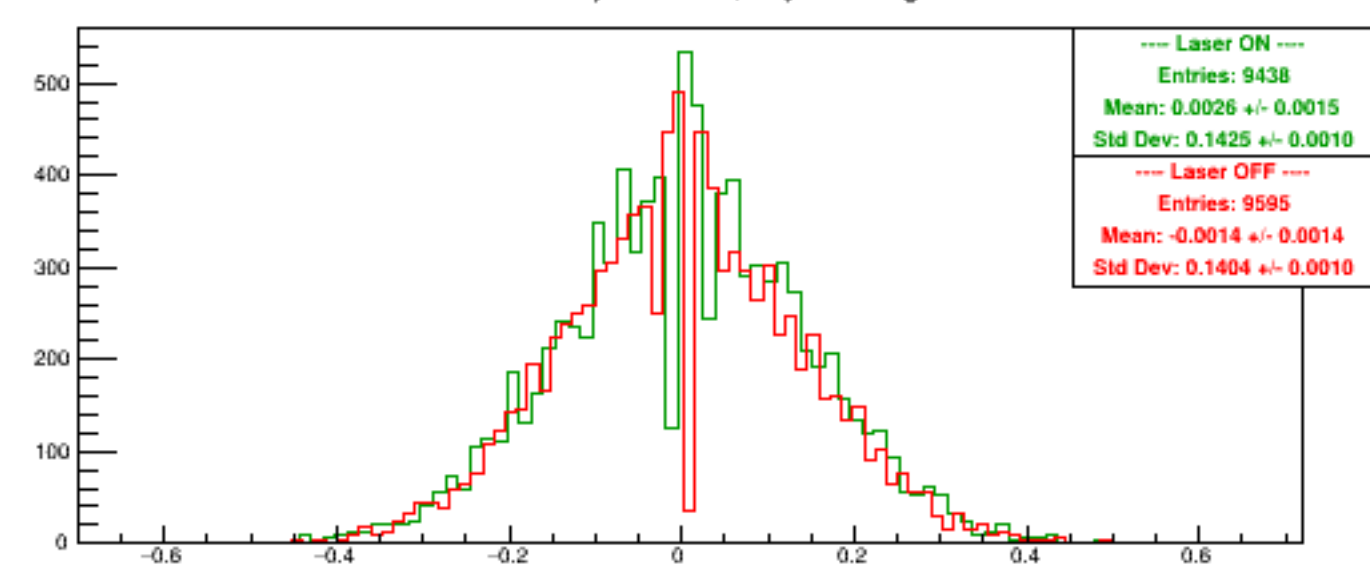
Run 5731 quartetwise, Asyms DSbg1
