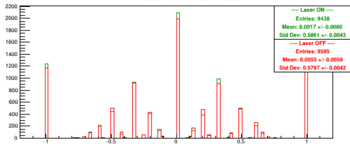
Run 5731 quartetwise, Asyms USbg1
