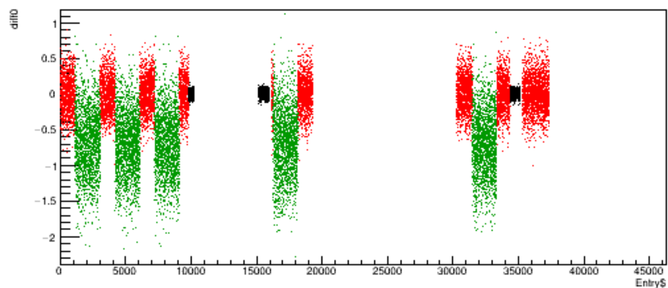
Run 5731 quartetwise, diff0 vs time
