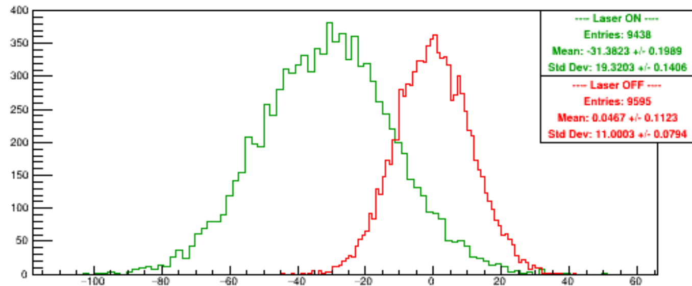
Run 5731 quartetwise, Asyms0
