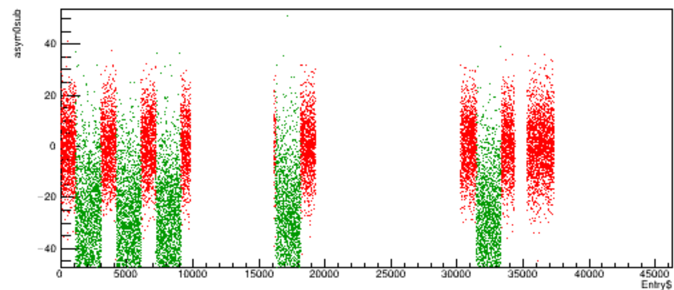
Run 5731 quartetwise, asym0sub vs time
