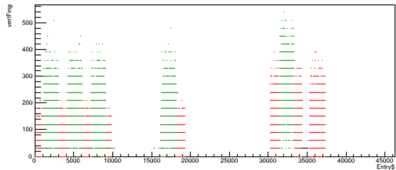
Run 5731 quartetwise, vertFing vs time
