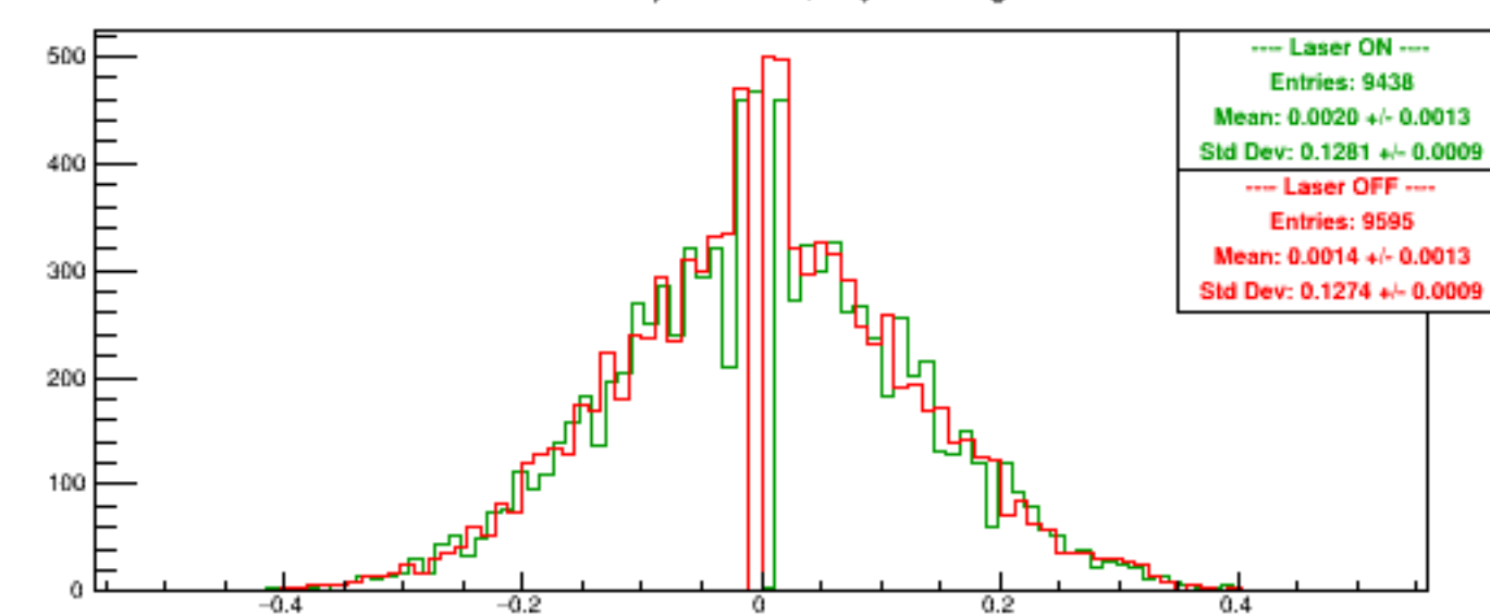
Run 5731 quartetwise, Asyms DSbg2
