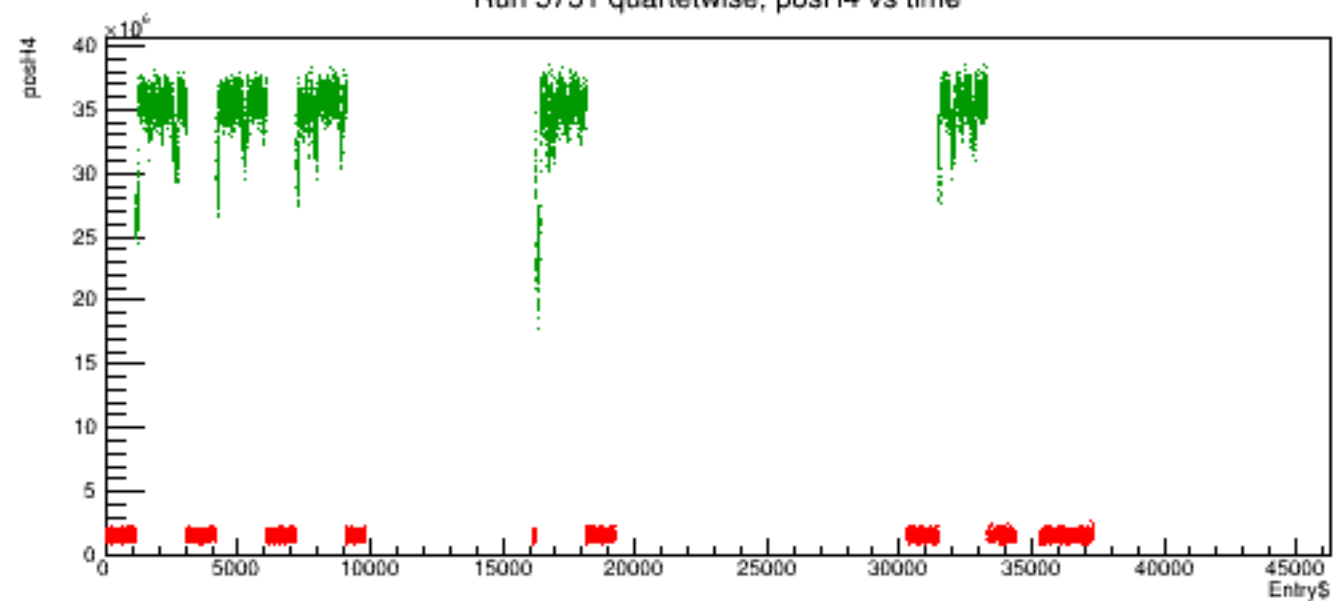
Run 5731 quartetwise, posH4 vs time
