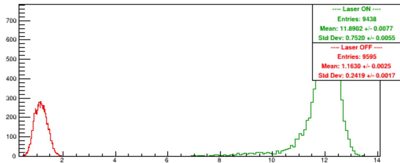
Run 5731 quartetwise, PosHelAcc0/NSamples0
