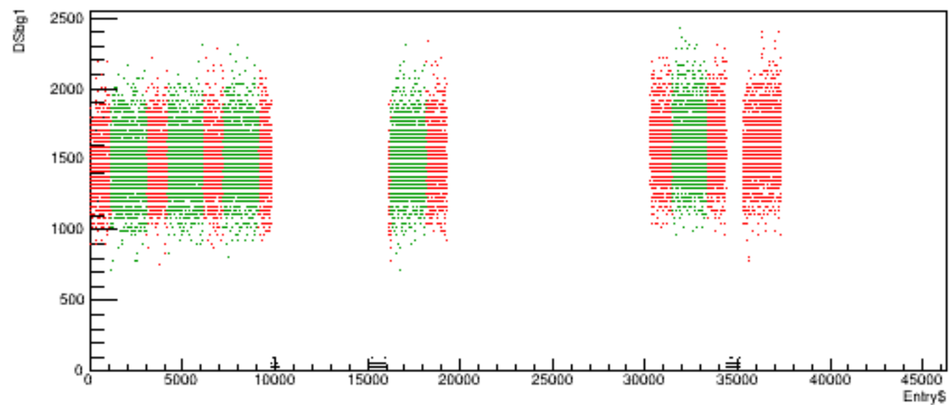
Run 5731 quartetwise, DSbg1 vs time
