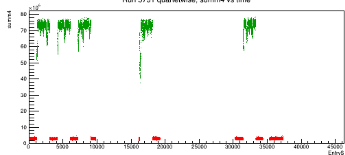
Run 5731 quartetwise, summ4 vs time
