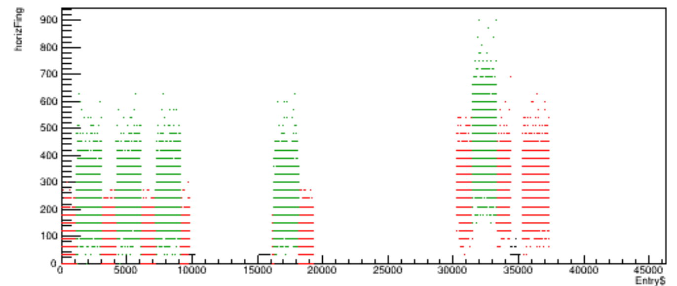
Run 5731 quartetwise, horizFing vs time
