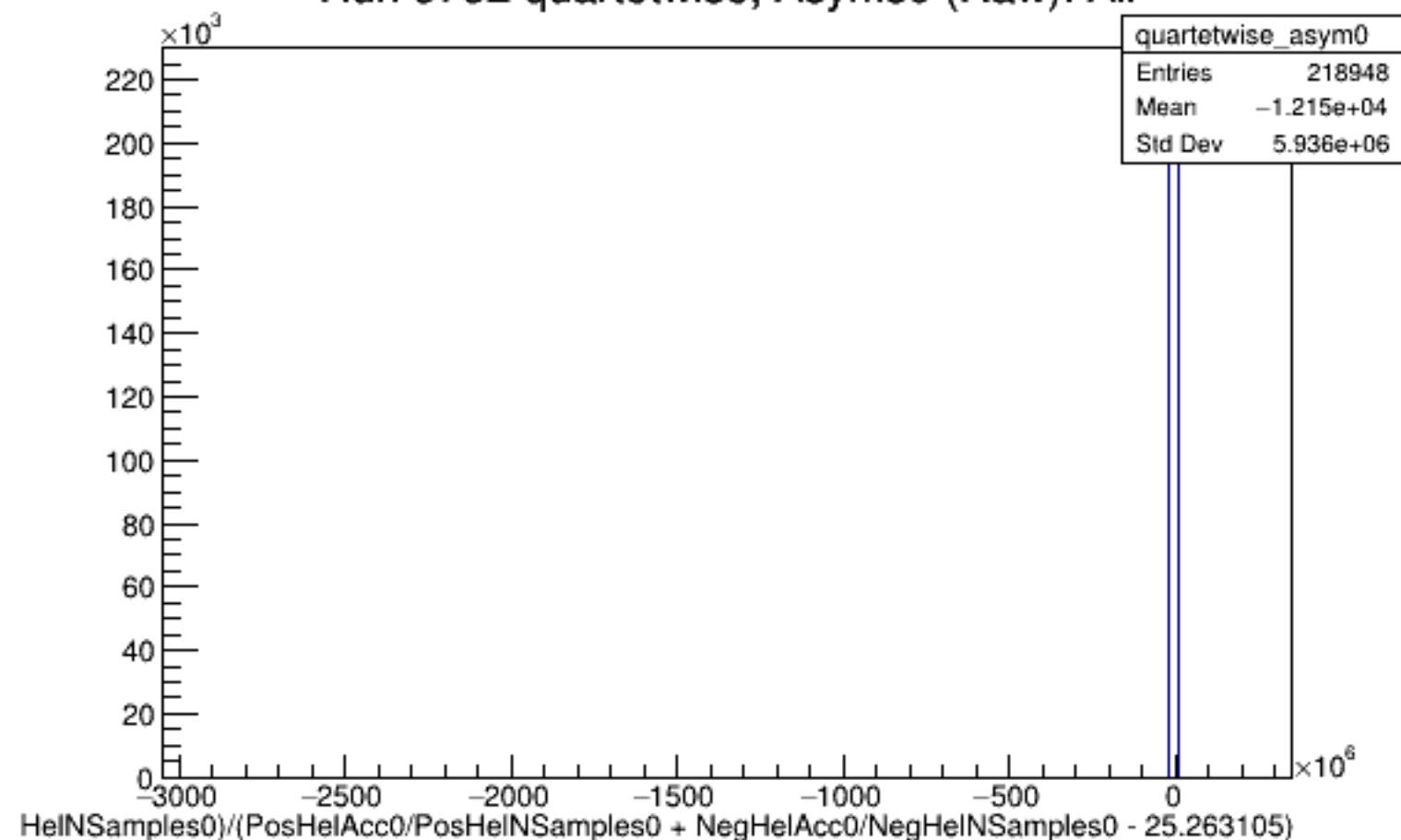
Run 5732 quartetwise, Asyms0 (Raw): All
