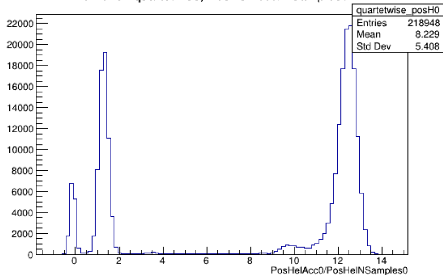
Run 5732 quartetwise, PosHelAcc0/NSamples0: All
