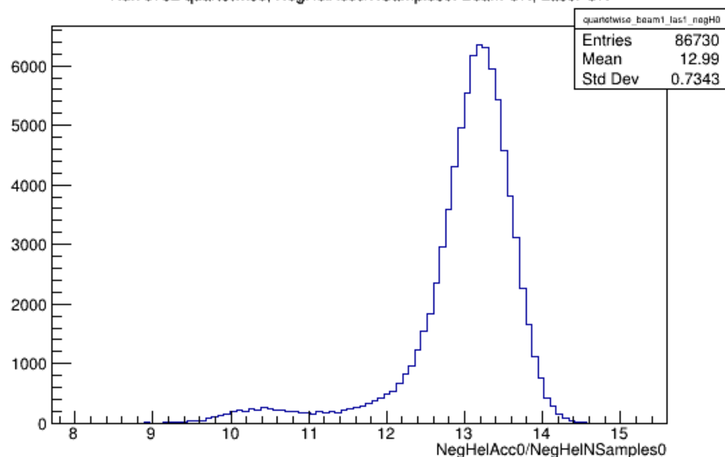
Run 5732 quartetwise, NegHelAcc0/NSamples0: Beam ON, Laser ON
