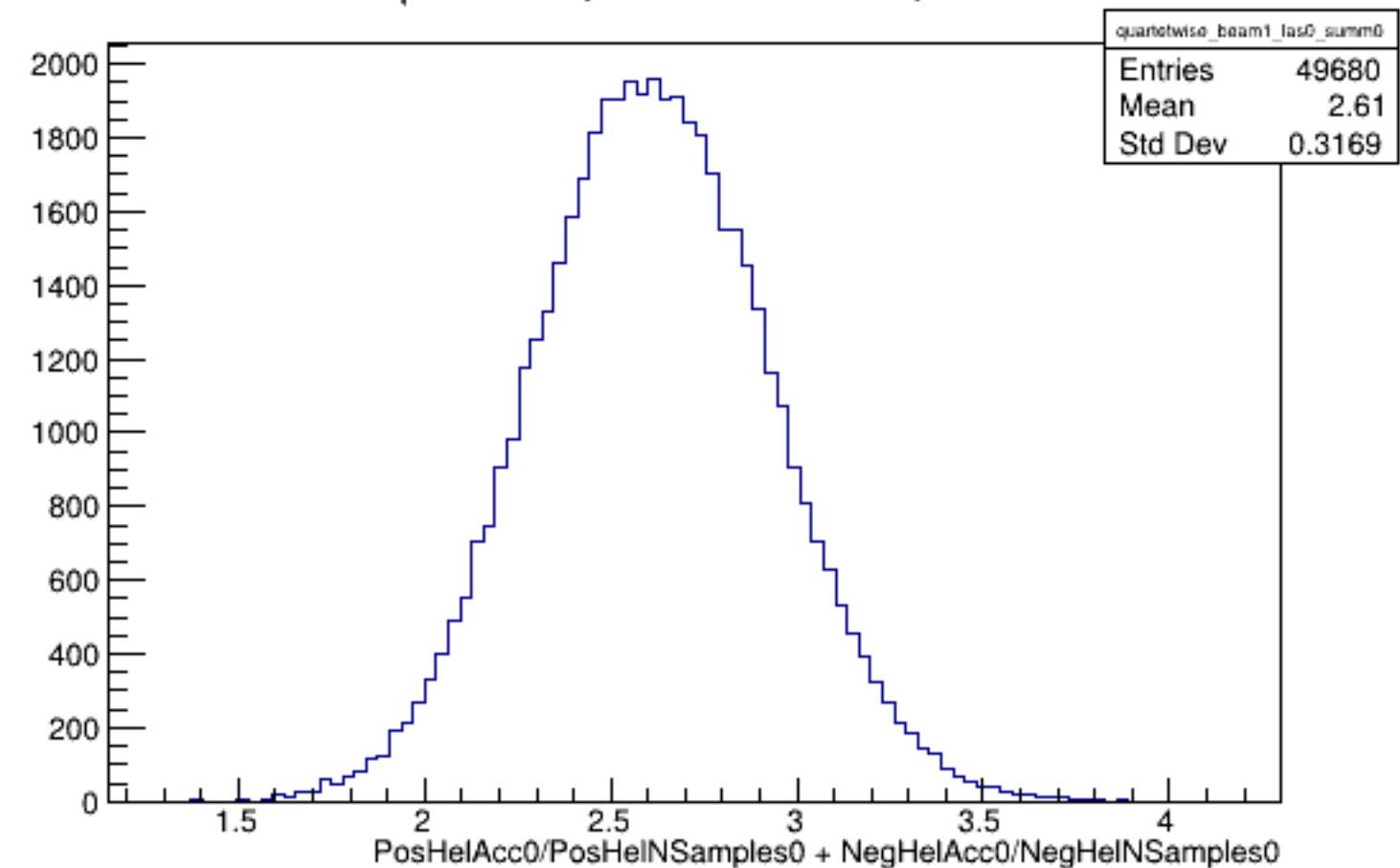
Run 5732 quartetwise, Sums0: Beam ON, Laser OFF
