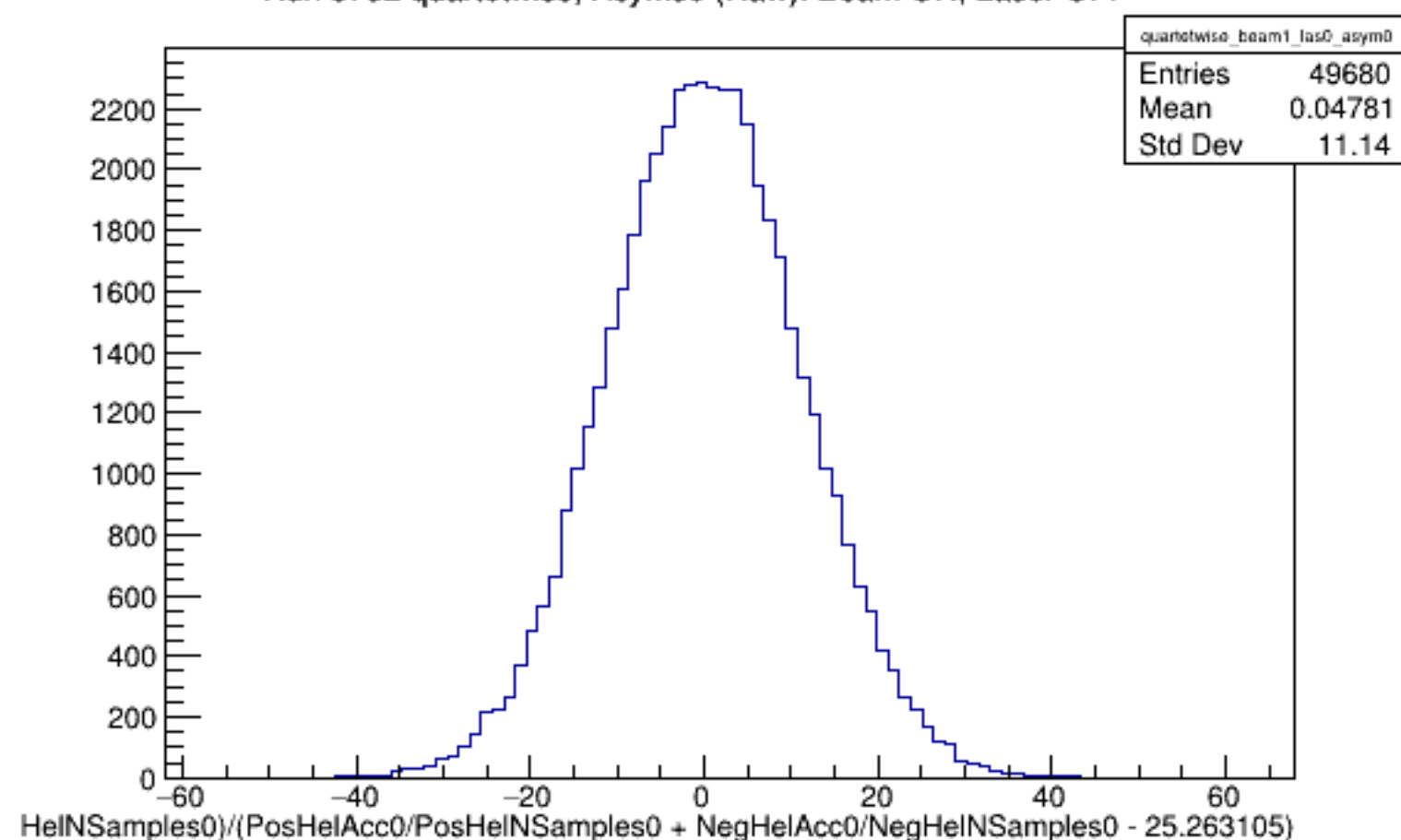
Run 5732 quartetwise, Asyms0 (Raw): Beam ON, Laser OFF
