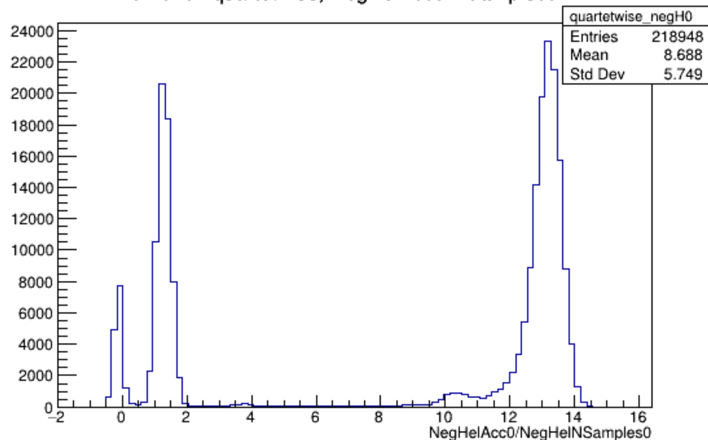
Run 5732 quartetwise, NegHelAcc0/NSamples0: All
