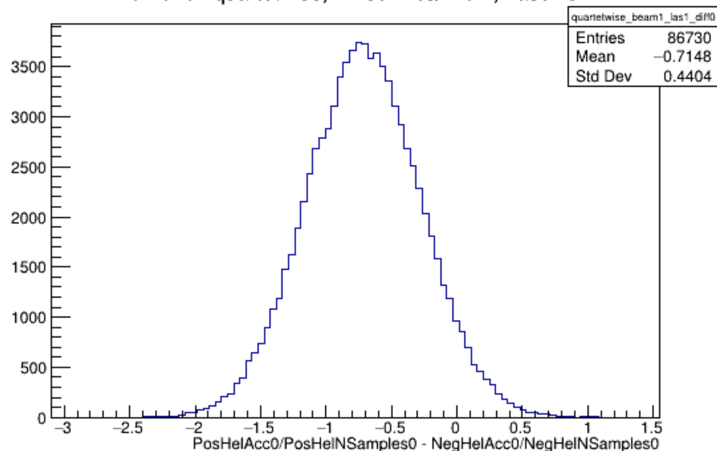
Run 5732 quartetwise, Diffs0: Beam ON, Laser ON
