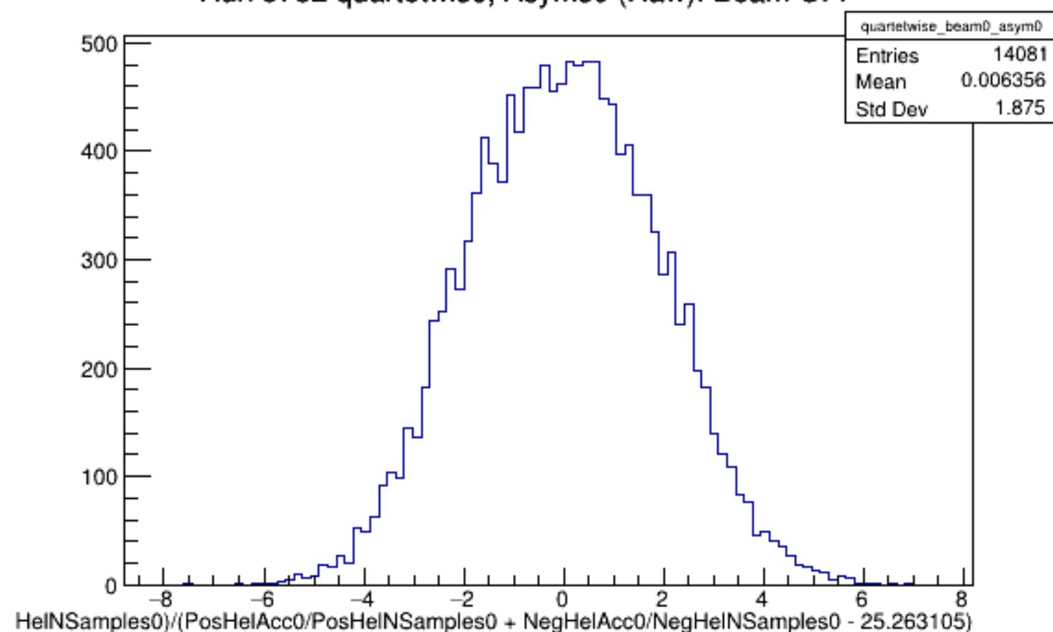
Run 5732 quartetwise, Asyms0 (Raw): Beam OFF
