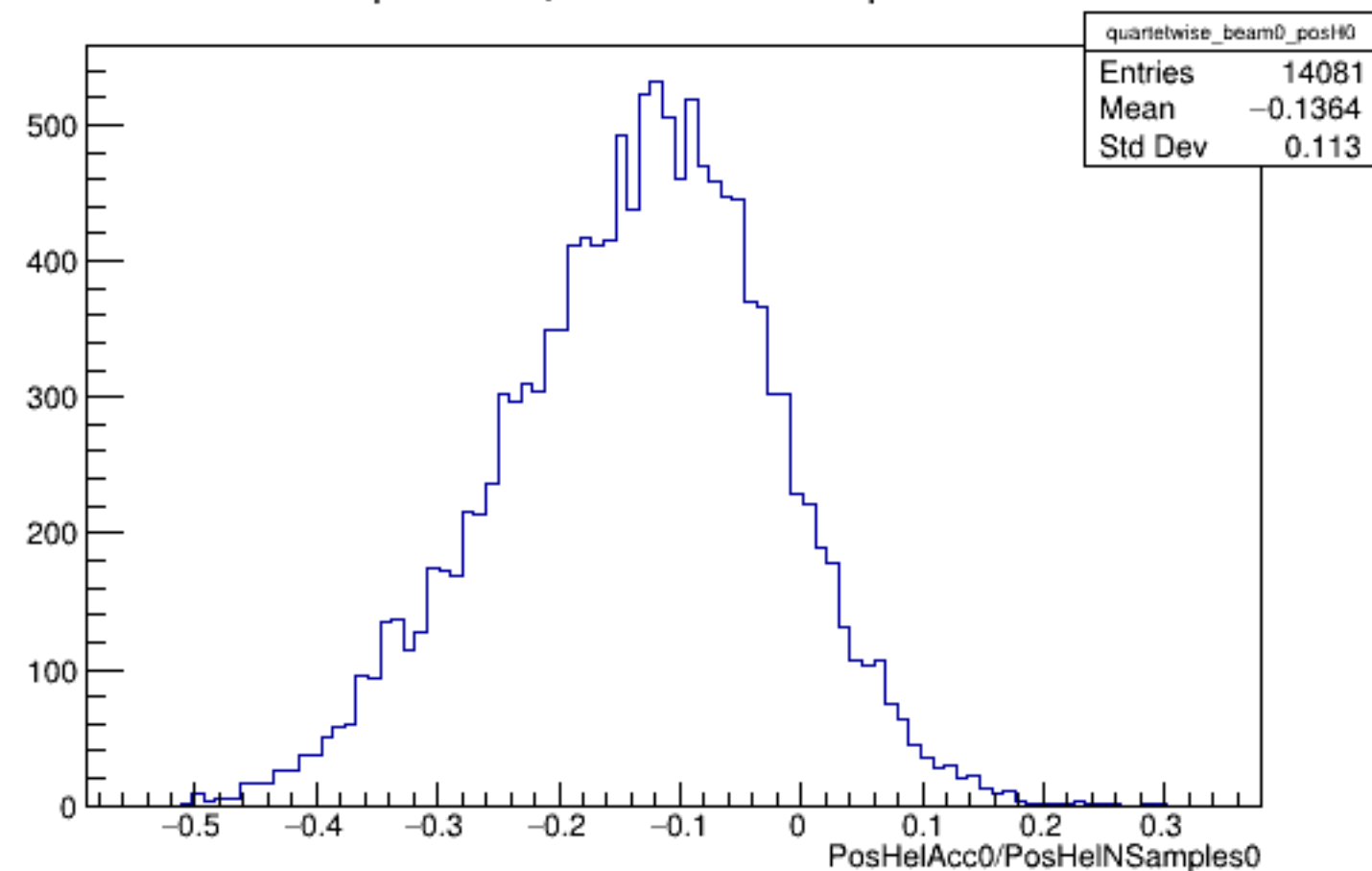
Run 5732 quartetwise, PosHelAcc0/NSamples0: Beam OFF
