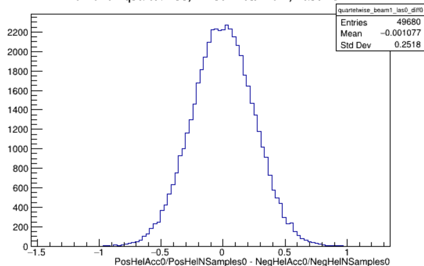
Run 5732 quartetwise, Diffs0: Beam ON, Laser OFF
