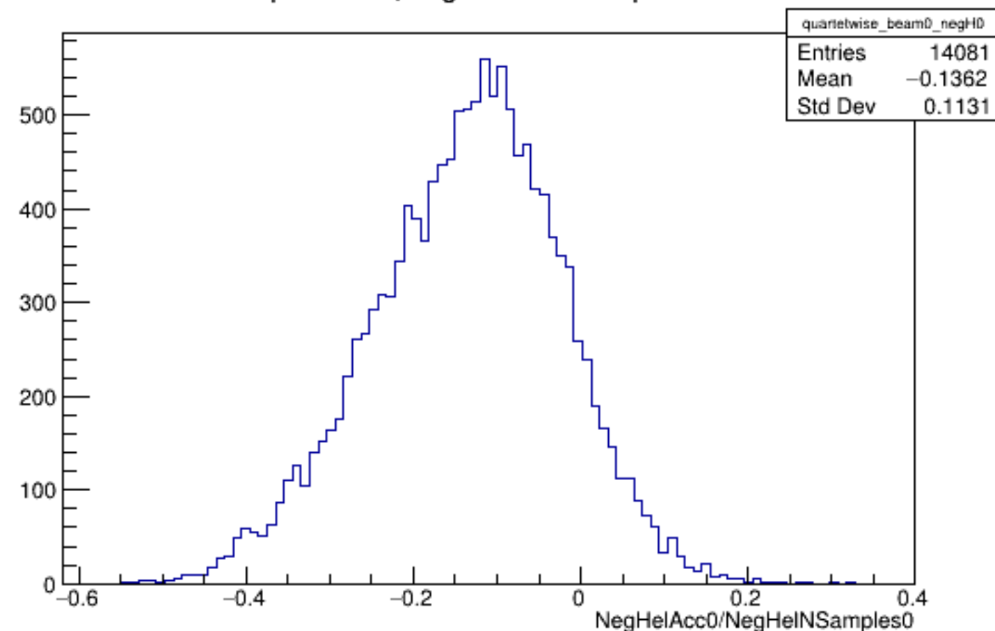
Run 5732 quartetwise, NegHelAcc0/NSamples0: Beam OFF
