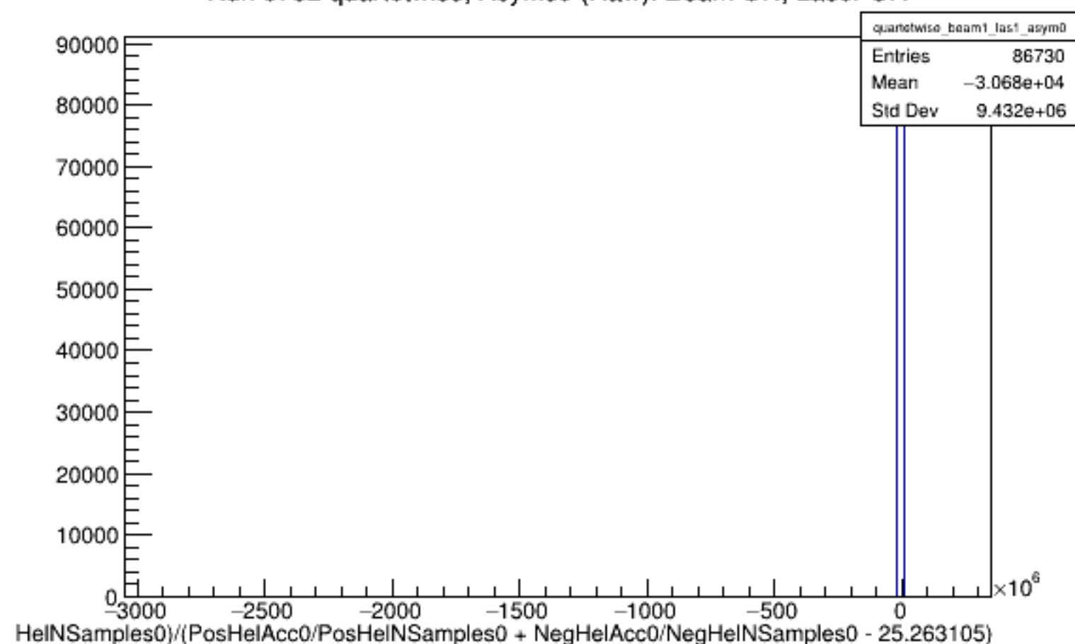
Run 5732 quartetwise, Asyms0 (Raw): Beam ON, Laser ON
