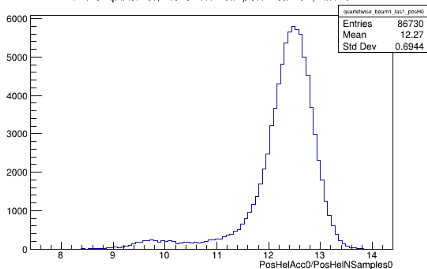
Run 5732 quartetwise, PosHelAcc0/NSamples0: Beam ON, Laser ON
