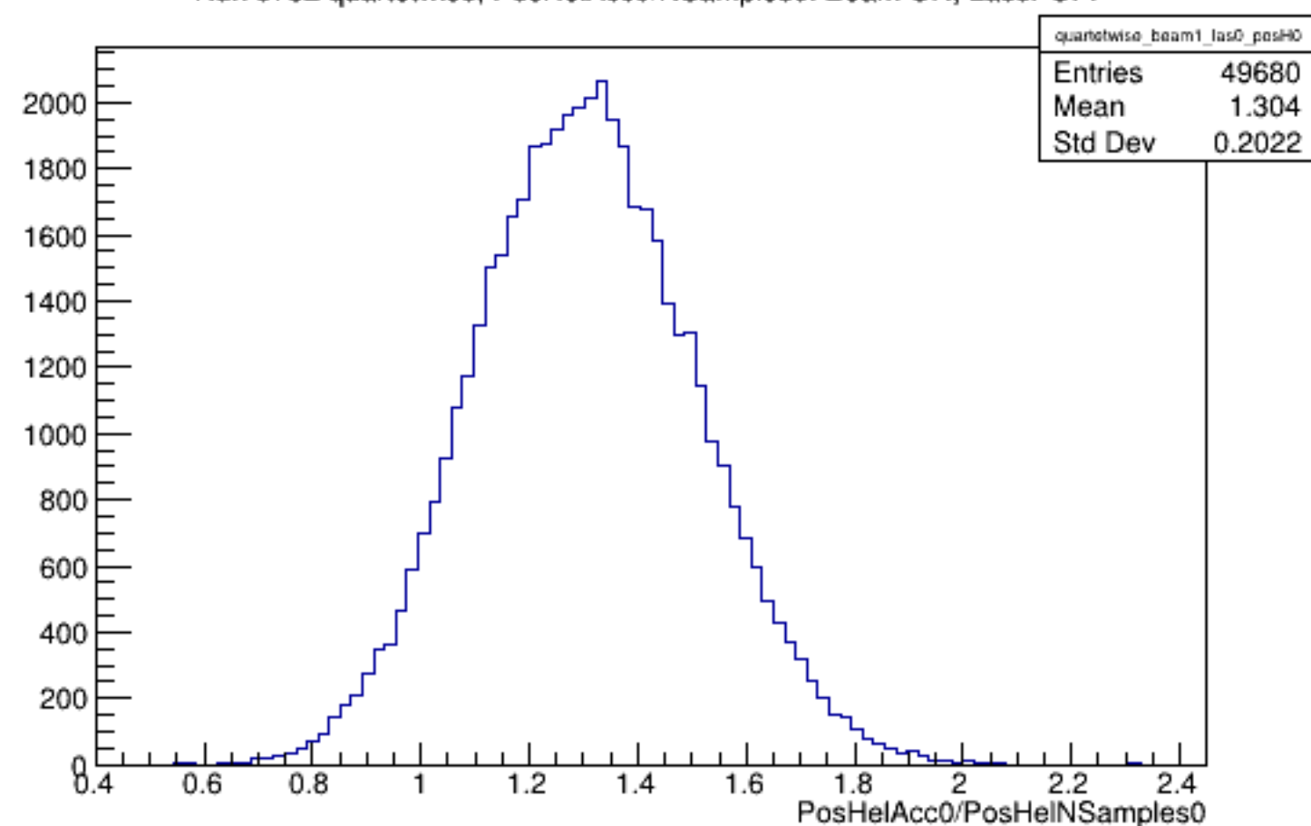
Run 5732 quartetwise, PosHelAcc0/NSamples0: Beam ON, Laser OFF
