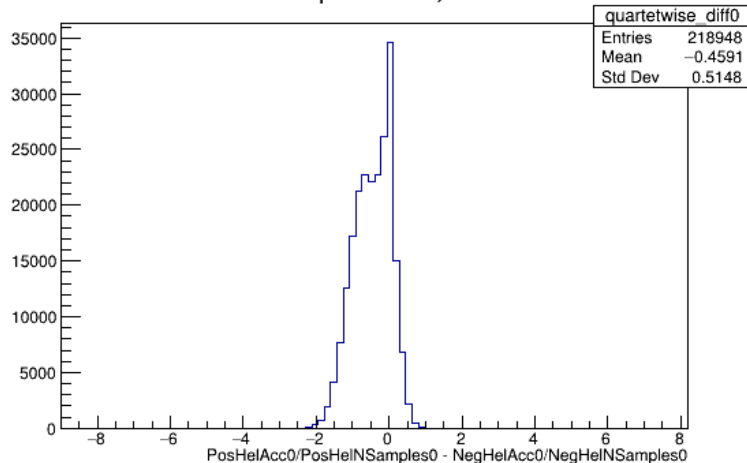
Run 5732 quartetwise, Diffs0: All
