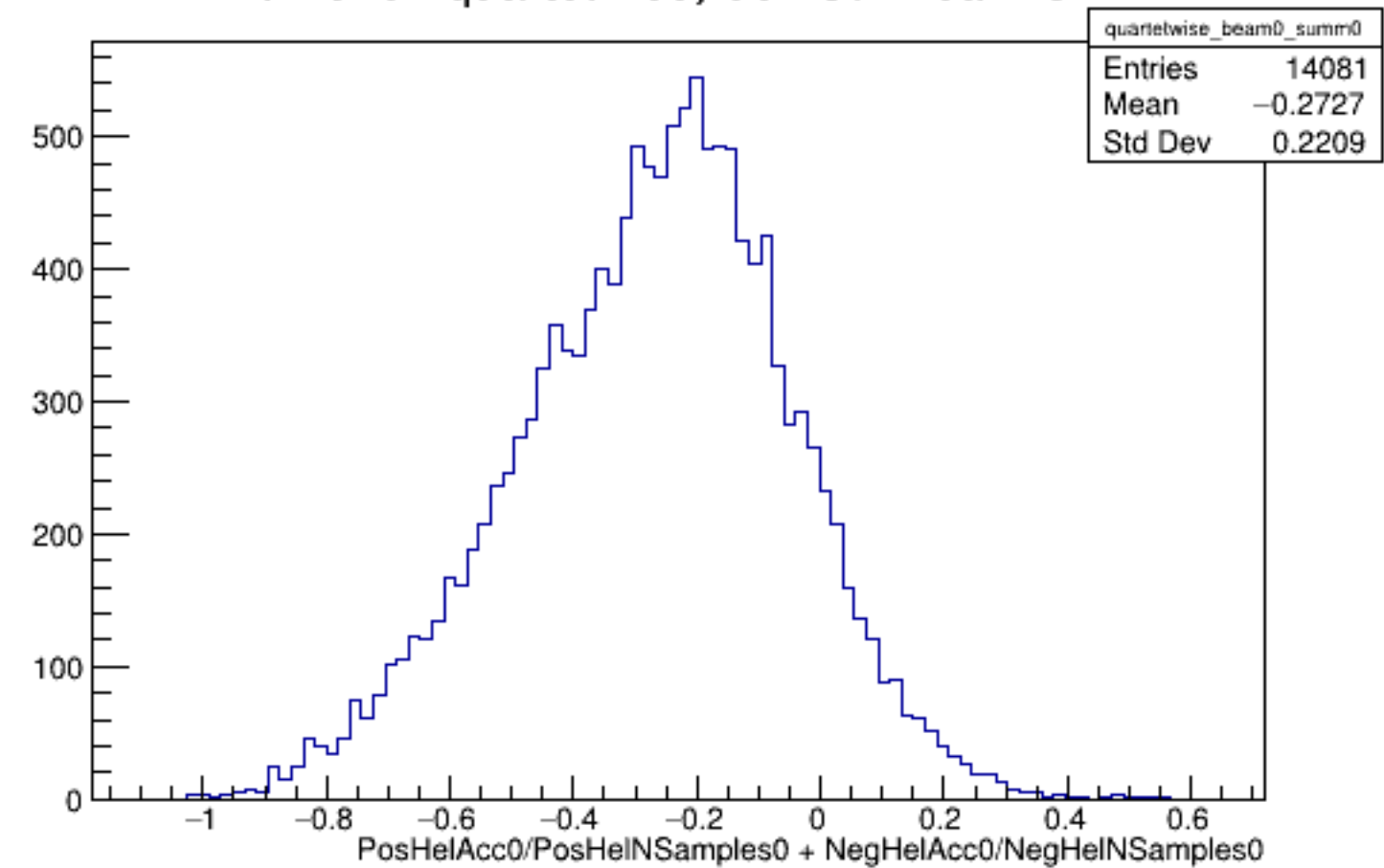
Run 5732 quartetwise, Sums0: Beam OFF
