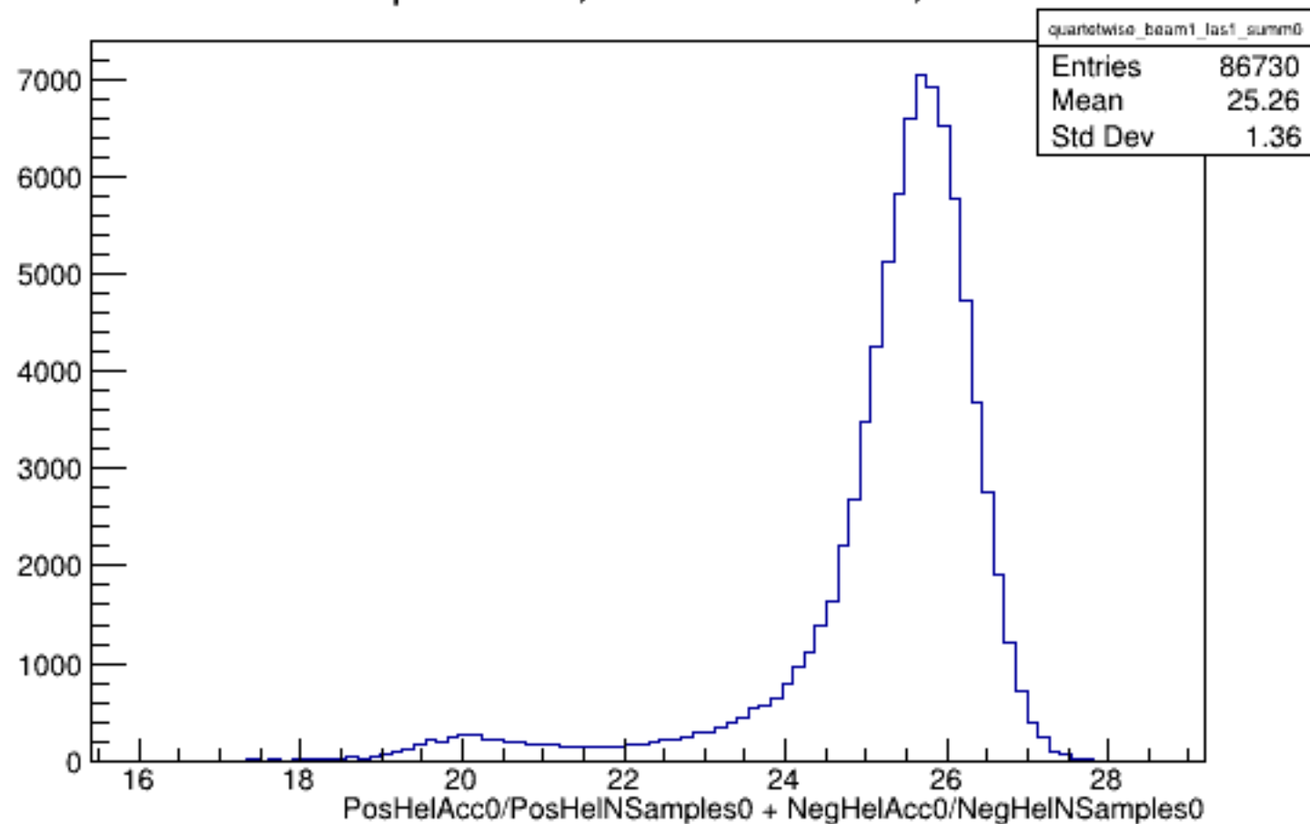
Run 5732 quartetwise, Sums0: Beam ON, Laser ON
