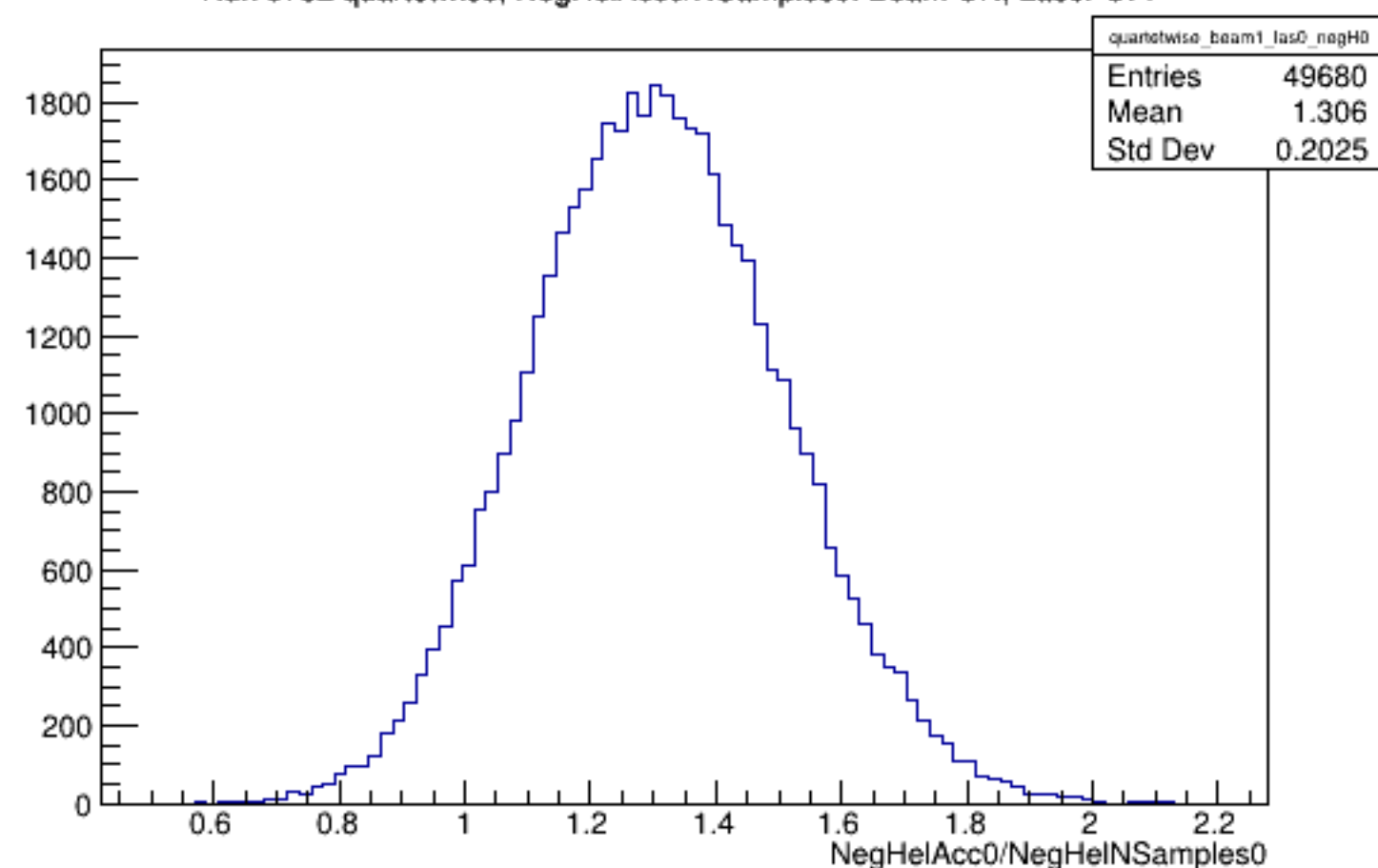
Run 5732 quartetwise, NegHelAcc0/NSamples0: Beam ON, Laser OFF
