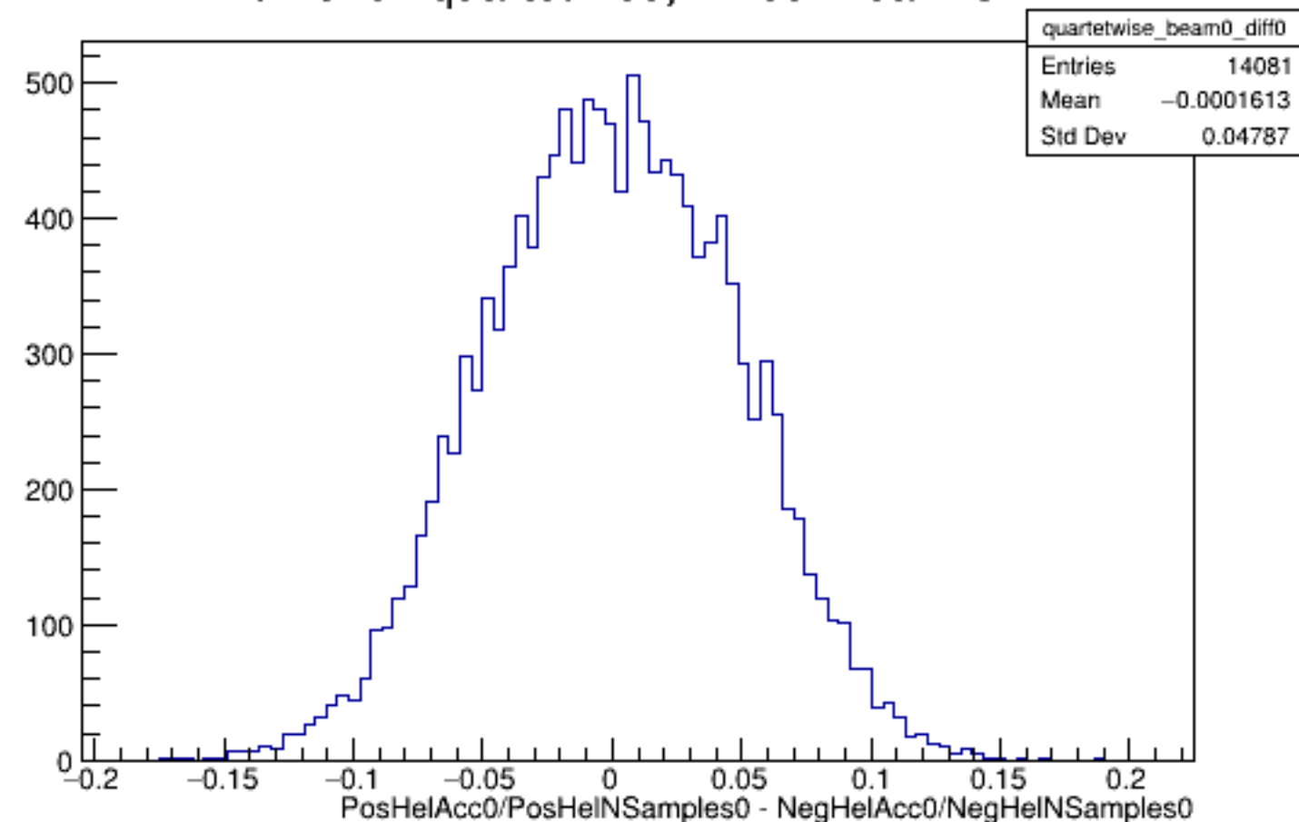
Run 5732 quartetwise, Diffs0: Beam OFF
