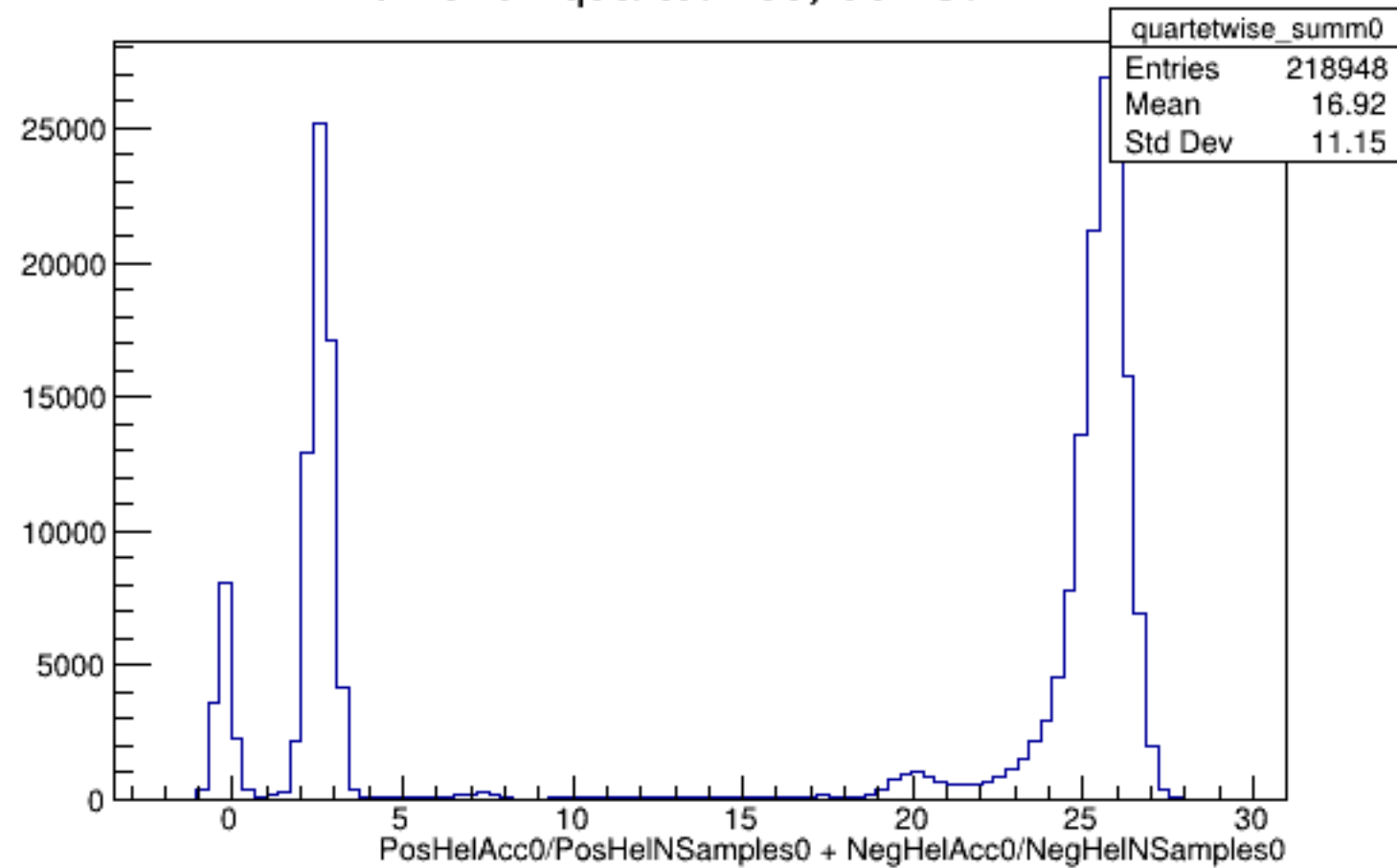
Run 5732 quartetwise, Sums0: All
