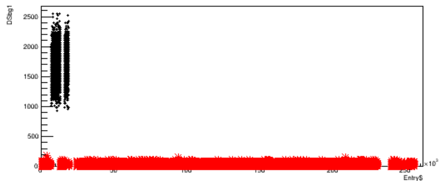
Run 5733, quartetwise: DSbg1 vs time
