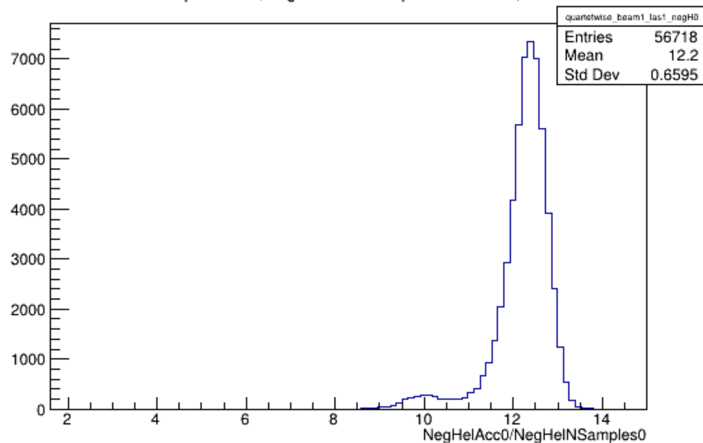
Run 5738 quartetwise, NegHelAcc0/NSamples0: Beam ON, Laser ON
