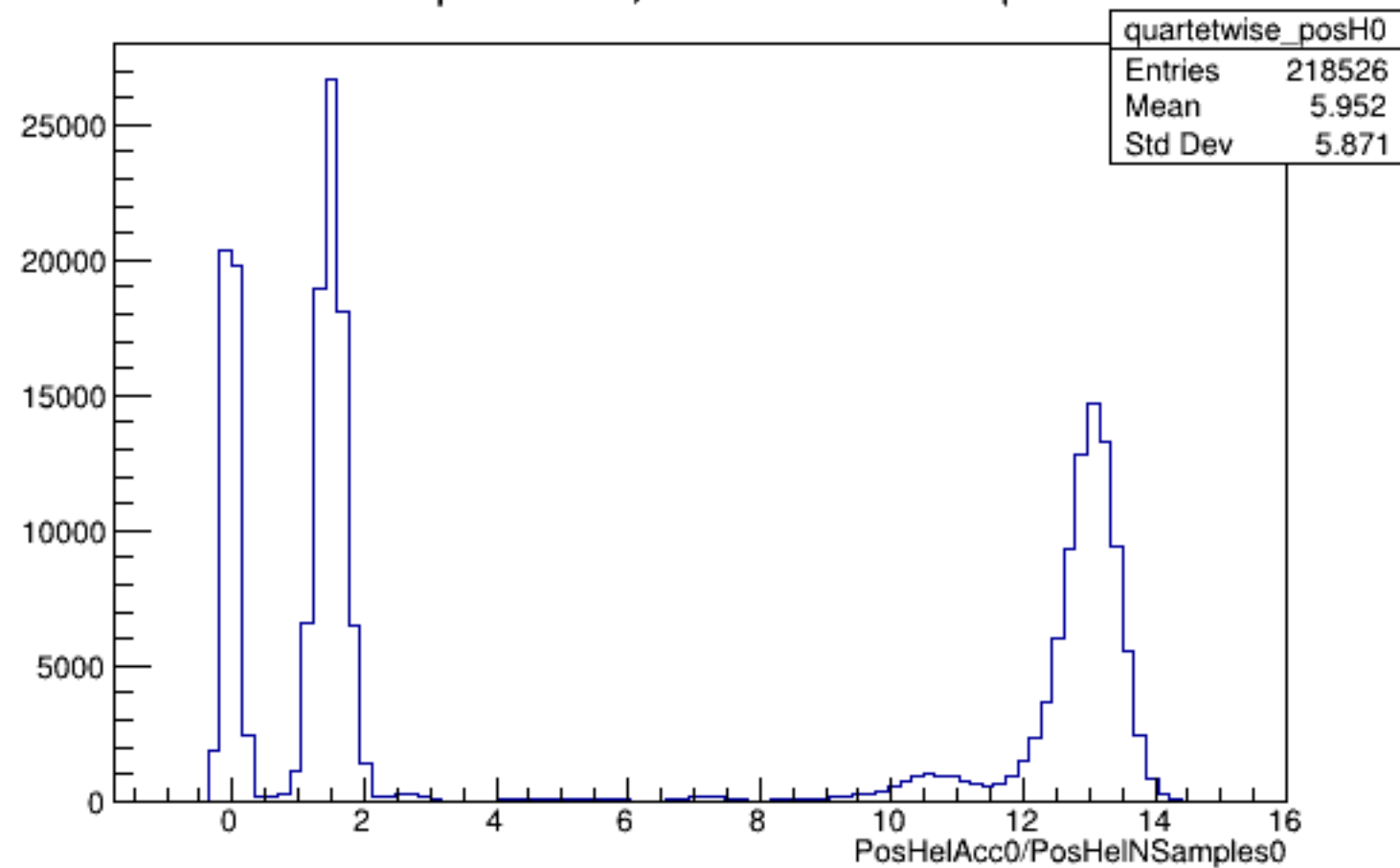
Run 5738 quartetwise, PosHelAcc0/NSamples0: All
