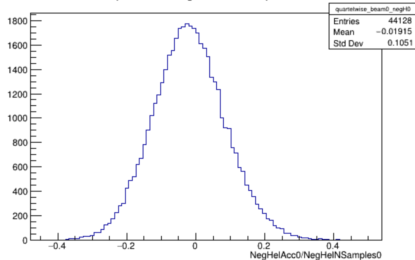
Run 5738 quartetwise, NegHelAcc0/NSamples0: Beam OFF
