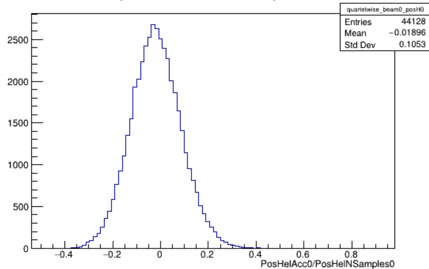
Run 5738 quartetwise, PosHelAcc0/NSamples0: Beam OFF
