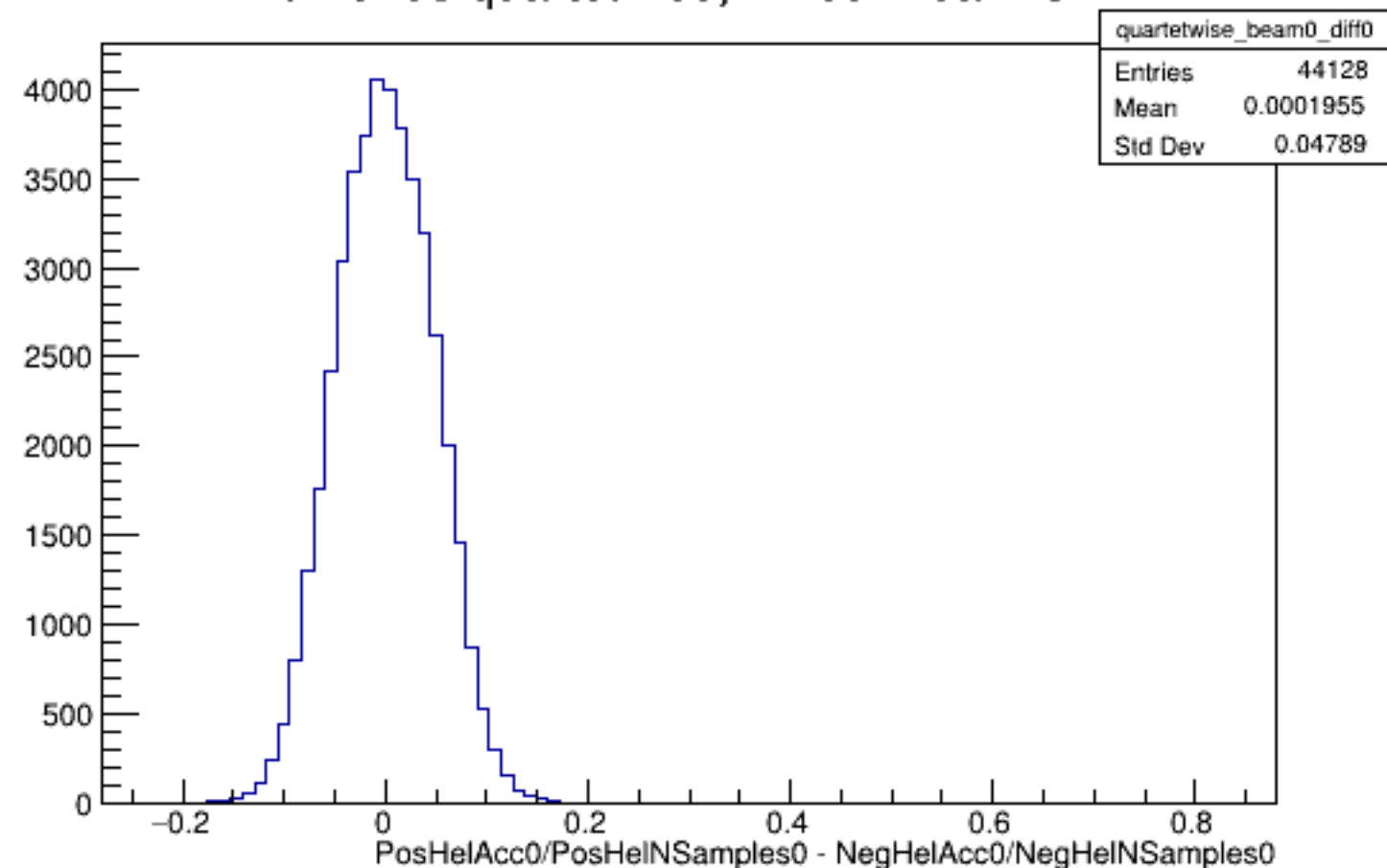
Run 5738 quartetwise, Diffs0: Beam OFF
