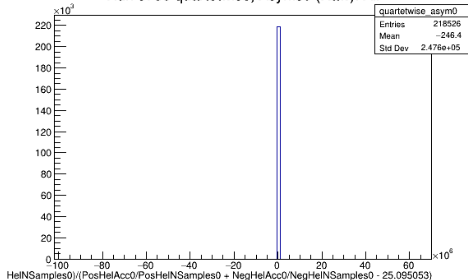
Run 5738 quartetwise, Asyms0 (Raw): All
