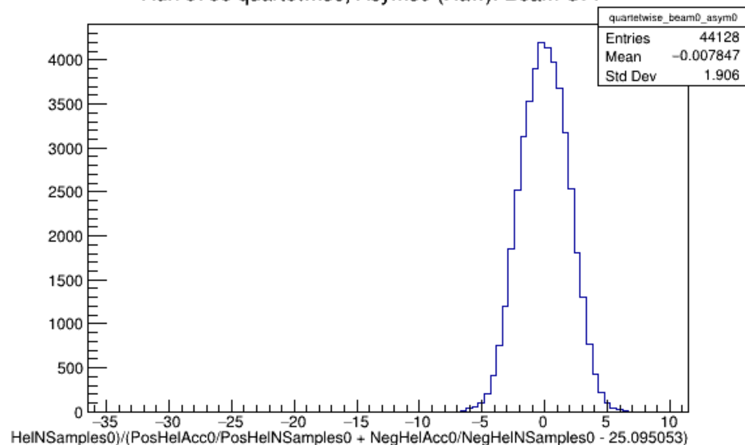
Run 5738 quartetwise, Asyms0 (Raw): Beam OFF
