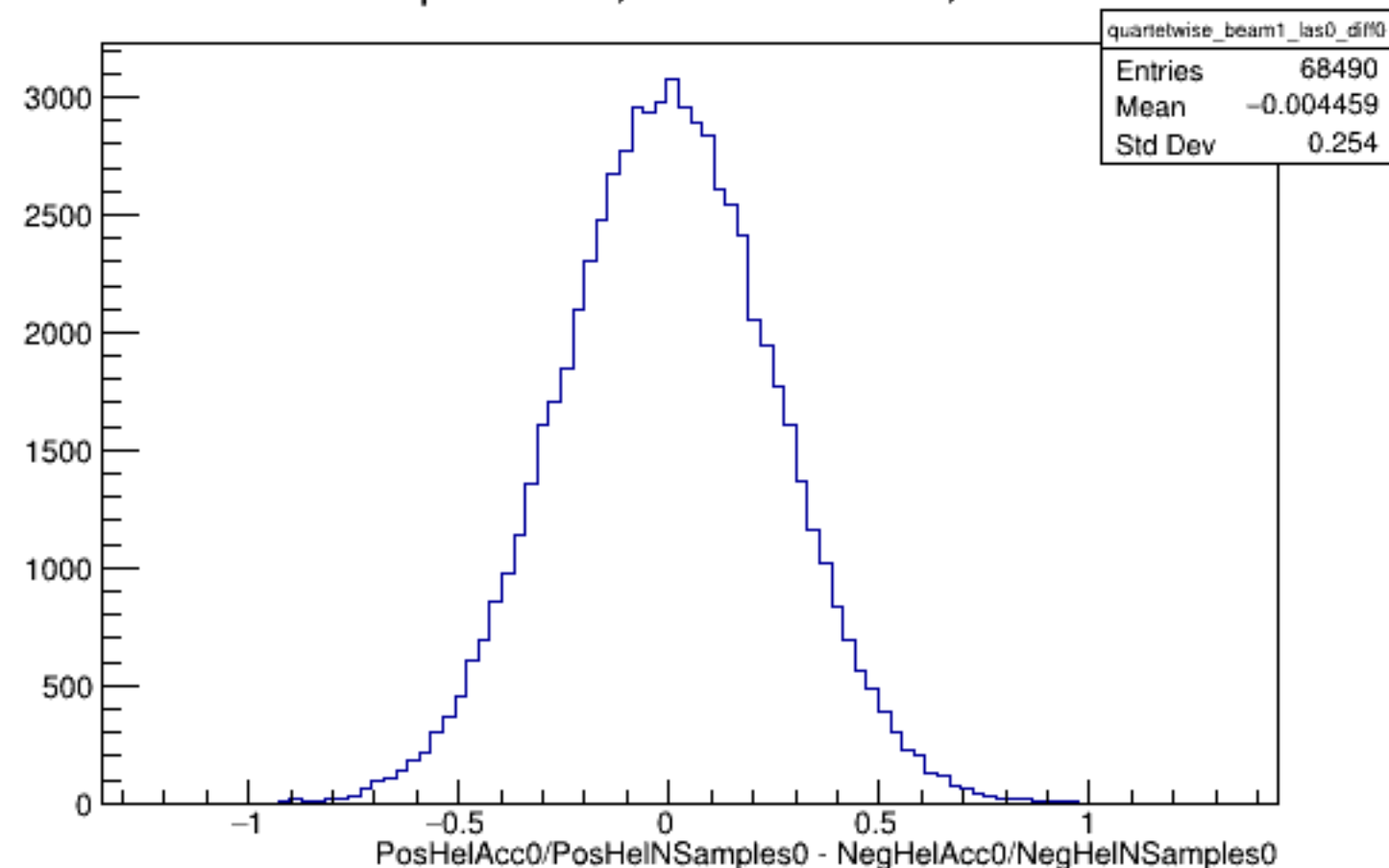
Run 5738 quartetwise, Diffs0: Beam ON, Laser OFF
