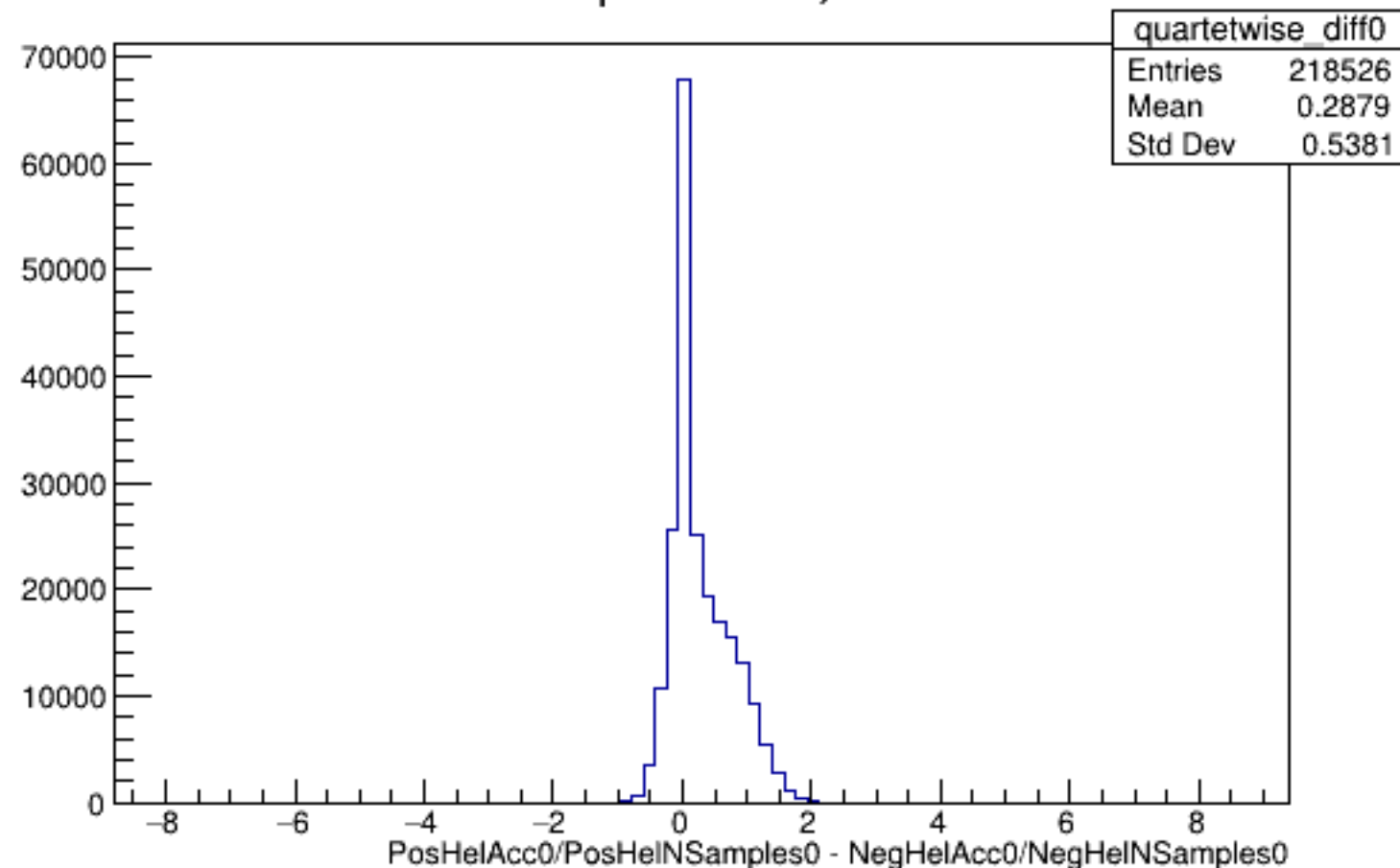
Run 5738 quartetwise, Diffs0: All
