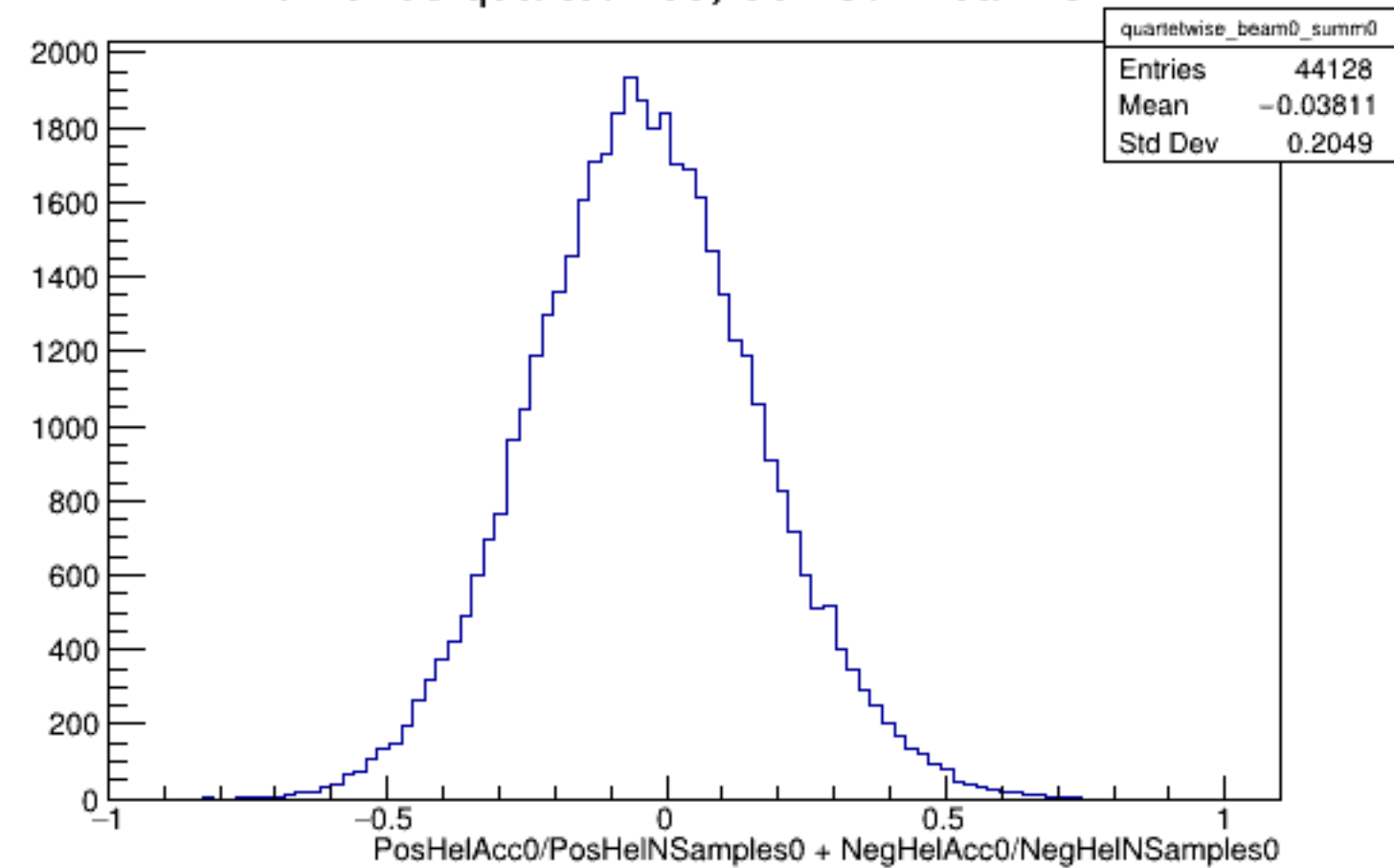
Run 5738 quartetwise, Sums0: Beam OFF
