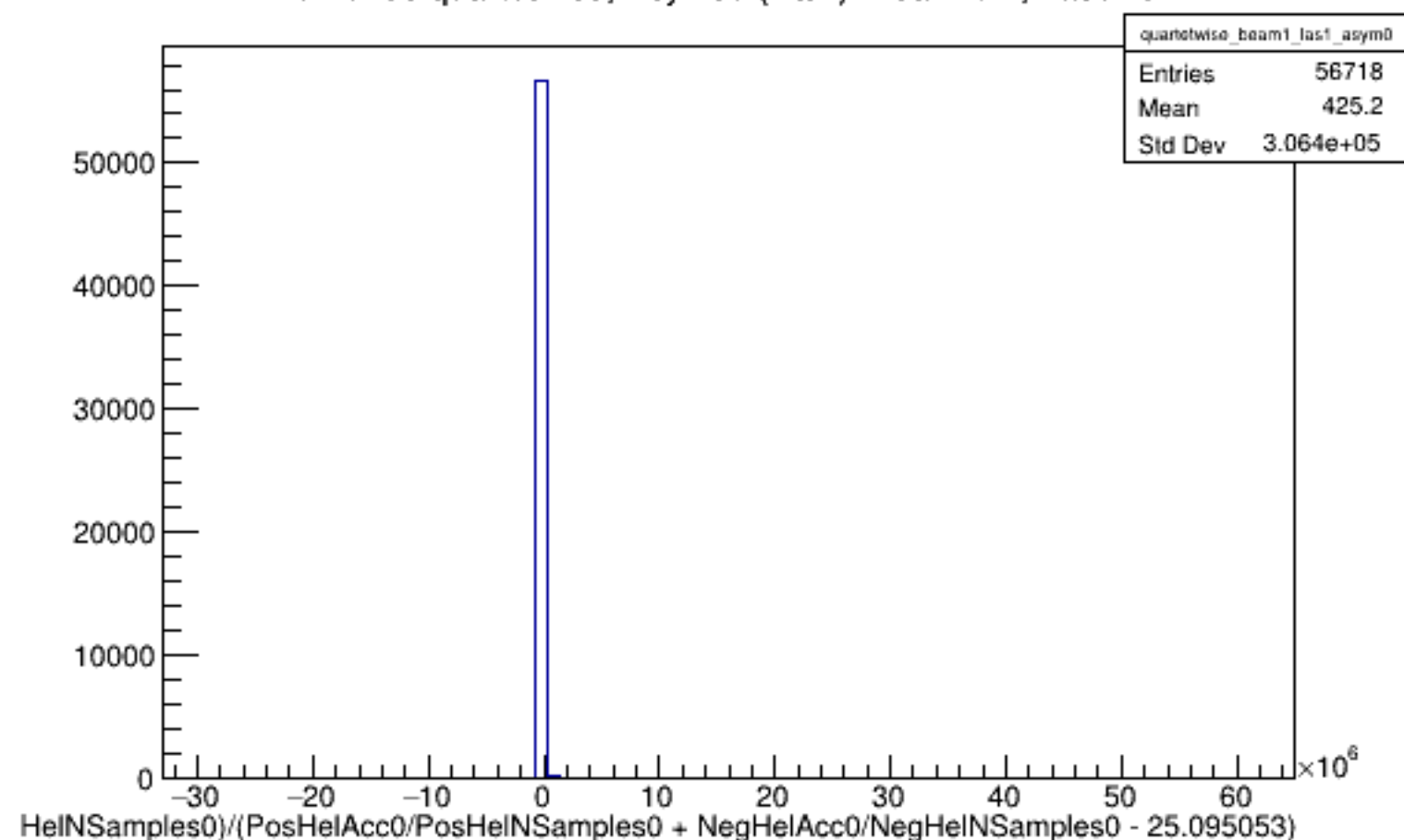
Run 5738 quartetwise, Asyms0 (Raw): Beam ON, Laser ON
