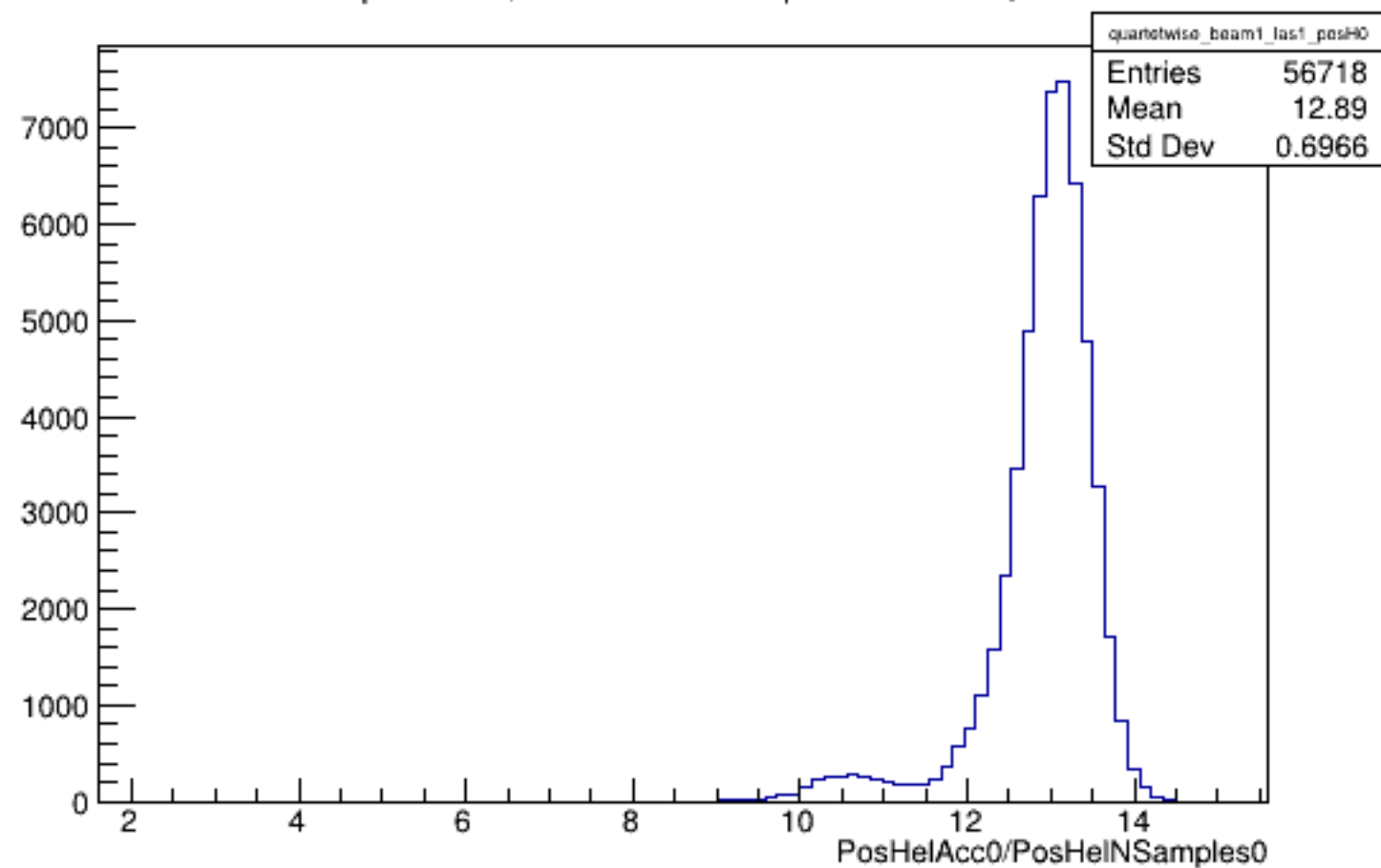
Run 5738 quartetwise, PosHelAcc0/NSamples0: Beam ON, Laser ON
