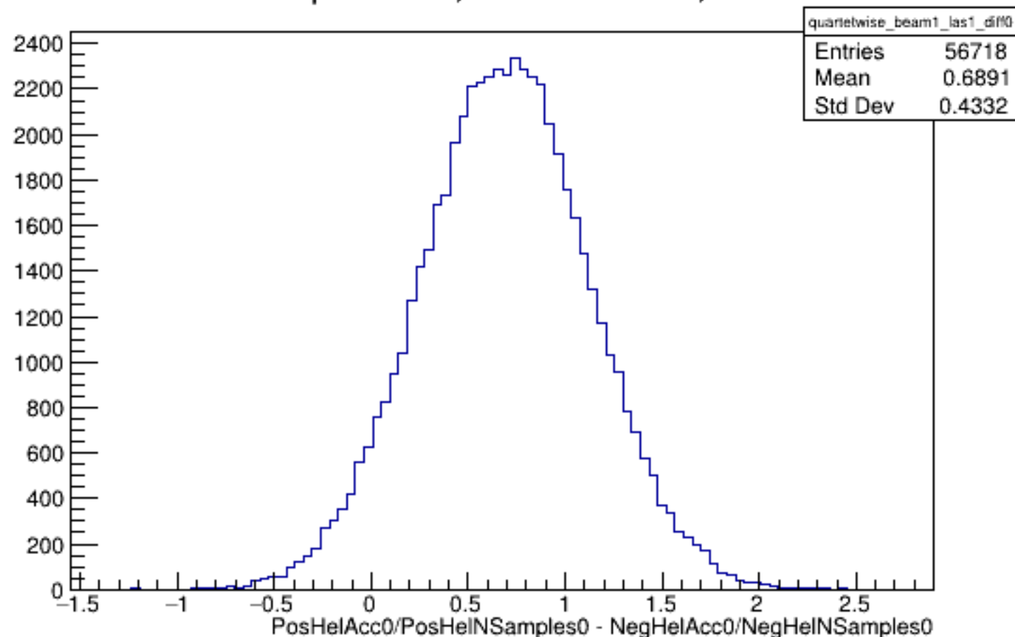
Run 5738 quartetwise, Diffs0: Beam ON, Laser ON
