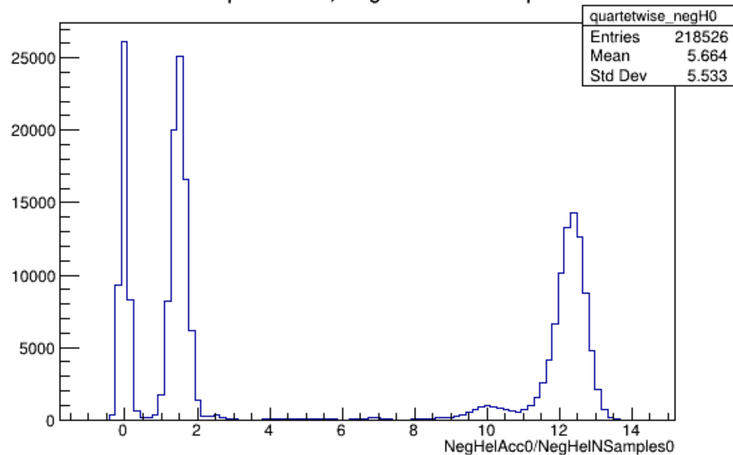
Run 5738 quartetwise, NegHelAcc0/NSamples0: All
