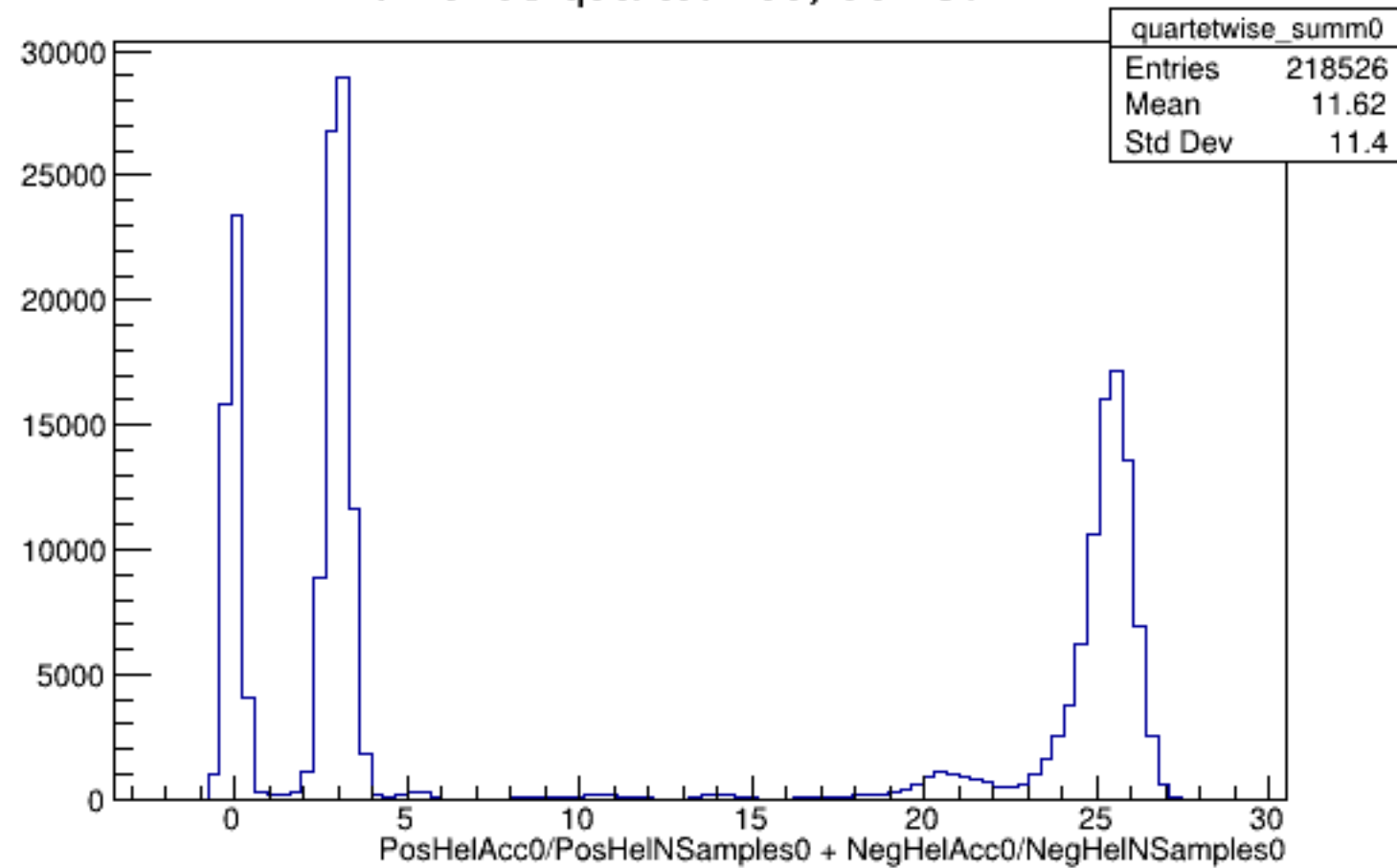
Run 5738 quartetwise, Sums0: All
