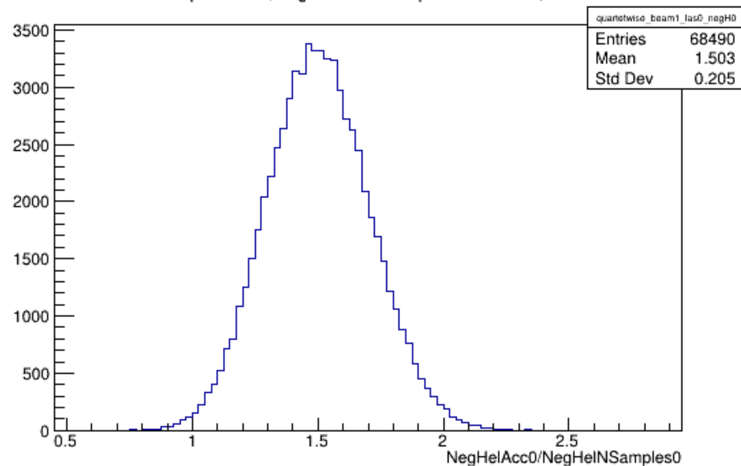
Run 5738 quartetwise, NegHelAcc0/NSamples0: Beam ON, Laser OFF
