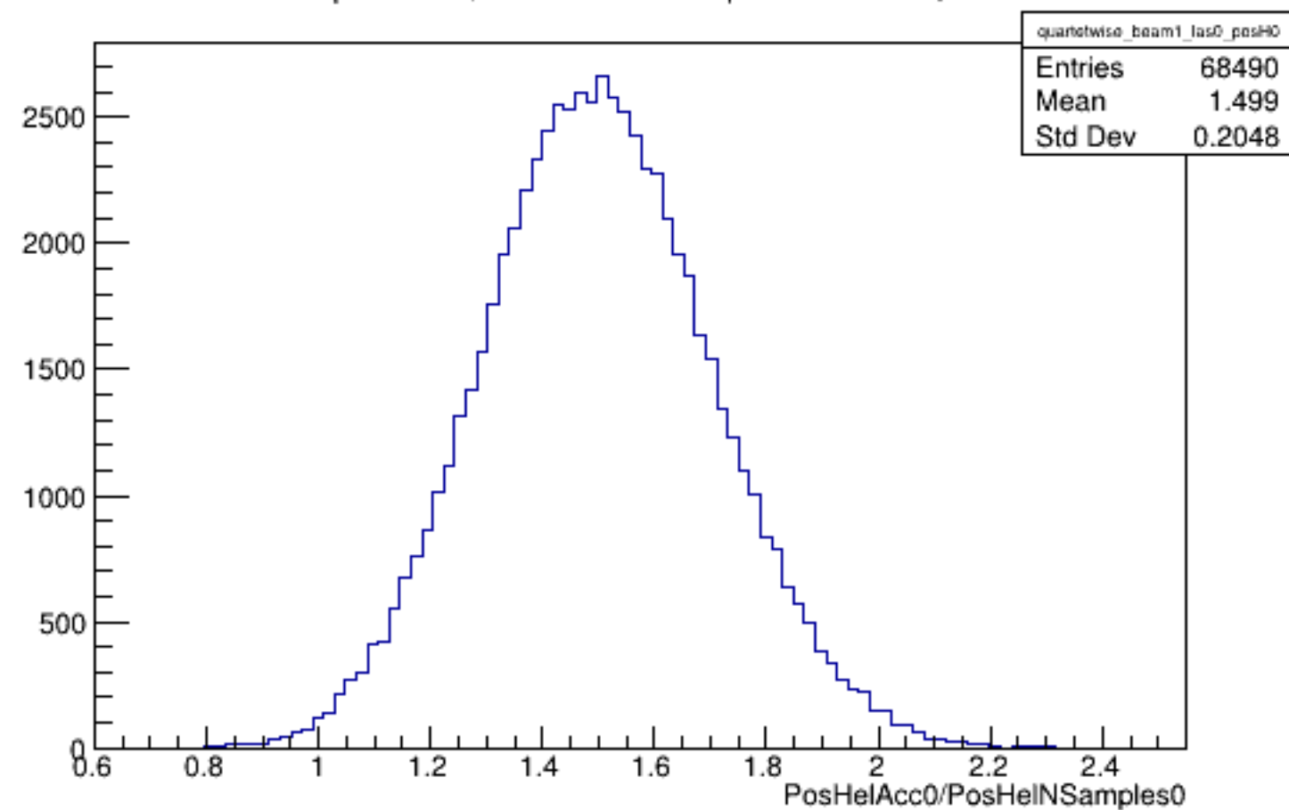
Run 5738 quartetwise, PosHelAcc0/NSamples0: Beam ON, Laser OFF
