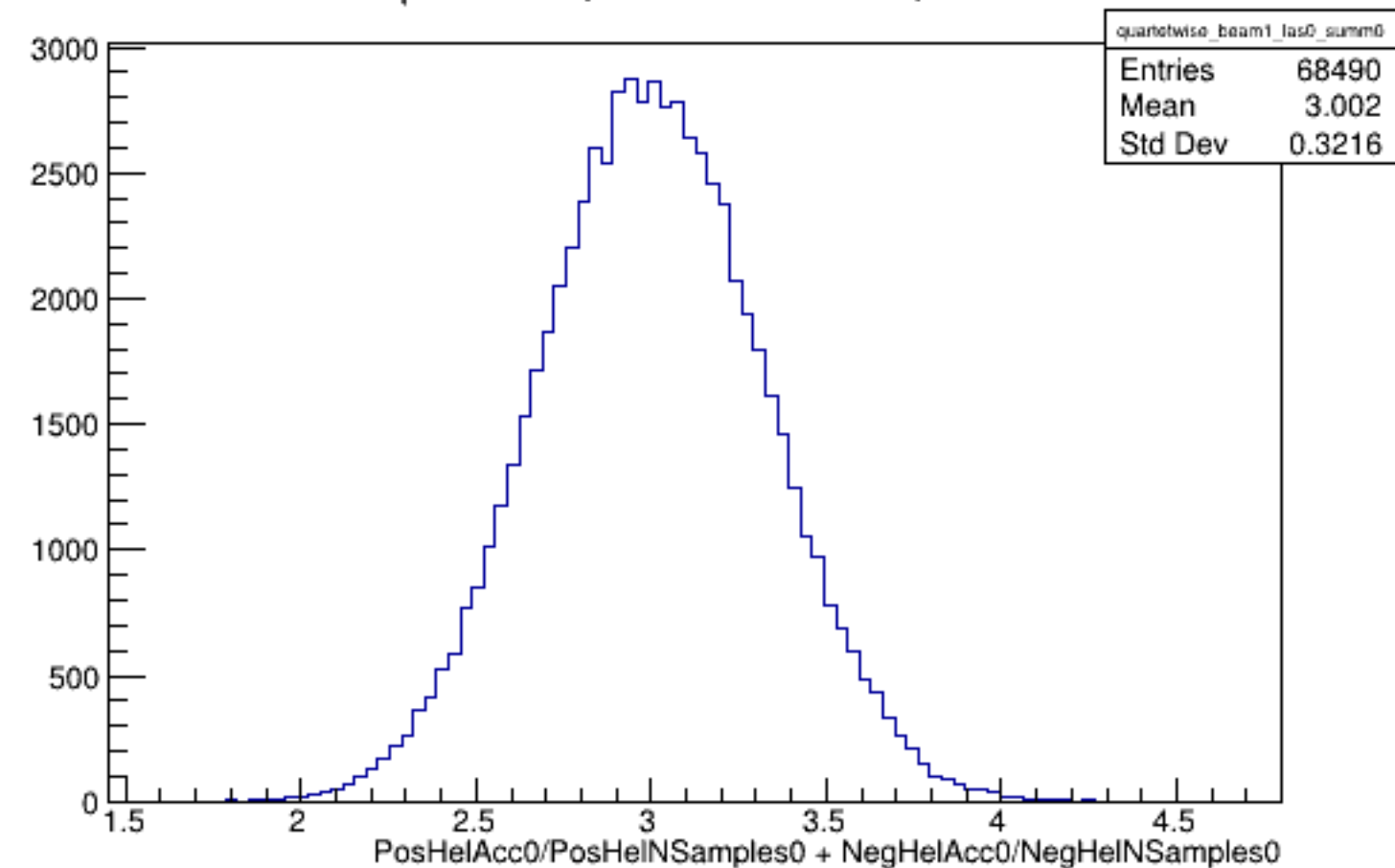
Run 5738 quartetwise, Sums0: Beam ON, Laser OFF
