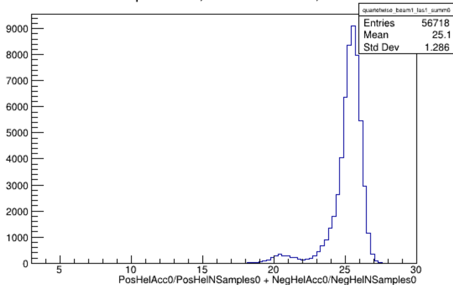
Run 5738 quartetwise, Sums0: Beam ON, Laser ON
