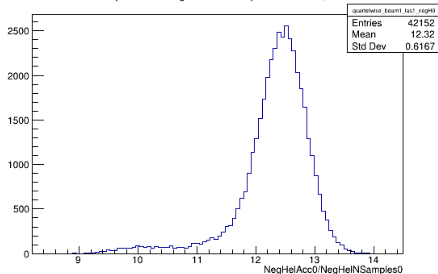
Run 5740 quartetwise, NegHelAcc0/NSamples0: Beam ON, Laser ON
