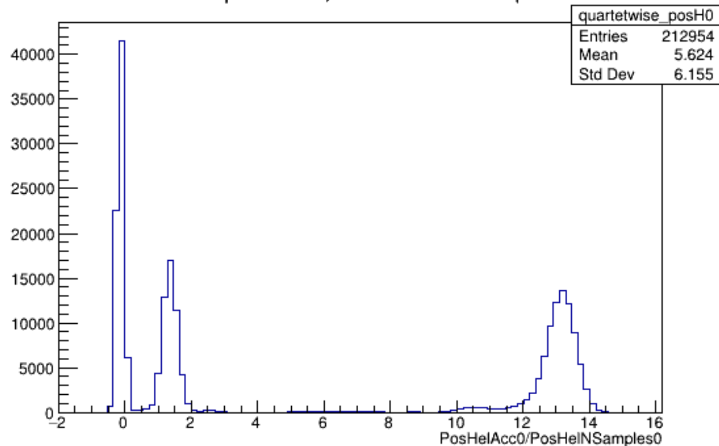
Run 5740 quartetwise, PosHelAcc0/NSamples0: All
