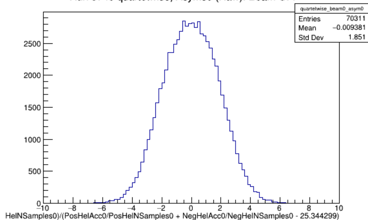
Run 5740 quartetwise, Asyms0 (Raw): Beam OFF
