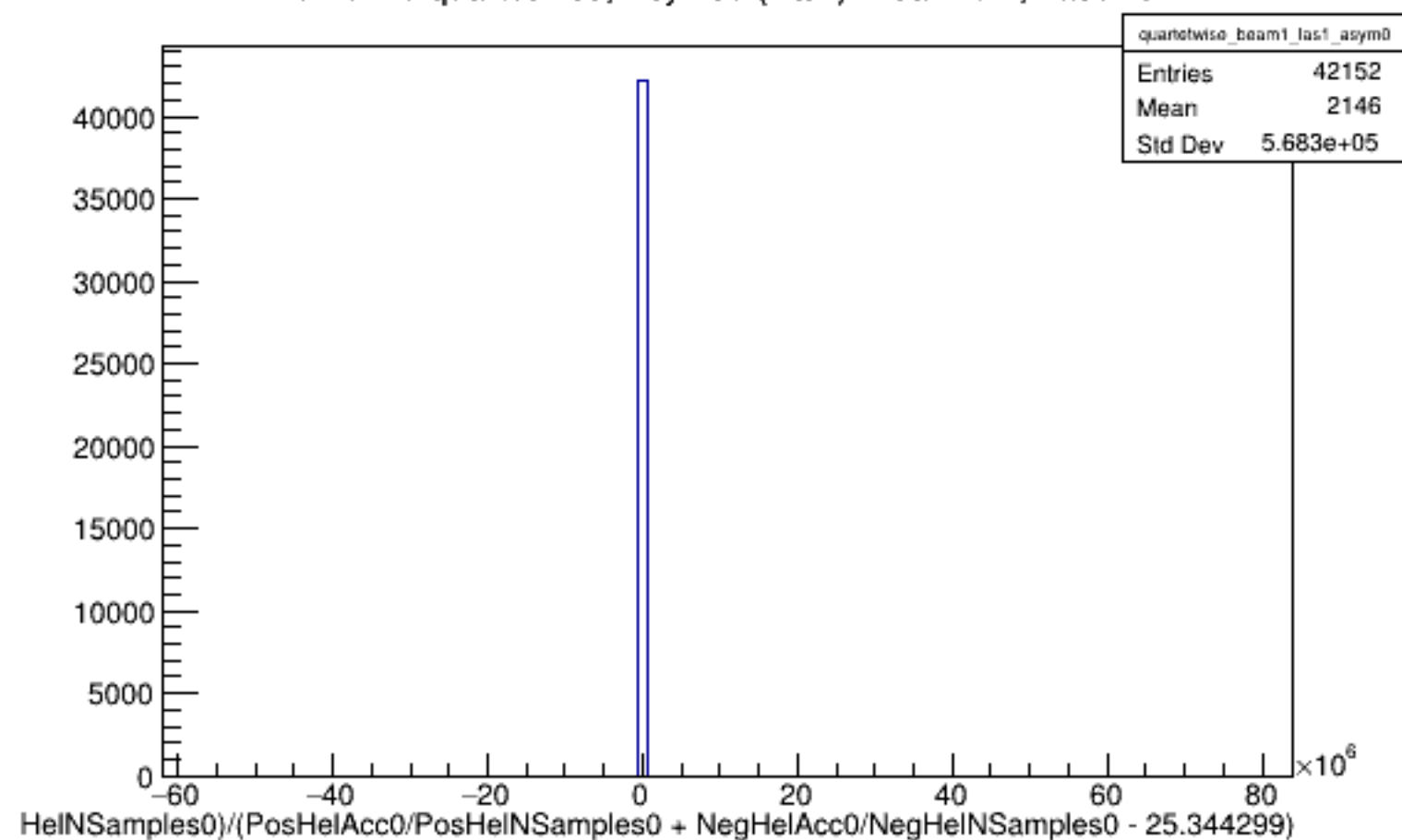
Run 5740 quartetwise, Asyms0 (Raw): Beam ON, Laser ON
