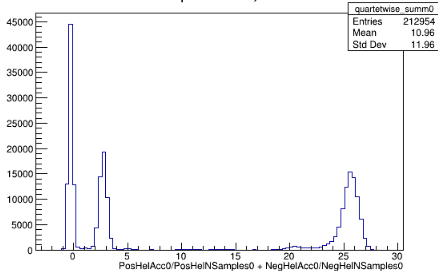
Run 5740 quartetwise, Sums0: All
