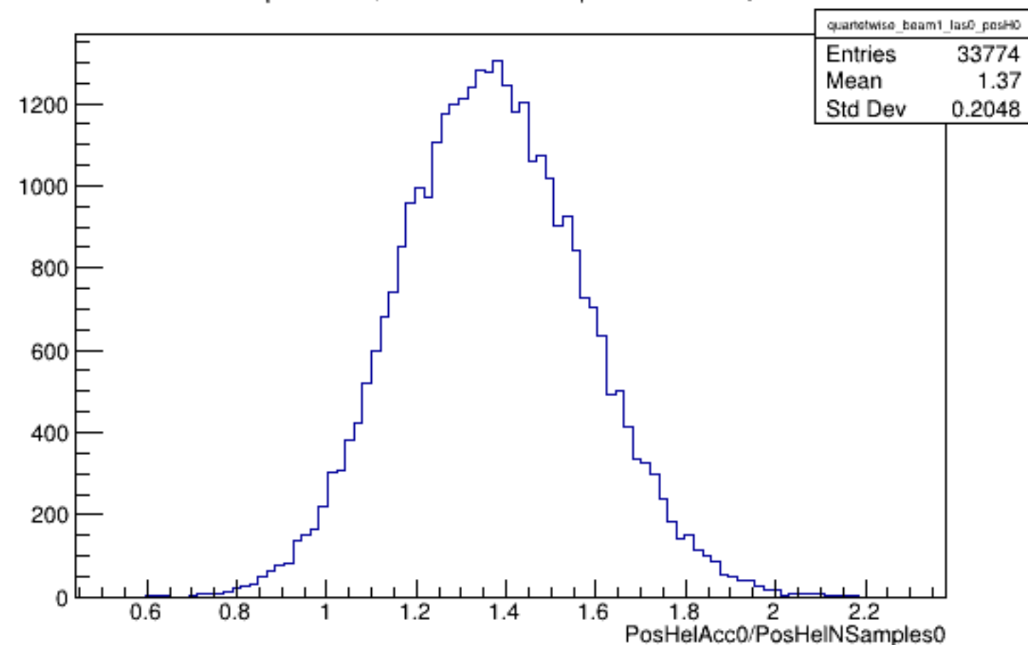
Run 5740 quartetwise, PosHelAcc0/NSamples0: Beam ON, Laser OFF
