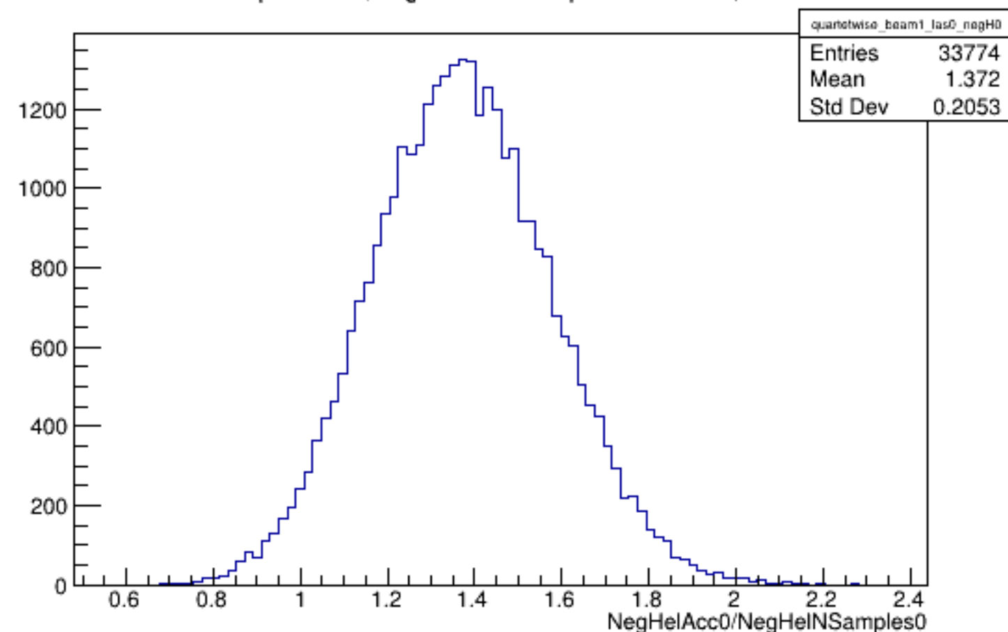
Run 5740 quartetwise, NegHelAcc0/NSamples0: Beam ON, Laser OFF
