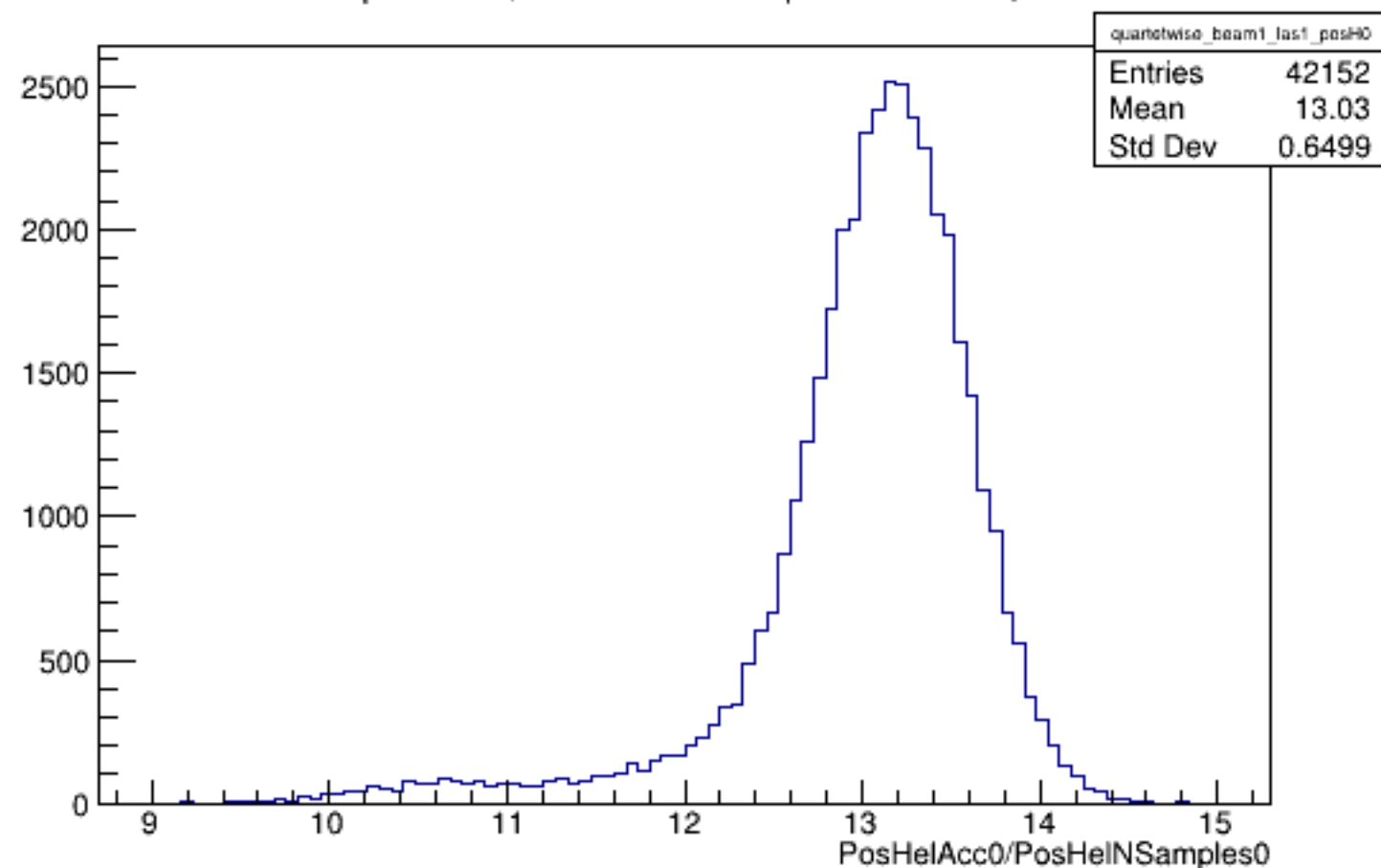
Run 5740 quartetwise, PosHelAcc0/NSamples0: Beam ON, Laser ON
