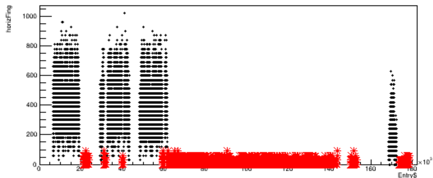
Run 5743, quartetwise: horizFing vs time
