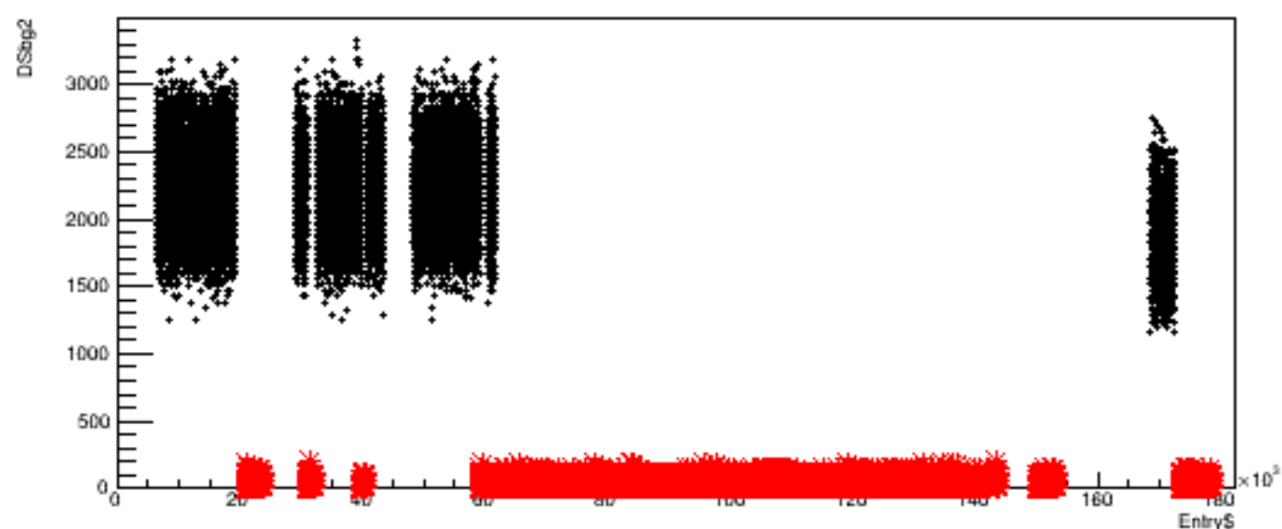
Run 5743, quartetwise: DSbg2 vs time
