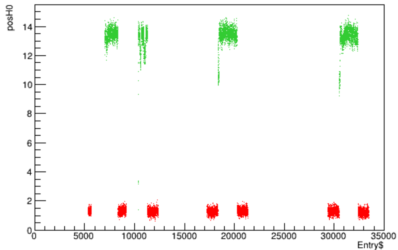
Run 5750 quartetwise, posH0 vs time
