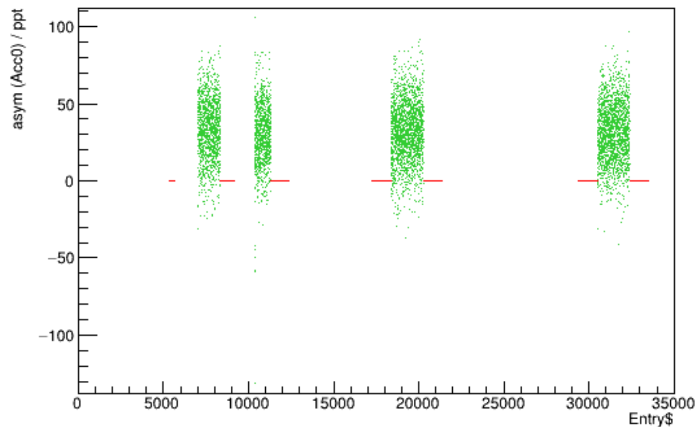
Run 5750 quartetwise, asym0sub vs time
