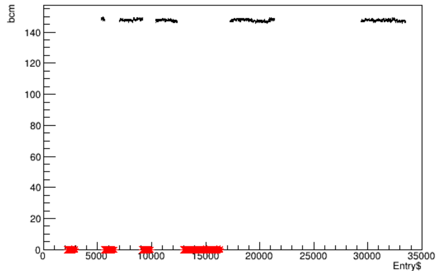
Run 5750 quartetwise, bcm vs time
