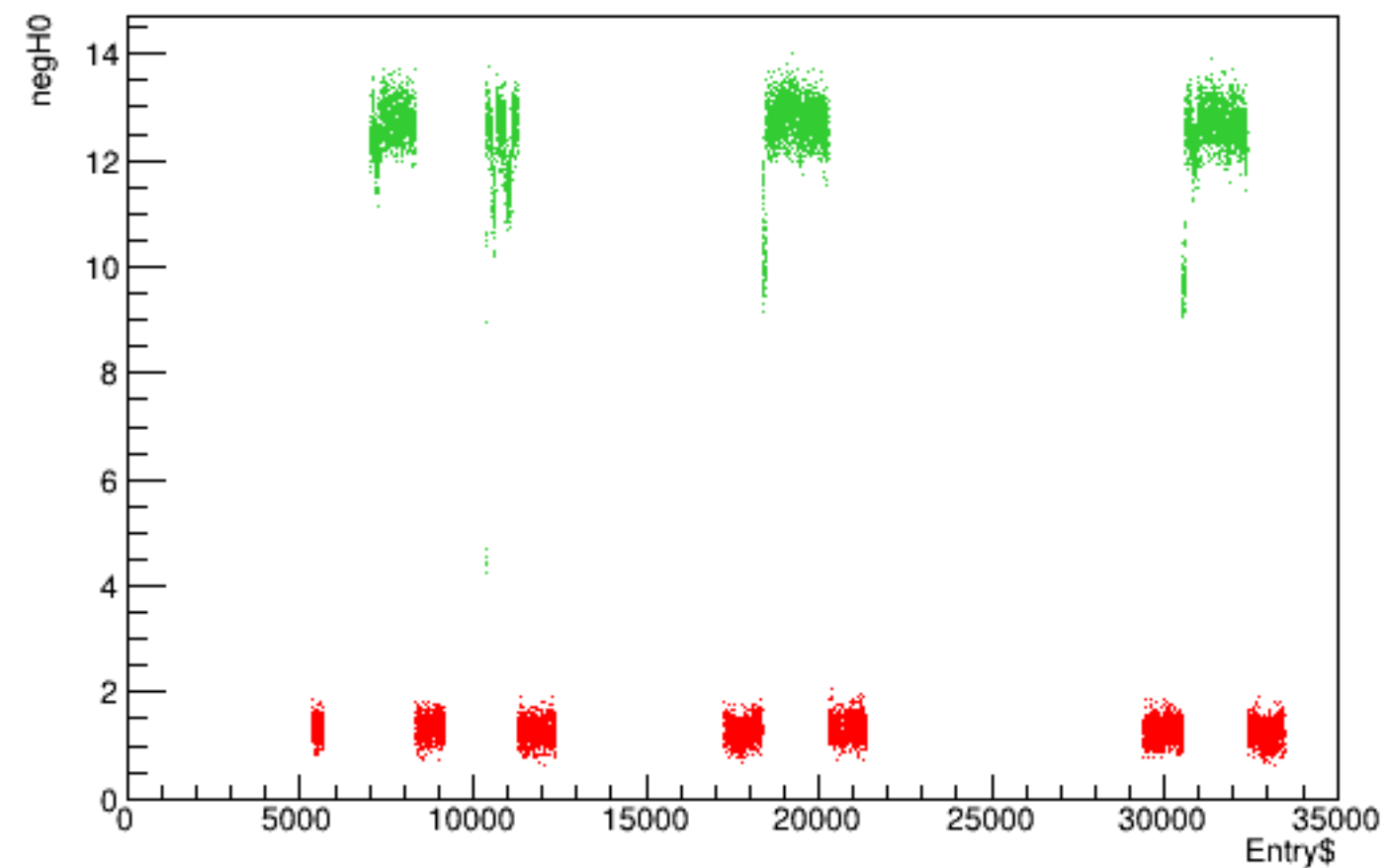
Run 5750 quartetwise, negH0 vs time
