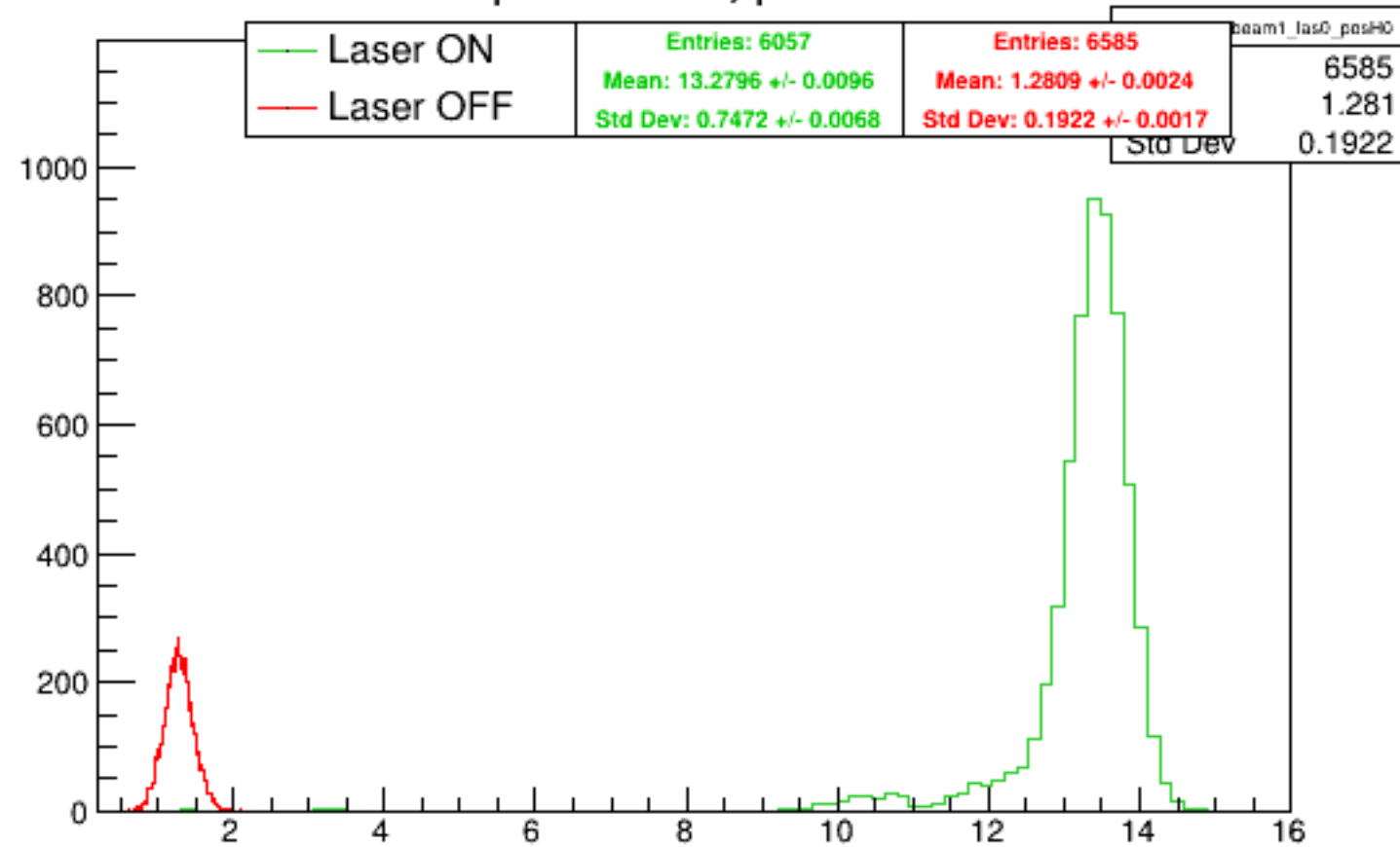
Run 5750 quartetwise, posH0: Beam ON
