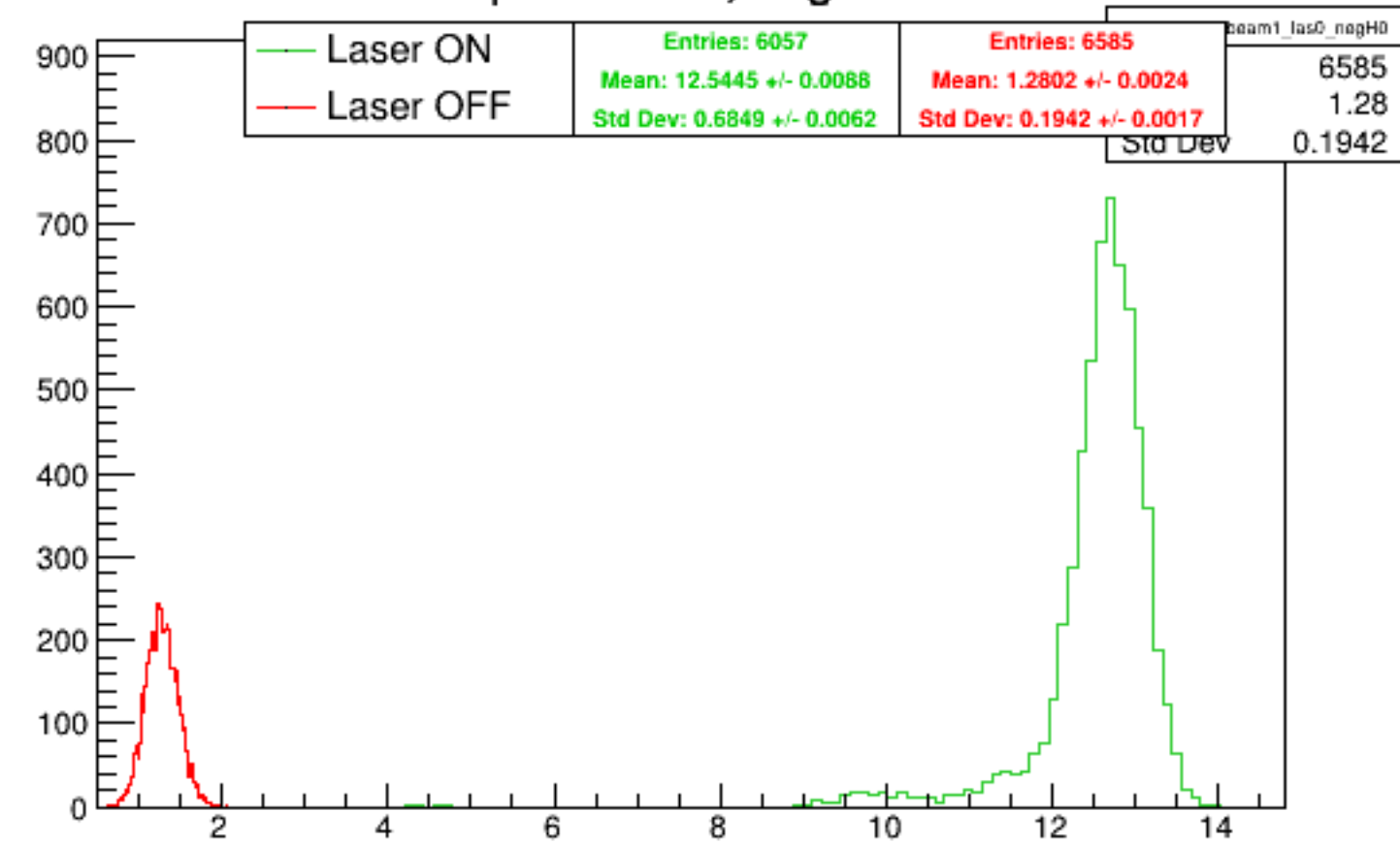
Run 5750 quartetwise, negH0: Beam ON
