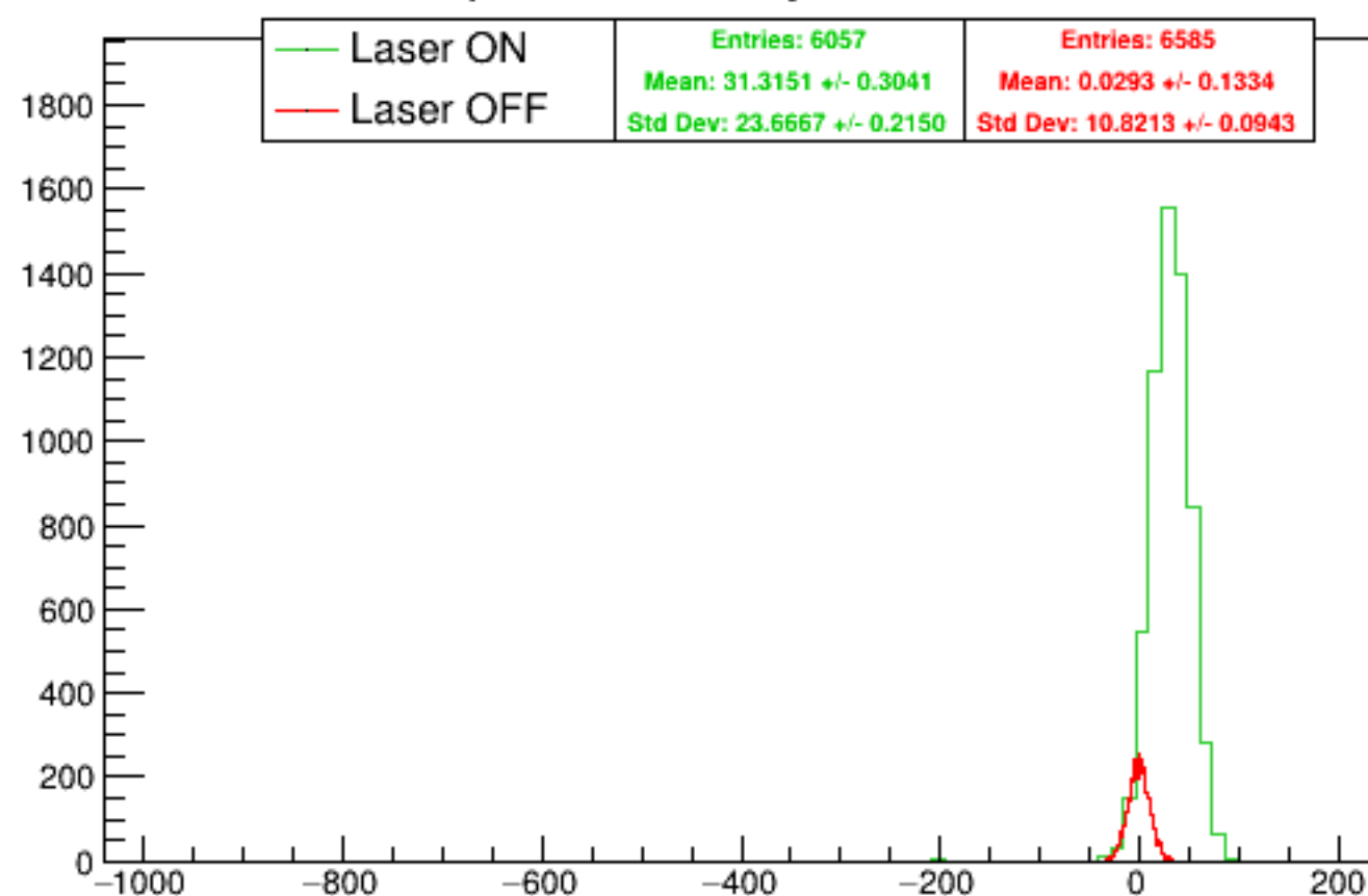
Run 5750 quartetwise, asym0sub: Beam ON
