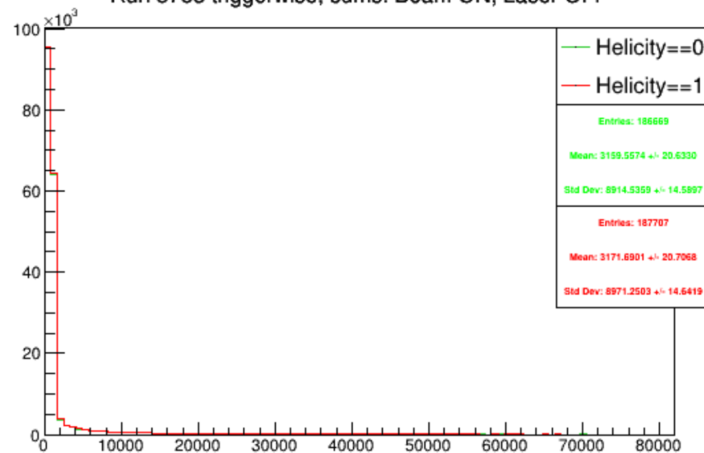
Run 5753 triggerwise, sums: Beam ON, Laser OFF
