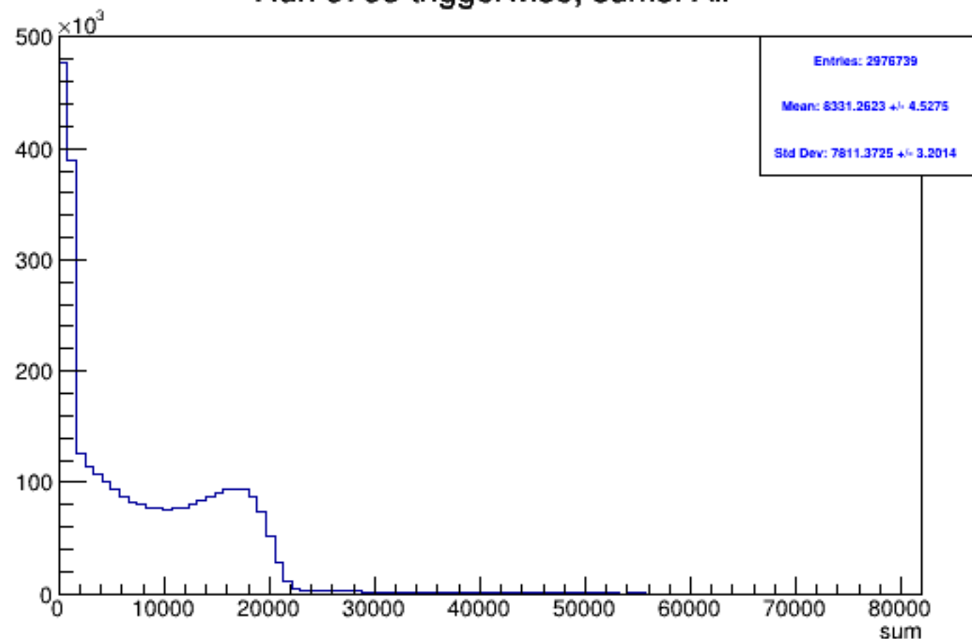
Run 5753 triggerwise, sums: All
