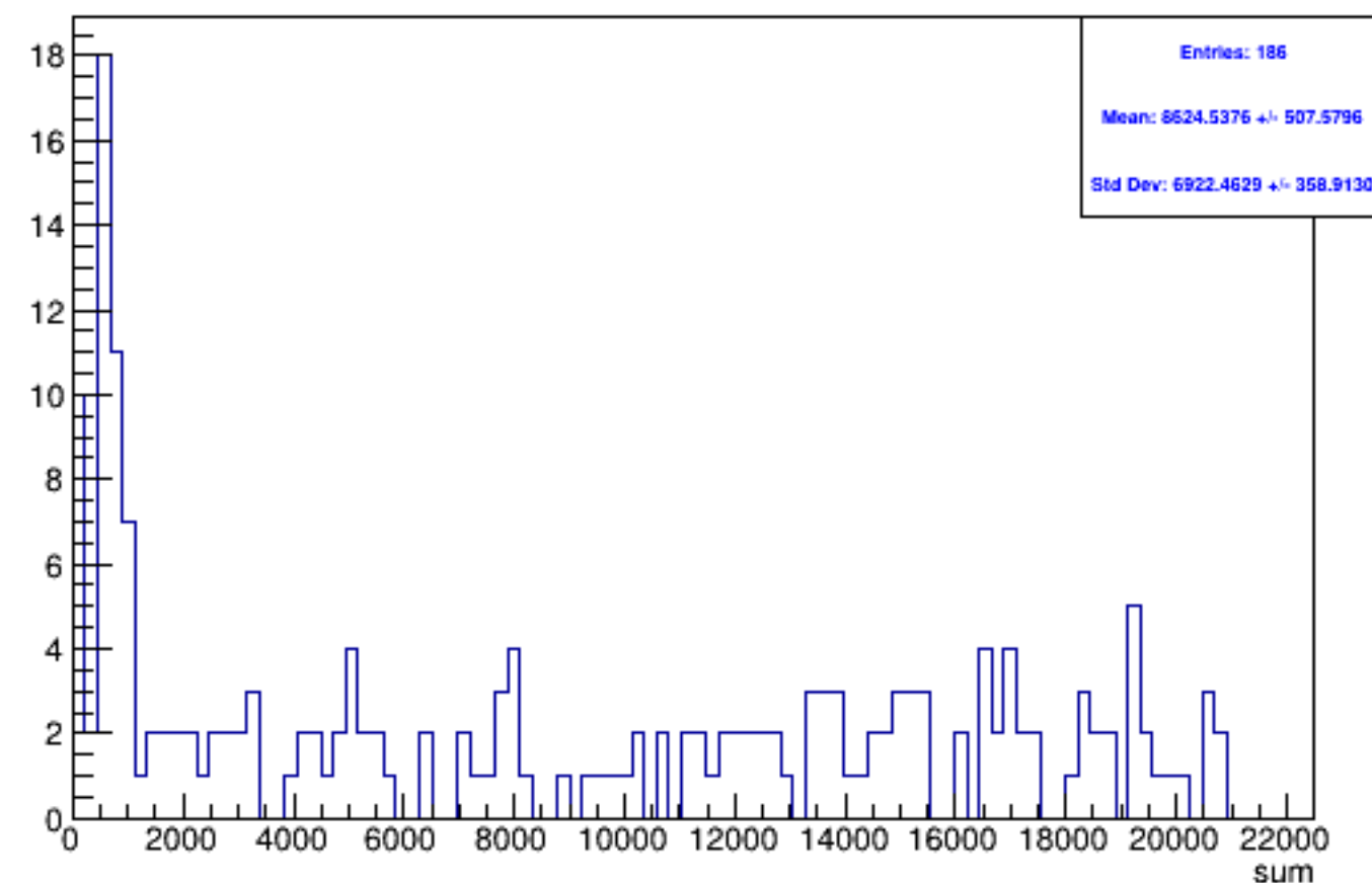
Run 5753 triggerwise, sums: Beam OFF
