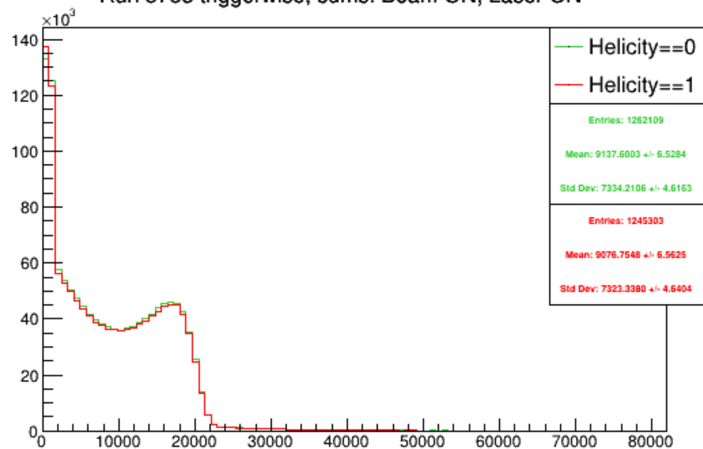
Run 5753 triggerwise, sums: Beam ON, Laser ON
