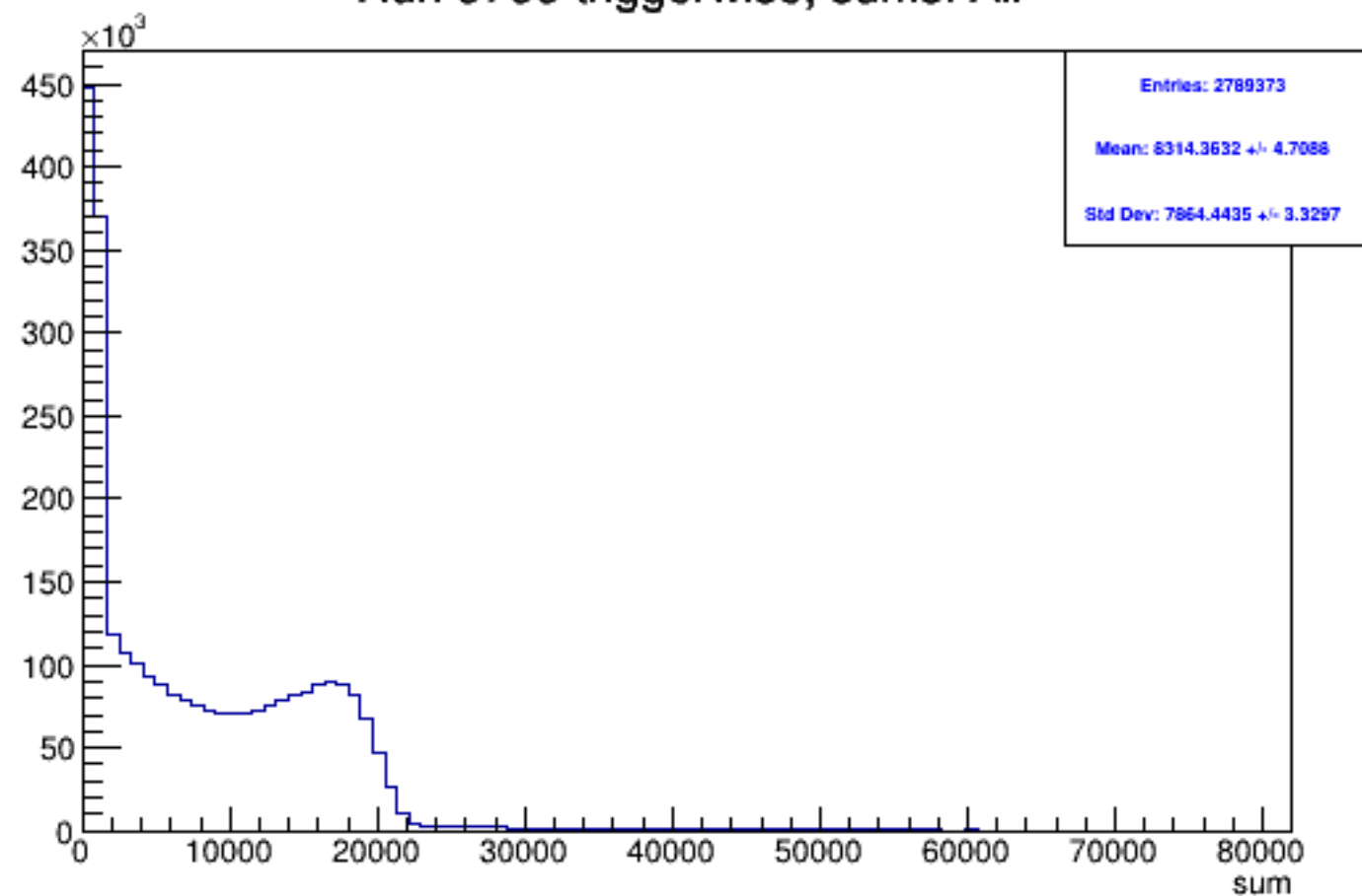
Run 5755 triggerwise, sums: All
