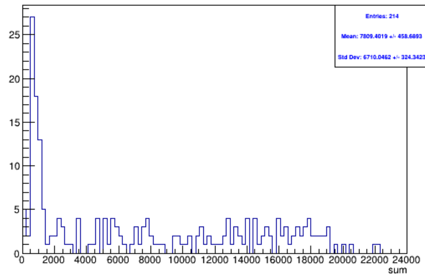
Run 5755 triggerwise, sums: Beam OFF
