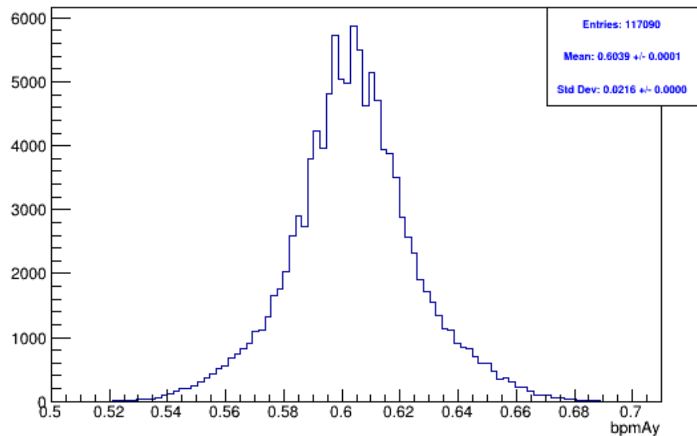
Run 5759, mpwise, bpmAy: Beam ON, Laser ON
