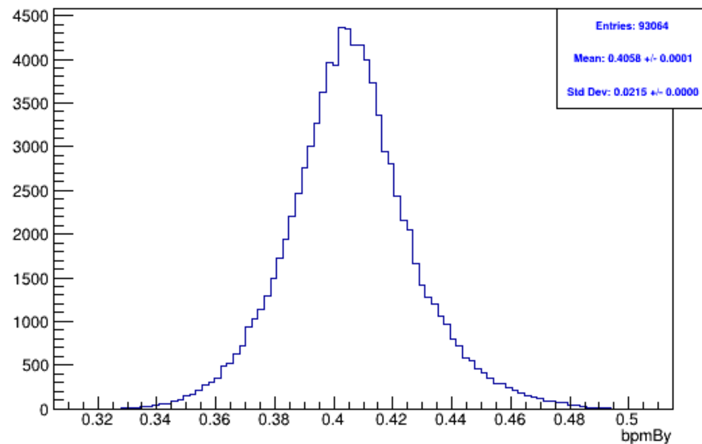
Run 5759, mpswise, bpmBy: Beam ON, Laser OFF
