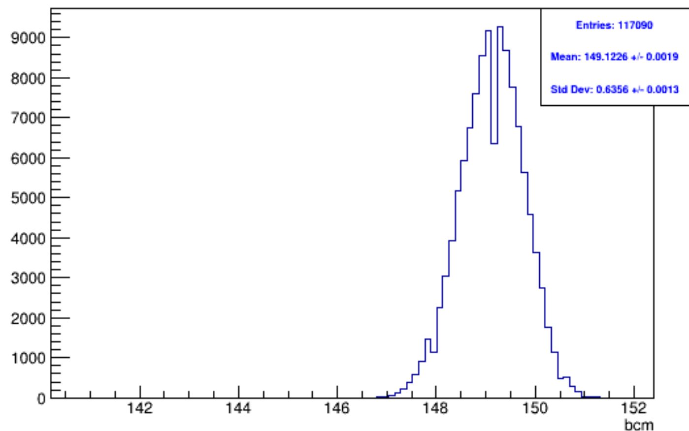
Run 5759, mpwise, BCM: Beam ON, Laser ON
