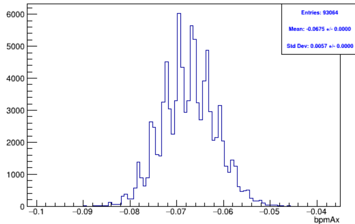
Run 5759, mpwise, bpmAx: Beam ON, Laser OFF
