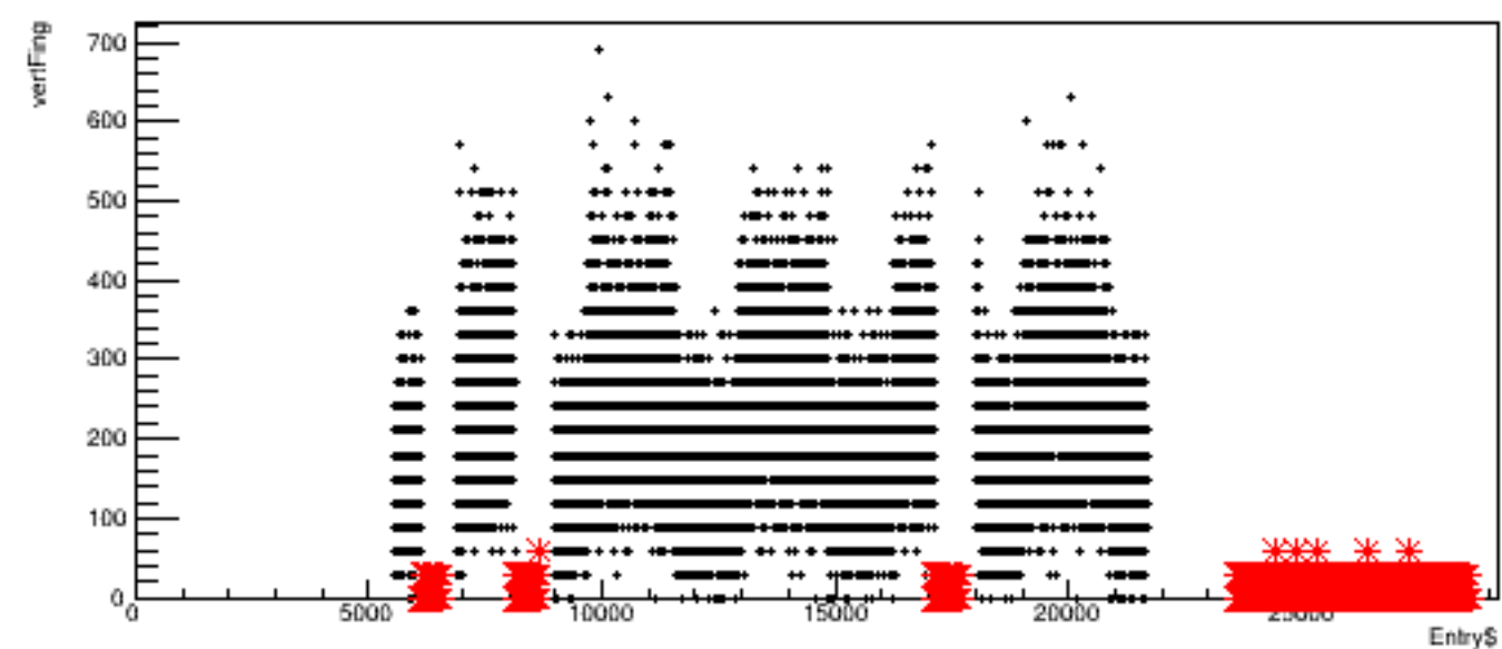
Run 5760, quartetwise: vertFing vs time
