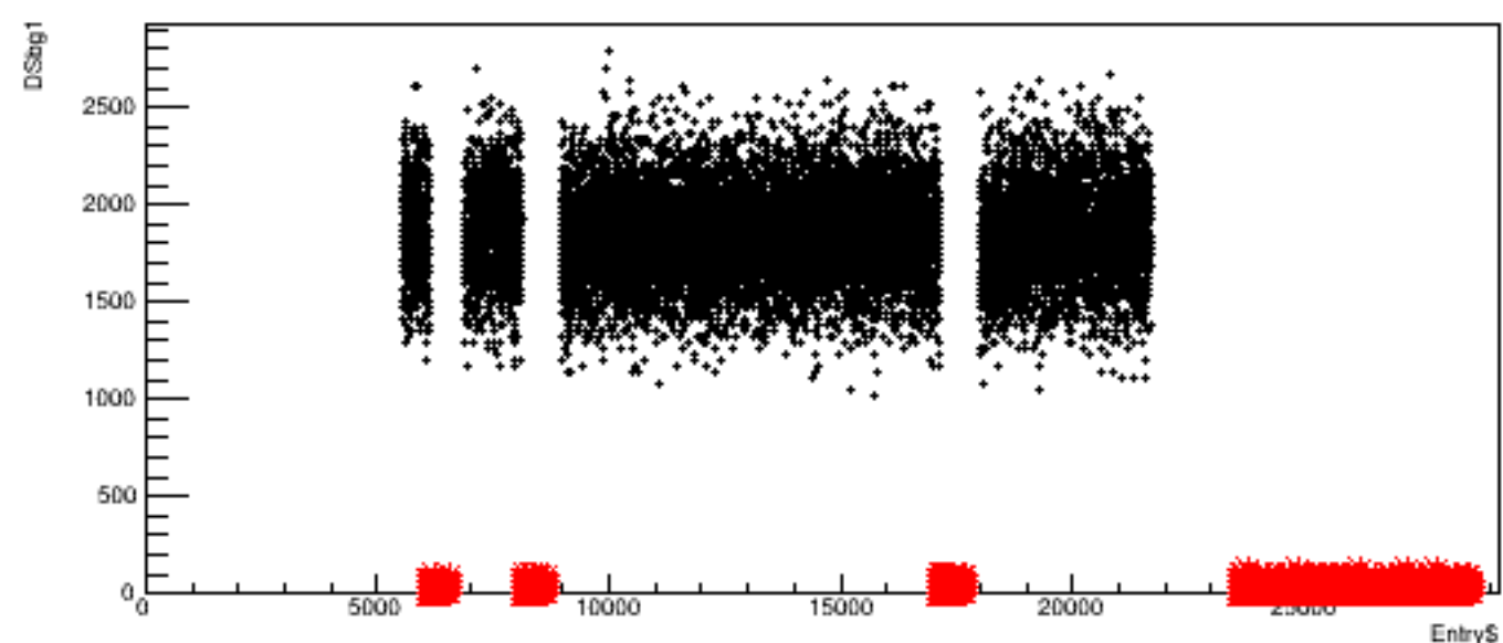
Run 5760, quartetwise: DSbg1 vs time
