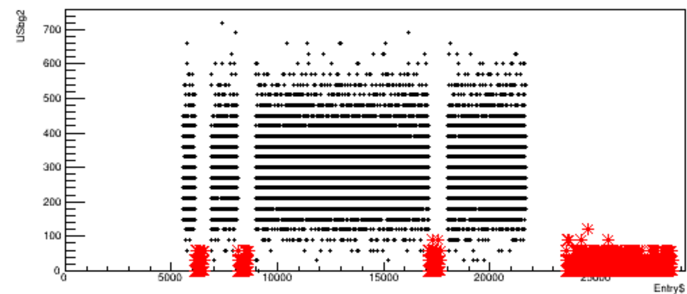
Run 5760, quartetwise: USbg2 vs time
