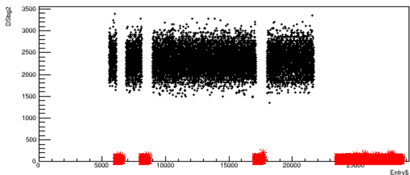
Run 5760, quartetwise: DSbg2 vs time
