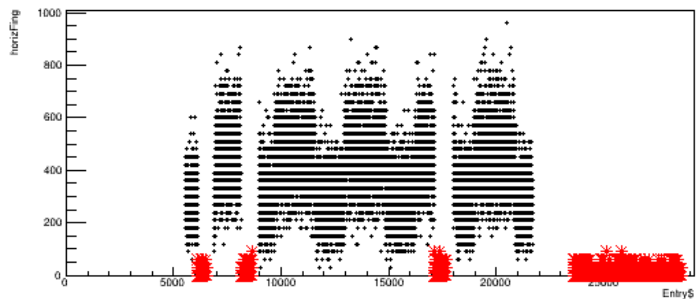
Run 5760, quartetwise: horizFing vs time
