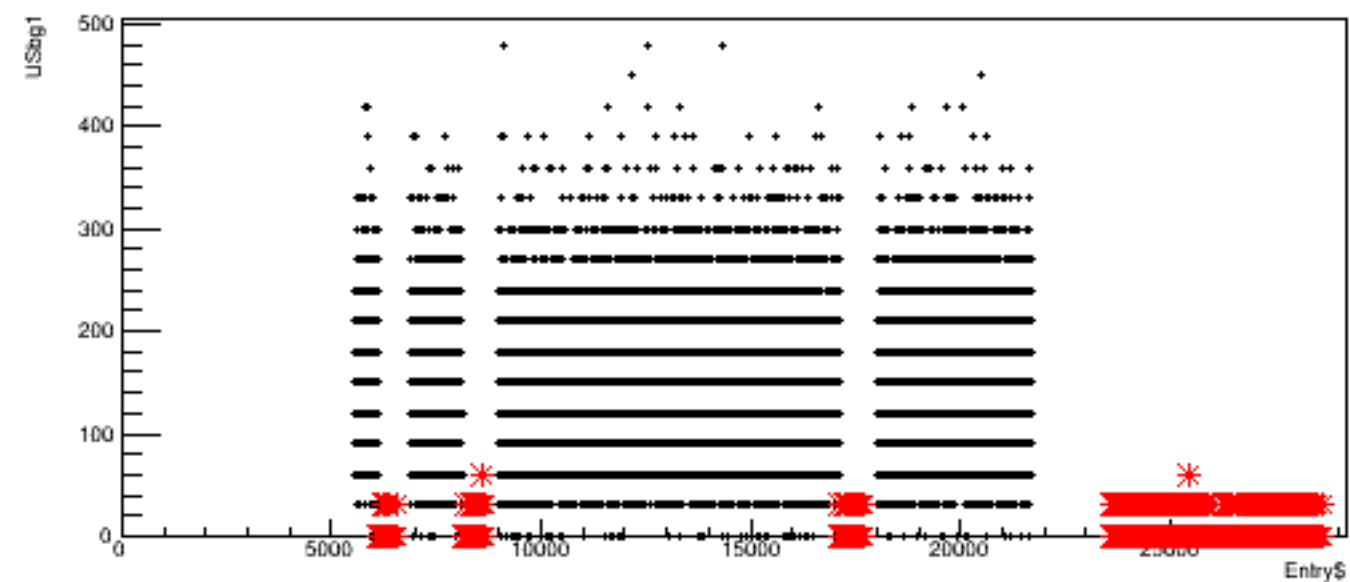
Run 5760, quartetwise: USbg1 vs time
