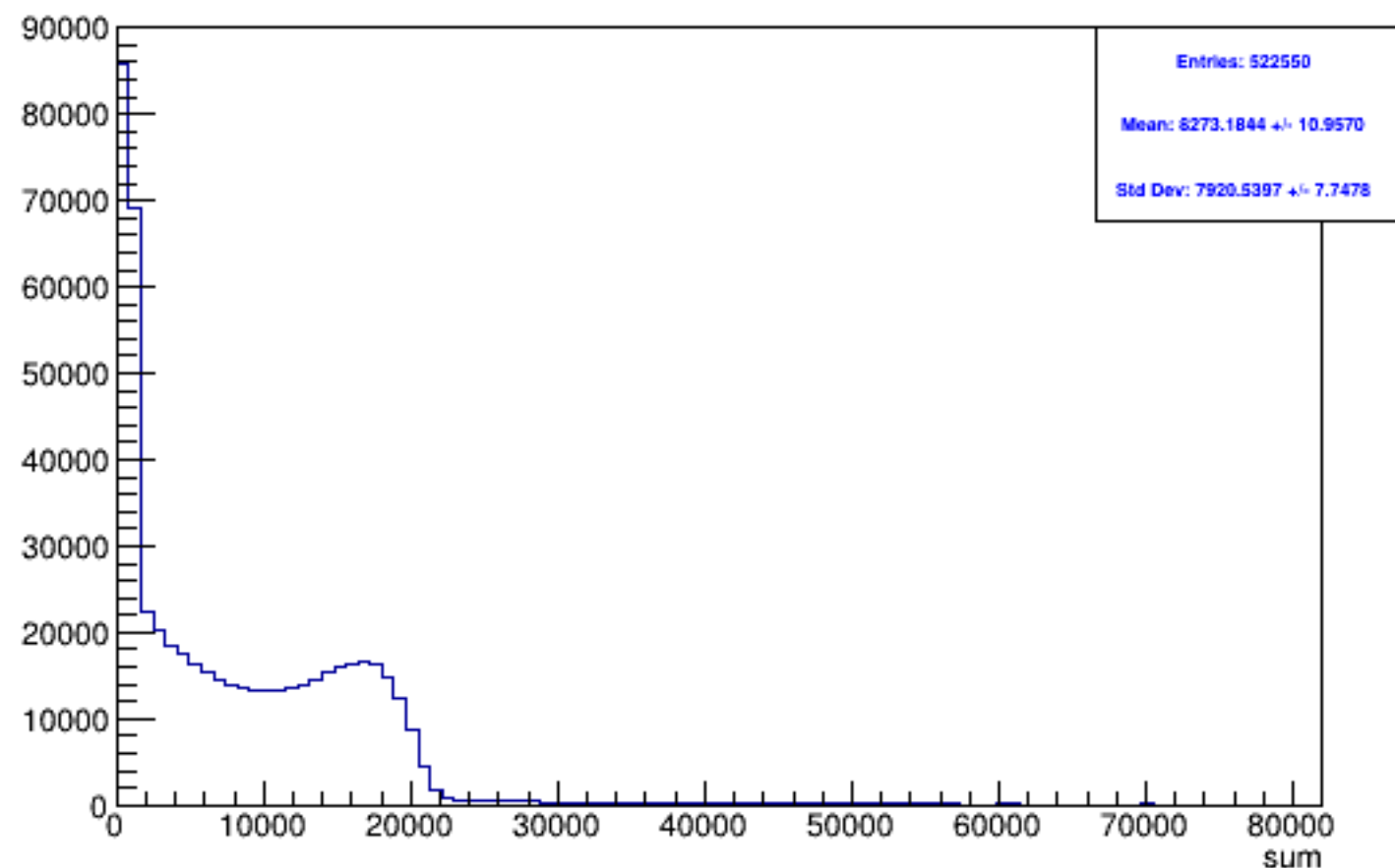
Run 5761 triggerwise, sums: All
