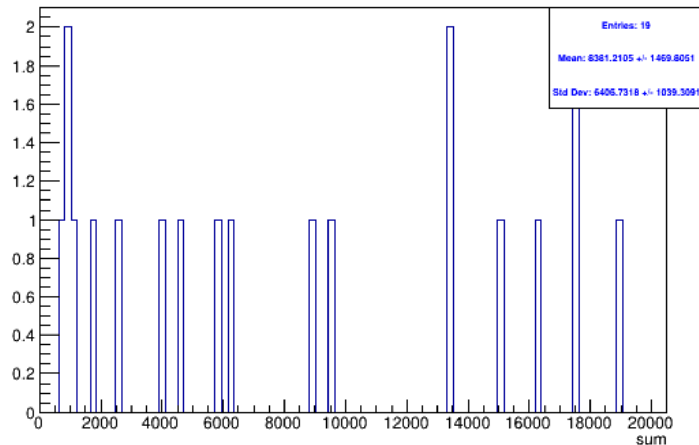
Run 5761 triggerwise, sums: Beam OFF
