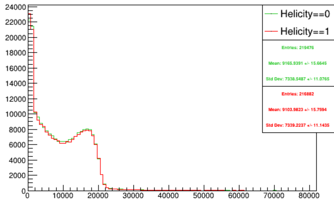
Run 5761 triggerwise, sums: Beam ON, Laser ON
