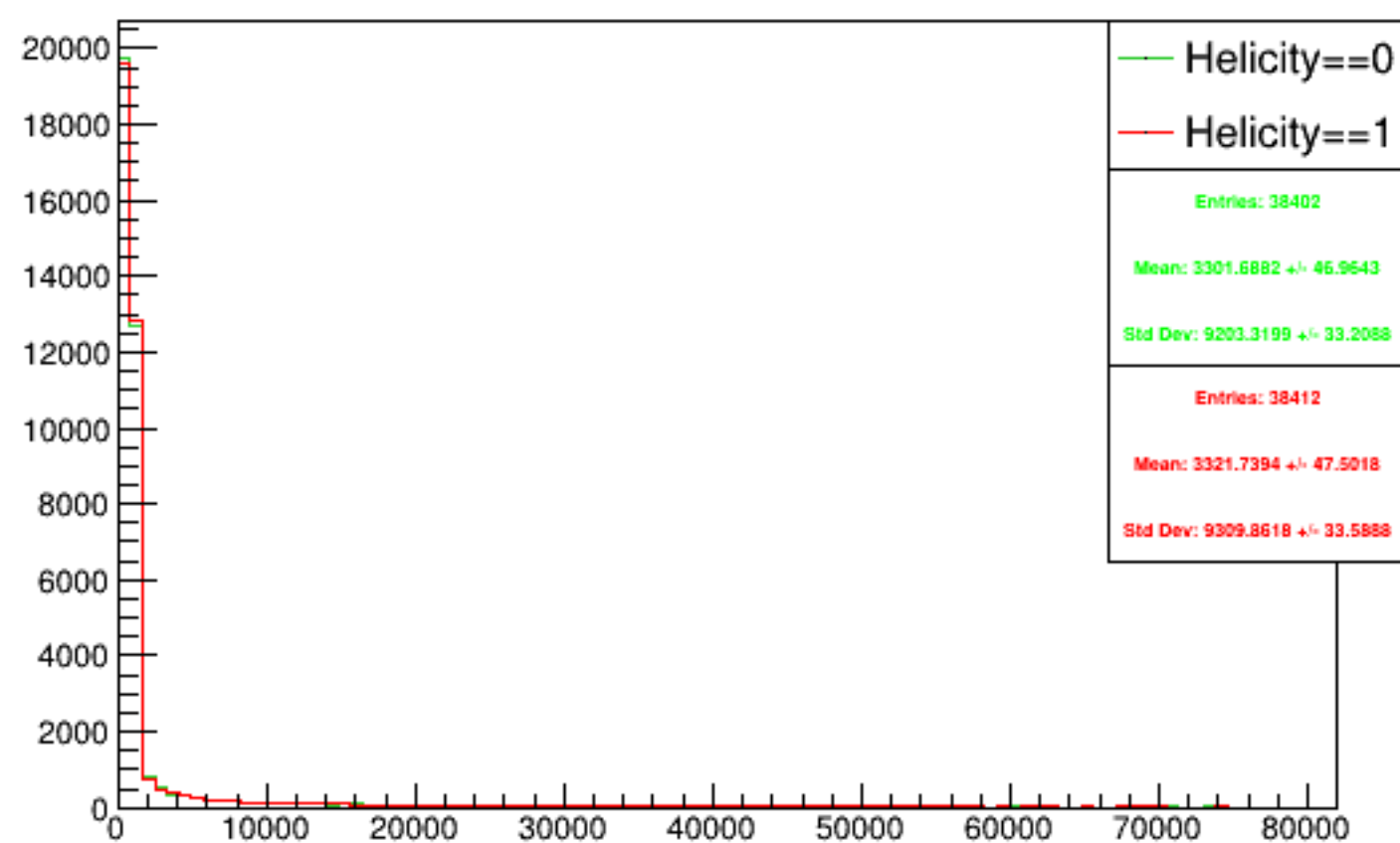
Run 5761 triggerwise, sums: Beam ON, Laser OFF
