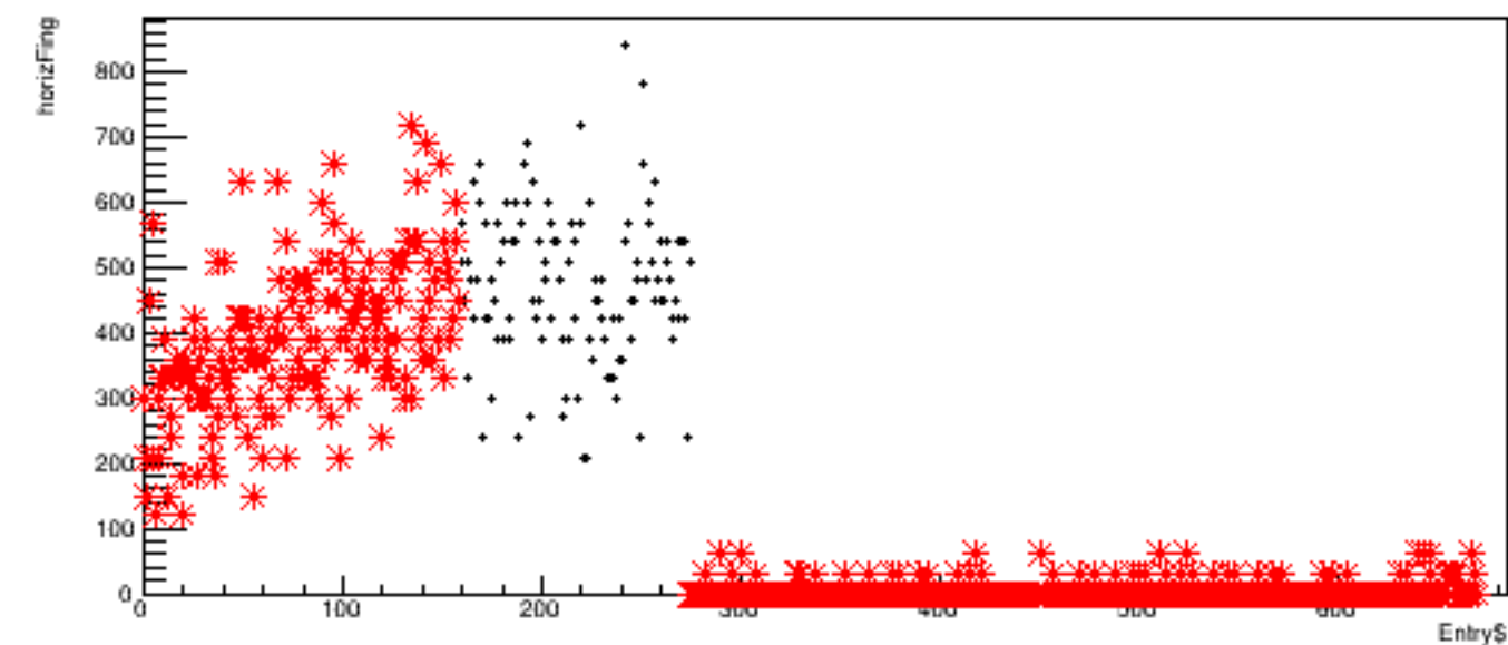
Run 5769, quartetwise: horizFing vs time
