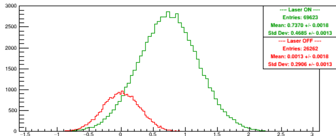
Run 5772 quartetwise, Diffs0
