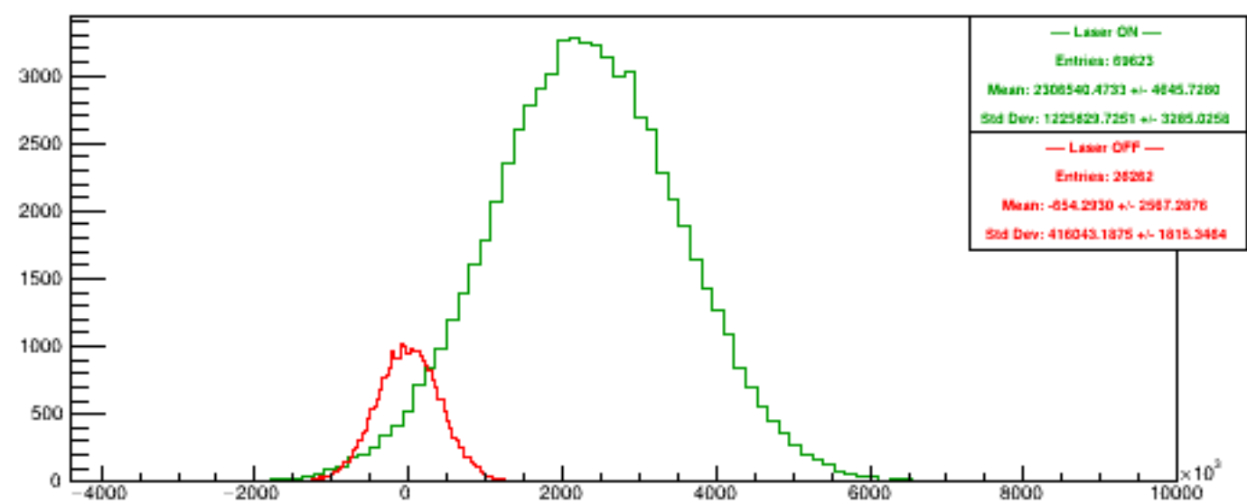
Run 5772 quartetwise, Diffs4
