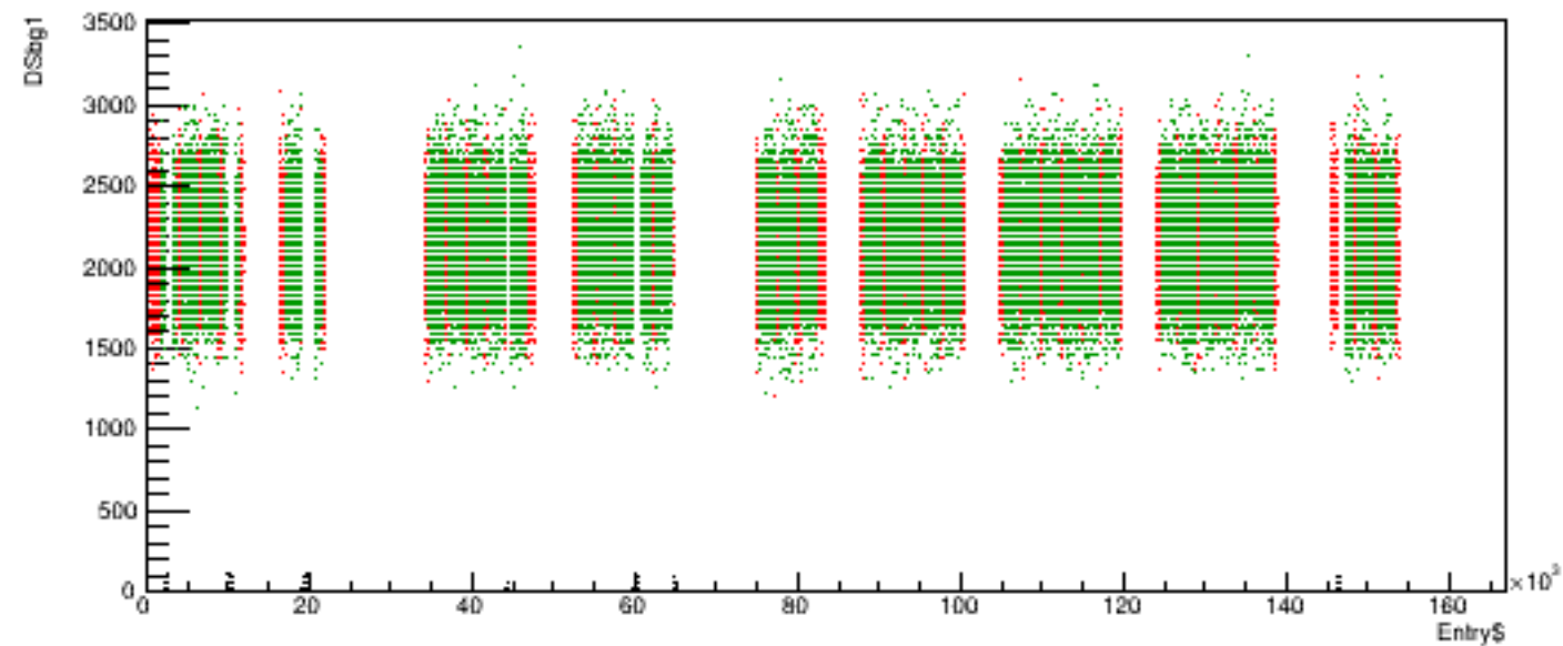
Run 5772 quartetwise, DSbg1 vs time
