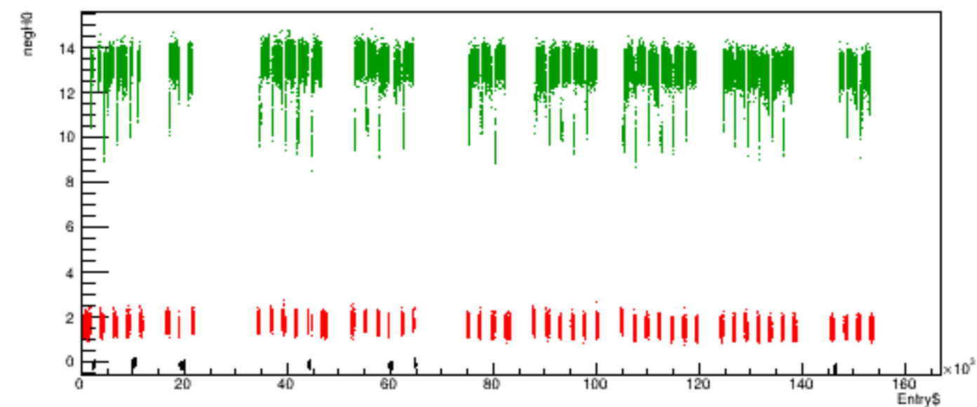
Run 5772 quartetwise, negH0 vs time
