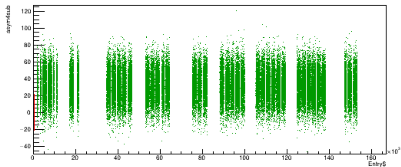
Run 5772 quartetwise, asym4sub vs time
