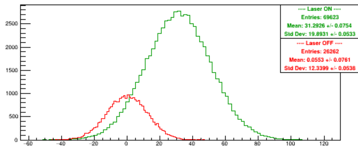
Run 5772 quartetwise, Asyms0
