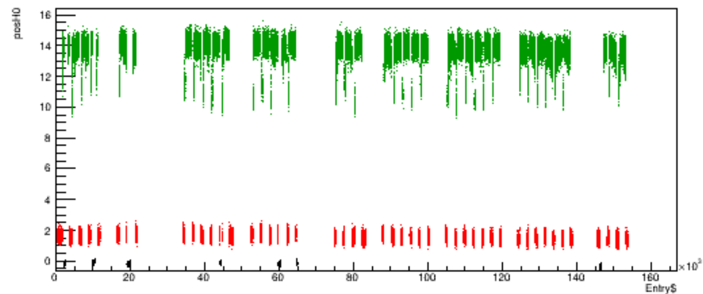
Run 5772 quartetwise, posH0 vs time
