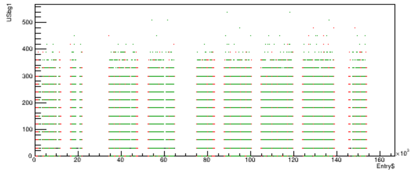
Run 5772 quartetwise, USbg1 vs time
