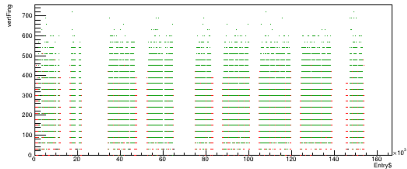
Run 5772 quartetwise, vertFing vs time
