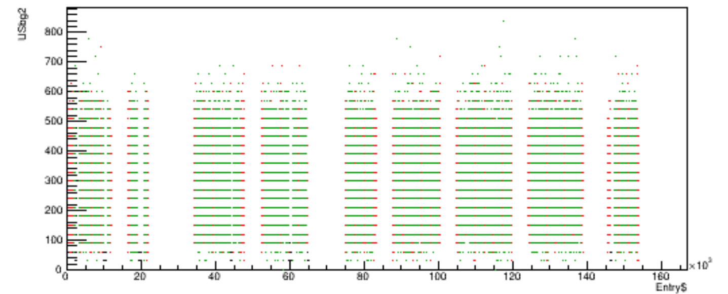
Run 5772 quartetwise, USbg2 vs time
