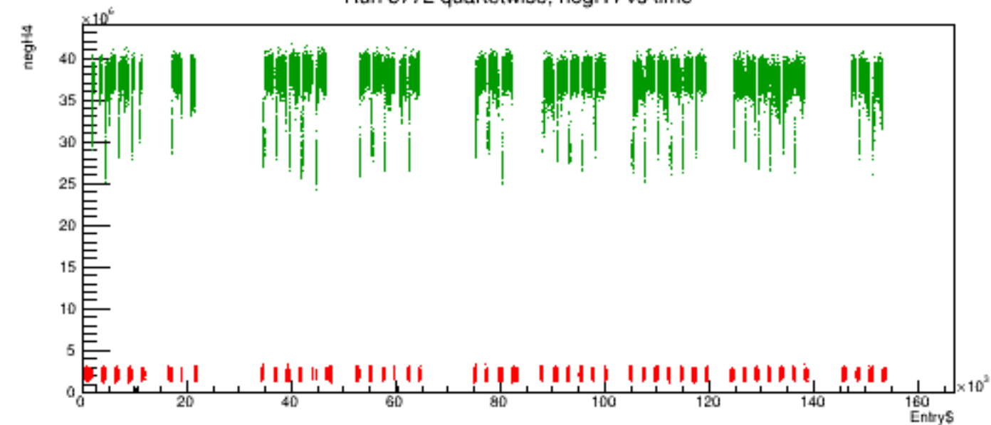
Run 5772 quartetwise, negH4 vs time
