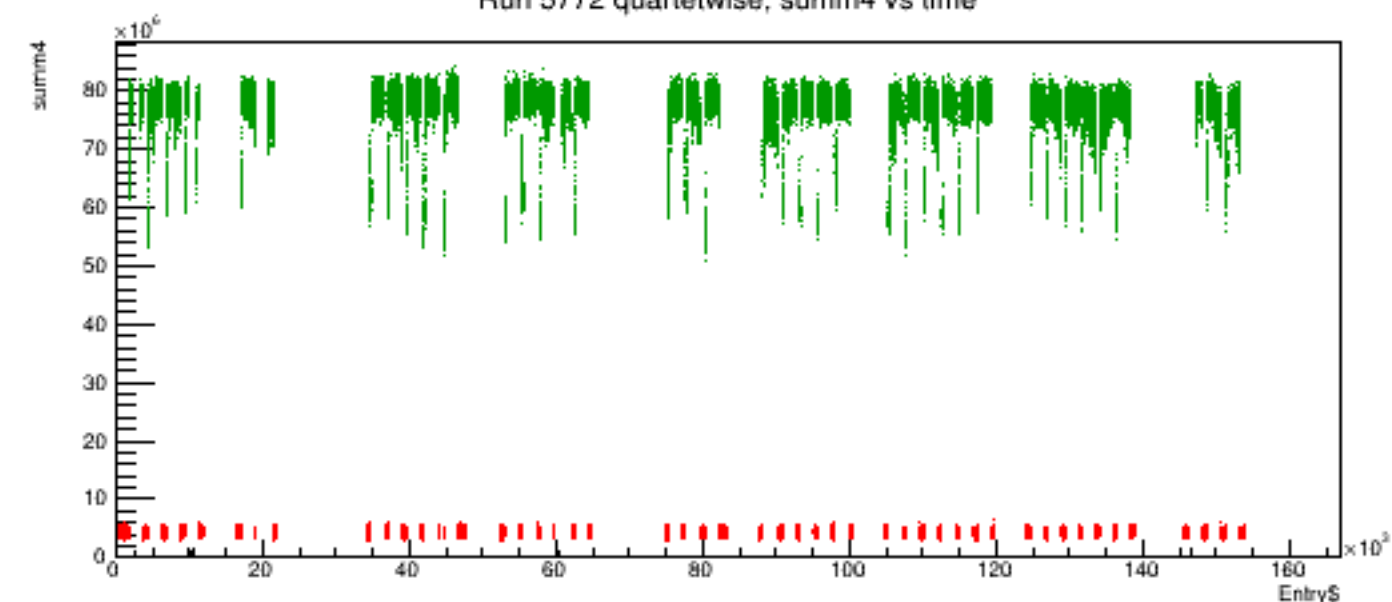
Run 5772 quartetwise, summ4 vs time
