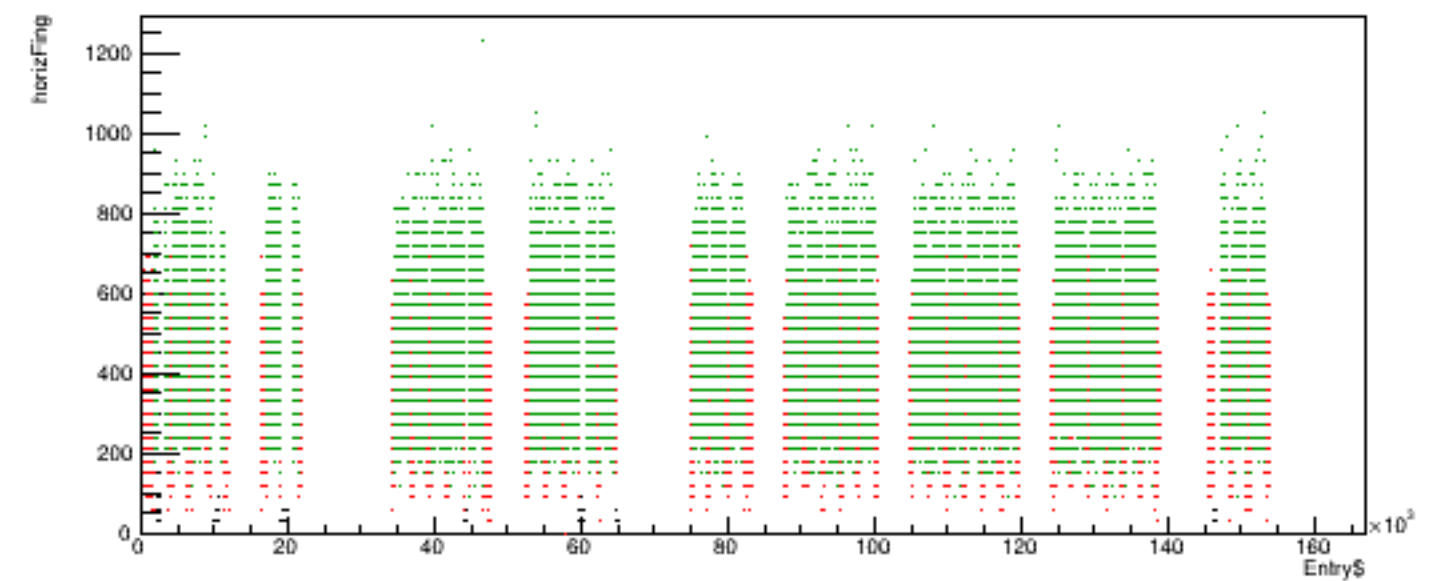
Run 5772 quartetwise, horizFing vs time
