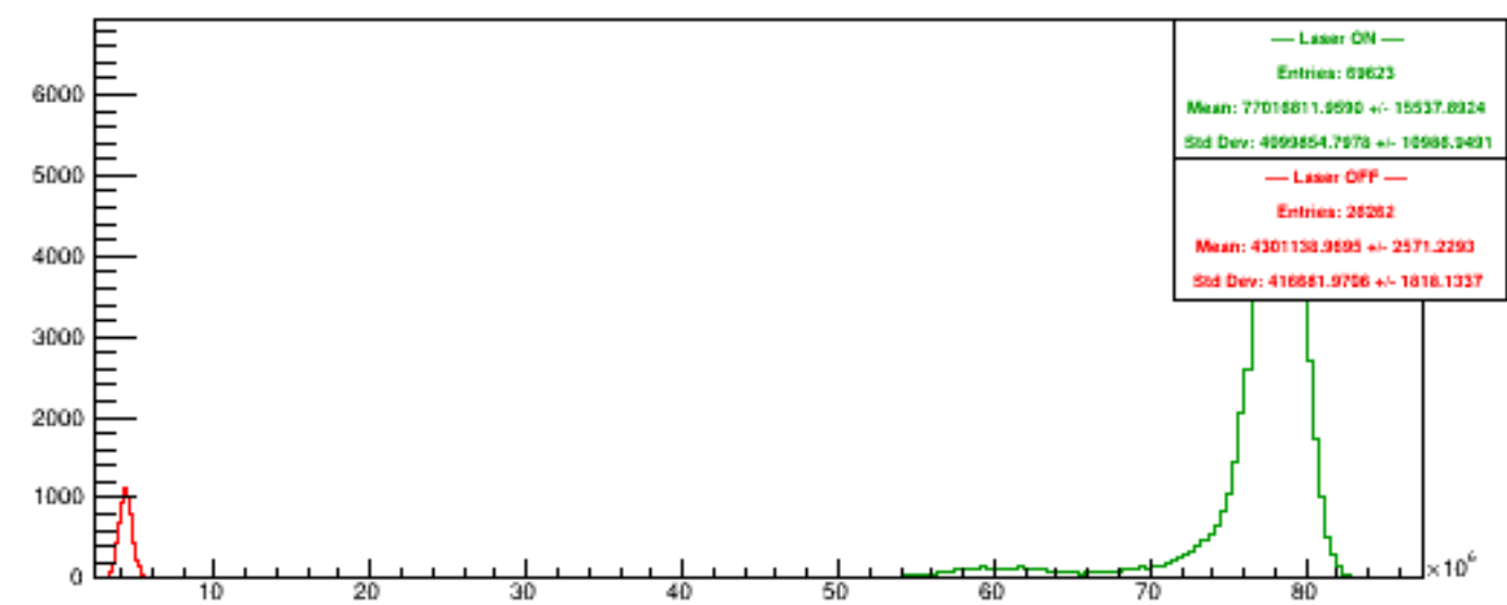
Run 5772 quartetwise, Sums4
