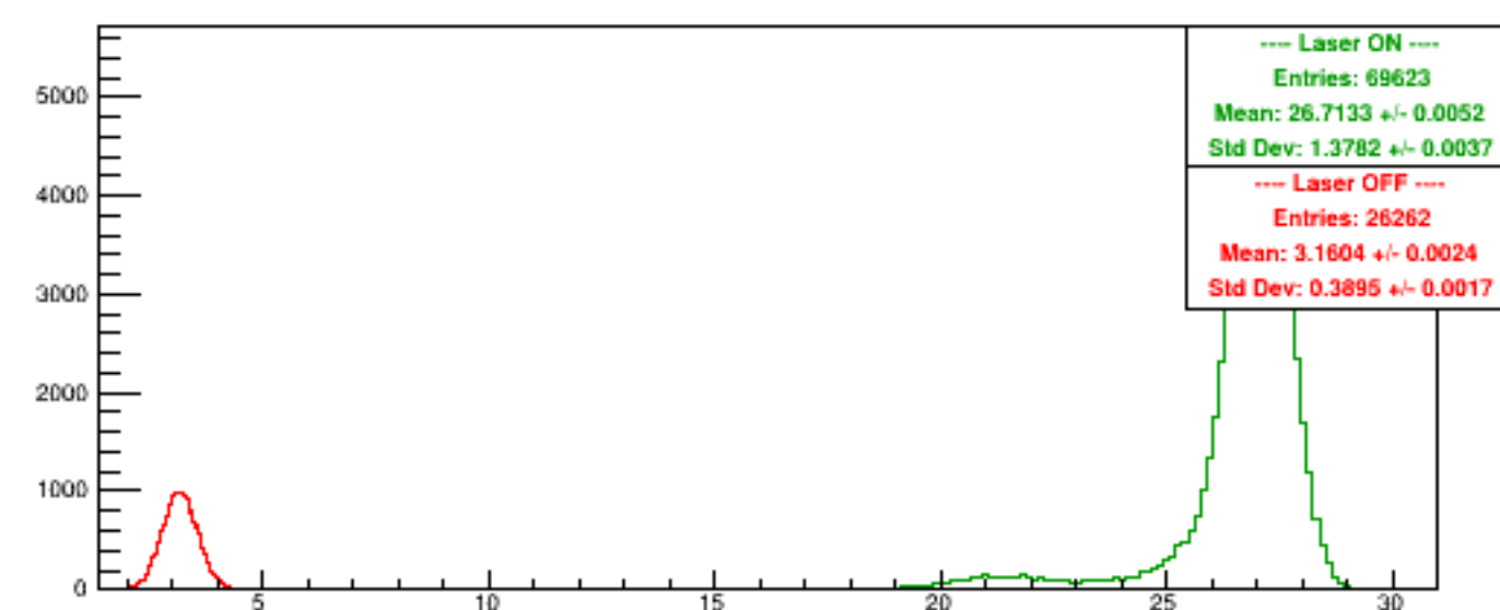
Run 5772 quartetwise, Sums0
