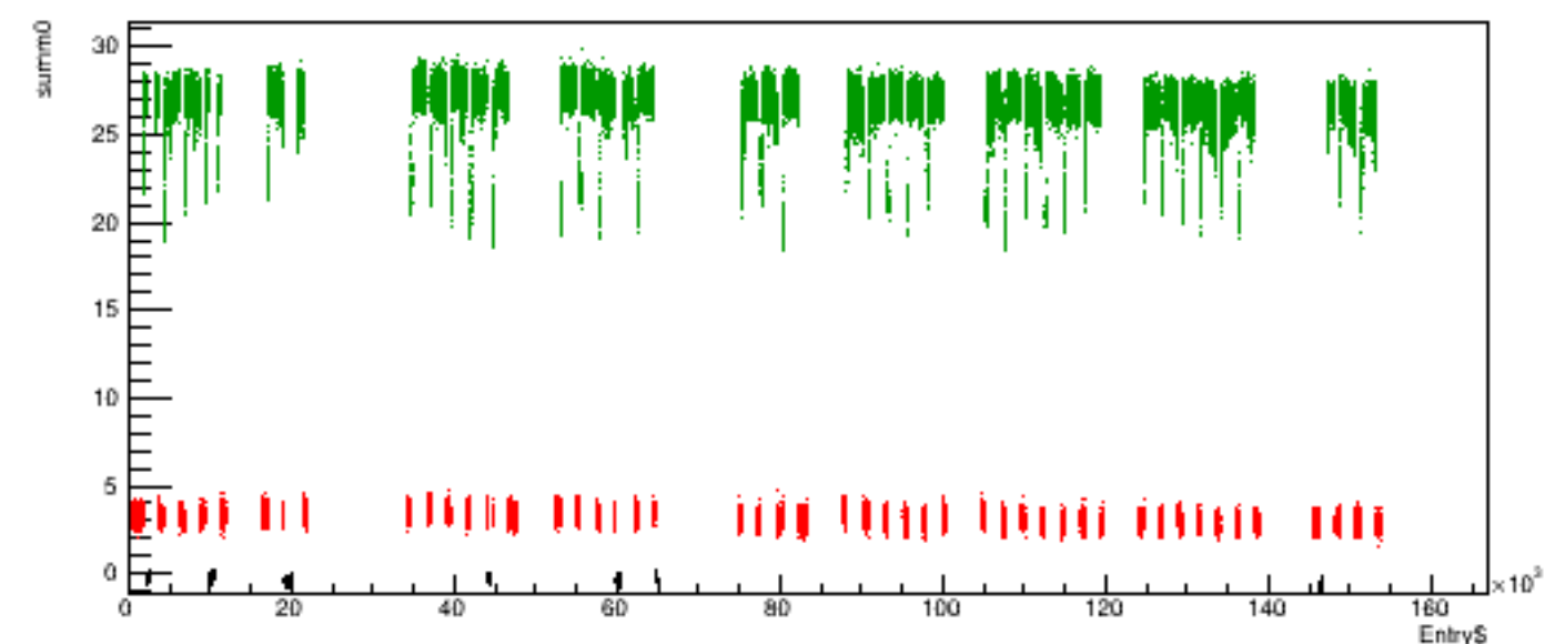
Run 5772 quartetwise, summ0 vs time
