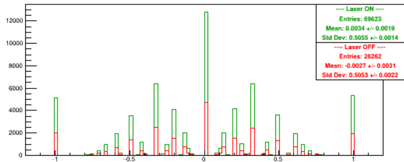
Run 5772 quartetwise, Asyms USbg1
