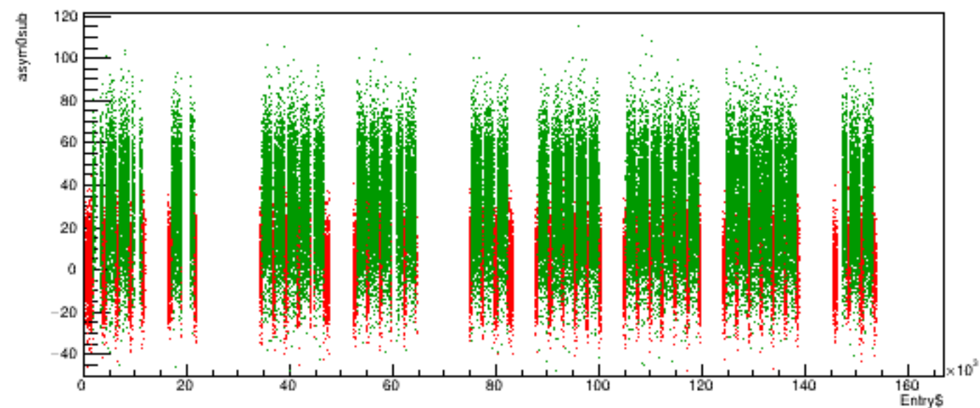
Run 5772 quartetwise, asym0sub vs time
