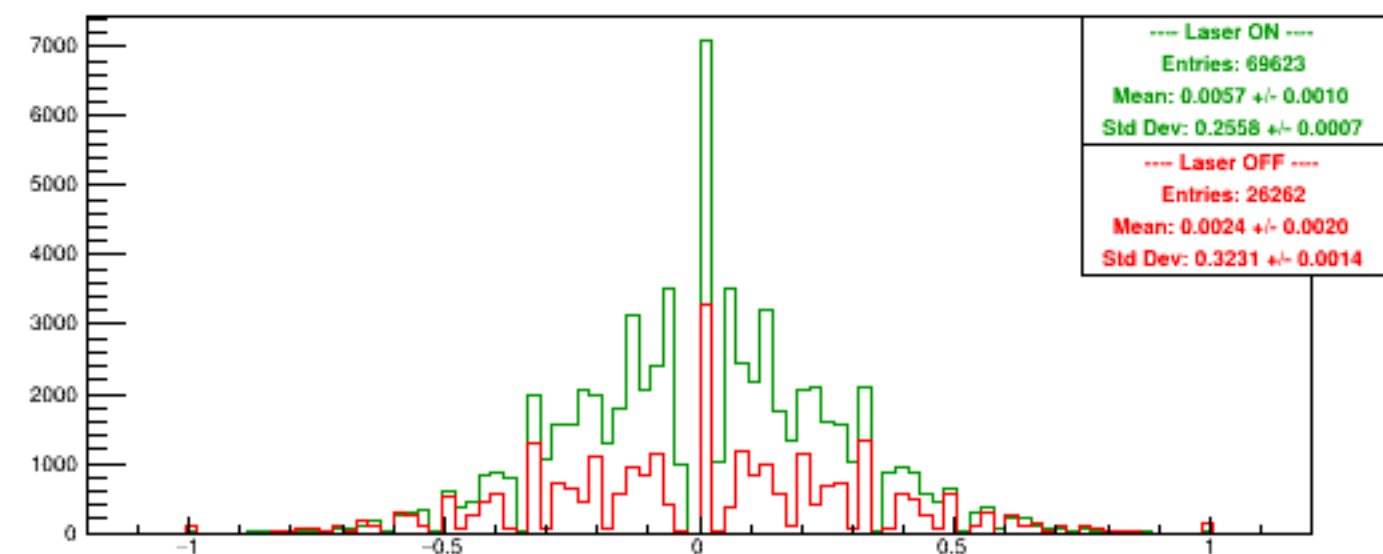
Run 5772 quartetwise, Asyms Vert Finger
