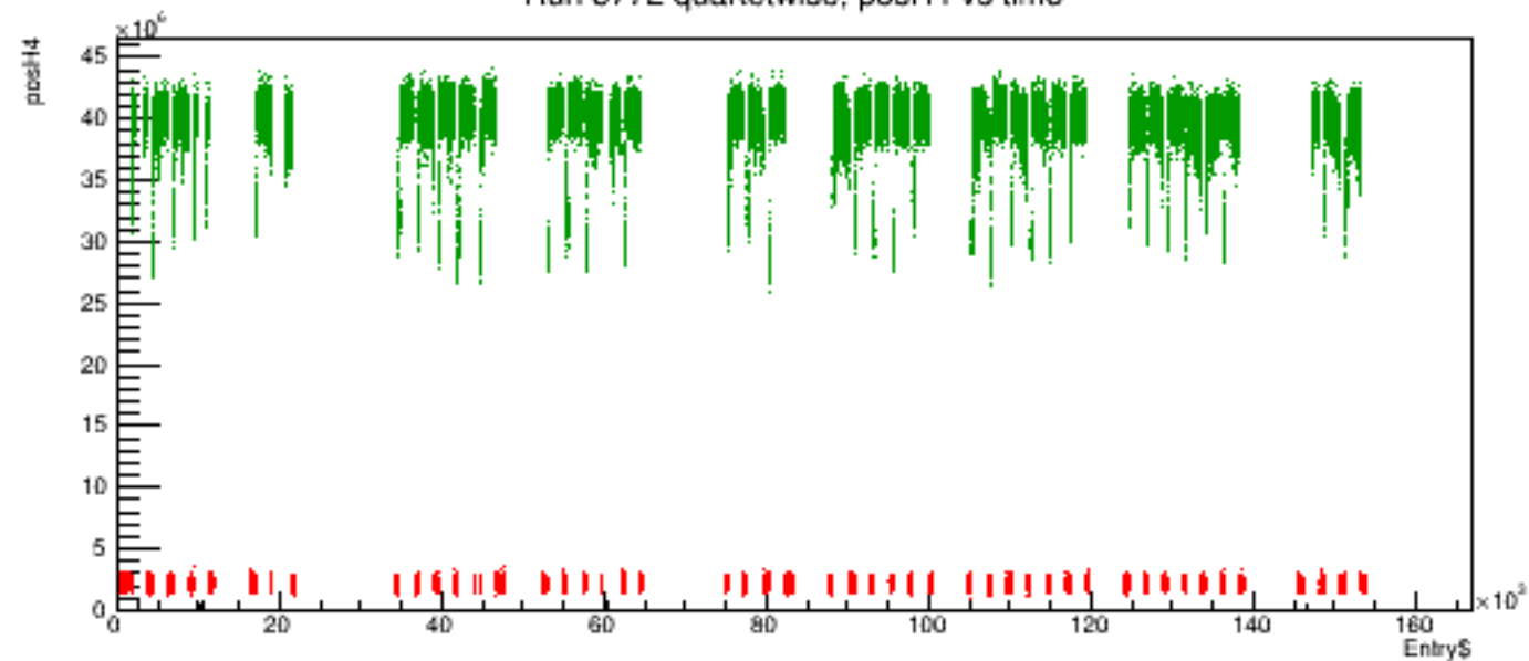
Run 5772 quartetwise, posH4 vs time
