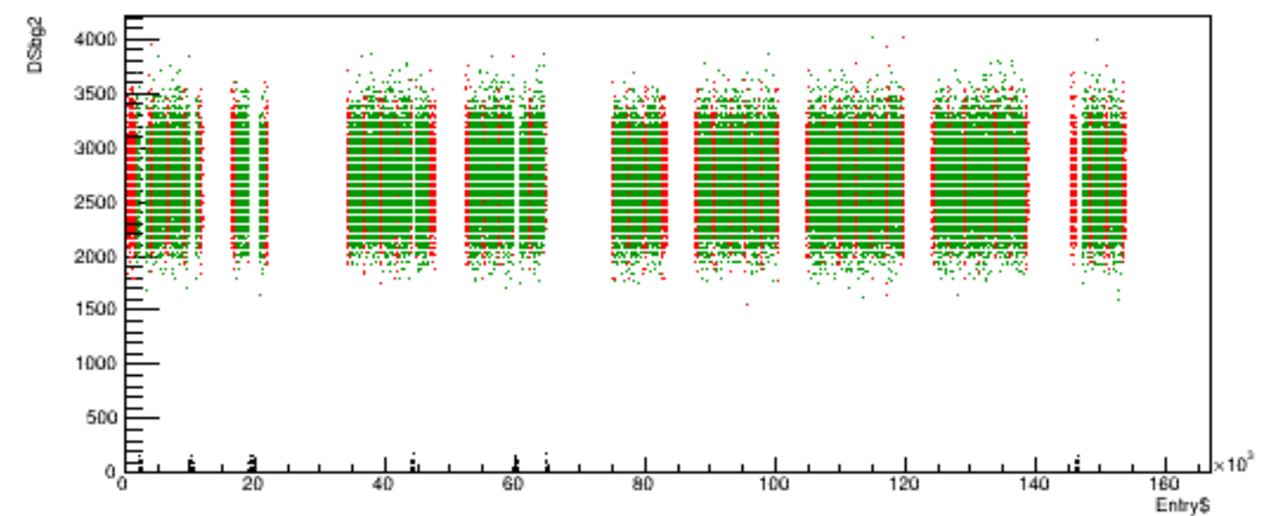
Run 5772 quartetwise, DSbg2 vs time
