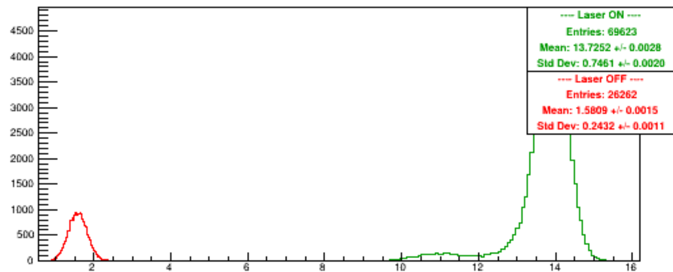
Run 5772 quartetwise, PosHelAcc0/NSamples0
