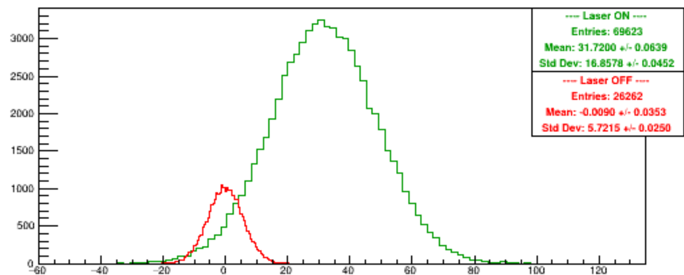
Run 5772 quartetwise, Asyms4
