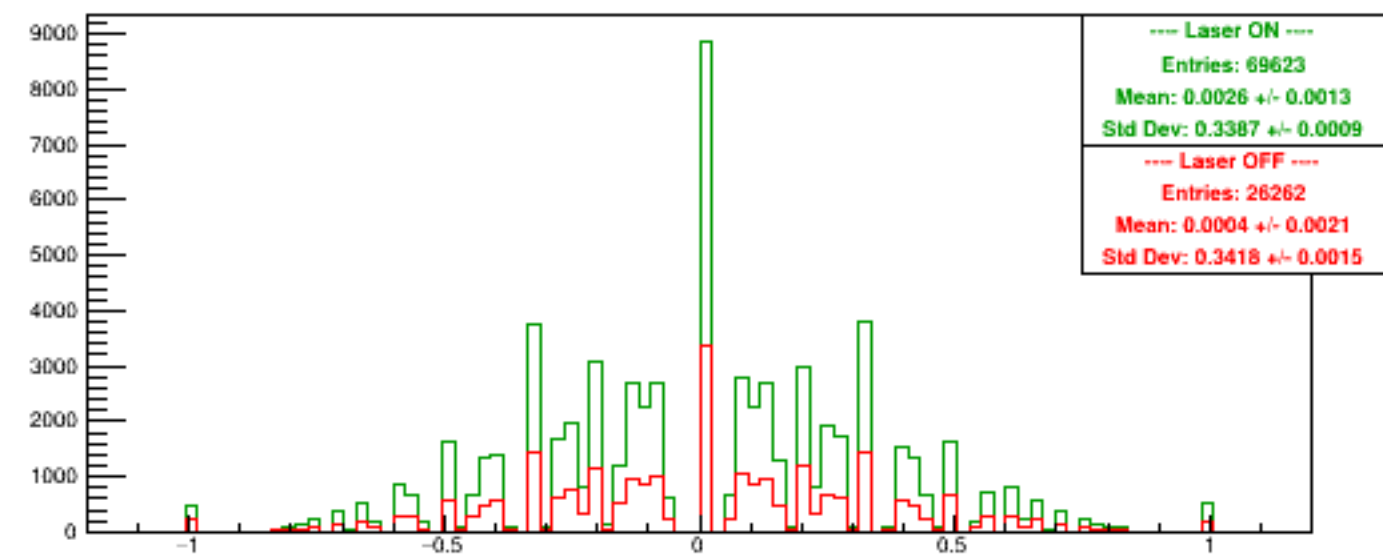
Run 5772 quartetwise, Asyms USbg2
