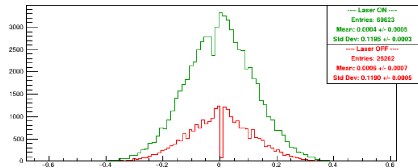
Run 5772 quartetwise, Asyms DSbg1
