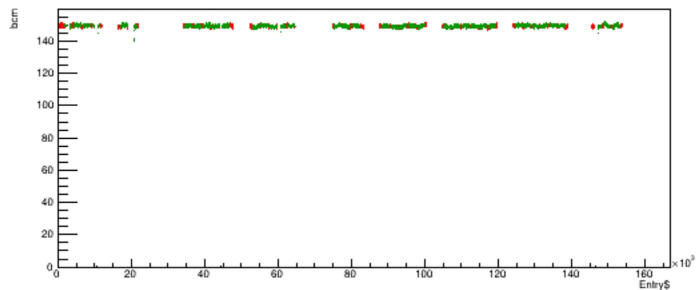
Run 5772 quartetwise, posH4 vs time
