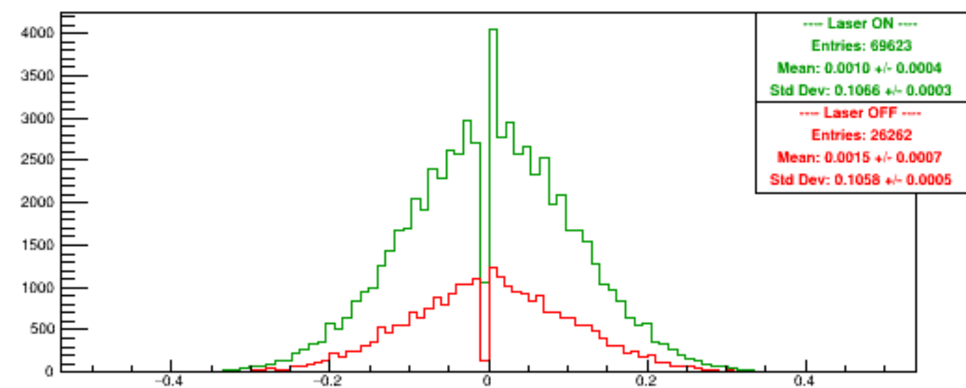
Run 5772 quartetwise, Asyms DSbg2
