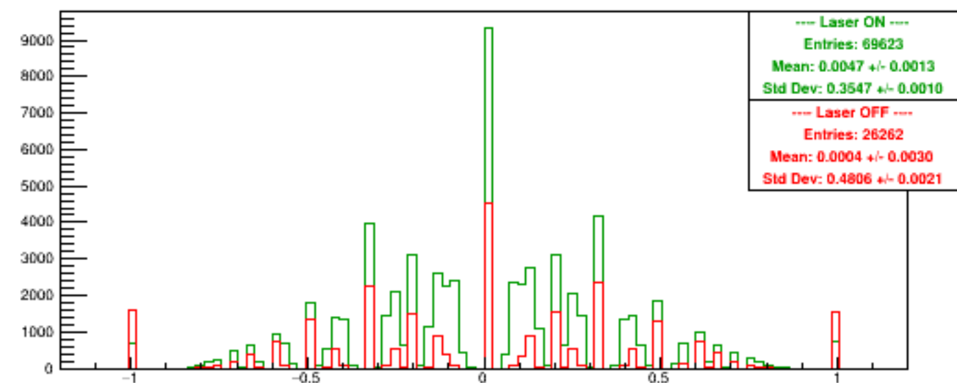
Run 5772 quartetwise, Asyms Horiz Finger
