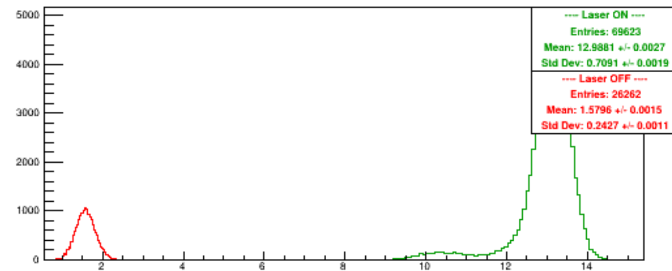
Run 5772 quartetwise, NegHelAcc0/NSamples0
