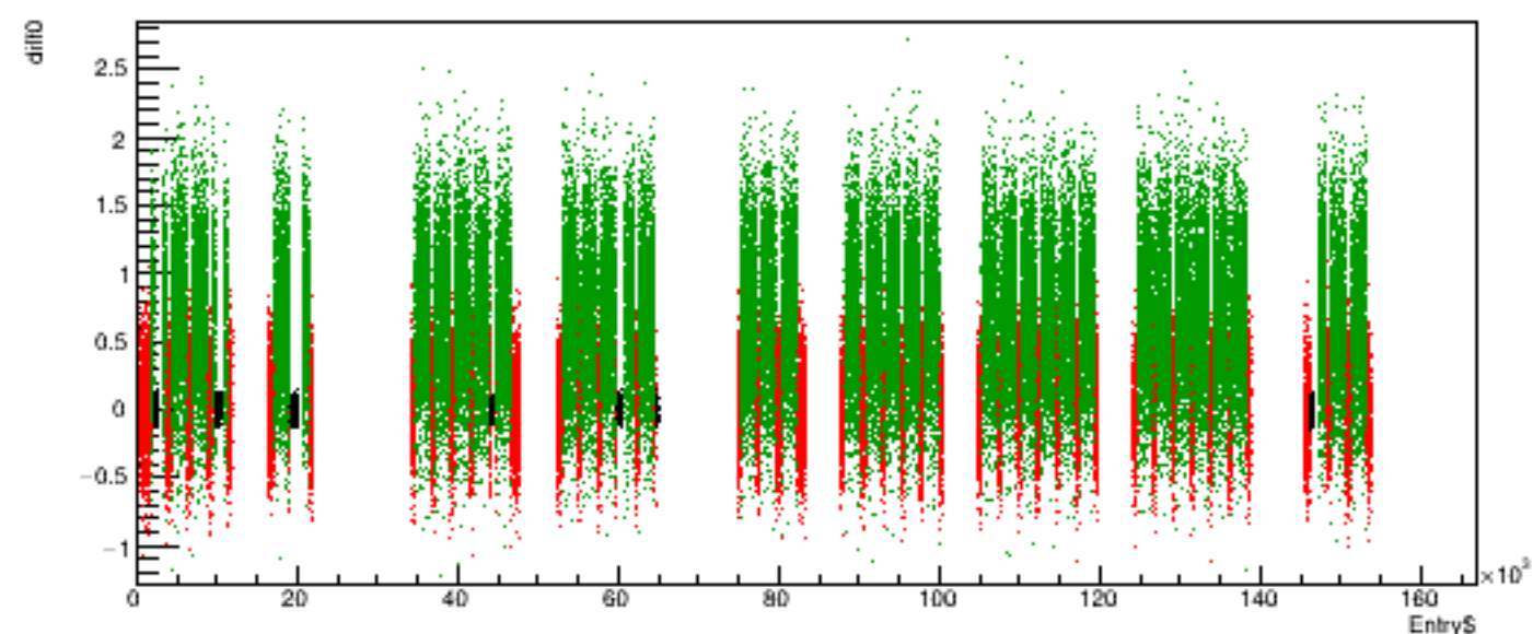
Run 5772 quartetwise, diff0 vs time
