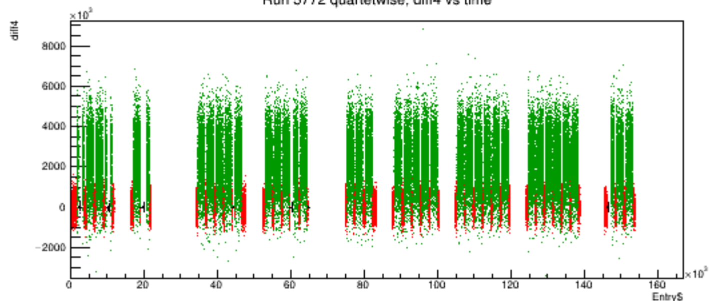
Run 5772 quartetwise, diff4 vs time
