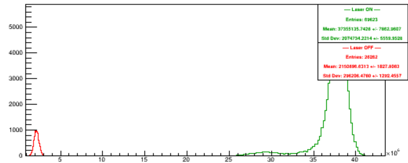
Run 5772 quartetwise, NegHelAcc4
