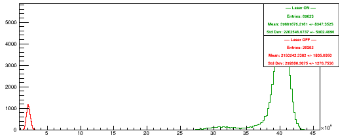
Run 5772 quartetwise, PosHelAcc4
