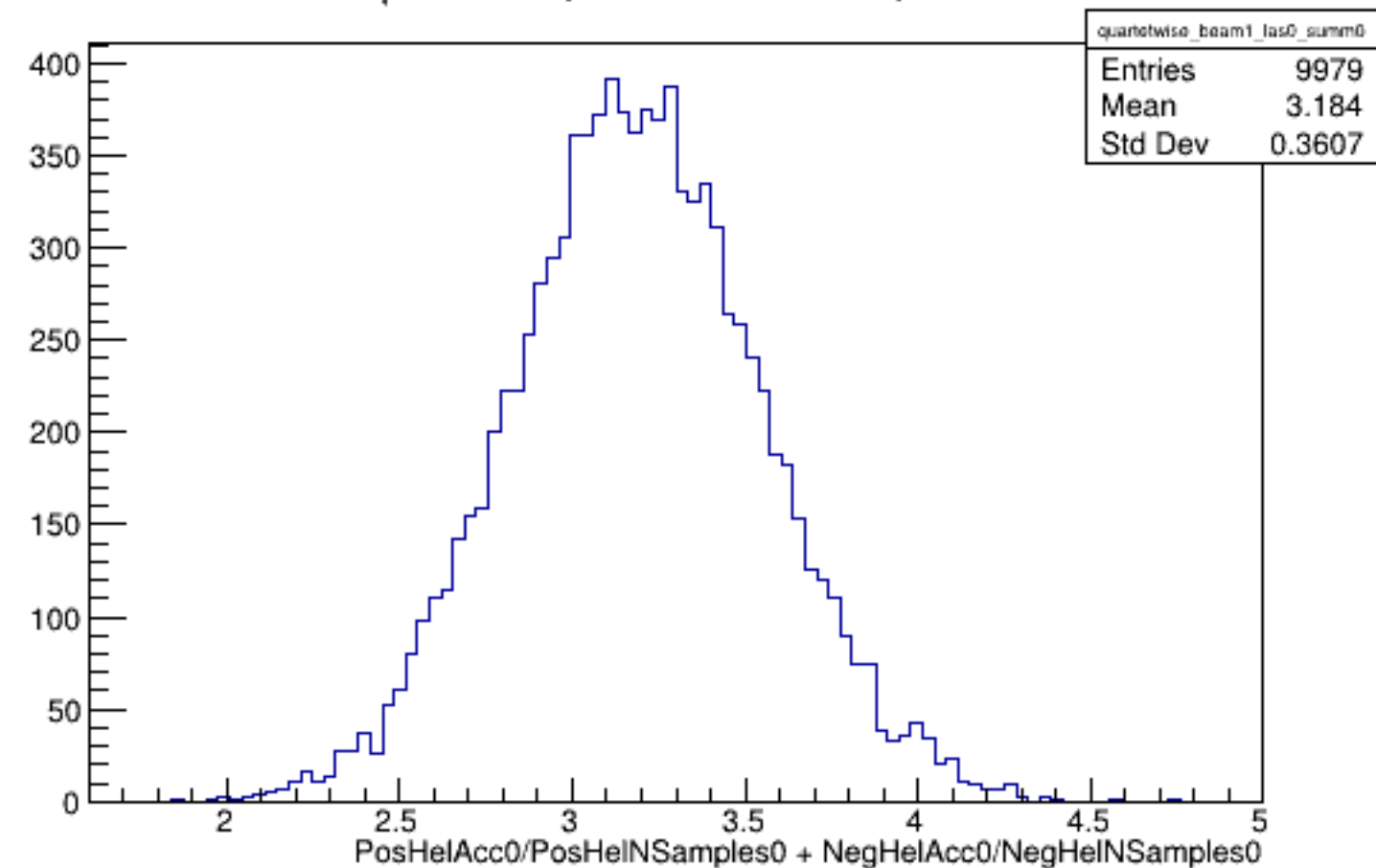
Run 5773 quartetwise, Sums0: Beam ON, Laser OFF
