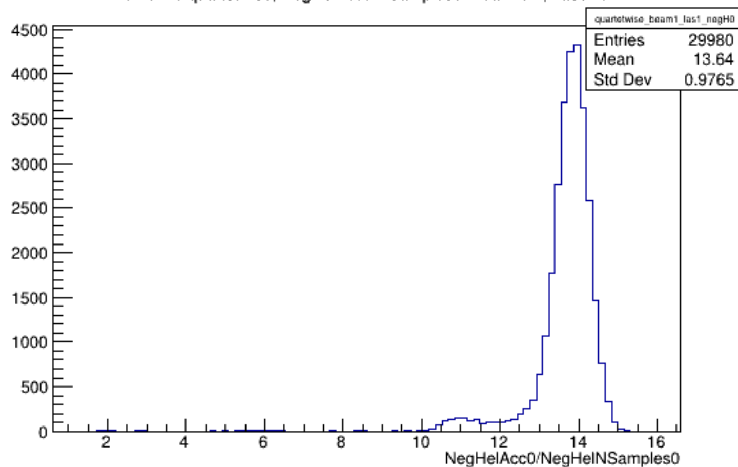
Run 5773 quartetwise, NegHelAcc0/NSamples0: Beam ON, Laser ON
