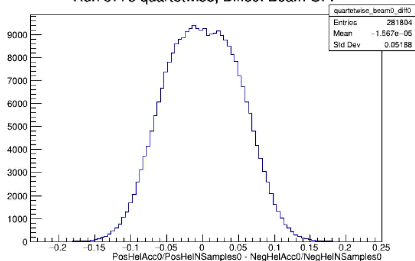
Run 5773 quartetwise, Diffs0: Beam OFF
