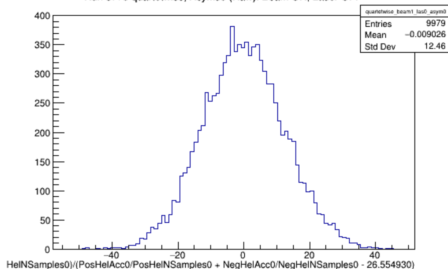
Run 5773 quartetwise, Asyms0 (Raw): Beam ON, Laser OFF
