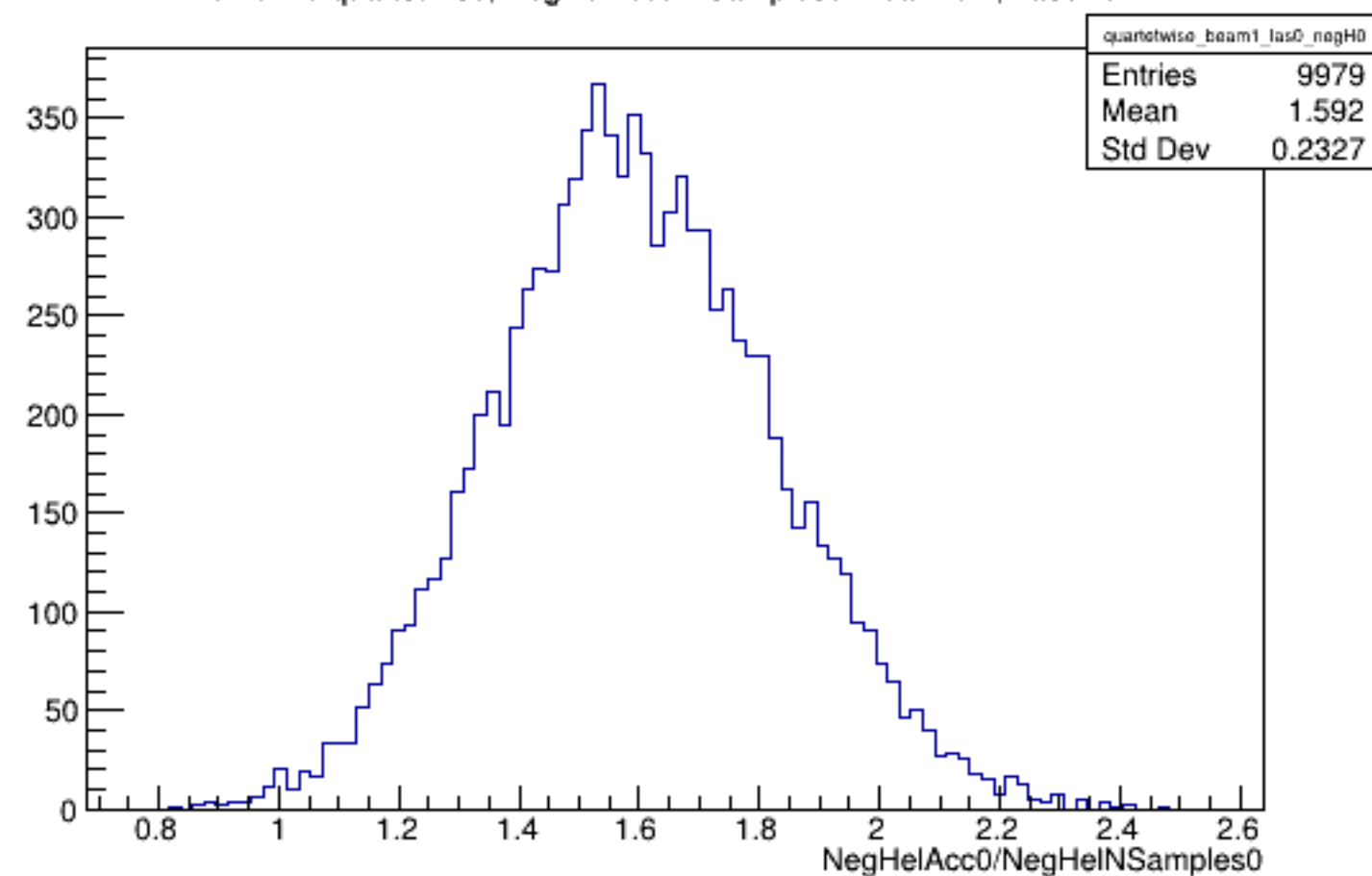
Run 5773 quartetwise, NegHelAcc0/NSamples0: Beam ON, Laser OFF
