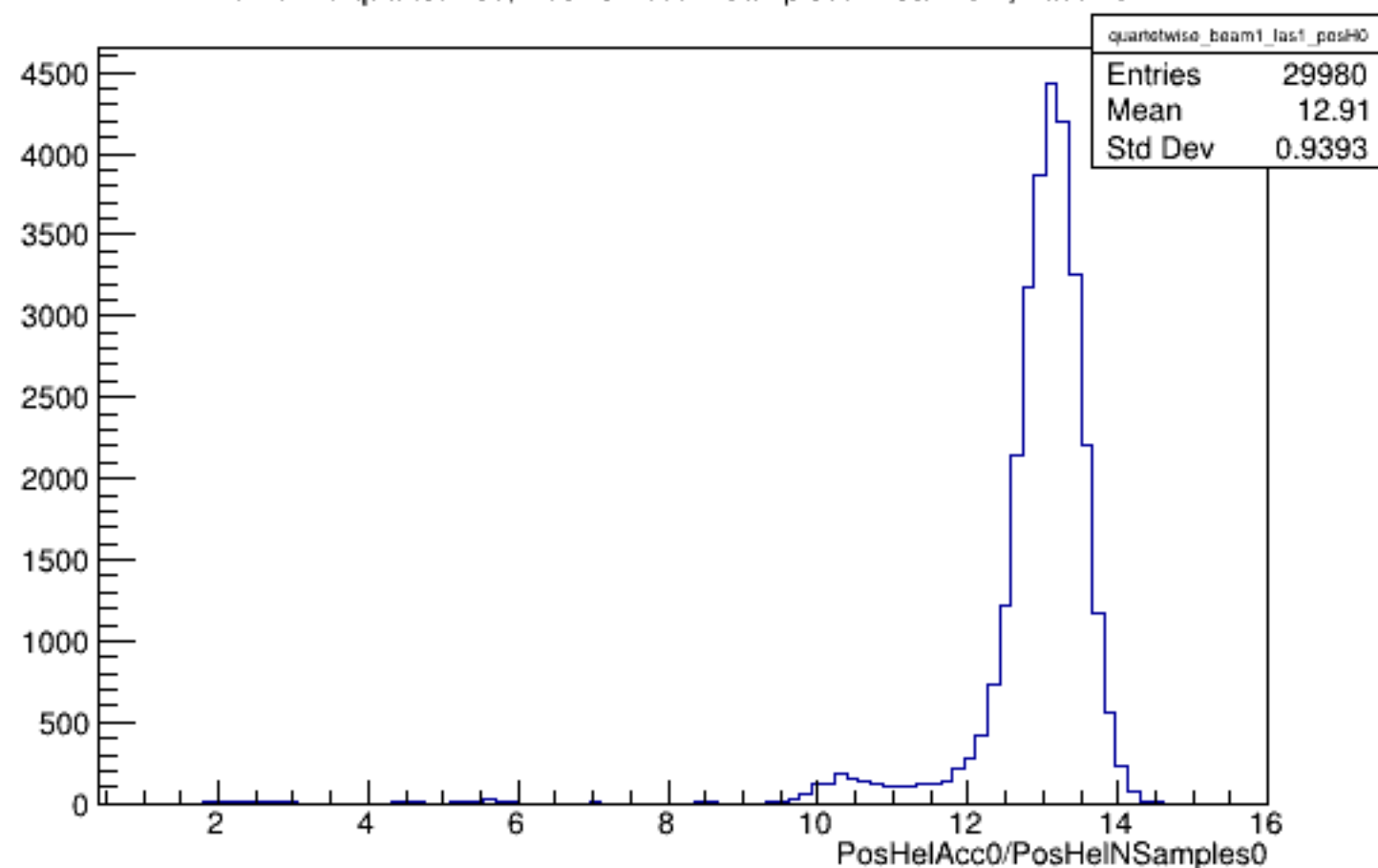
Run 5773 quartetwise, PosHelAcc0/NSamples0: Beam ON, Laser ON
