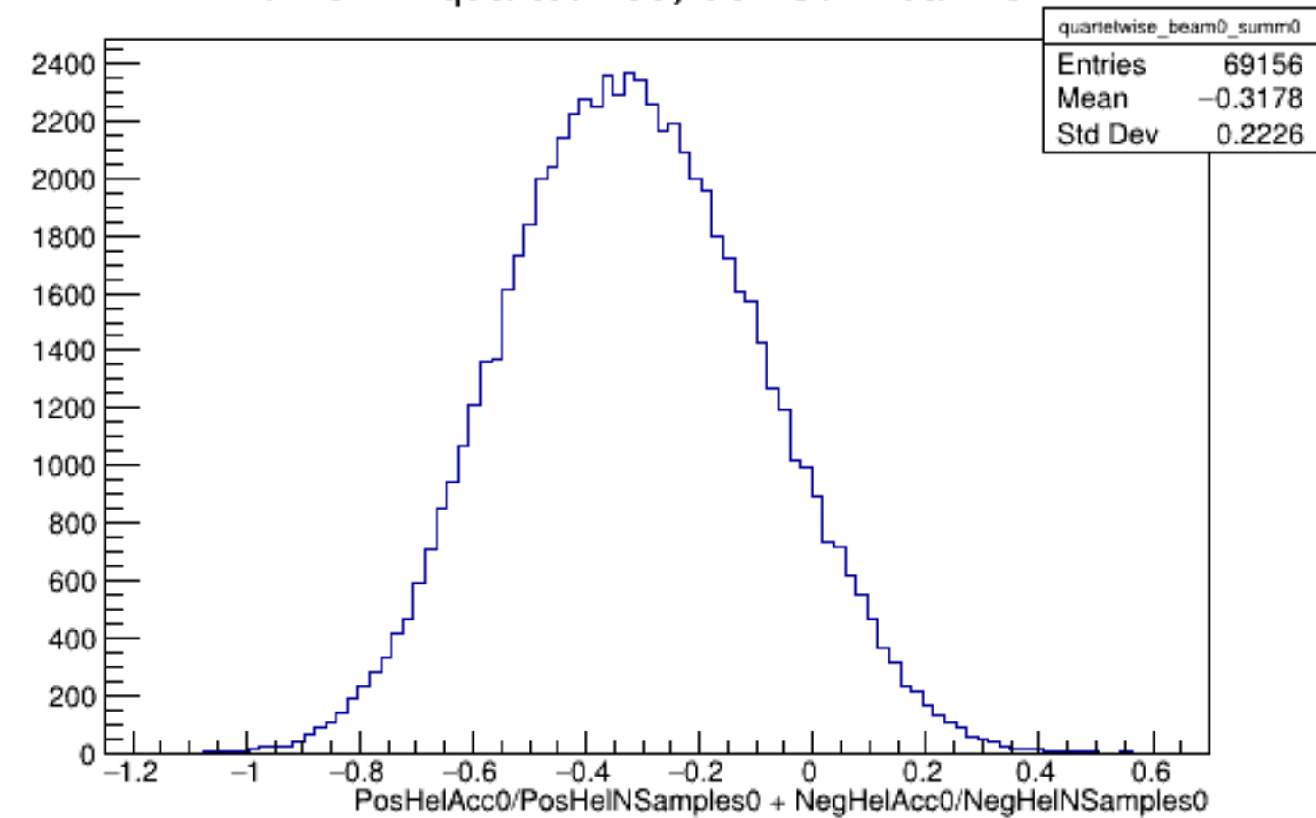
Run 5777 quartetwise, Sums0: Beam OFF
