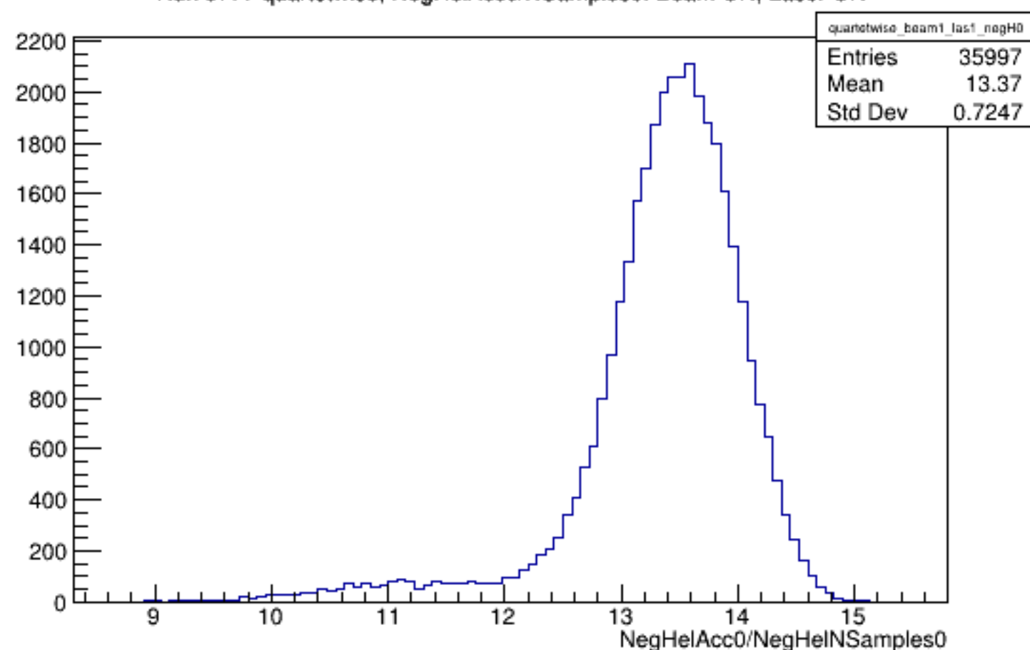
Run 5777 quartetwise, NegHelAcc0/NSamples0: Beam ON, Laser ON
