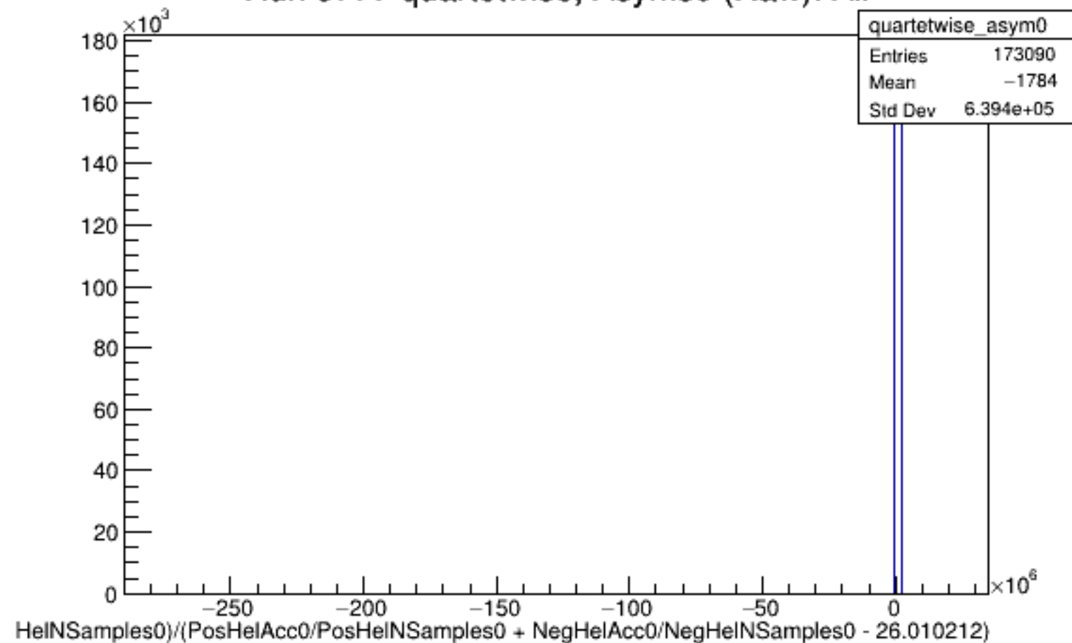
Run 5777 quartetwise, Asyms0 (Raw): All
