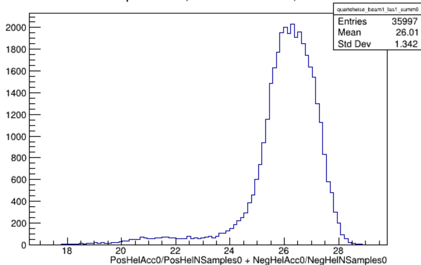
Run 5777 quartetwise, Sums0: Beam ON, Laser ON
