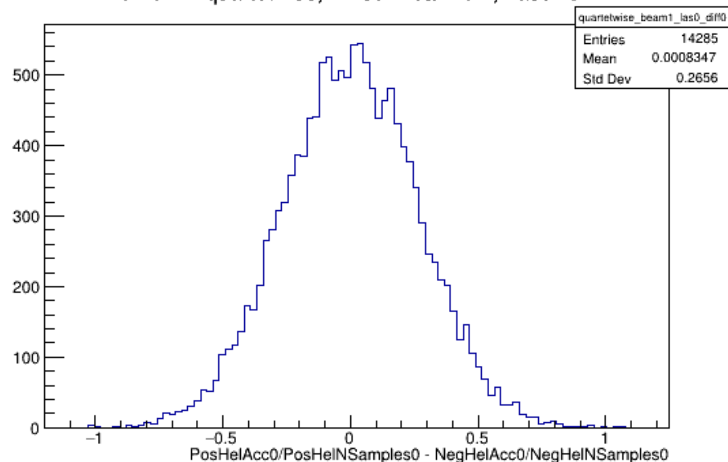
Run 5777 quartetwise, Diffs0: Beam ON, Laser OFF
