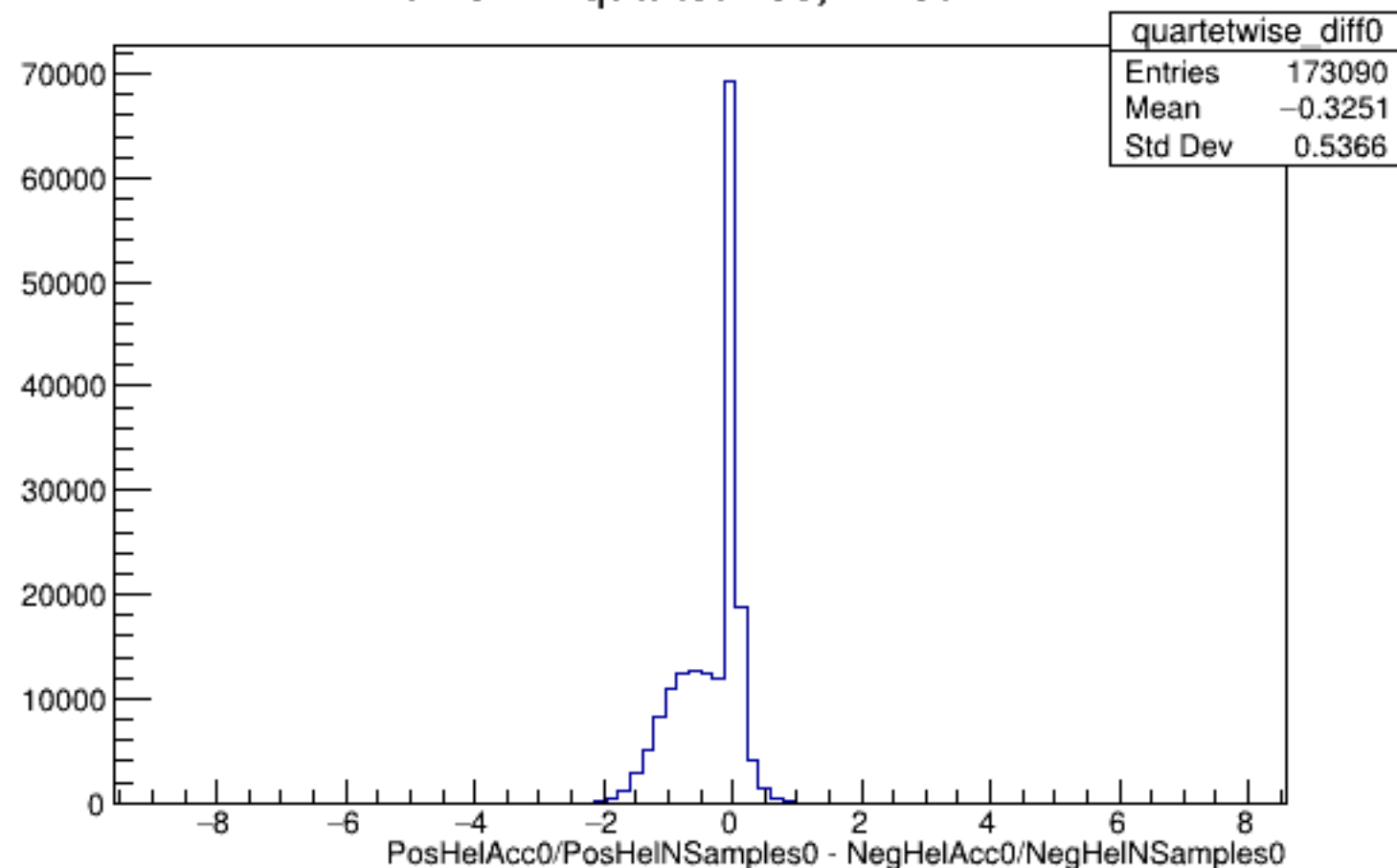
Run 5777 quartetwise, Diffs0: All
