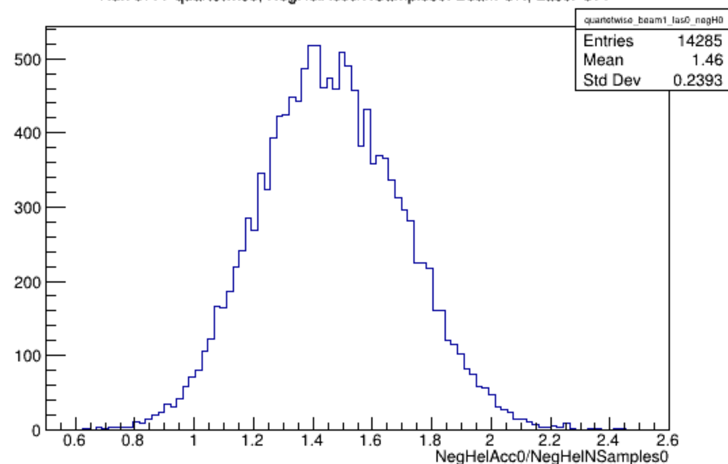
Run 5777 quartetwise, NegHelAcc0/NSamples0: Beam ON, Laser OFF
