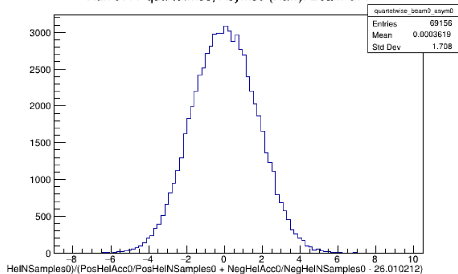
Run 5777 quartetwise, Asyms0 (Raw): Beam OFF
