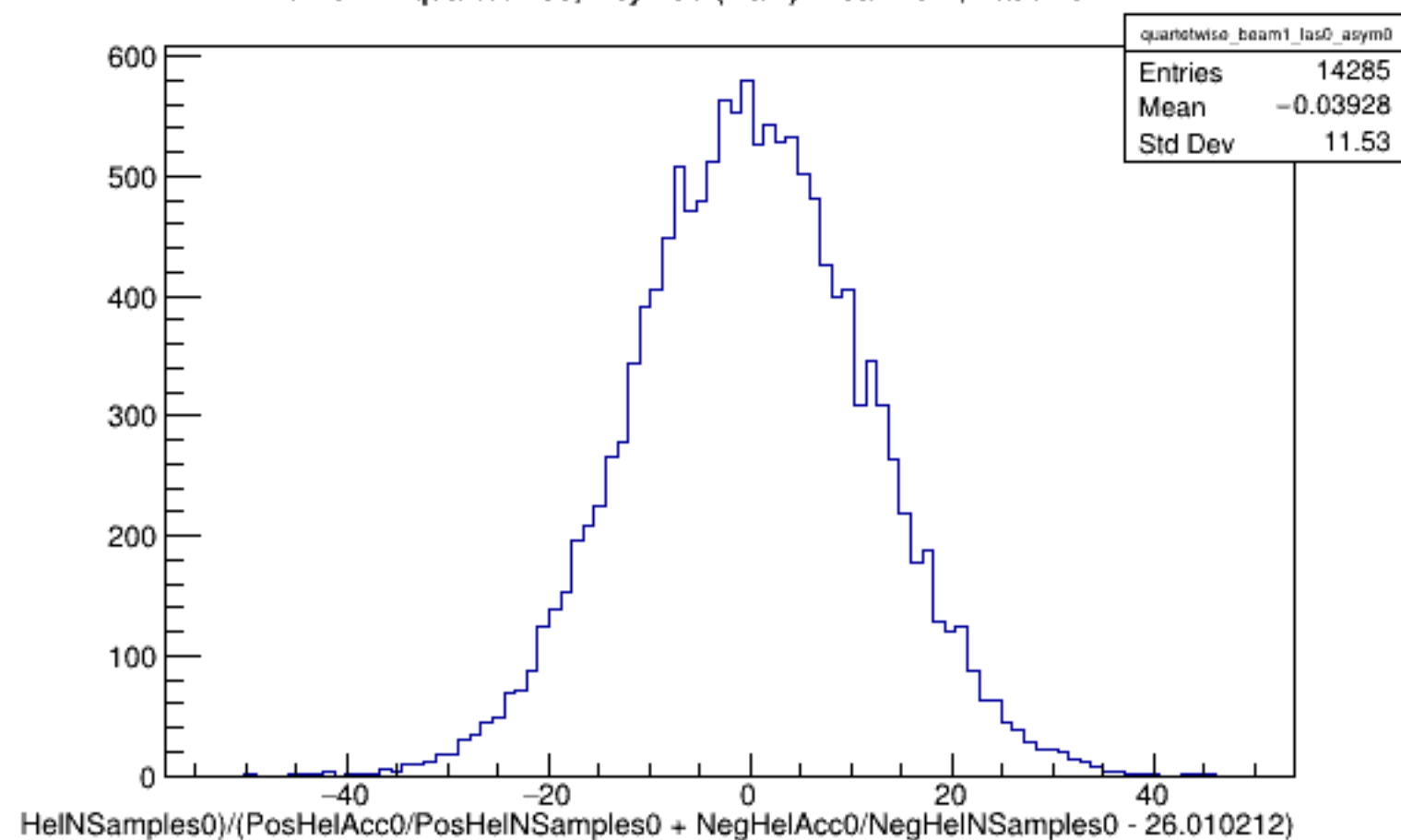
Run 5777 quartetwise, Asyms0 (Raw): Beam ON, Laser OFF
