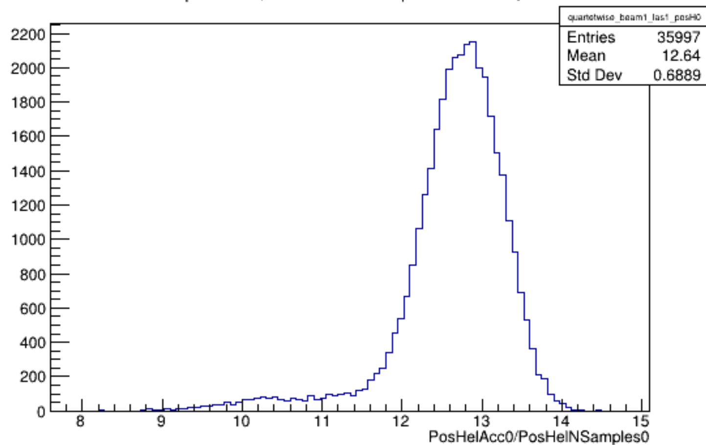
Run 5777 quartetwise, PosHelAcc0/NSamples0: Beam ON, Laser ON
