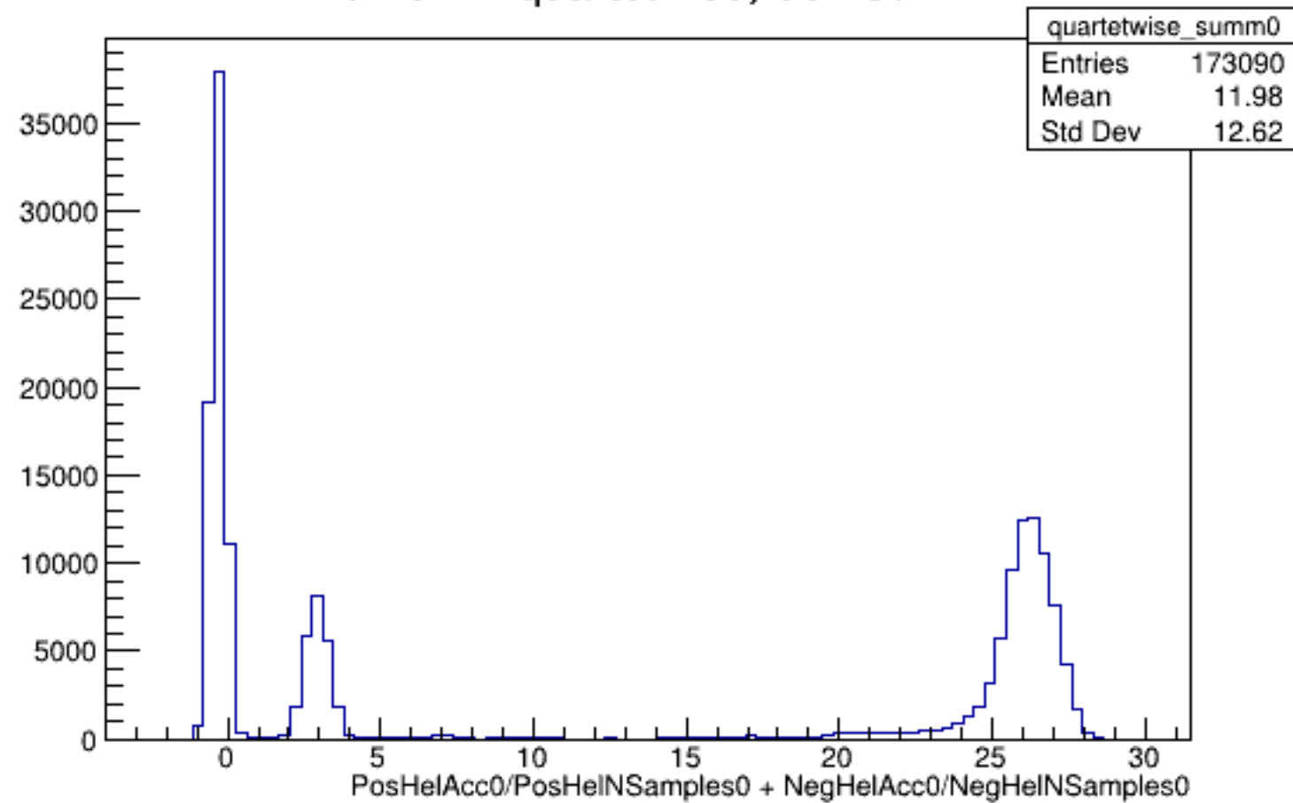
Run 5777 quartetwise, Sums0: All
