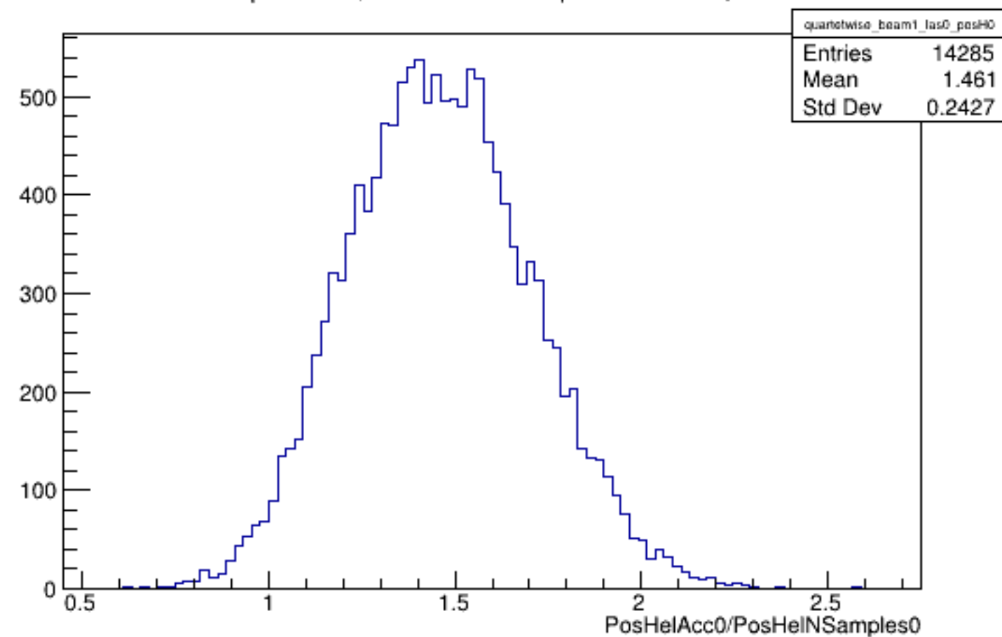
Run 5777 quartetwise, PosHelAcc0/NSamples0: Beam ON, Laser OFF
