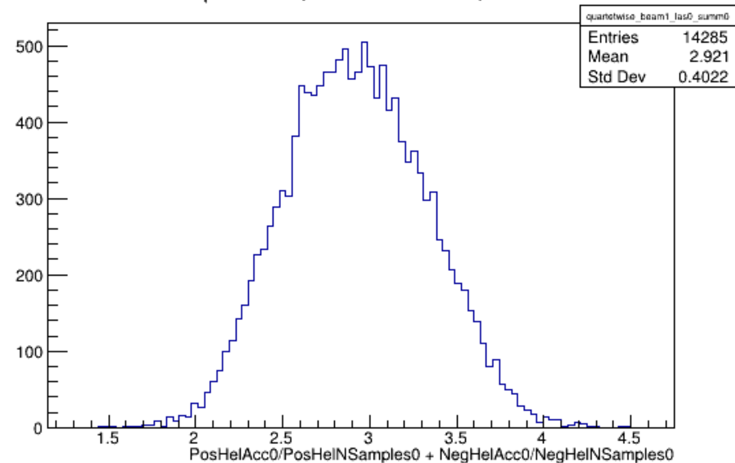
Run 5777 quartetwise, Sums0: Beam ON, Laser OFF
