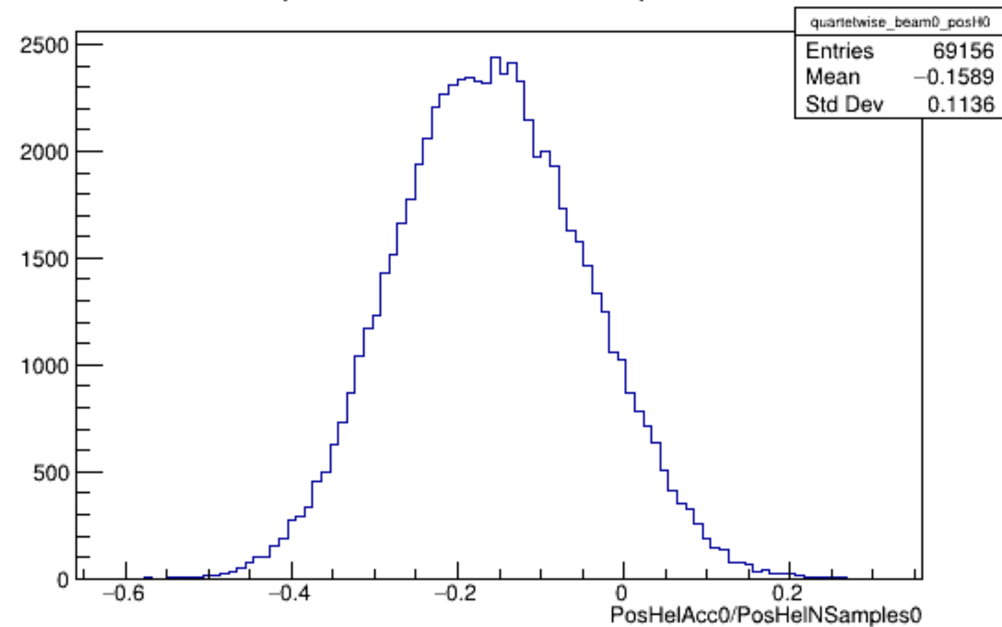
Run 5777 quartetwise, PosHelAcc0/NSamples0: Beam OFF
