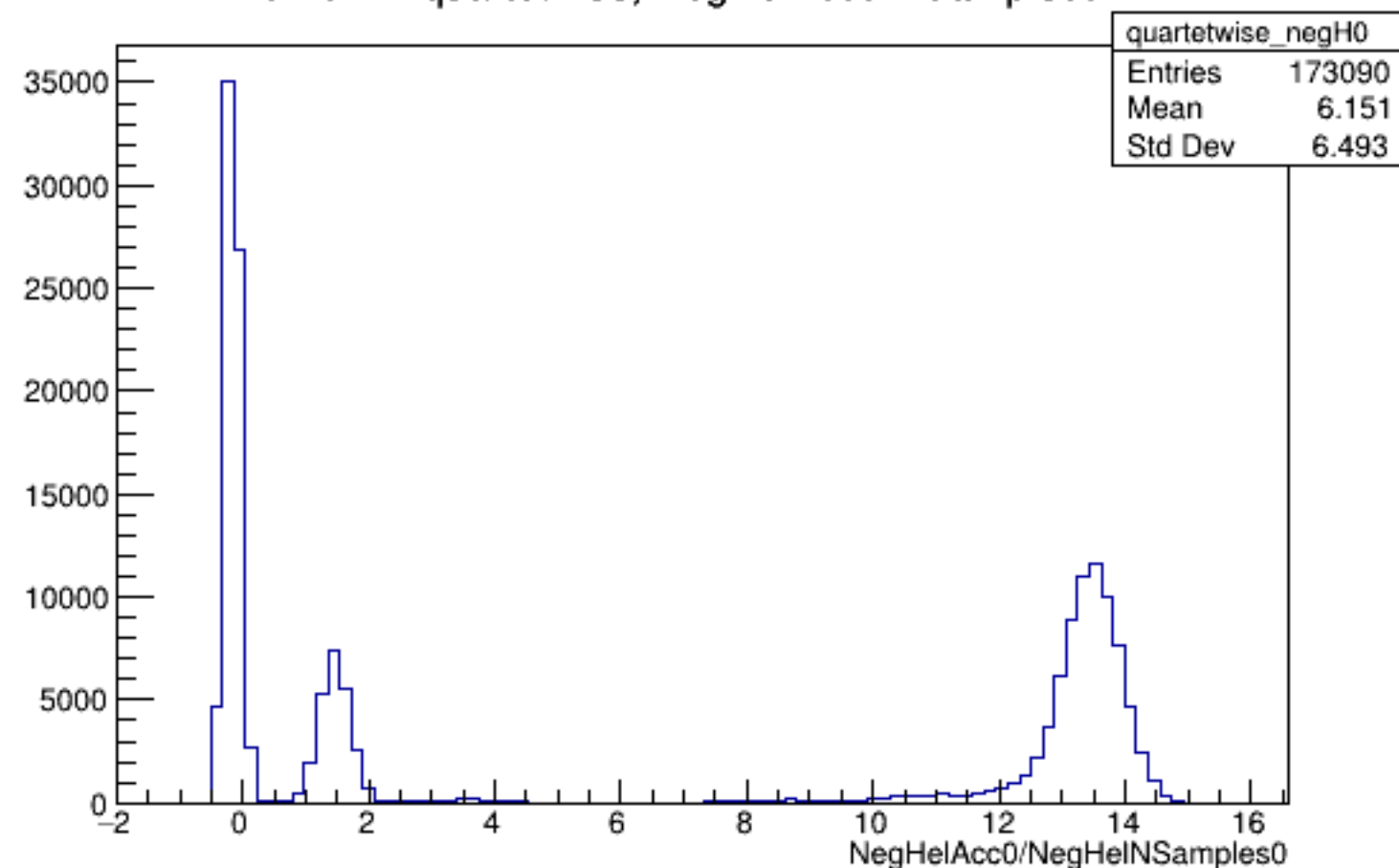
Run 5777 quartetwise, NegHelAcc0/NSamples0: All
