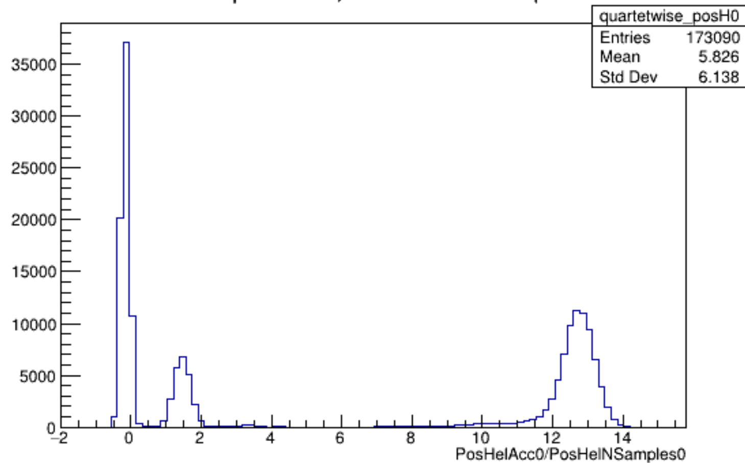
Run 5777 quartetwise, PosHelAcc0/NSamples0: All
