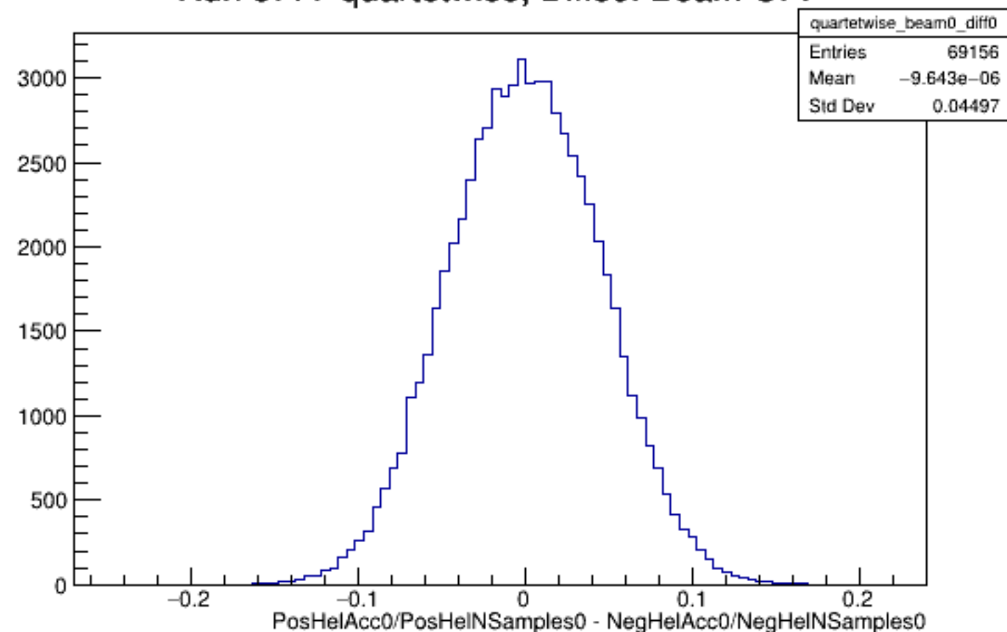
Run 5777 quartetwise, Diffs0: Beam OFF
