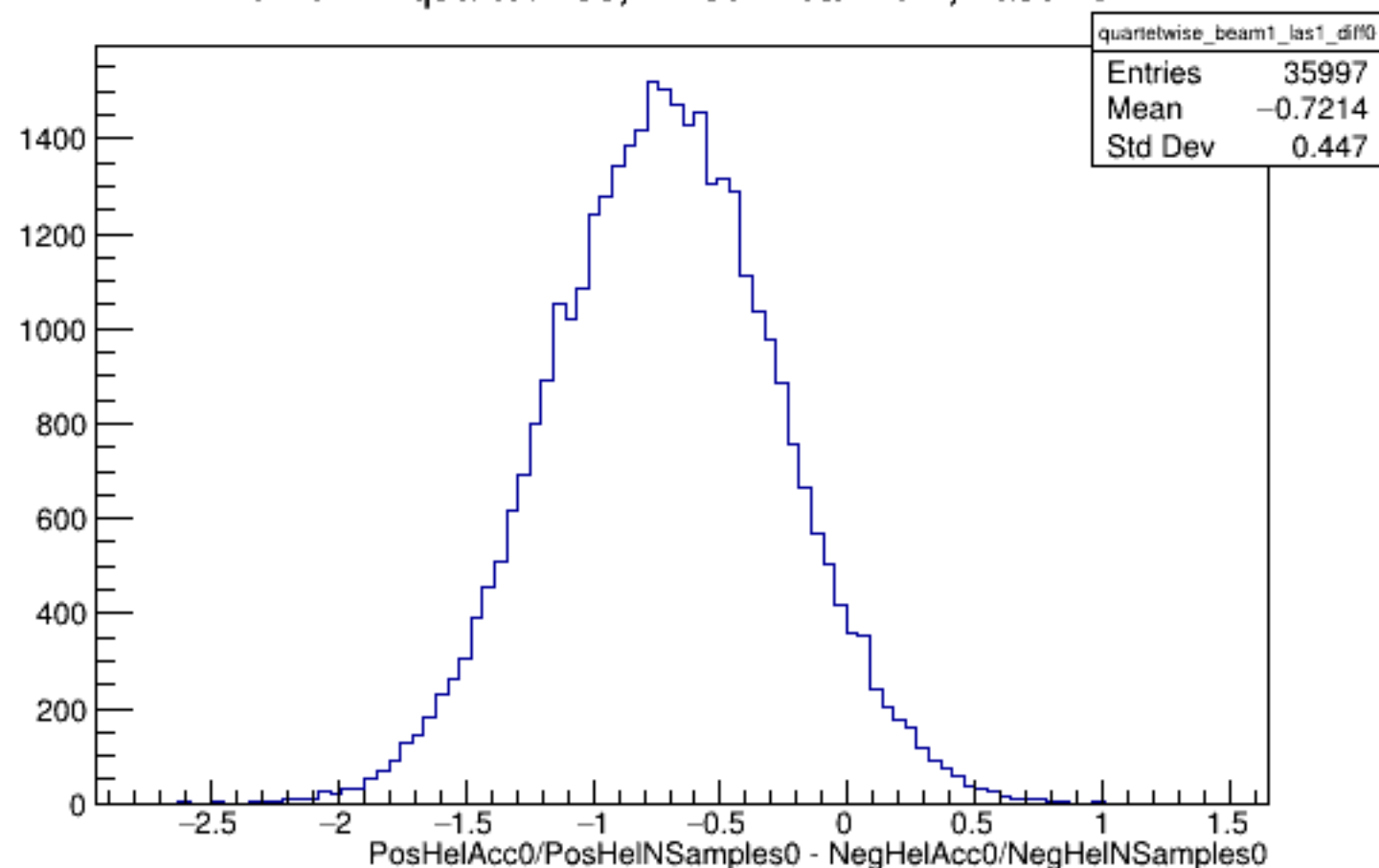
Run 5777 quartetwise, Diffs0: Beam ON, Laser ON
