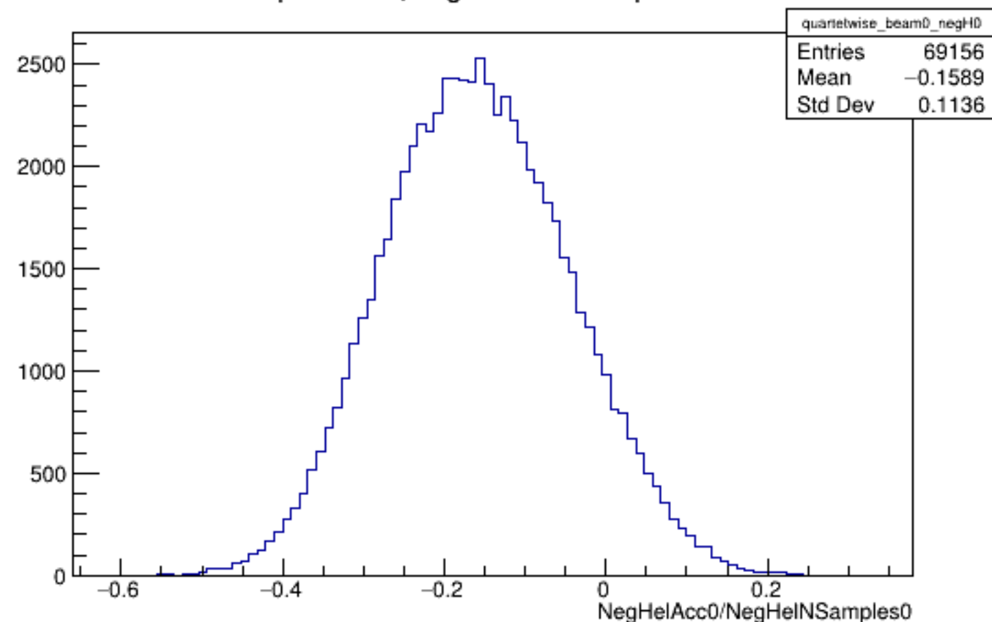
Run 5777 quartetwise, NegHelAcc0/NSamples0: Beam OFF
