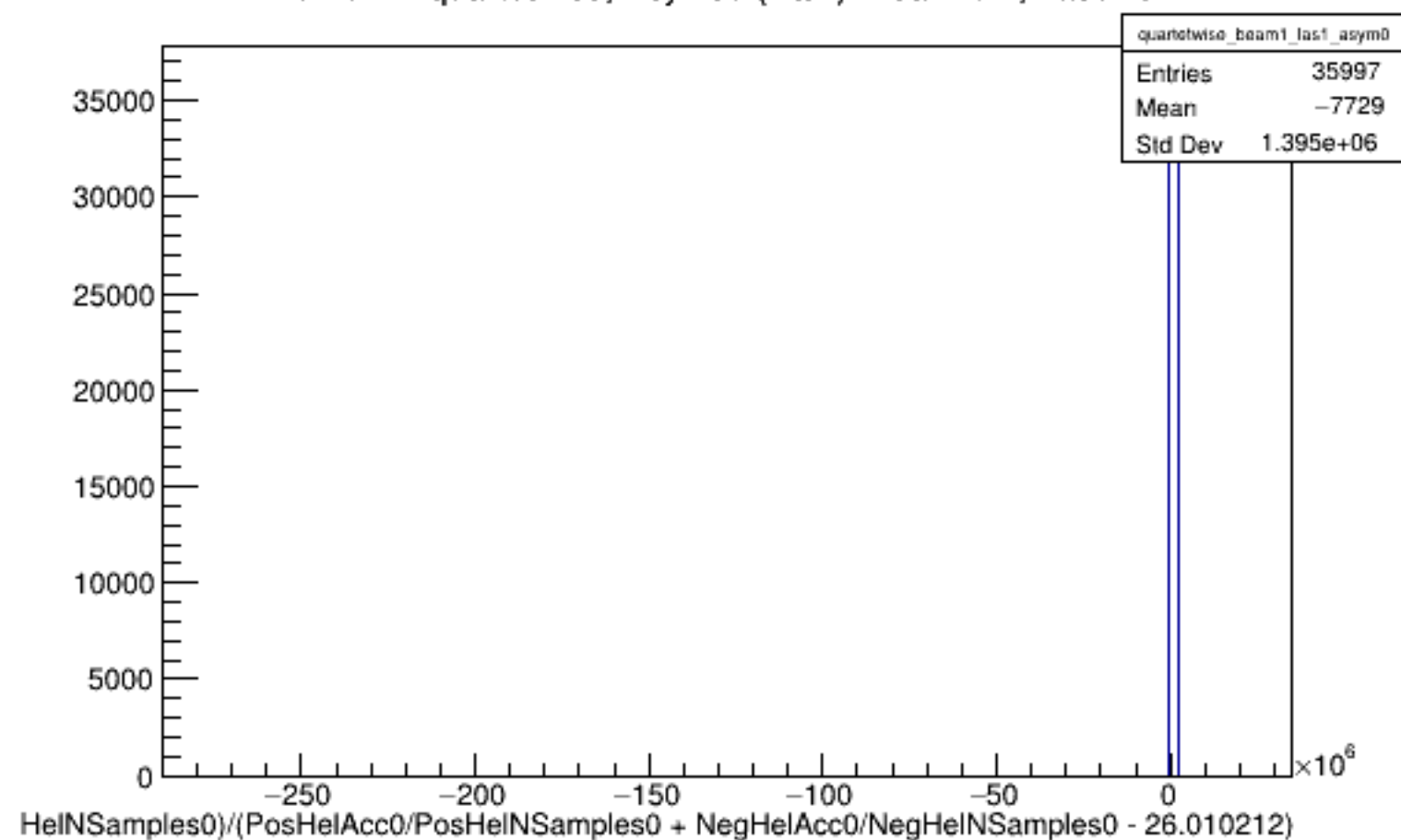
Run 5777 quartetwise, Asyms0 (Raw): Beam ON, Laser ON
