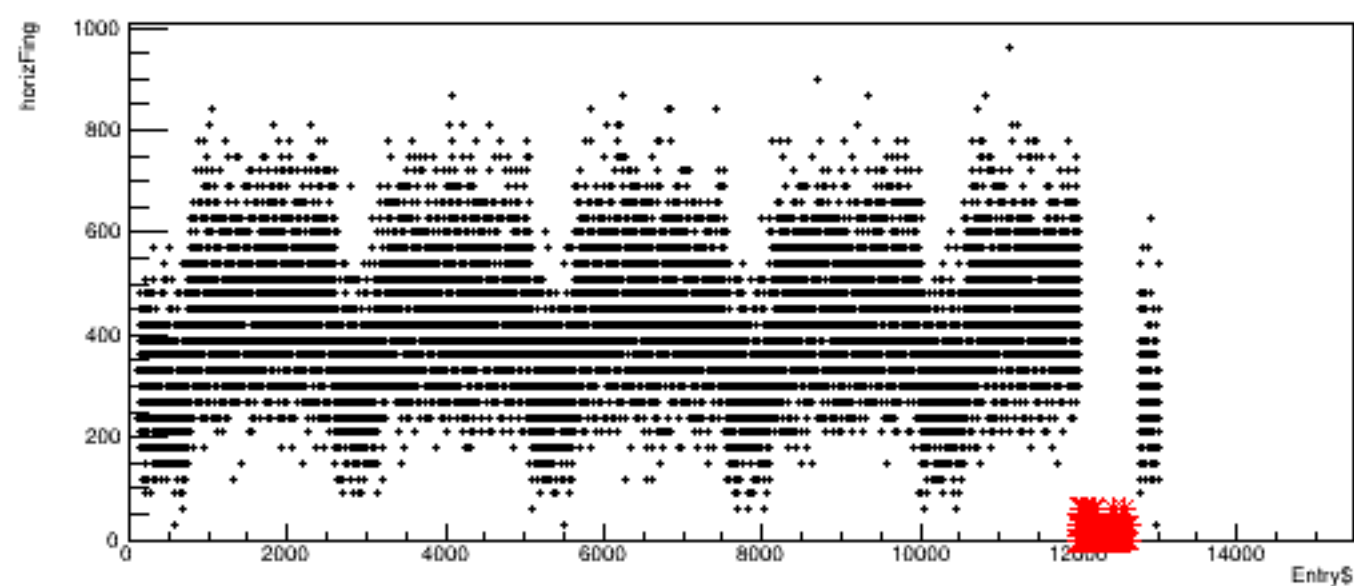
Run 5783, quartetwise: horizFing vs time
