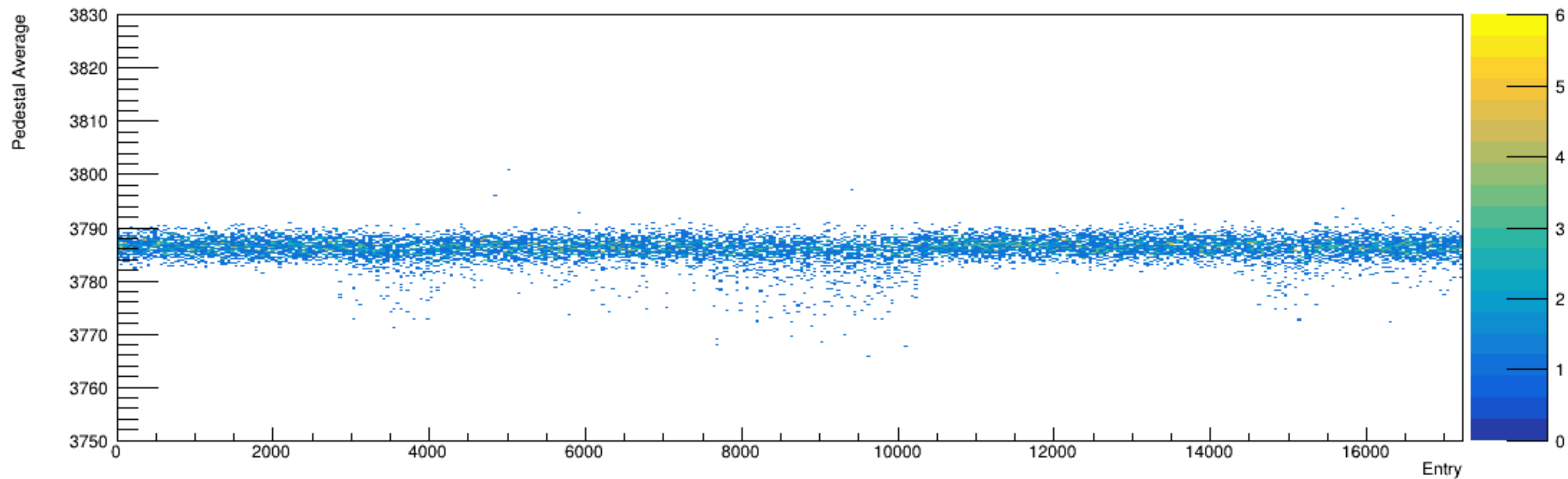
Run 5784, snapshots: Pedestal vs. Time
