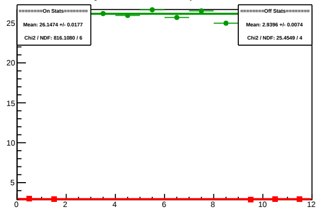
Cycle 5785.1: Multiplet Sums
