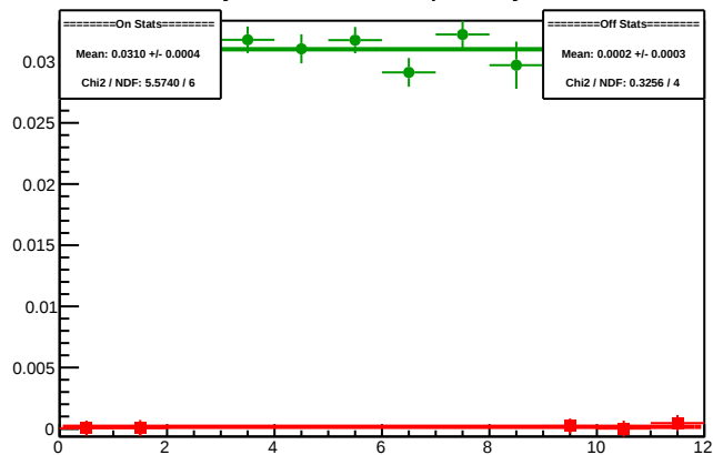
Cycle 5785.1: Multiplet Asyms
