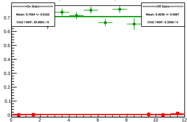
Cycle 5785.1: Multiplet Diffs
