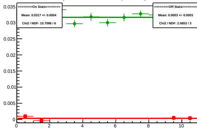
Cycle 5785.3: Multiplet Asyms
