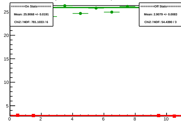
Cycle 5785.3: Multiplet Sums
