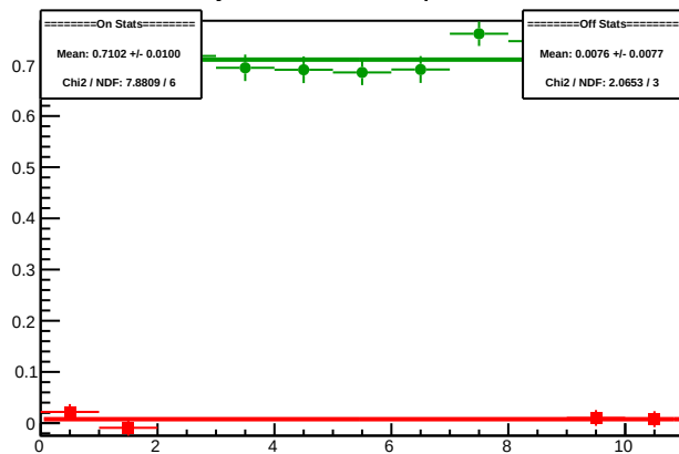
Cycle 5785.3: Multiplet Diffs
