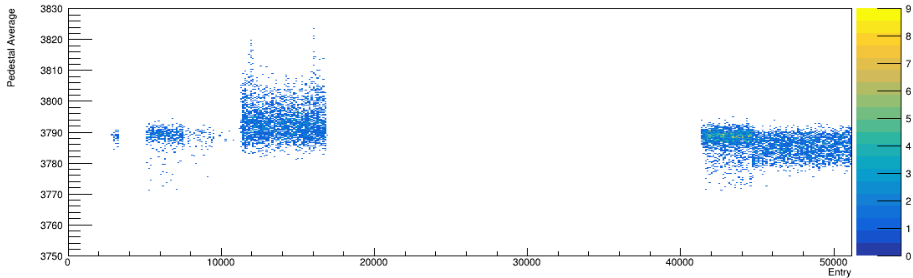
Run 5789, snapshots: Pedestal vs. Time
