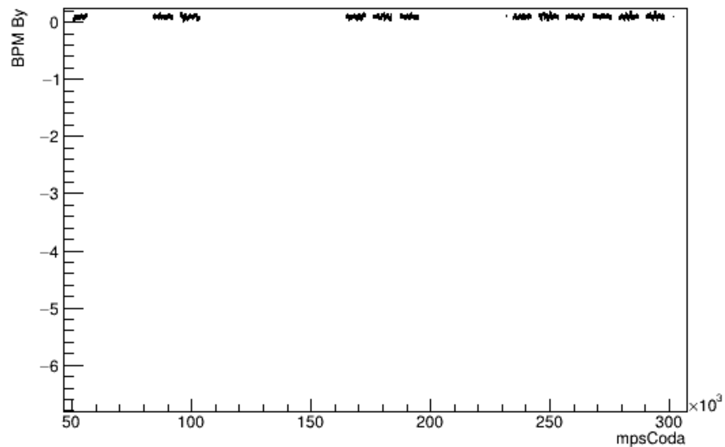
Run 5791 mpwise, beam ON, laser ON
