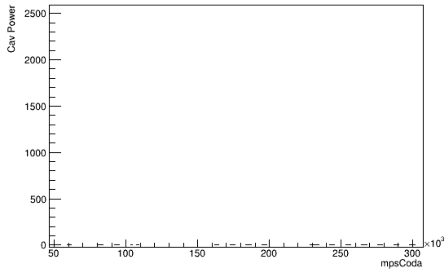
Run 5791 mpwise, beam ON, laser OFF
