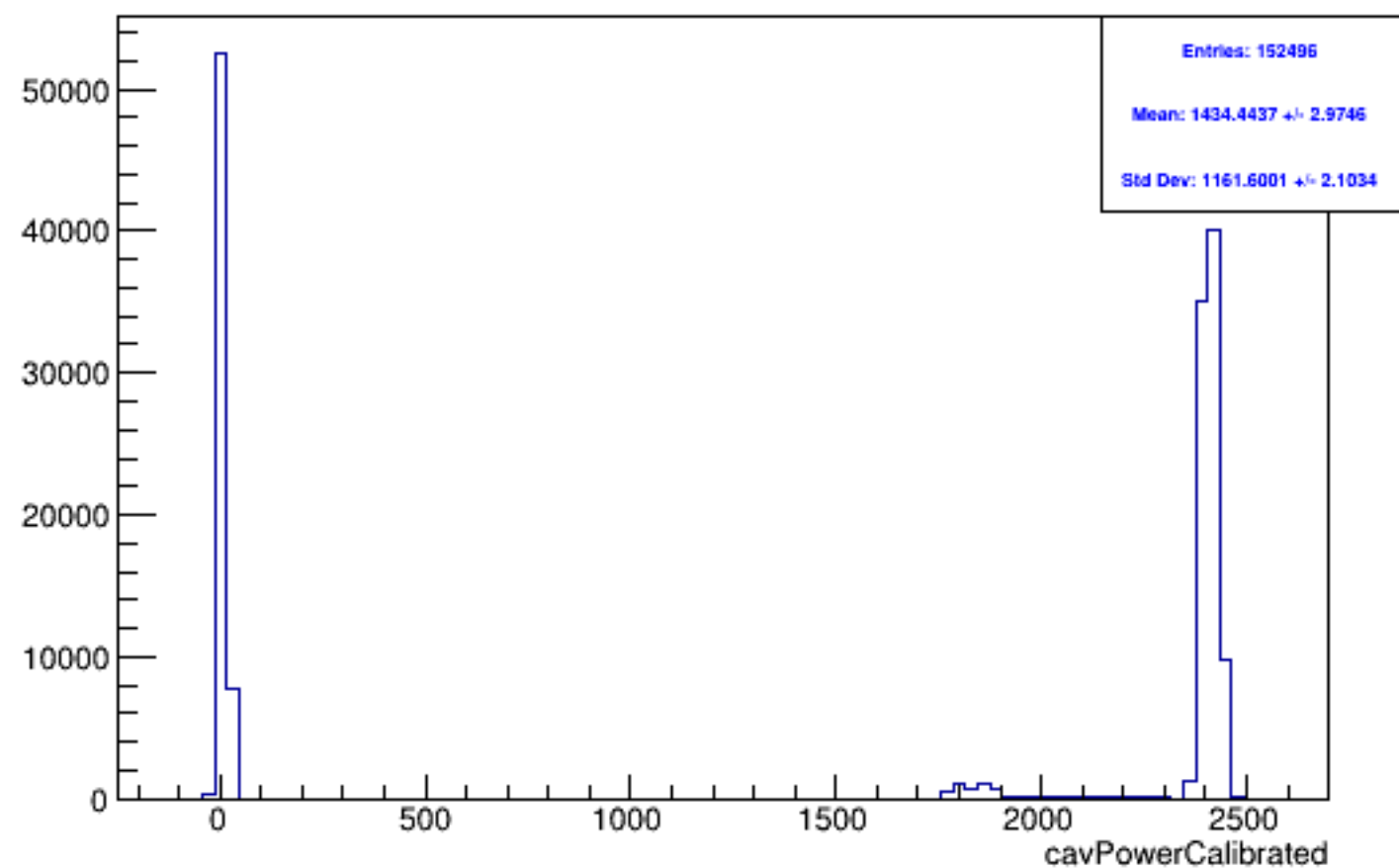
Run 5791 mpwise, lasPow: All
