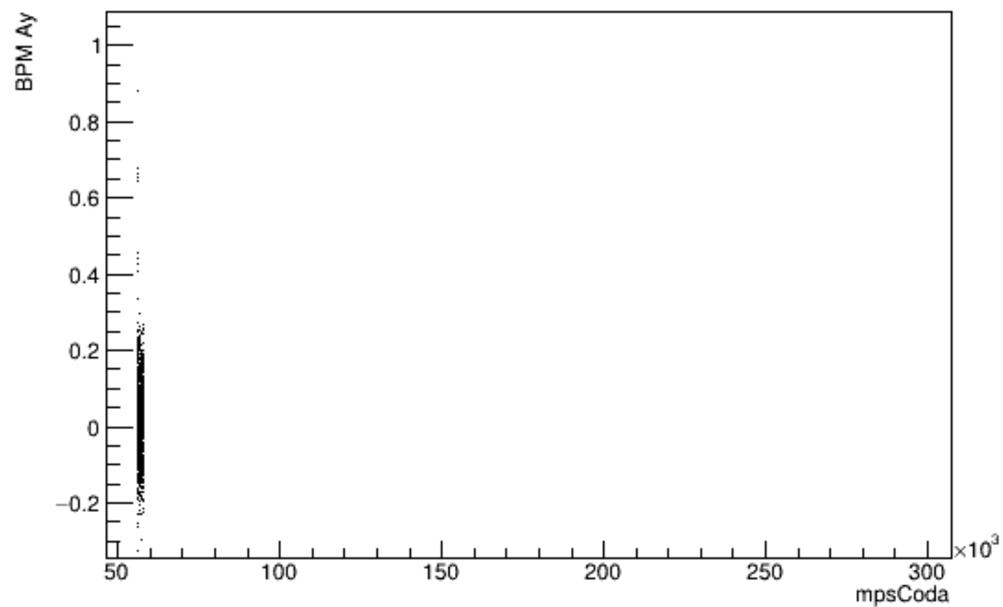
Run 5791 mpwise, beam OFF, laser ON
