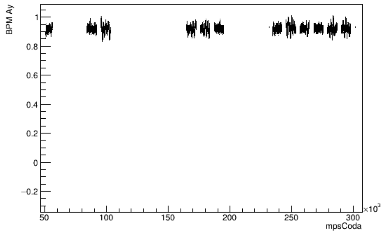
Run 5791 mpwise, beam ON, laser ON
