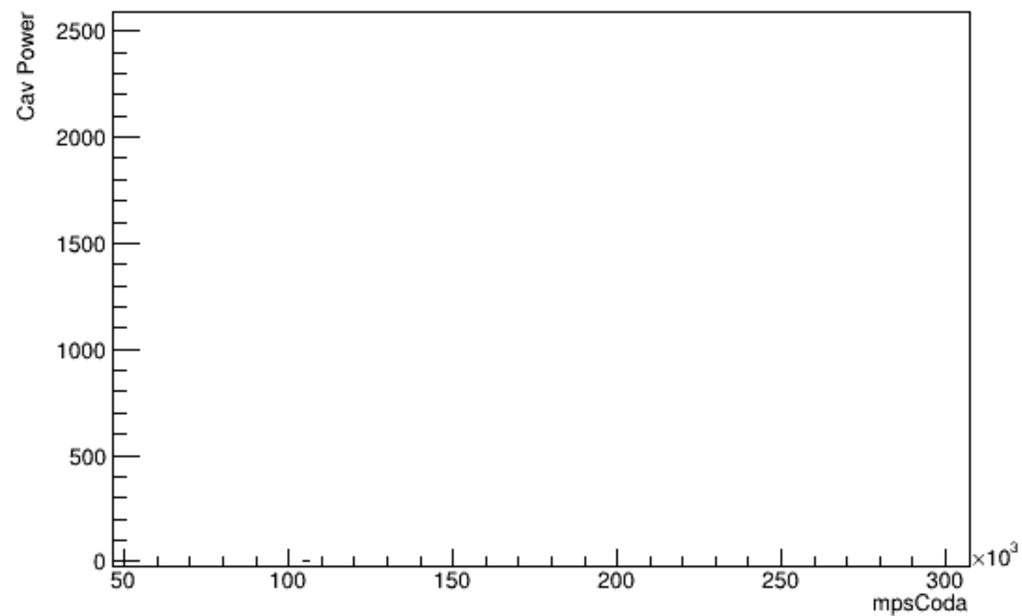
Run 5791 mpwise, beam OFF, laser OFF
