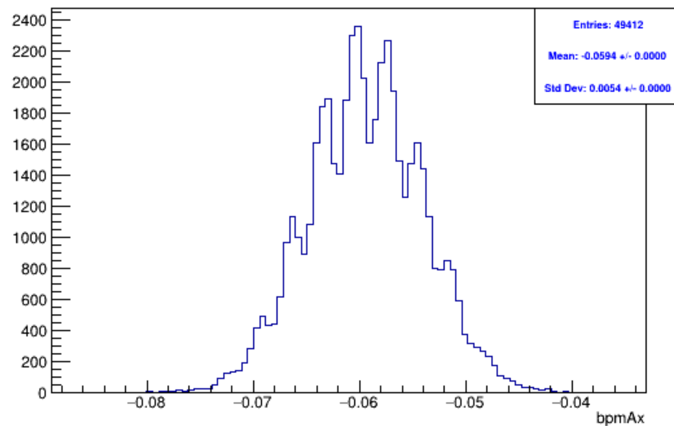
Run 5791, mpwise, bpmAx: Beam ON, Laser OFF
