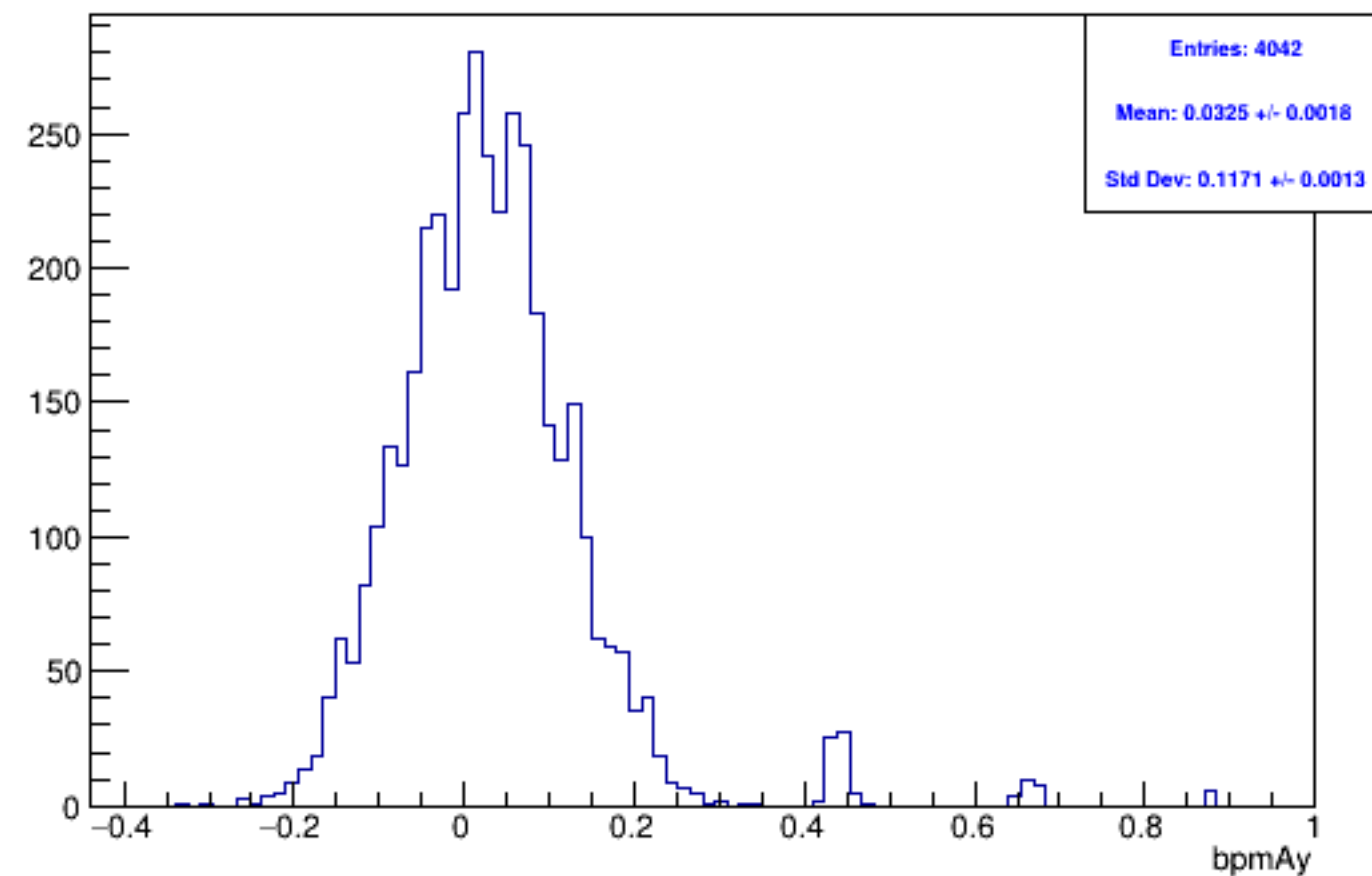
Run 5791 mpwise, bpmAy: Beam OFF
