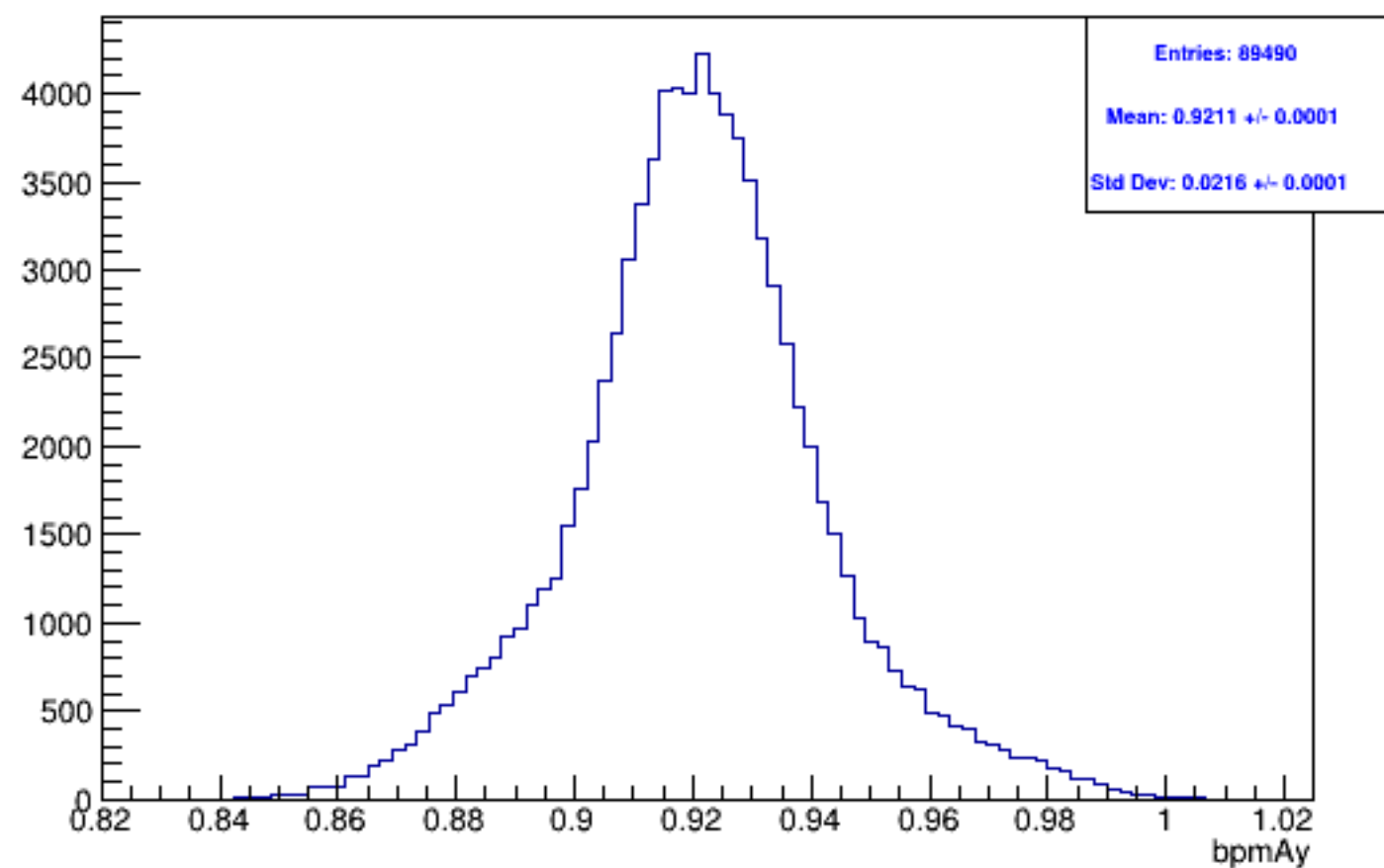
Run 5791, mpwise, bpmAy: Beam ON, Laser ON
