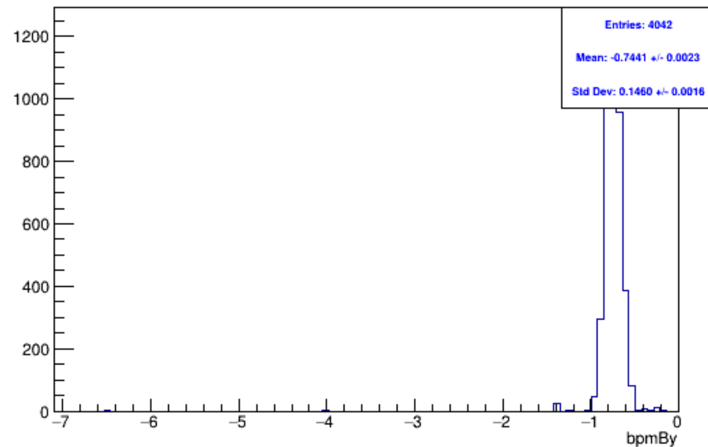
Run 5791 mpswise, bpmBy: Beam OFF
