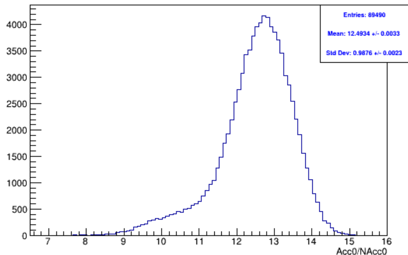
Run 5791, mpwise, acc0: Beam ON, Laser ON
