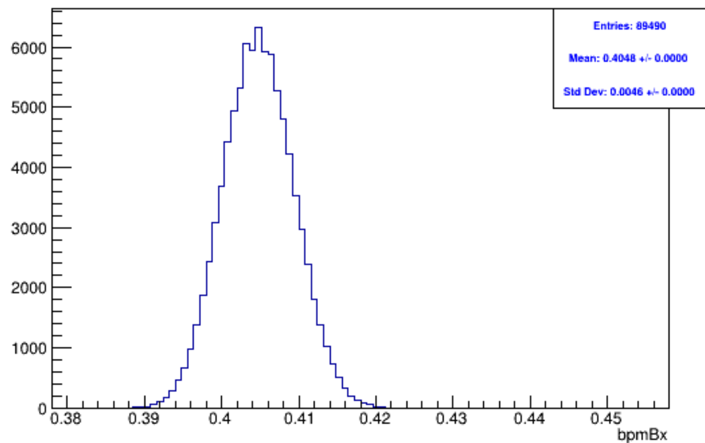
Run 5791, mpswise, bpmBx: Beam ON, Laser ON
