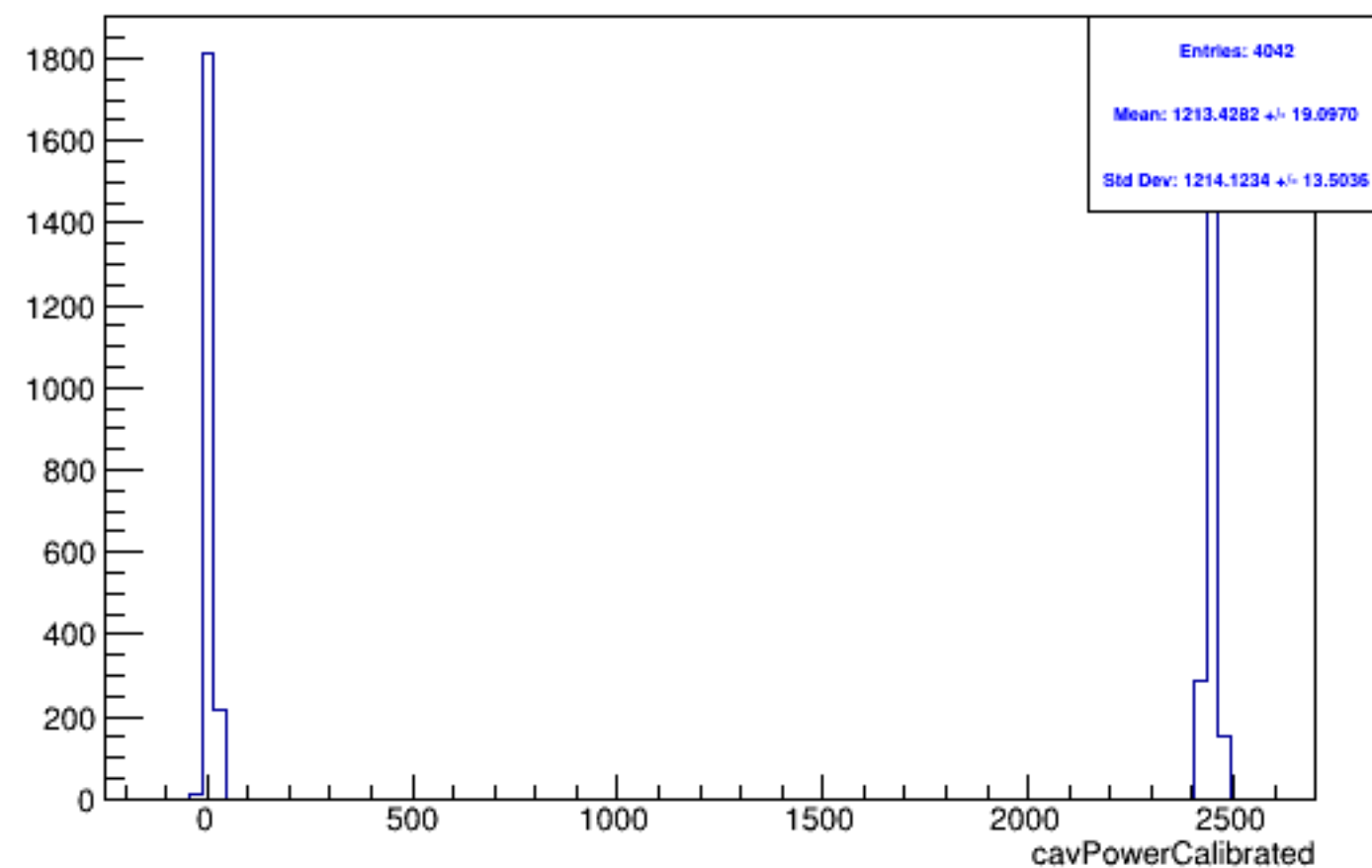
Run 5791 mpwise, lasPow: Beam OFF
