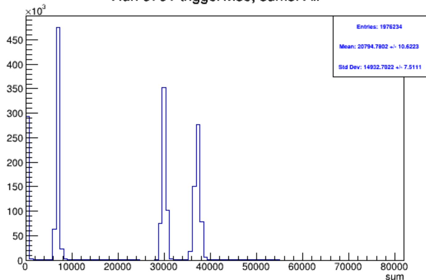
Run 5791 triggerwise, sums: All
