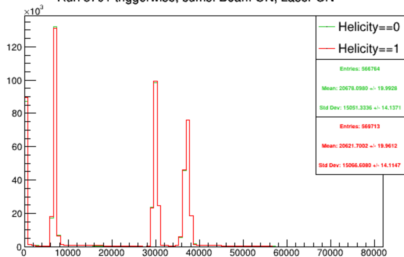
Run 5791 triggerwise, sums: Beam ON, Laser ON
