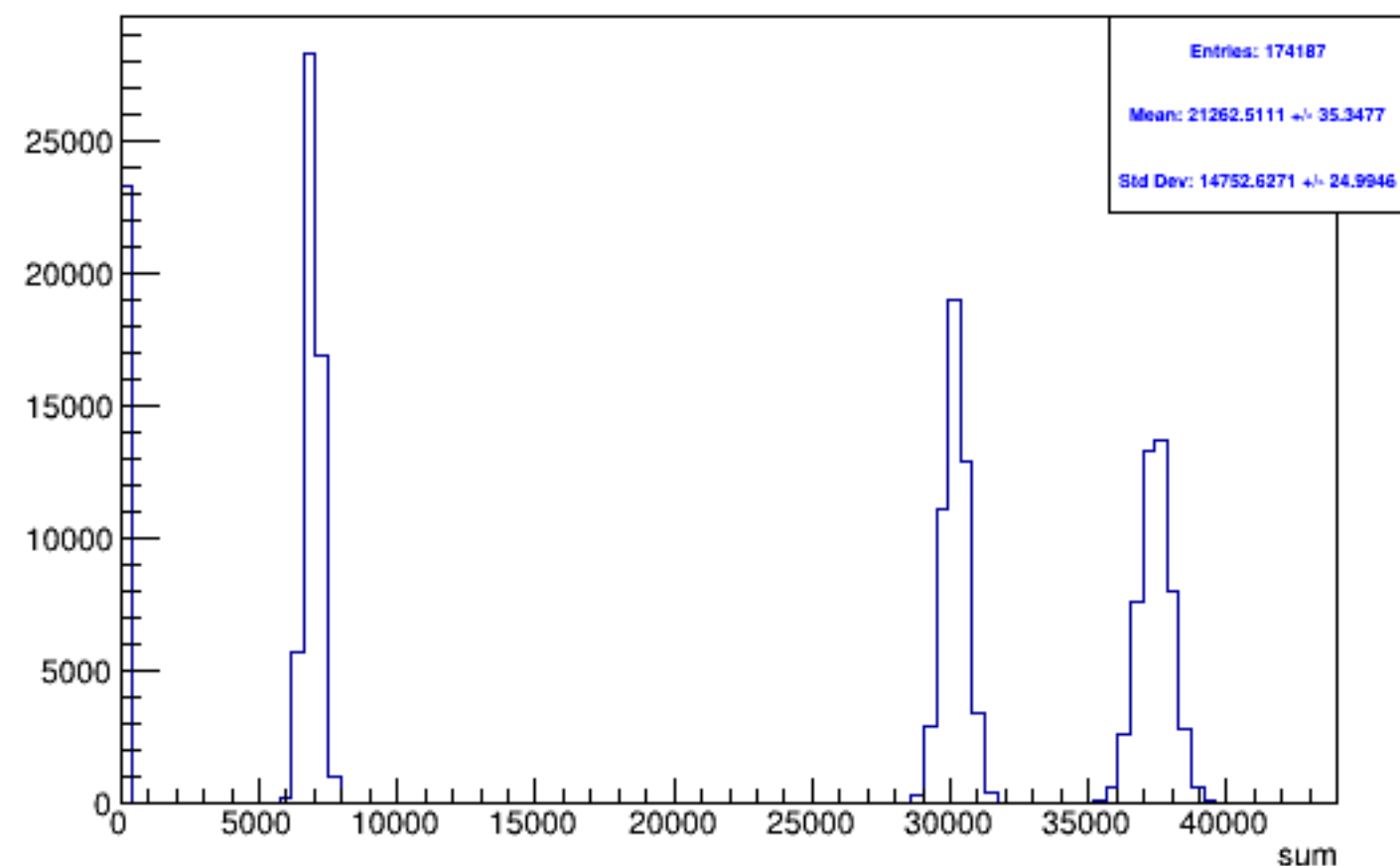
Run 5791 triggerwise, sums: Beam OFF
