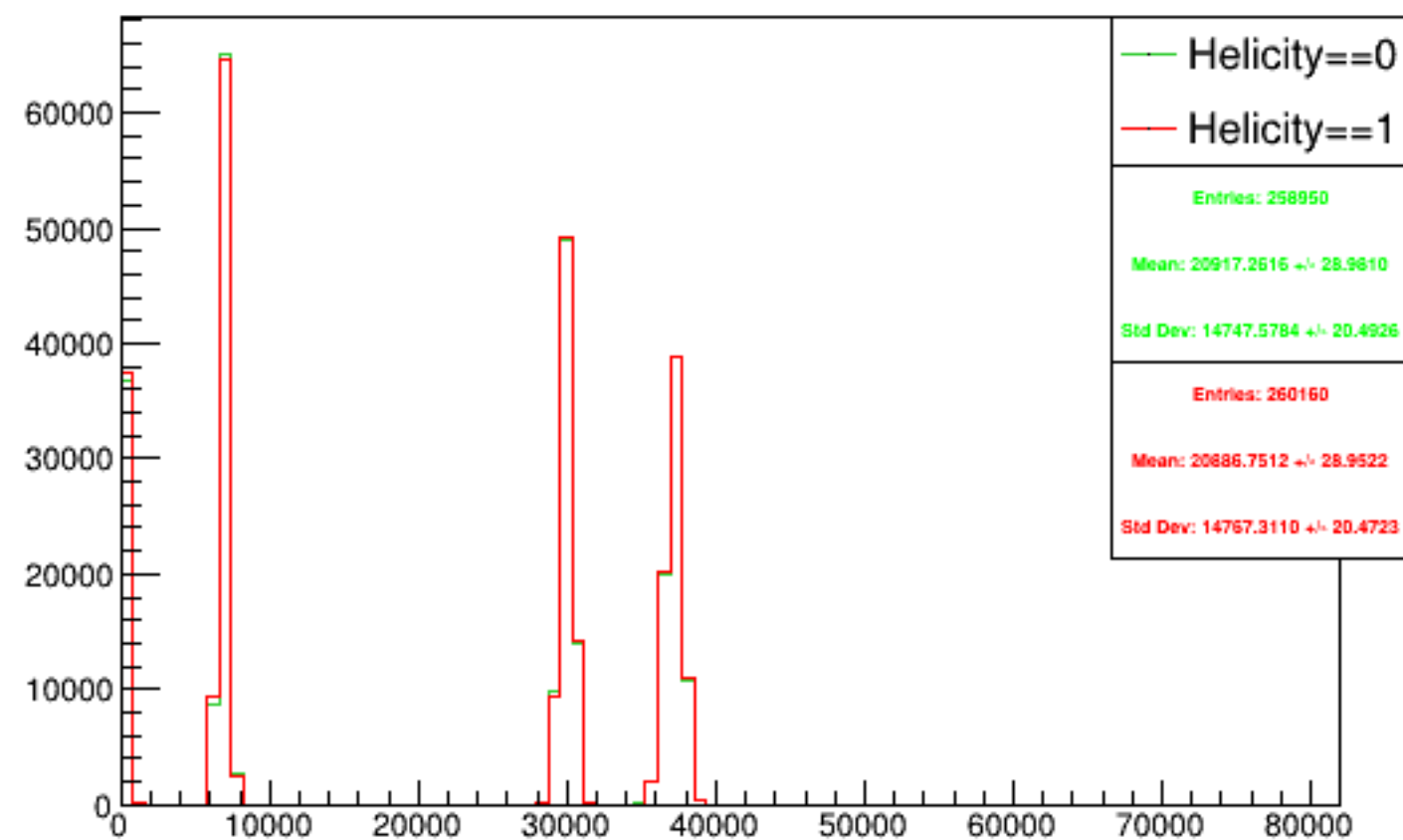
Run 5791 triggerwise, sums: Beam ON, Laser OFF
