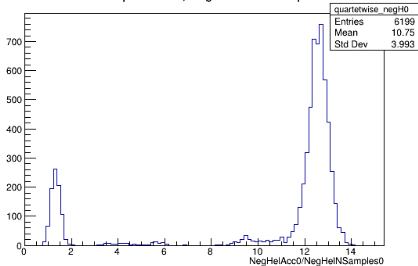
Run 5792 quartetwise, NegHelAcc0/NSamples0: All
