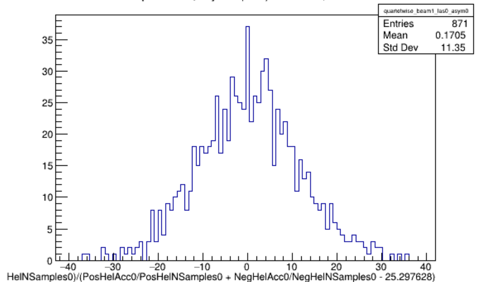
Run 5792 quartetwise, Asyms0 (Raw): Beam ON, Laser OFF
