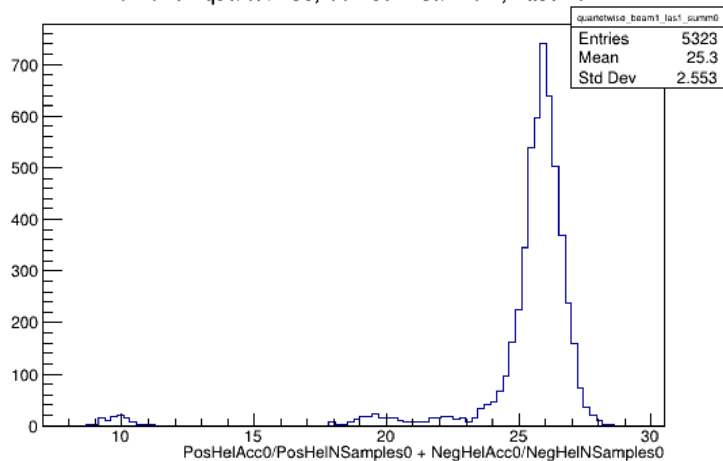
Run 5792 quartetwise, Sums0: Beam ON, Laser ON
