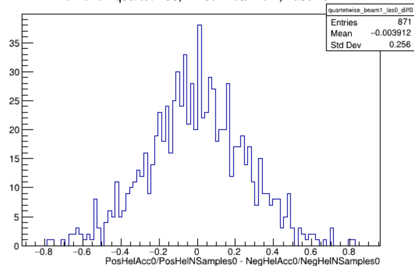
Run 5792 quartetwise, Diffs0: Beam ON, Laser OFF
