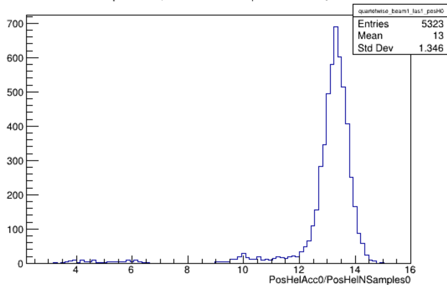
Run 5792 quartetwise, PosHelAcc0/NSamples0: Beam ON, Laser ON
