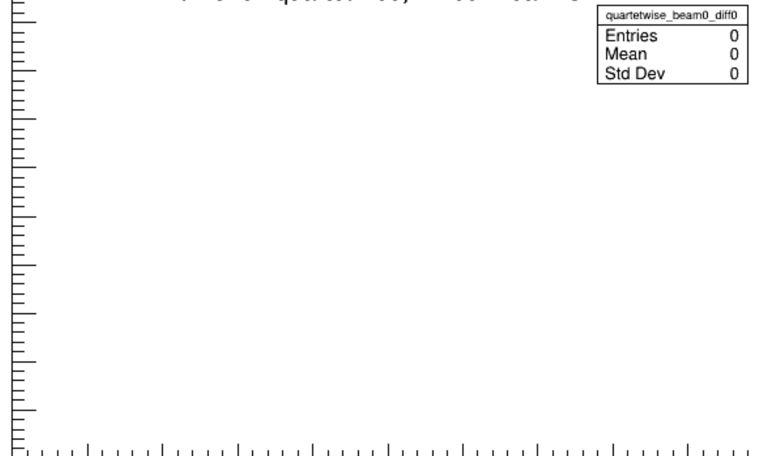
Run 5792 quartetwise, Diffs0: Beam OFF
