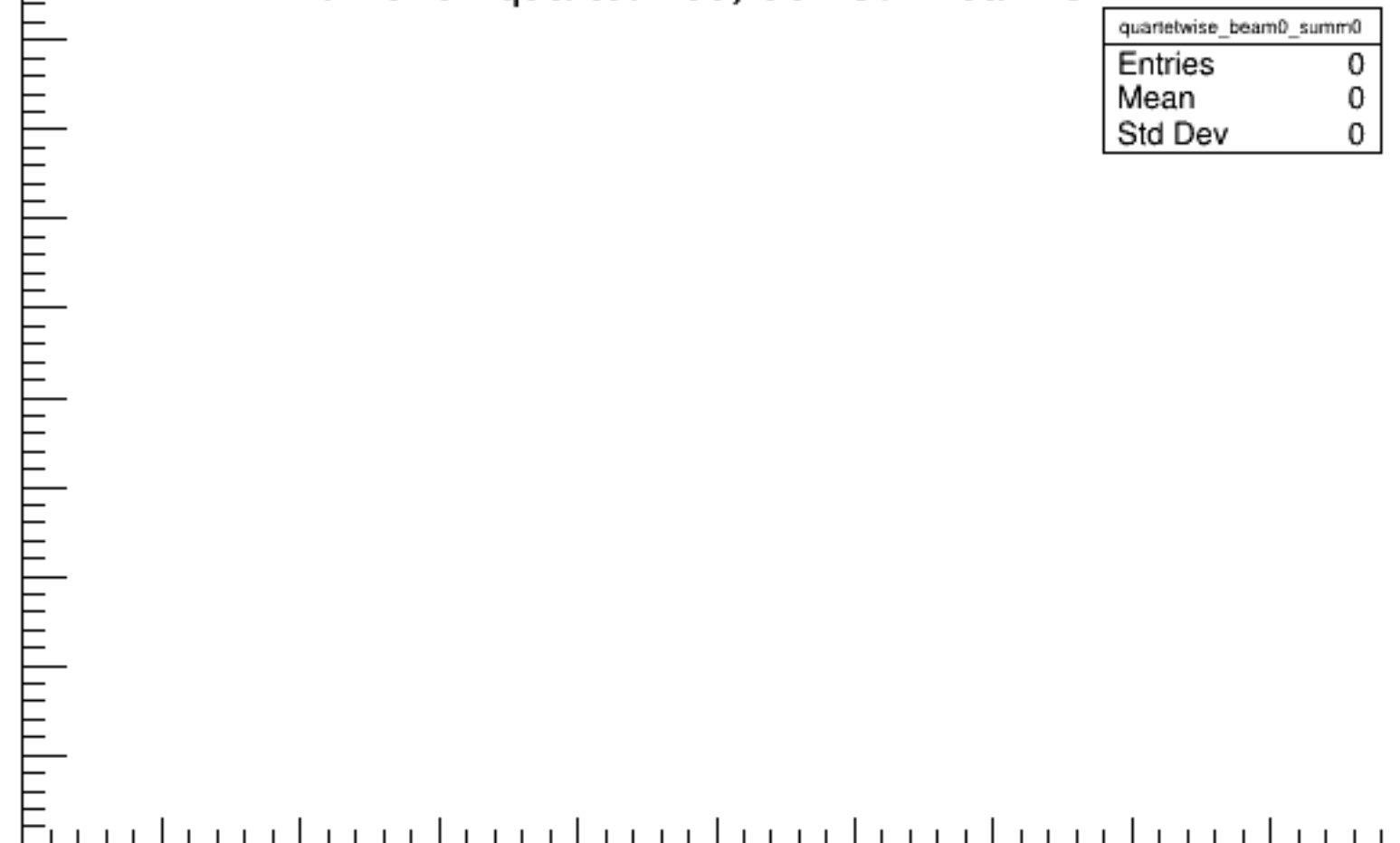
Run 5792 quartetwise, Sums0: Beam OFF
