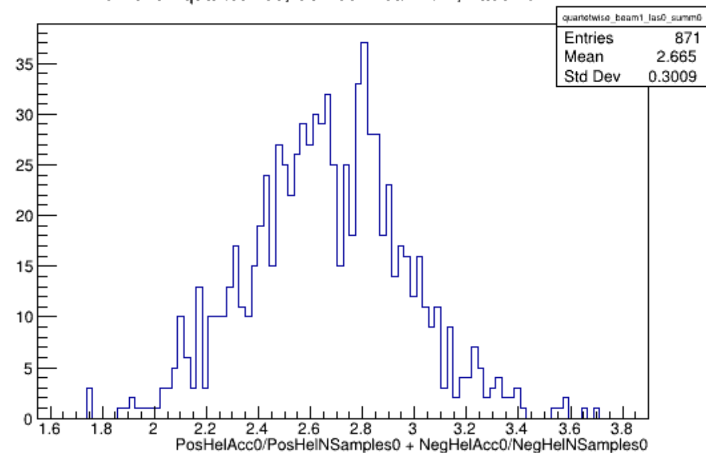
Run 5792 quartetwise, Sums0: Beam ON, Laser OFF
