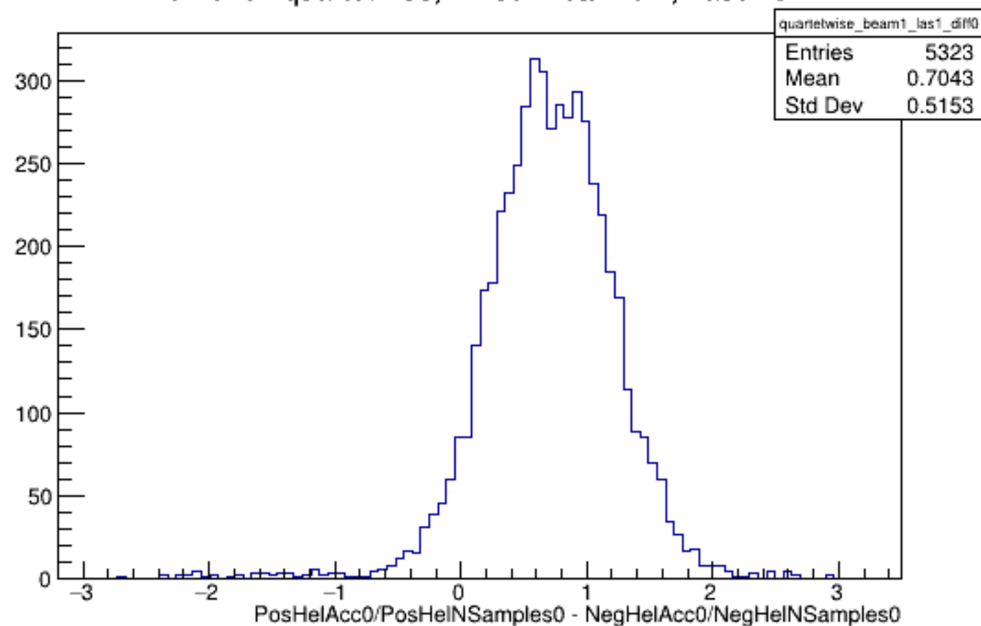
Run 5792 quartetwise, Diffs0: Beam ON, Laser ON
