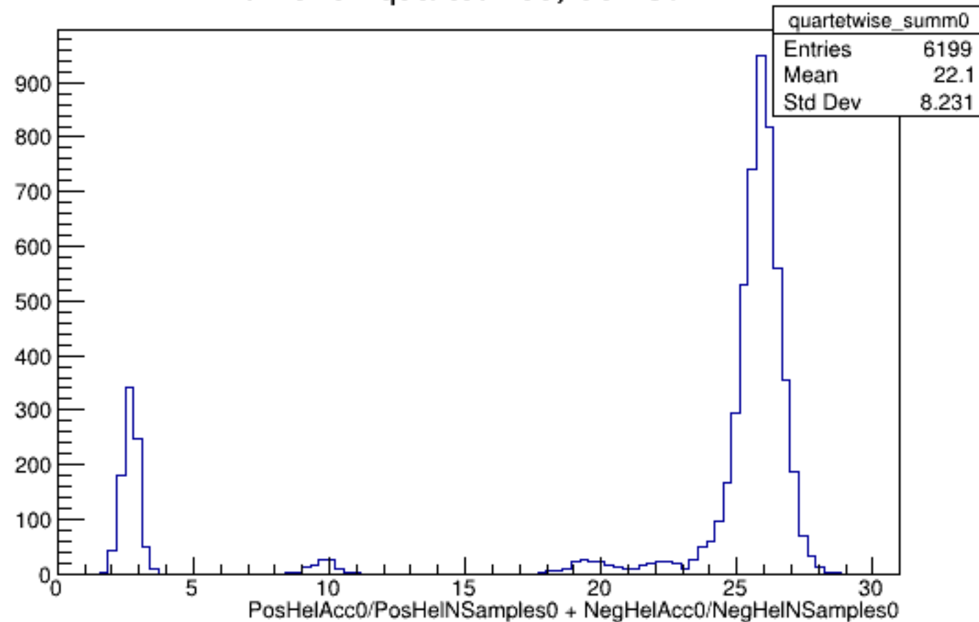
Run 5792 quartetwise, Sums0: All
