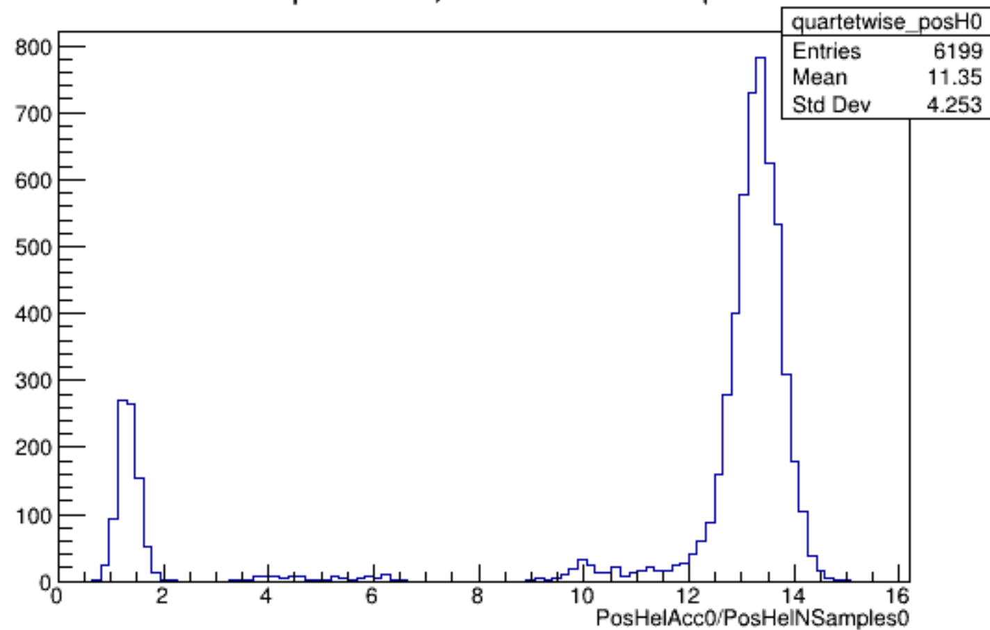
Run 5792 quartetwise, PosHelAcc0/NSamples0: All
