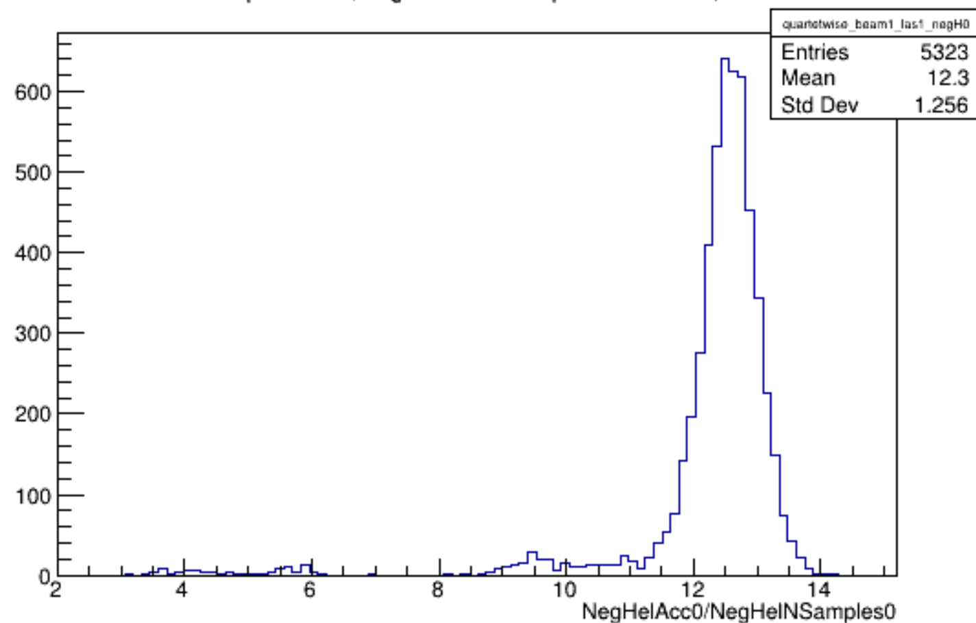
Run 5792 quartetwise, NegHelAcc0/NSamples0: Beam ON, Laser ON
