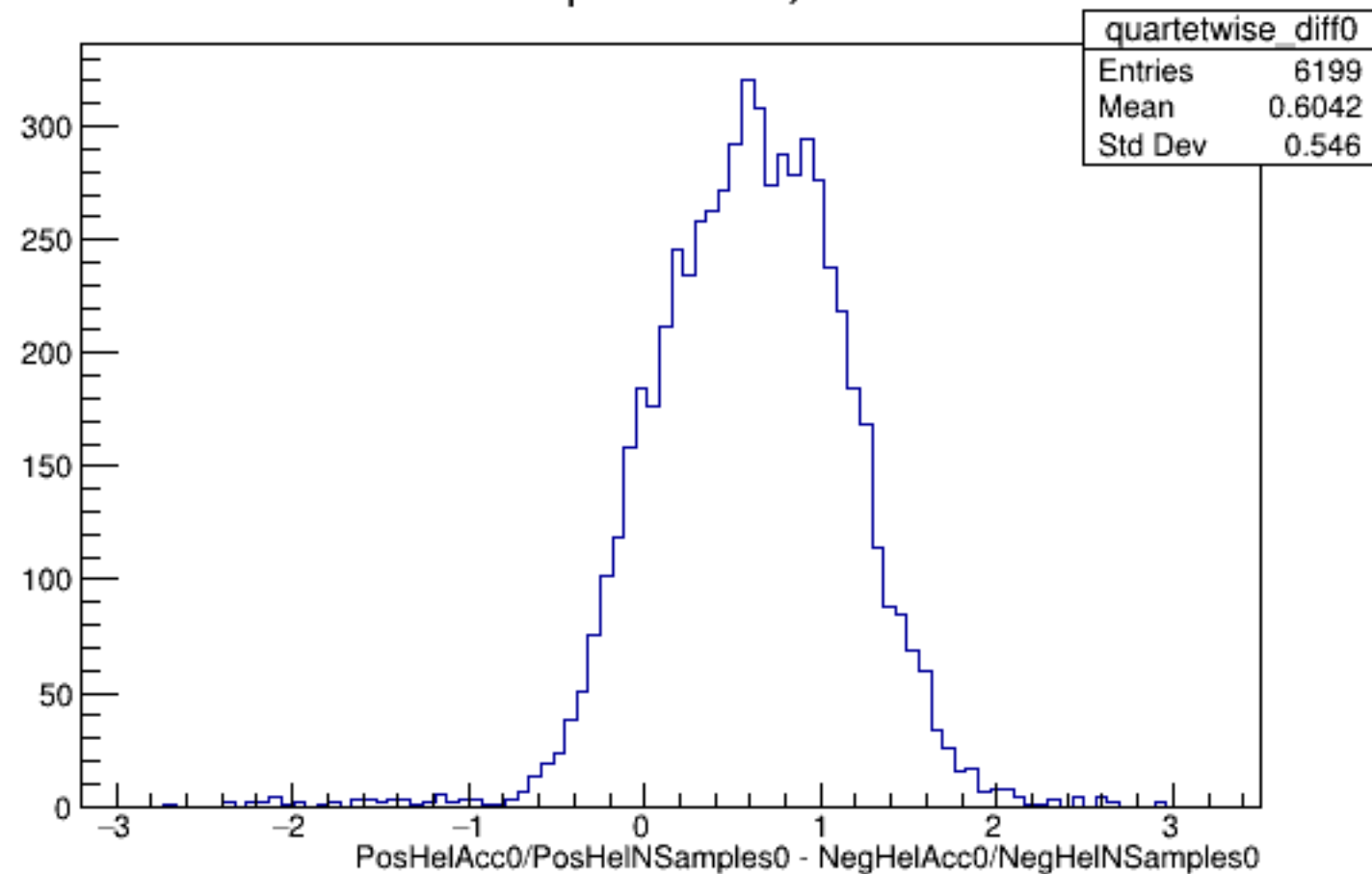
Run 5792 quartetwise, Diffs0: All
