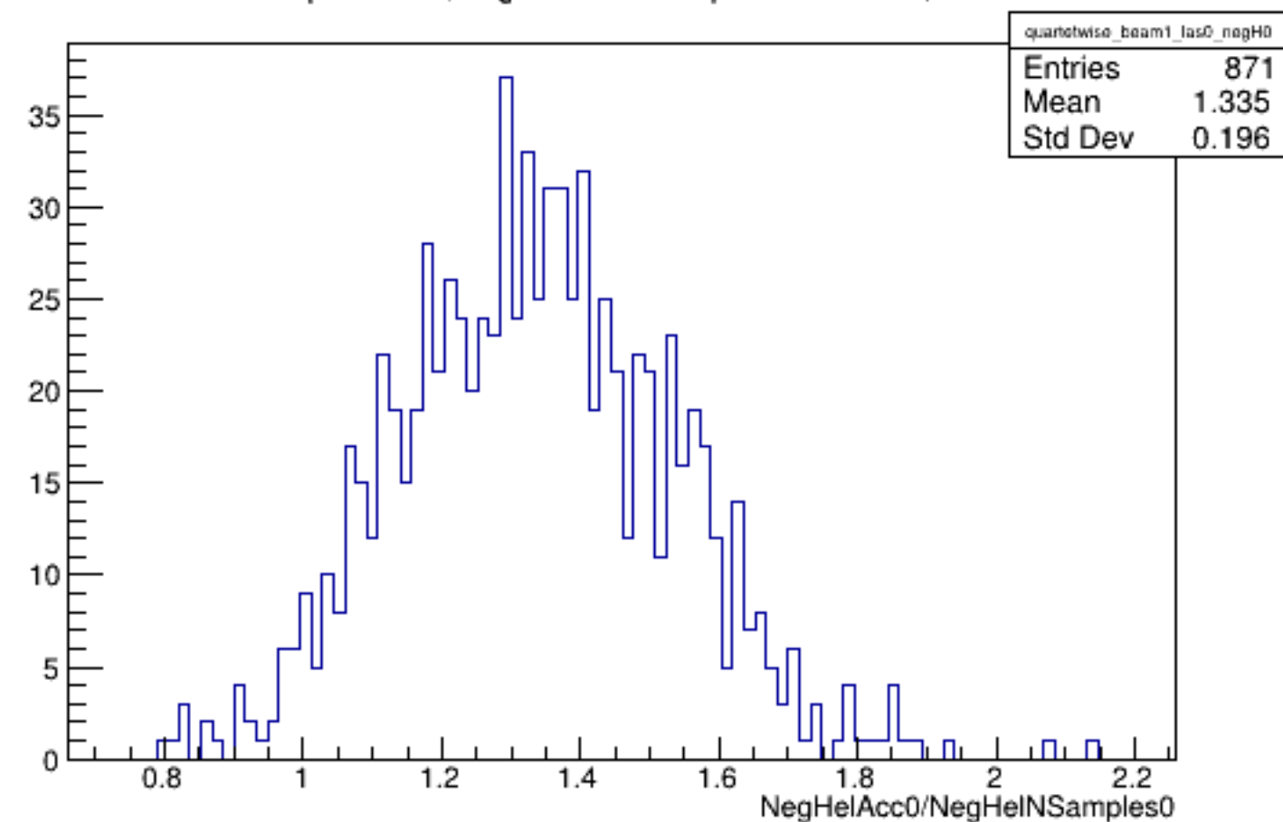
Run 5792 quartetwise, NegHelAcc0/NSamples0: Beam ON, Laser OFF
