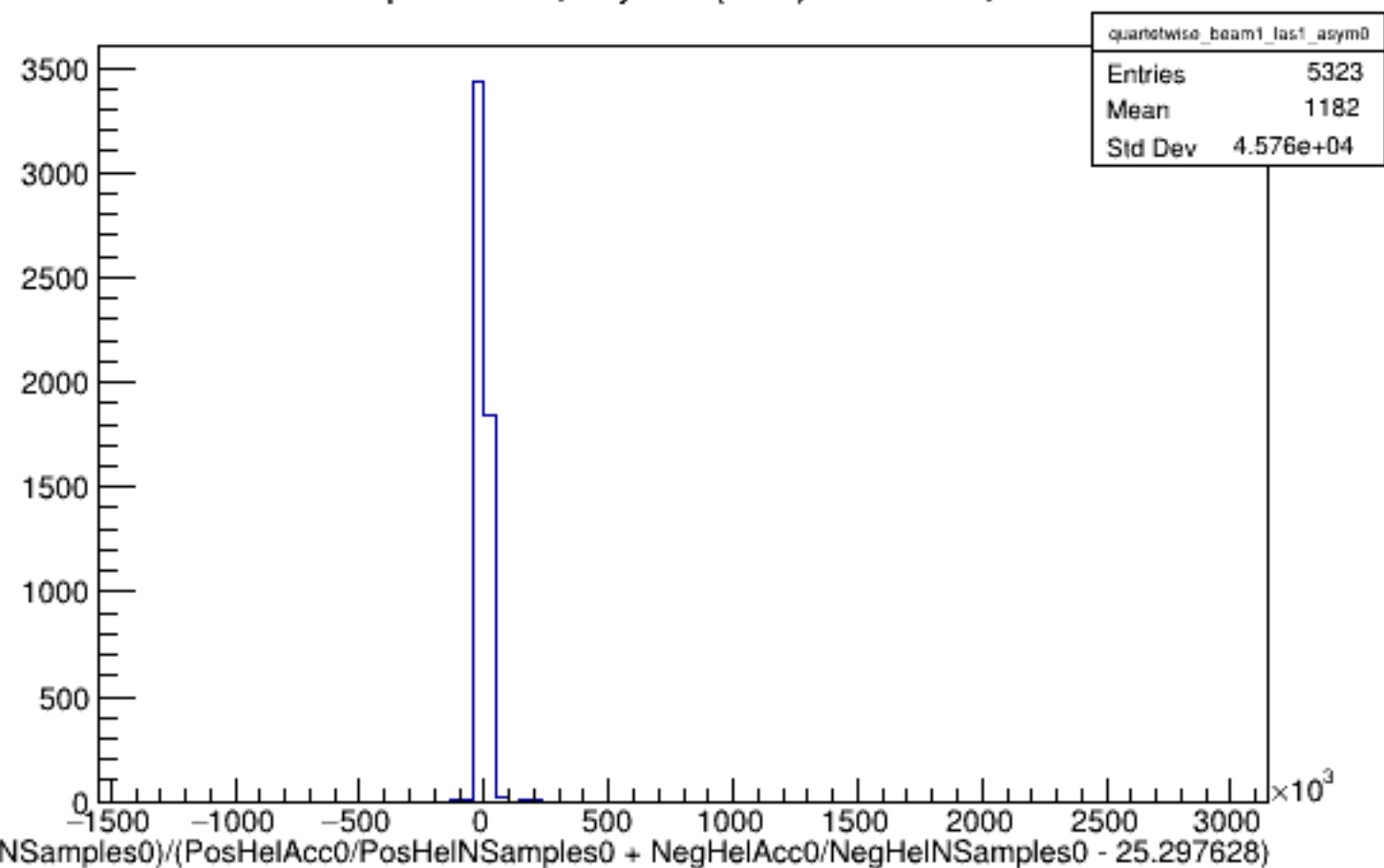
Run 5792 quartetwise, Asyms0 (Raw): Beam ON, Laser ON
