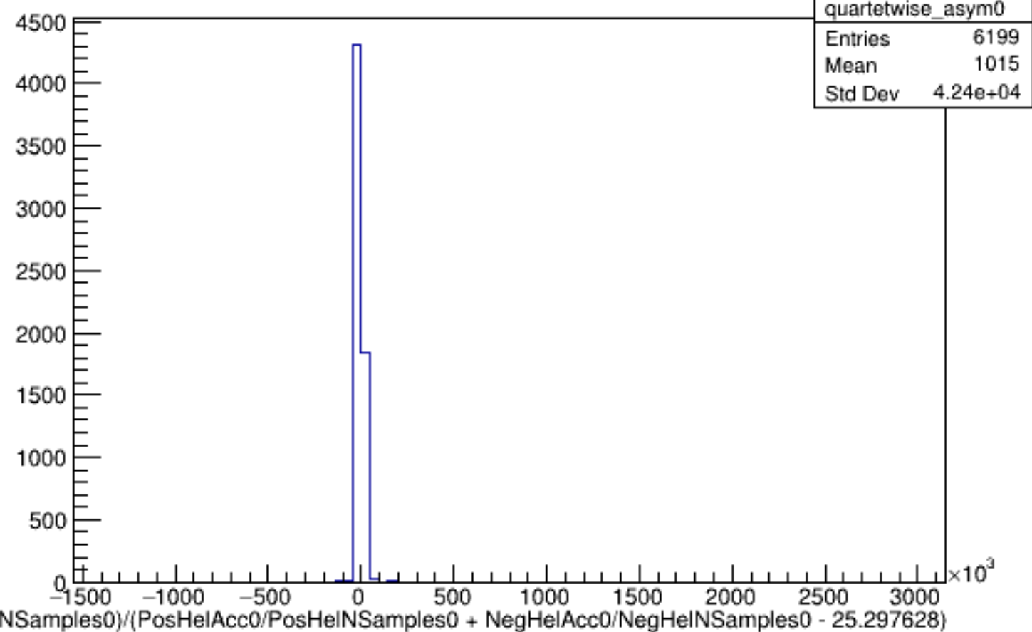
Run 5792 quartetwise, Asyms0 (Raw): All
