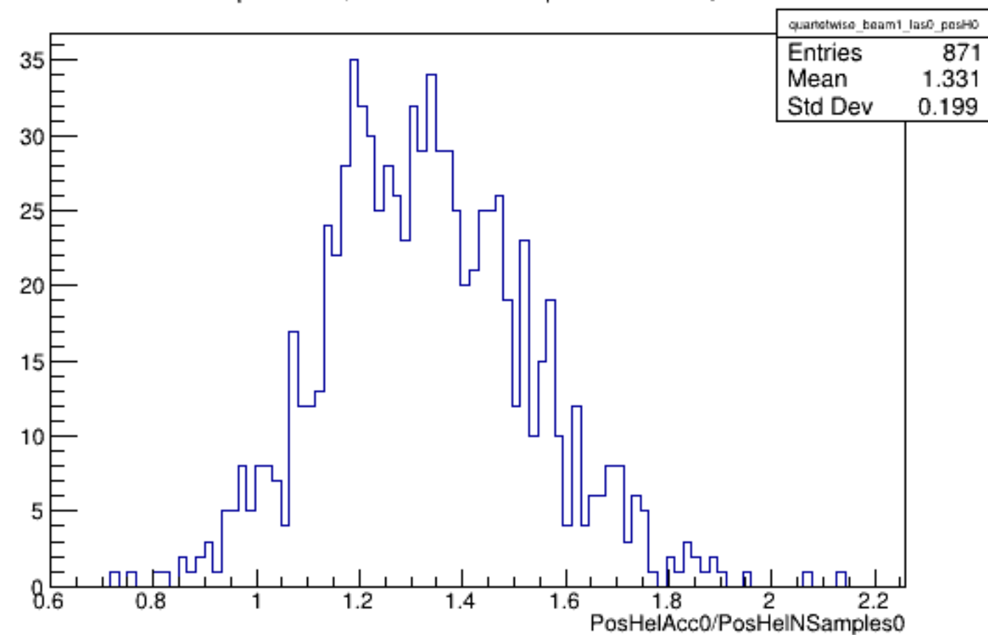
Run 5792 quartetwise, PosHelAcc0/NSamples0: Beam ON, Laser OFF
