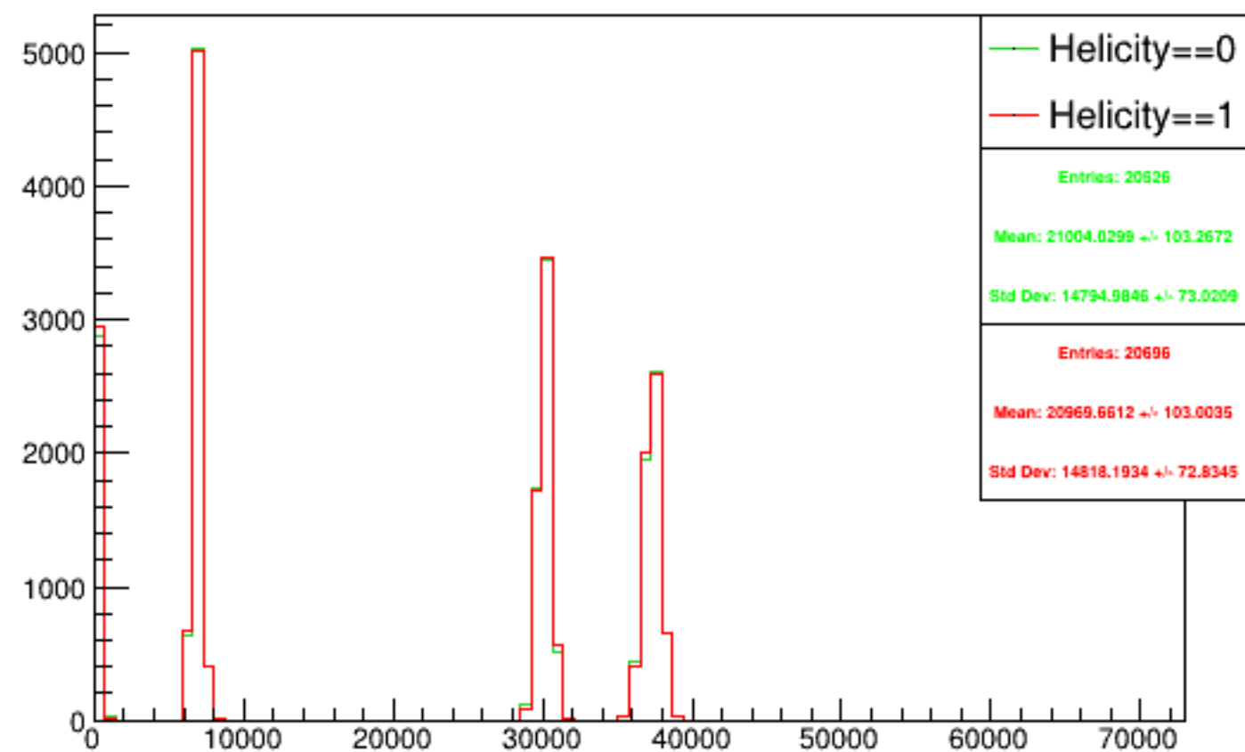
Run 5792 triggerwise, sums: Beam ON, Laser OFF
