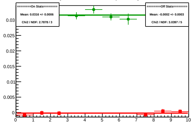
Cycle 5794.4: Multiplet Asyms
