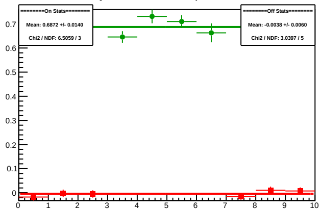
Cycle 5794.4: Multiplet Diffs
