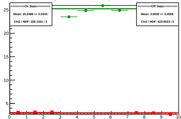
Cycle 5794.4: Multiplet Sums
