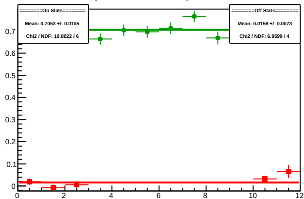
Cycle 5794.6: Multiplet Diffs
