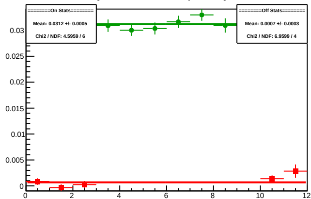
Cycle 5794.6: Multiplet Asyms
