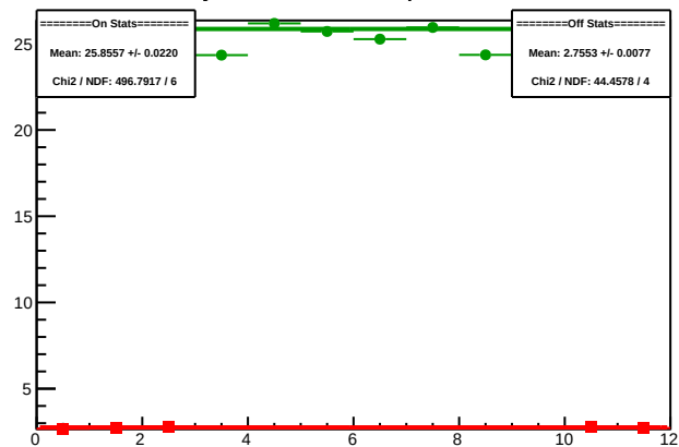
Cycle 5794.6: Multiplet Sums
