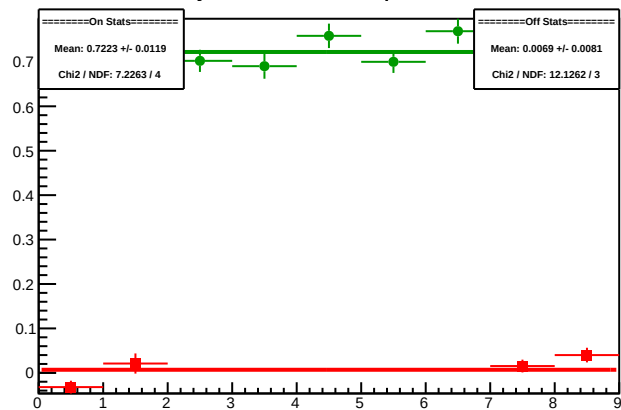
Cycle 5794.7: Multiplet Diffs
