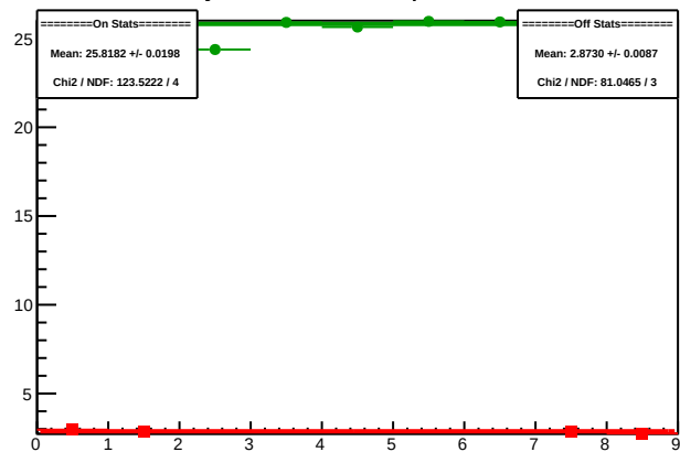
Cycle 5794.7: Multiplet Sums
