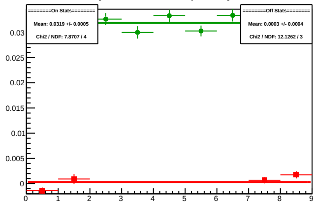
Cycle 5794.7: Multiplet Asyms
