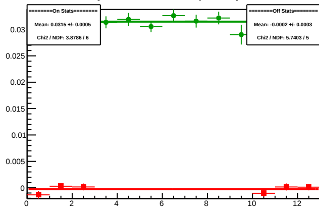
Cycle 5794.18: Multiplet Asyms
