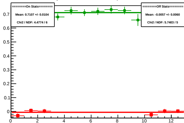
Cycle 5794.18: Multiplet Diff
