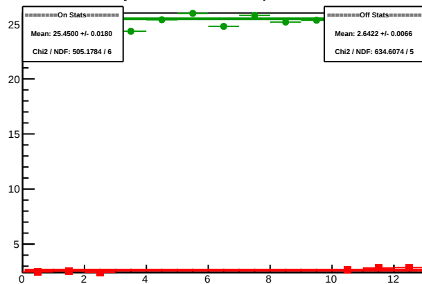
Cycle 5794.18: Multiplet Sums
