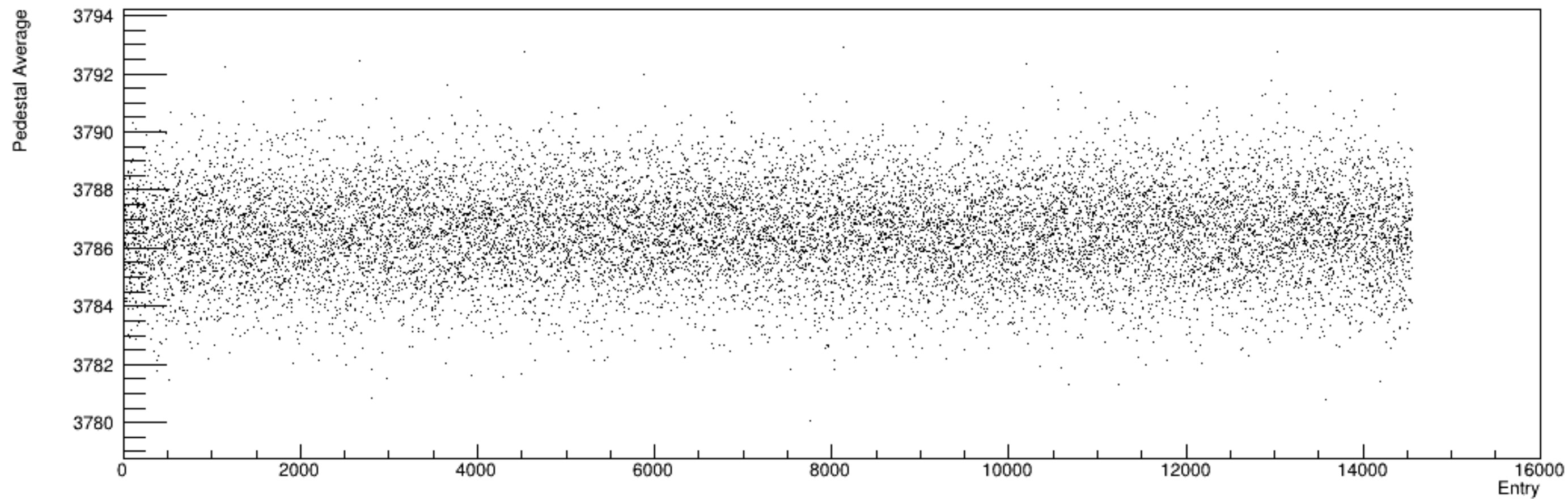
Run 5797, snapshots: Pedestal vs. Time
