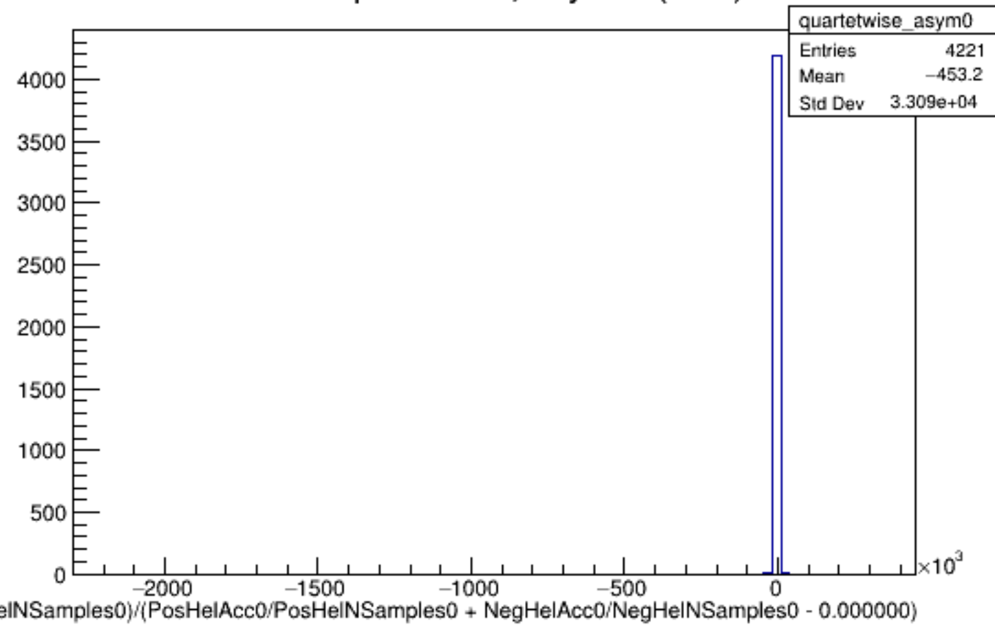
Run 5800 quartetwise, Asyms0 (Raw): All
