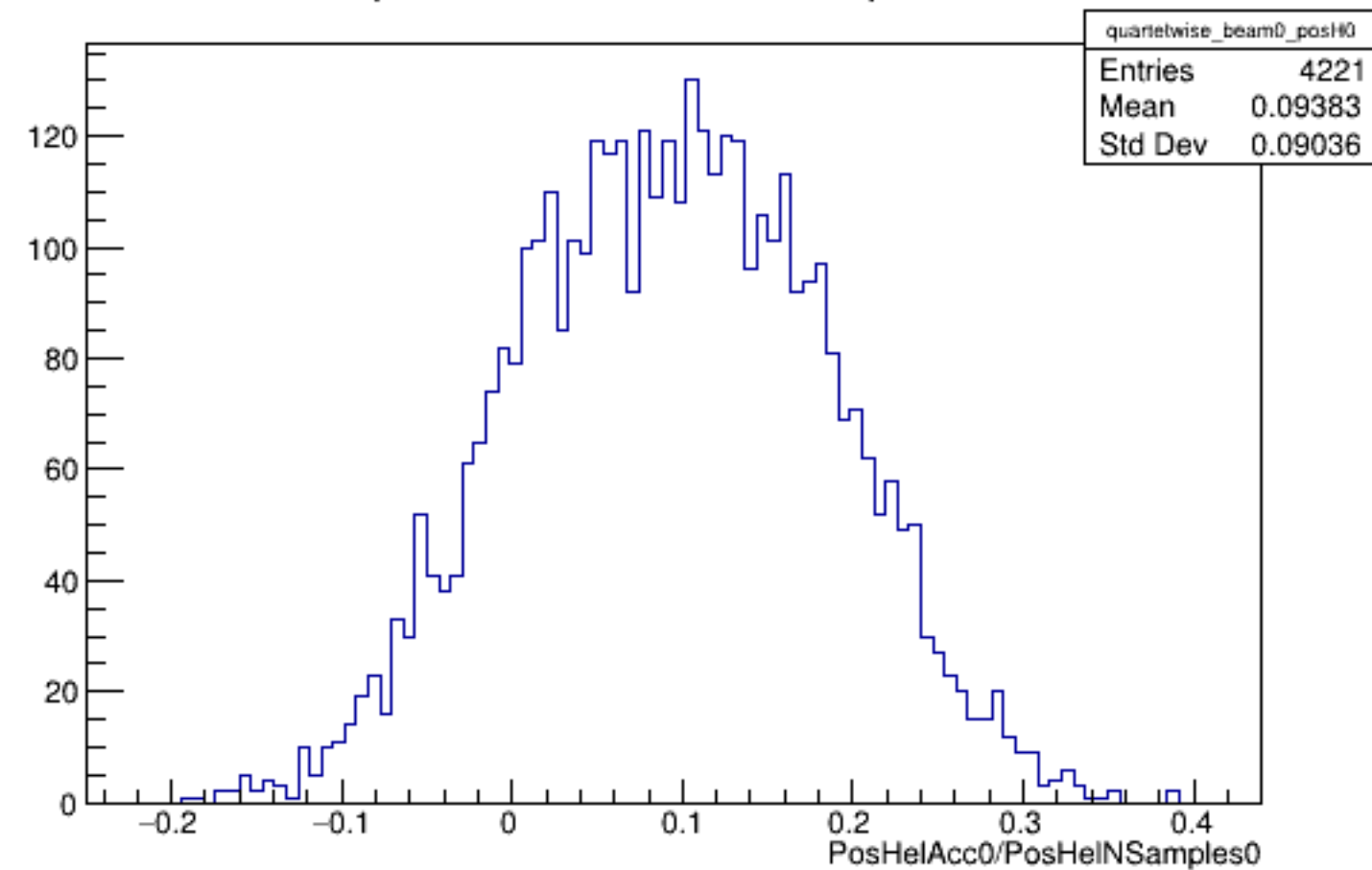
Run 5800 quartetwise, PosHelAcc0/NSamples0: Beam OFF
