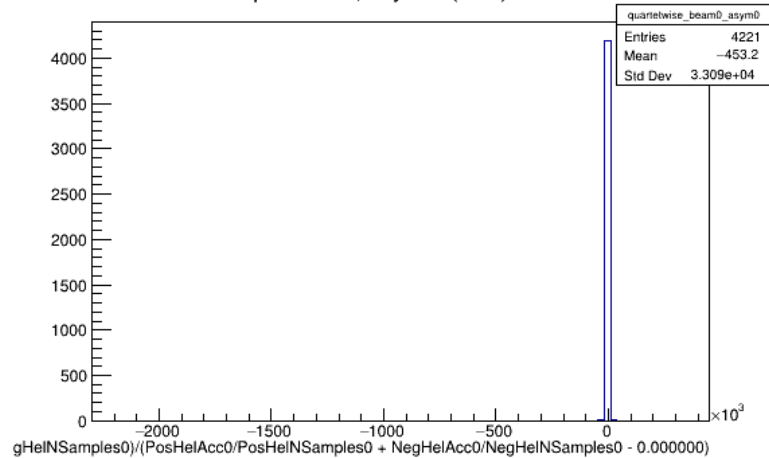
Run 5800 quartetwise, Asyms0 (Raw): Beam OFF
