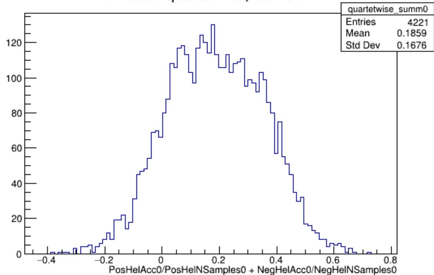
Run 5800 quartetwise, Sums0: All
