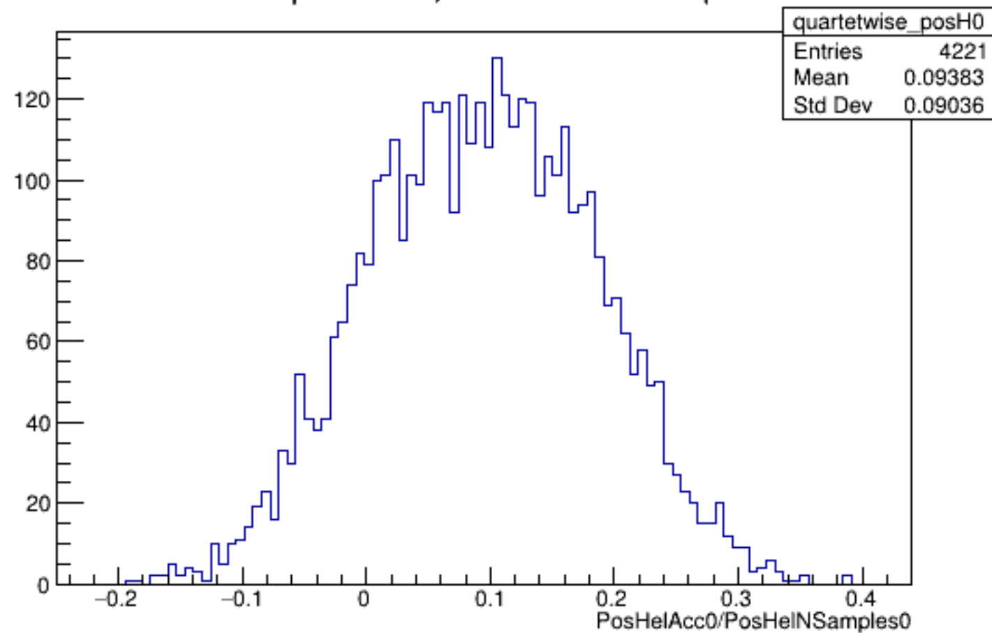
Run 5800 quartetwise, PosHelAcc0/NSamples0: All
