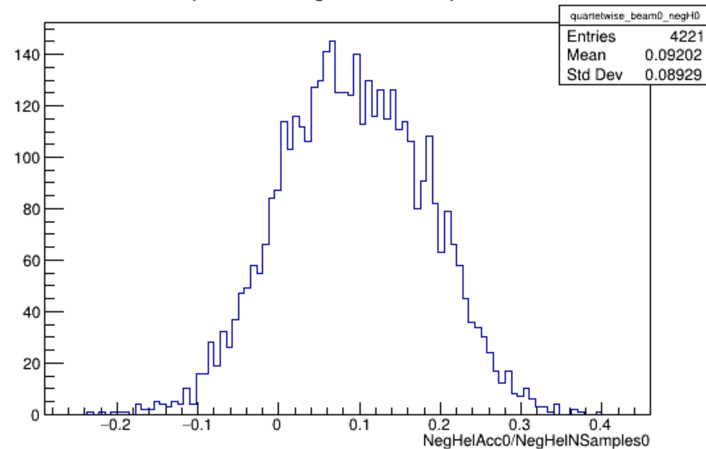
Run 5800 quartetwise, NegHelAcc0/NSamples0: Beam OFF
