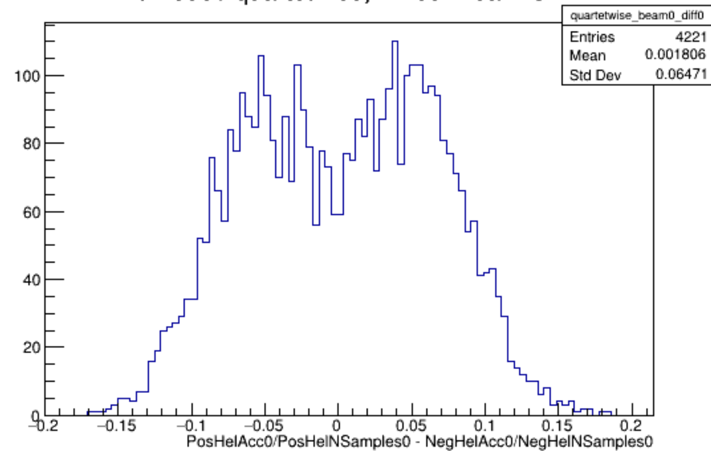
Run 5800 quartetwise, Diffs0: Beam OFF
