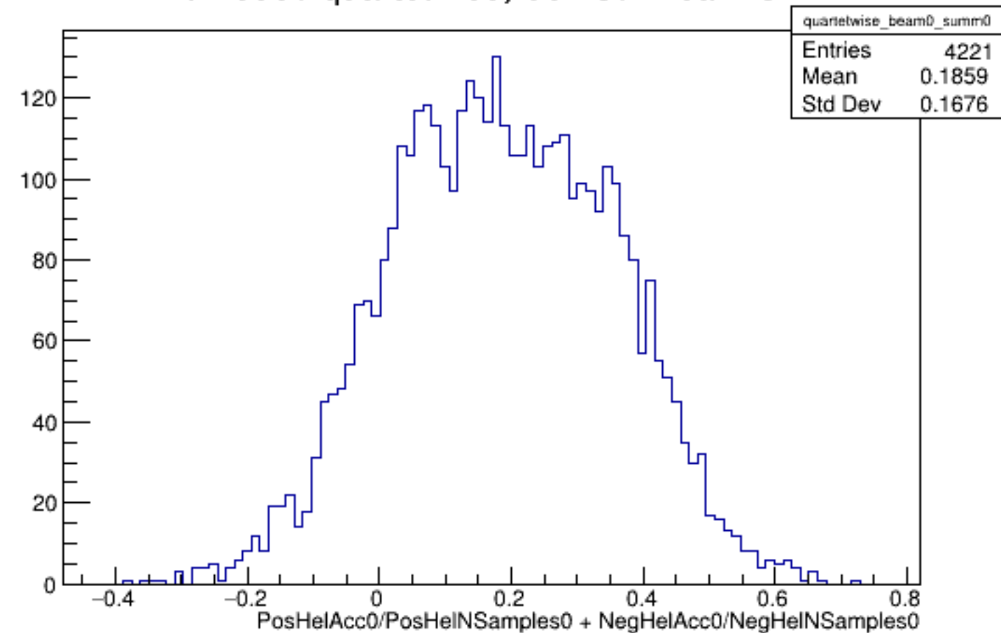
Run 5800 quartetwise, Sums0: Beam OFF
