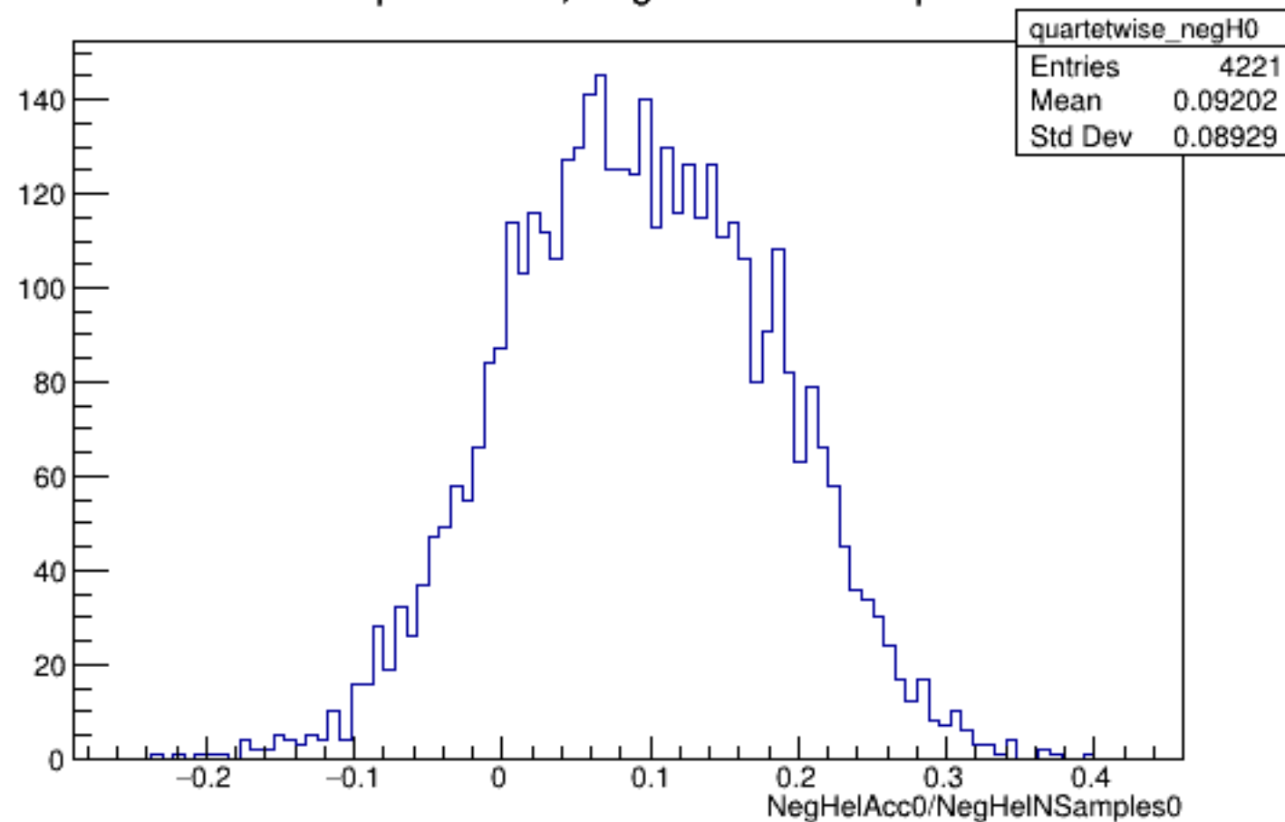
Run 5800 quartetwise, NegHelAcc0/NSamples0: All
