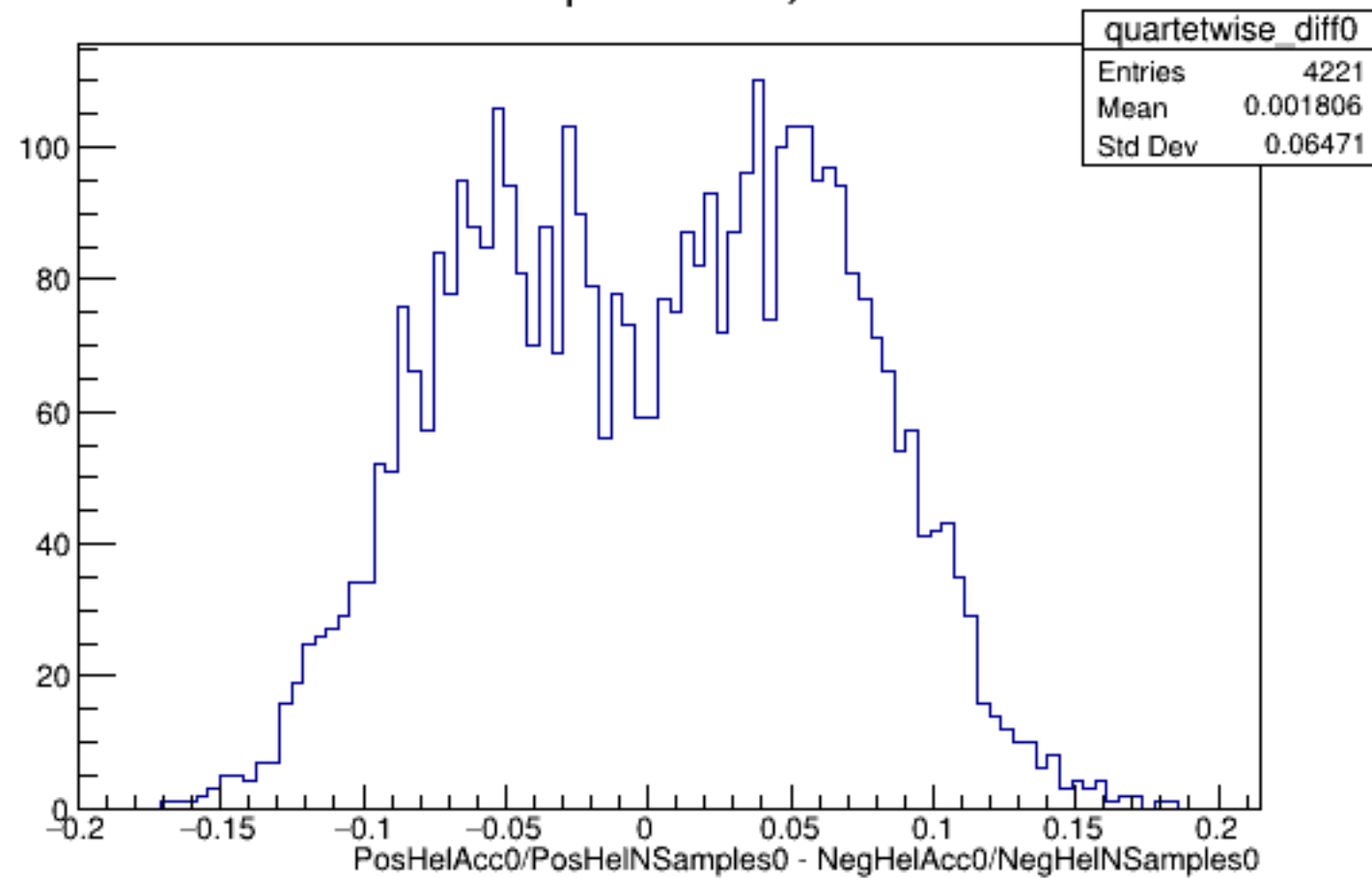
Run 5800 quartetwise, Diffs0: All
