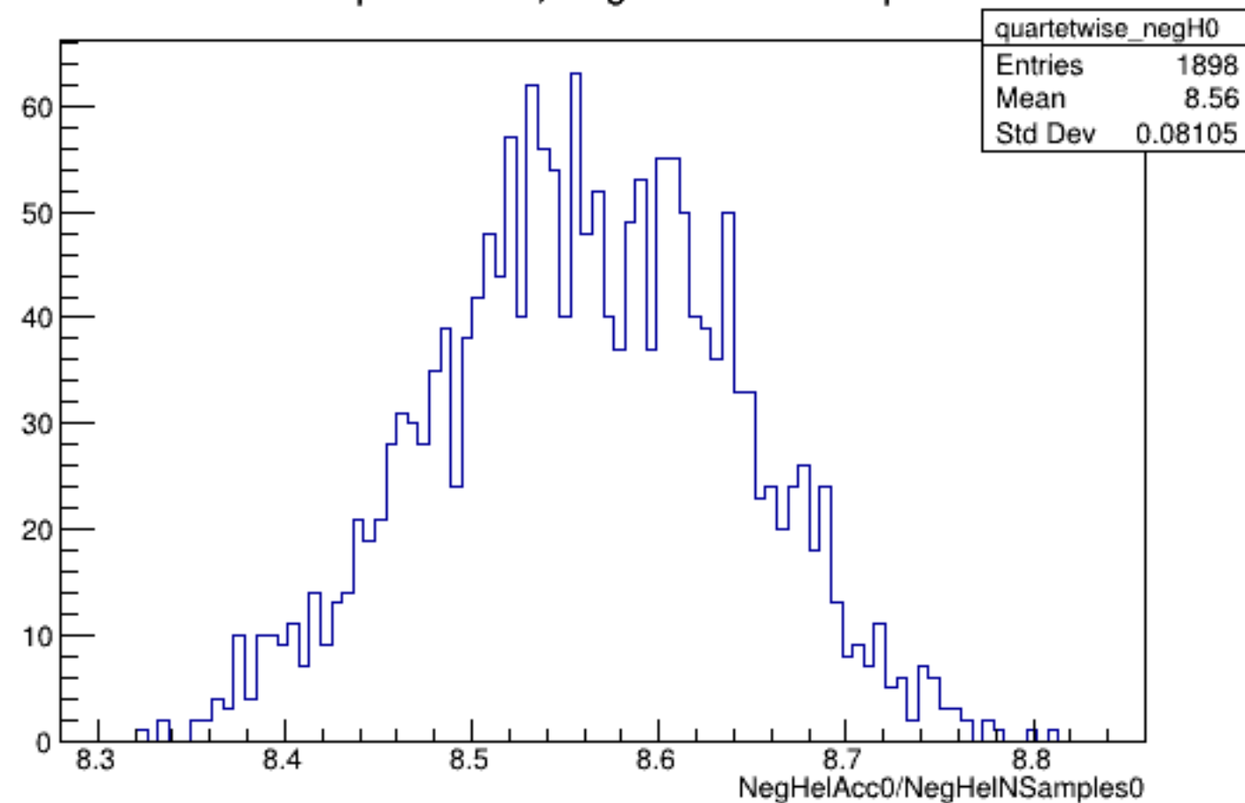
Run 5814 quartetwise, NegHelAcc0/NSamples0: All
