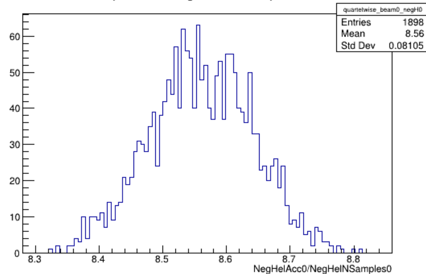
Run 5814 quartetwise, NegHelAcc0/NSamples0: Beam OFF
