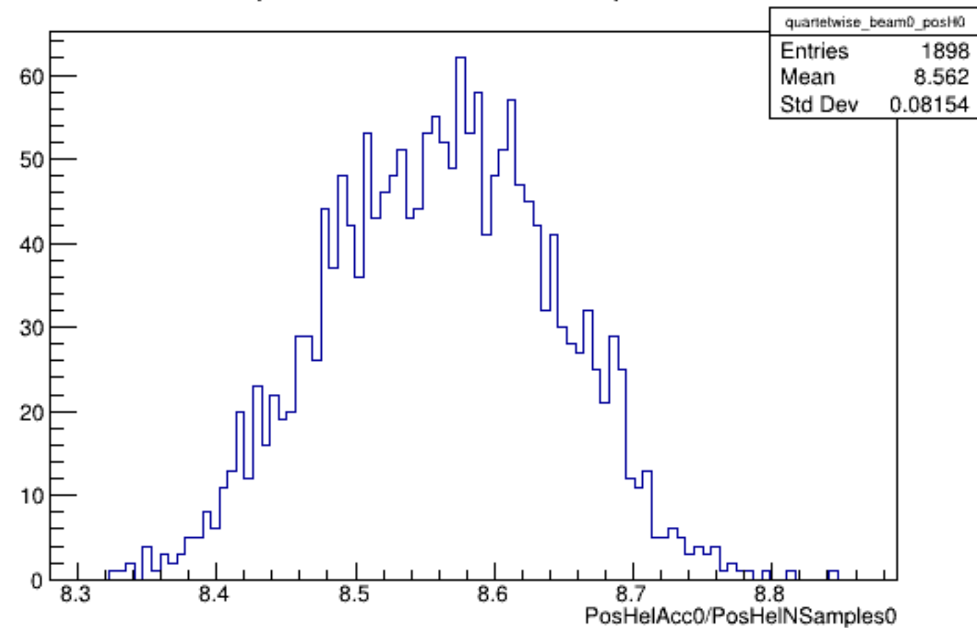
Run 5814 quartetwise, PosHelAcc0/NSamples0: Beam OFF
