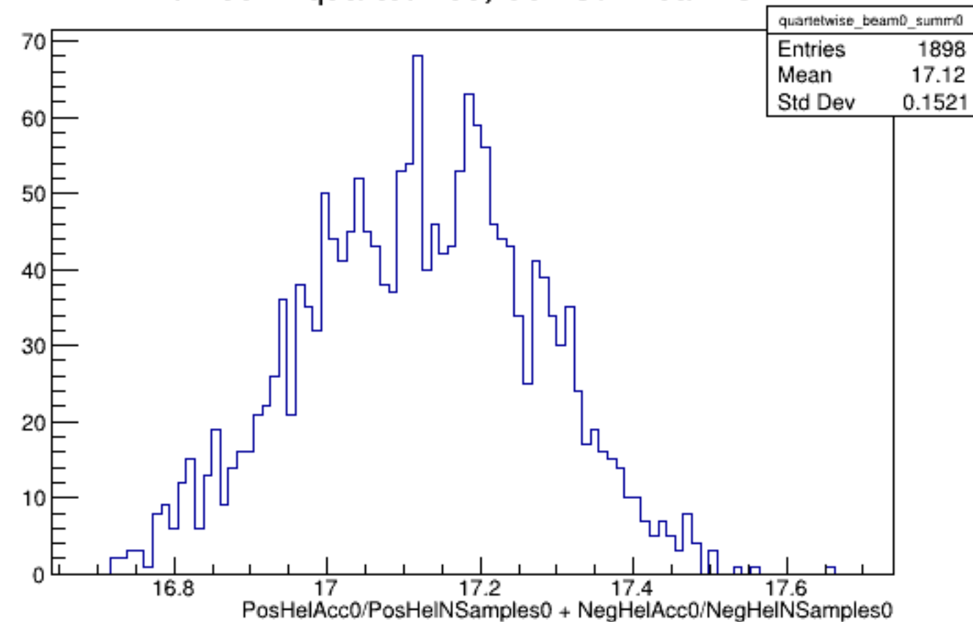
Run 5814 quartetwise, Sums0: Beam OFF
