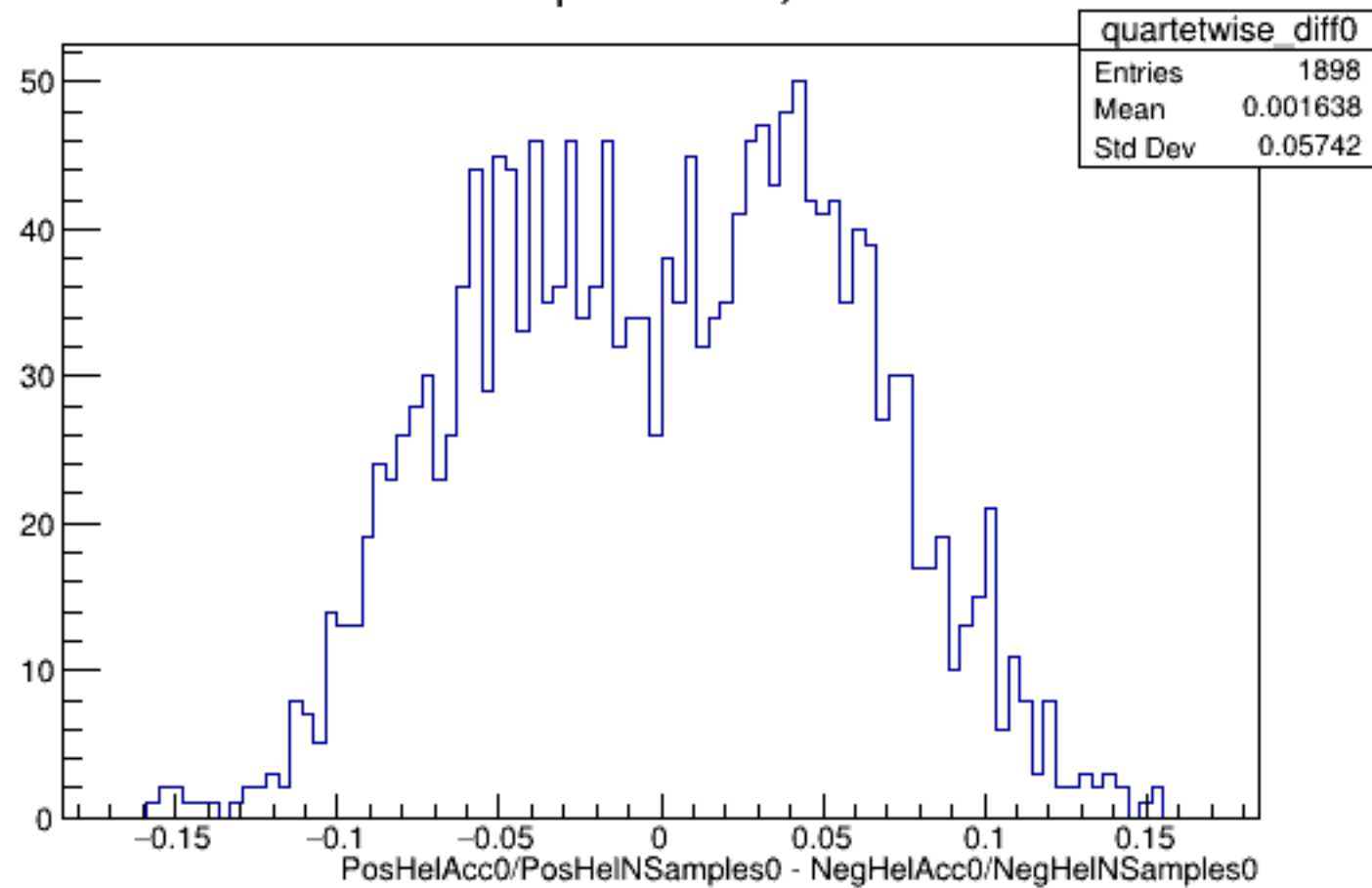
Run 5814 quartetwise, Diffs0: All
