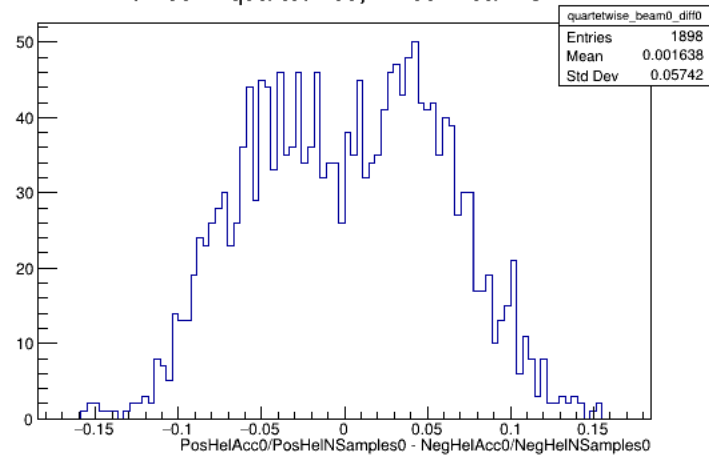
Run 5814 quartetwise, Diffs0: Beam OFF
