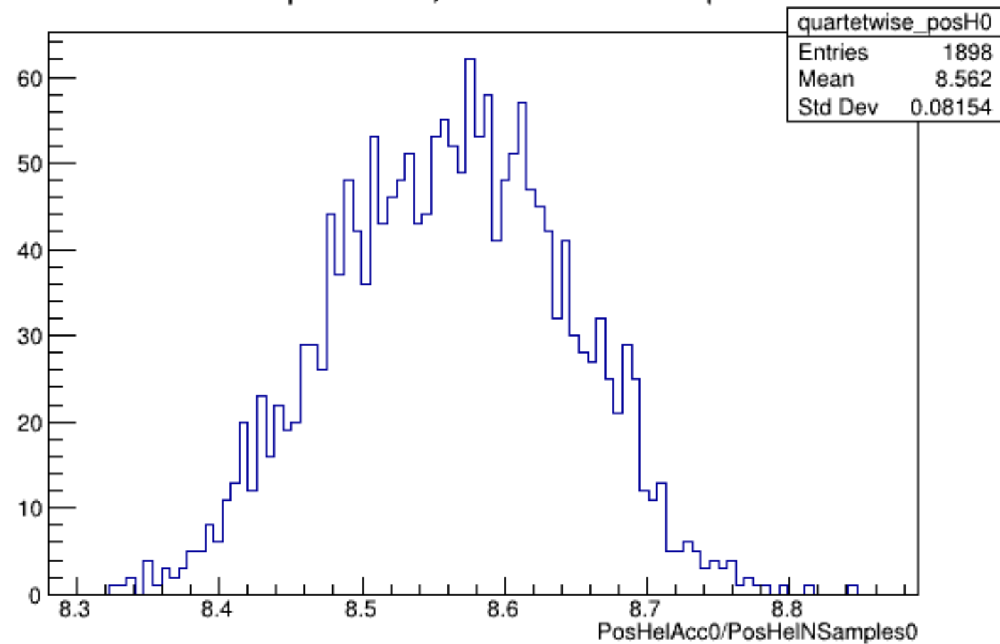
Run 5814 quartetwise, PosHelAcc0/NSamples0: All
