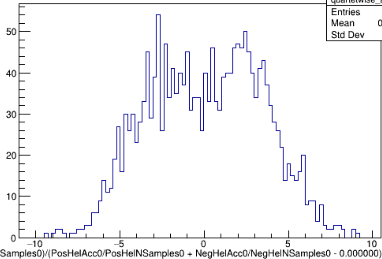
Run 5814 quartetwise, Asyms0 (Raw): All
