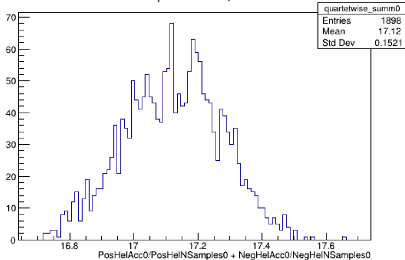
Run 5814 quartetwise, Sums0: All
