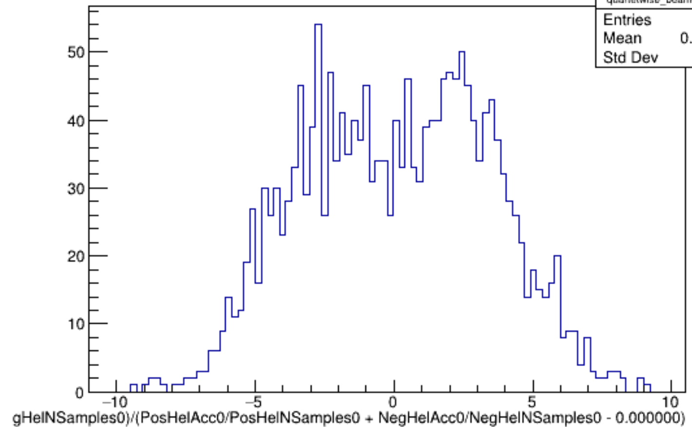
Run 5814 quartetwise, Asyms0 (Raw): Beam OFF
