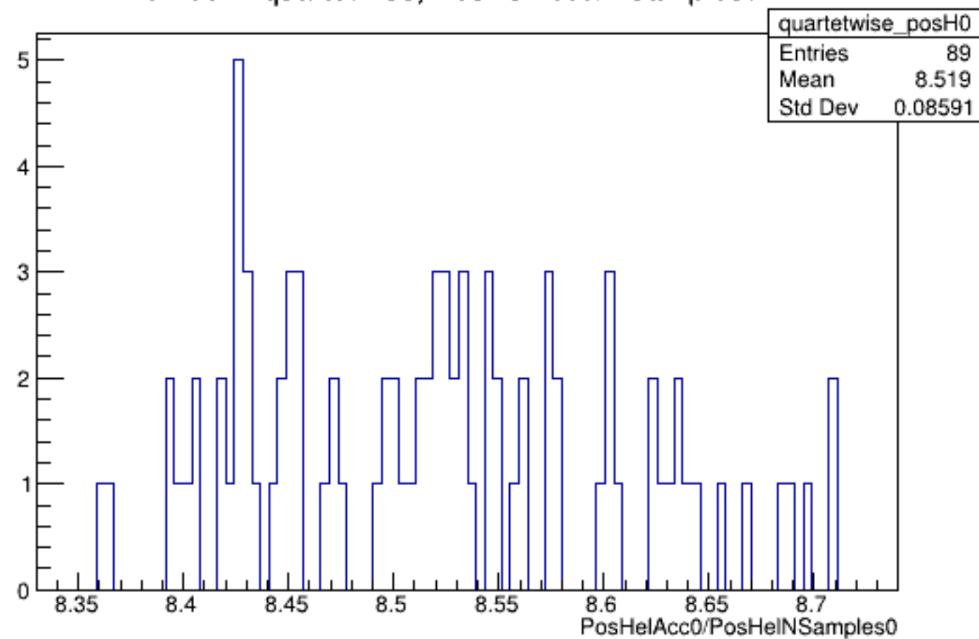
Run 5817 quartetwise, PosHelAcc0/NSamples0: All
