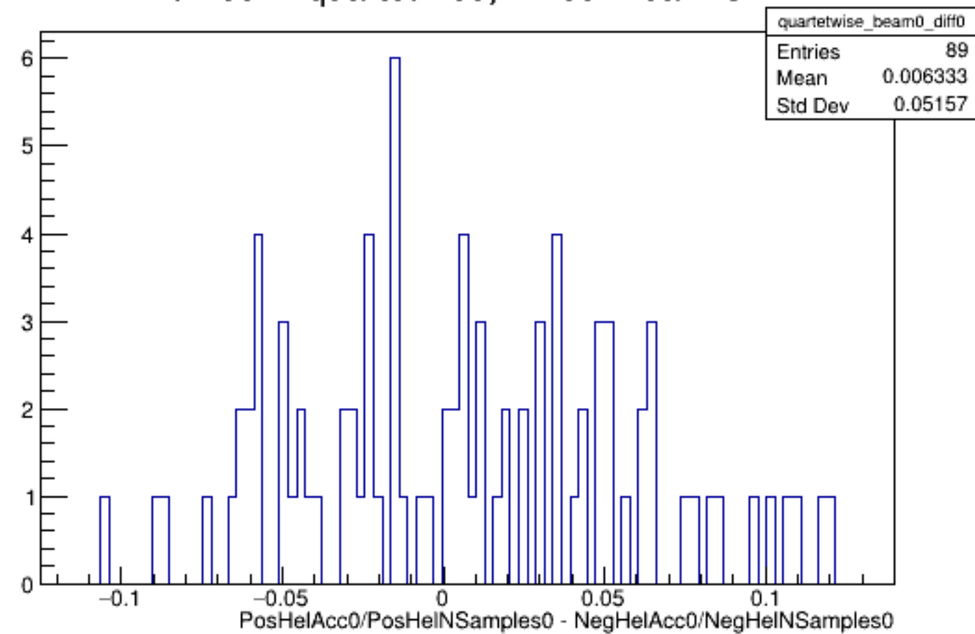
Run 5817 quartetwise, Diffs0: Beam OFF
