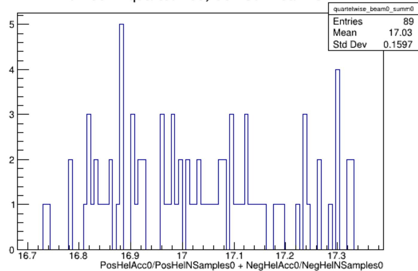
Run 5817 quartetwise, Sums0: Beam OFF
