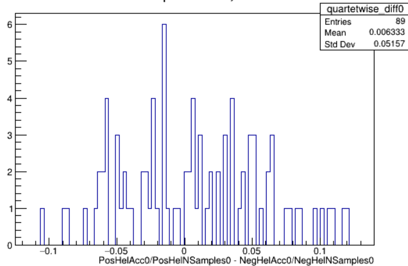
Run 5817 quartetwise, Diffs0: All
