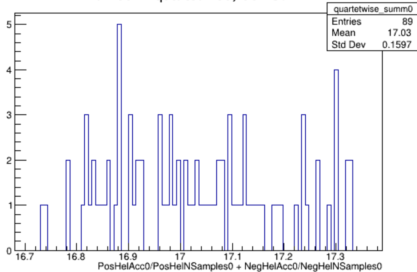
Run 5817 quartetwise, Sums0: All
