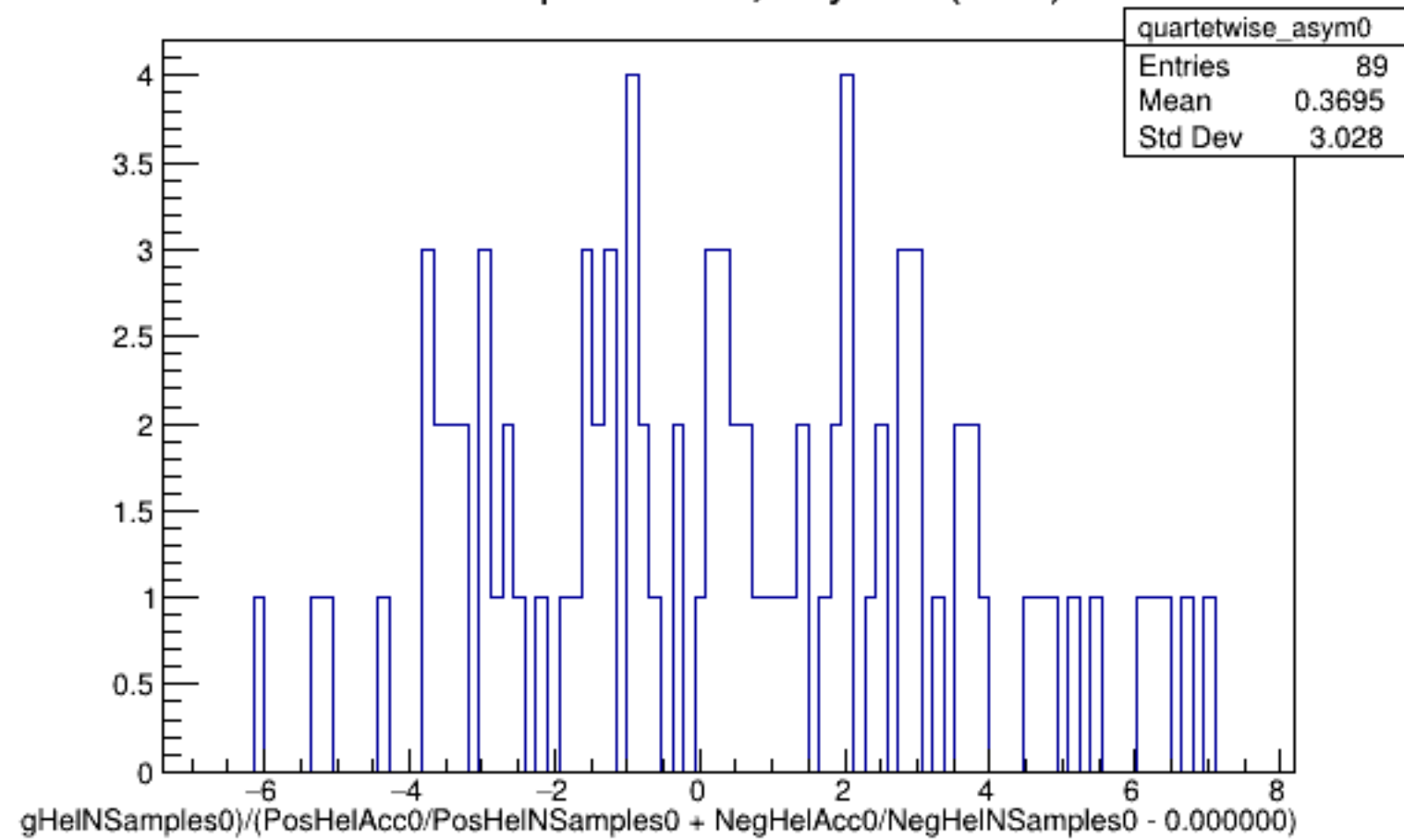
Run 5817 quartetwise, Asyms0 (Raw): All
