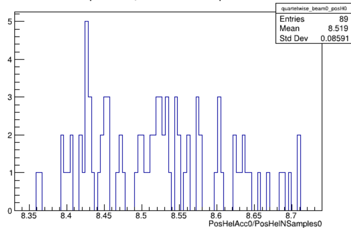
Run 5817 quartetwise, PosHelAcc0/NSamples0: Beam OFF
