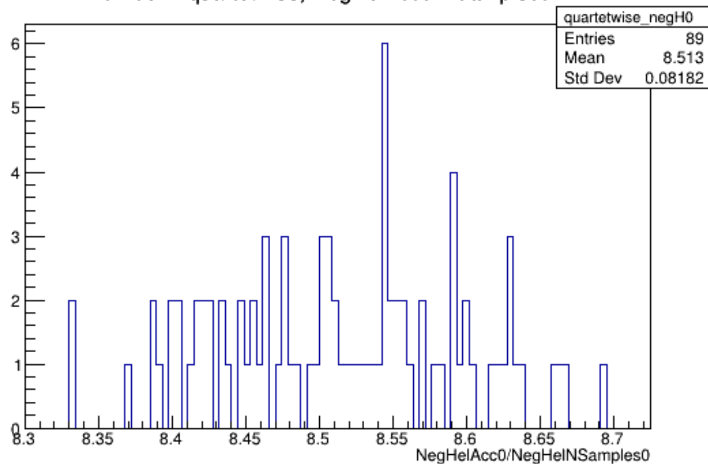
Run 5817 quartetwise, NegHelAcc0/NSamples0: All
