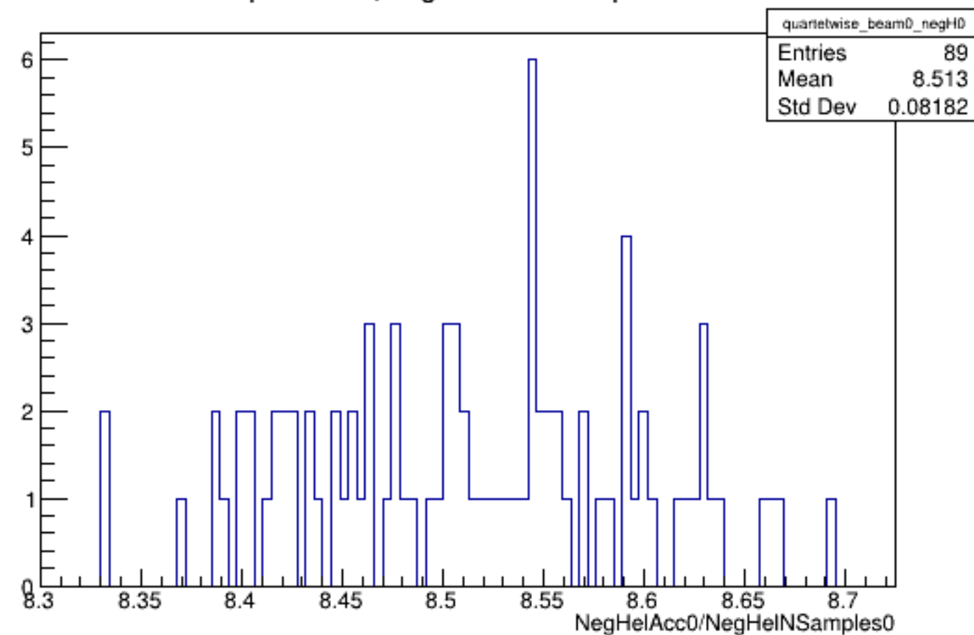
Run 5817 quartetwise, NegHelAcc0/NSamples0: Beam OFF
