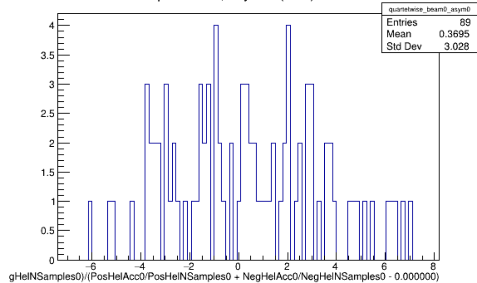
Run 5817 quartetwise, Asyms0 (Raw): Beam OFF
