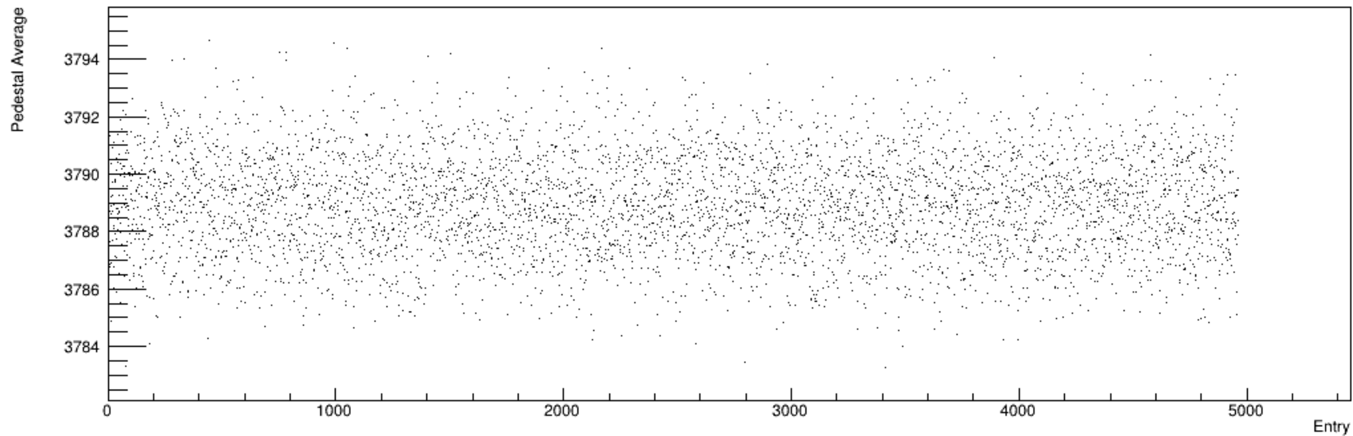
Run 5821, snapshots: Pedestal vs. Time
