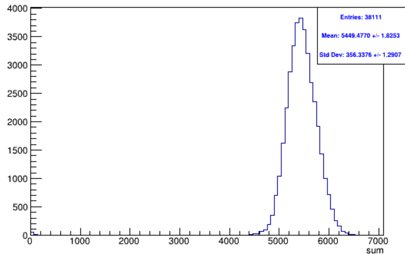
Run 5821 triggerwise, sums: Beam OFF
