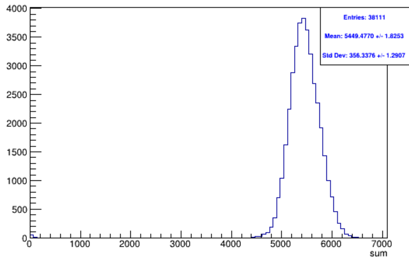
Run 5821 triggerwise, sums: All
