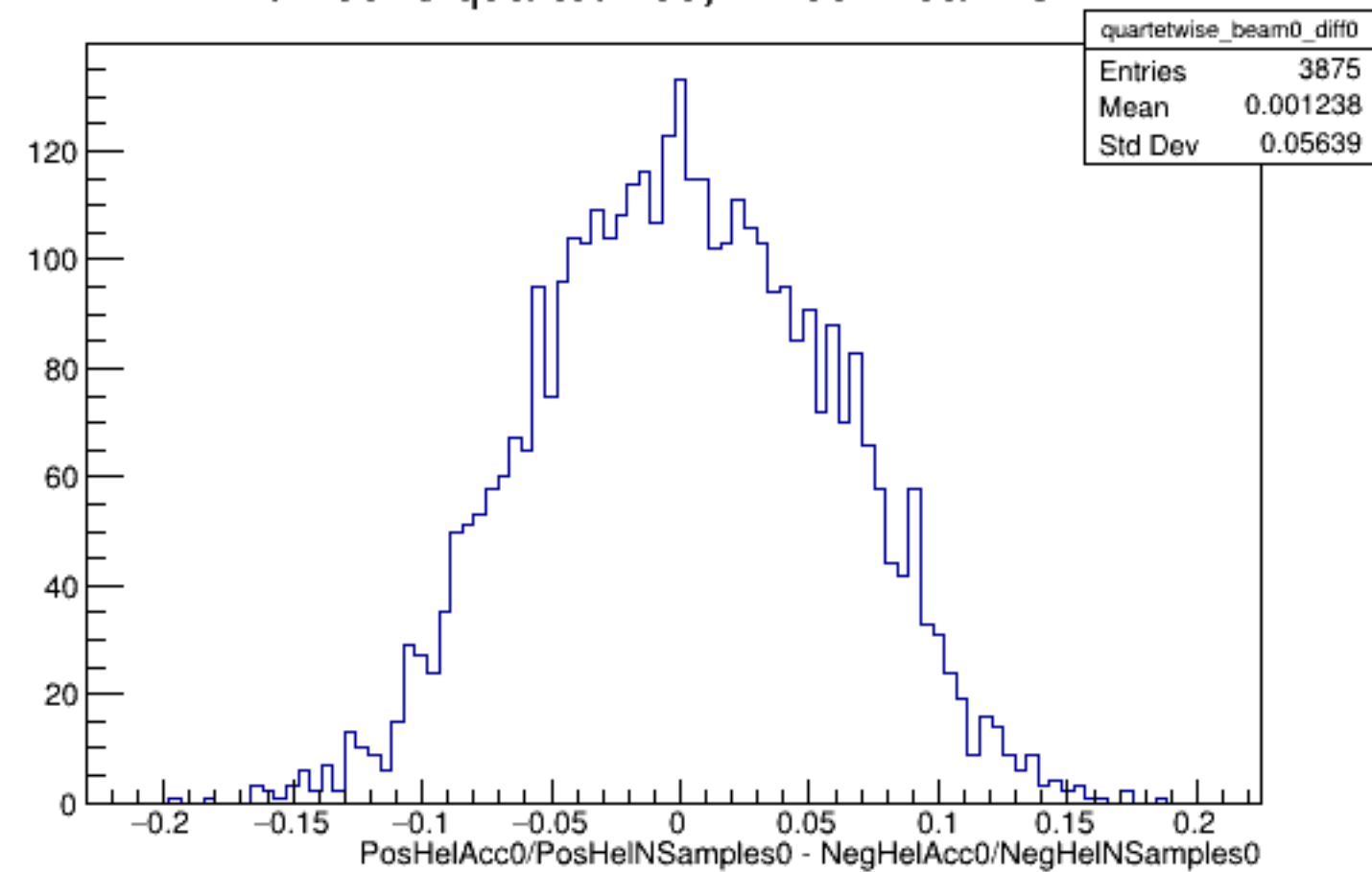
Run 5823 quartetwise, Diffs0: Beam OFF
