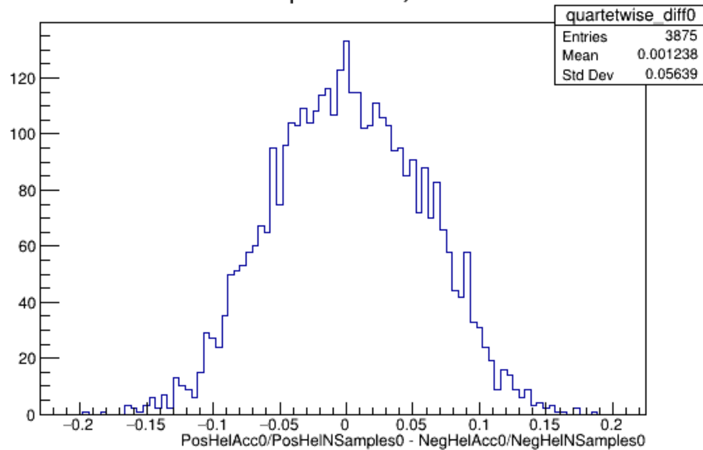
Run 5823 quartetwise, Diffs0: All
