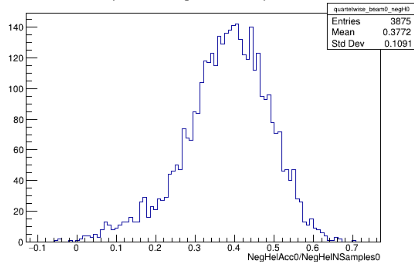
Run 5823 quartetwise, NegHelAcc0/NSamples0: Beam OFF
