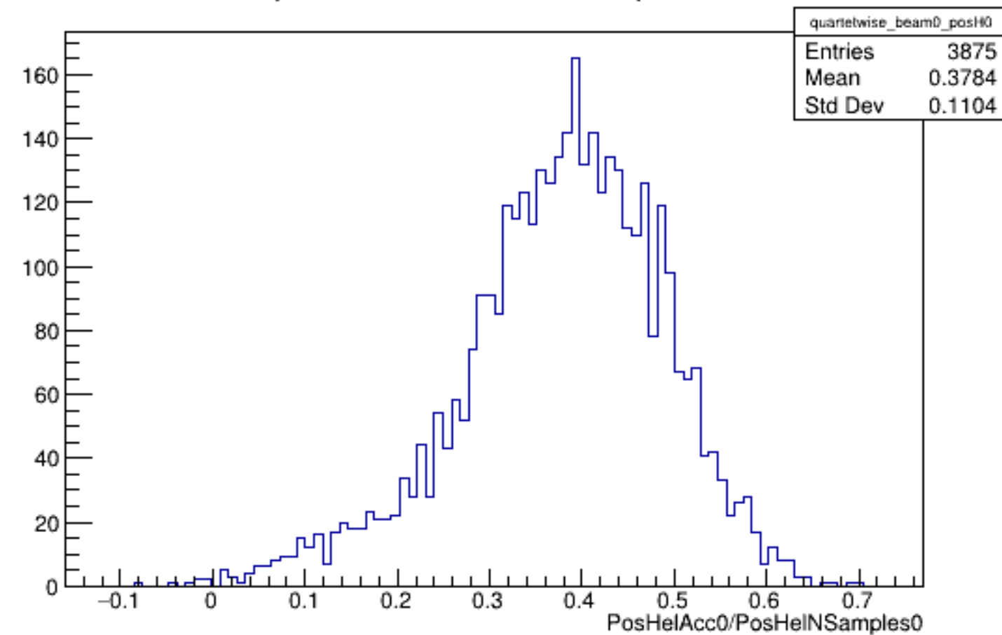
Run 5823 quartetwise, PosHelAcc0/NSamples0: Beam OFF
