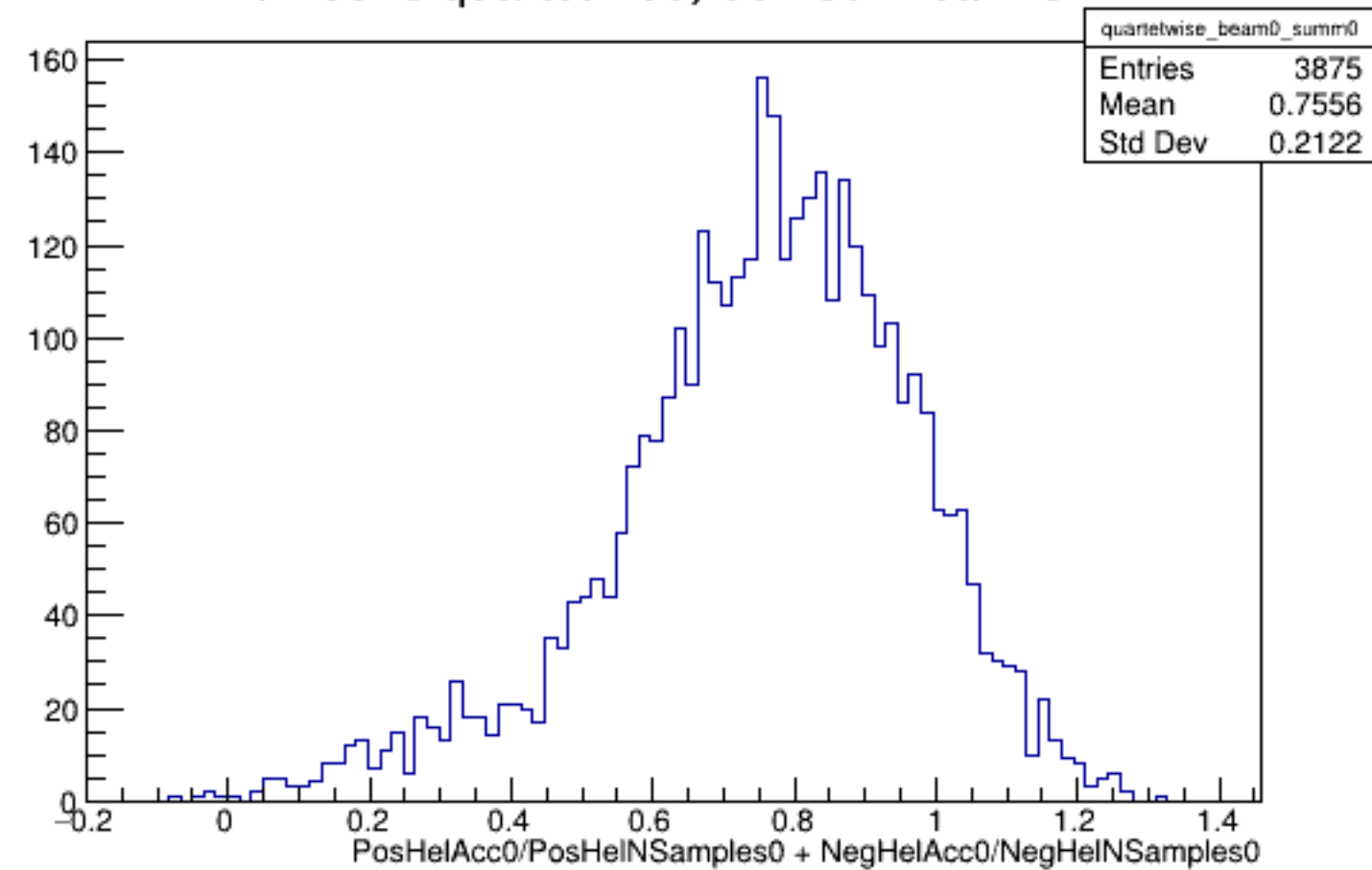
Run 5823 quartetwise, Sums0: Beam OFF
