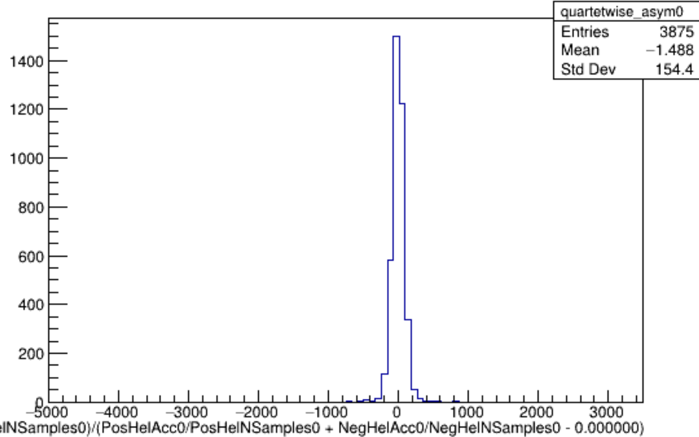
Run 5823 quartetwise, Asyms0 (Raw): All
