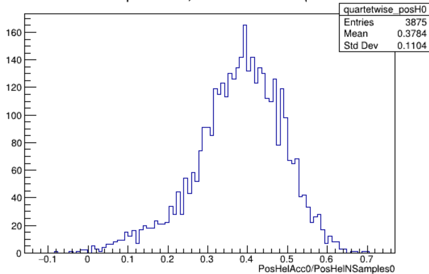
Run 5823 quartetwise, PosHelAcc0/NSamples0: All
