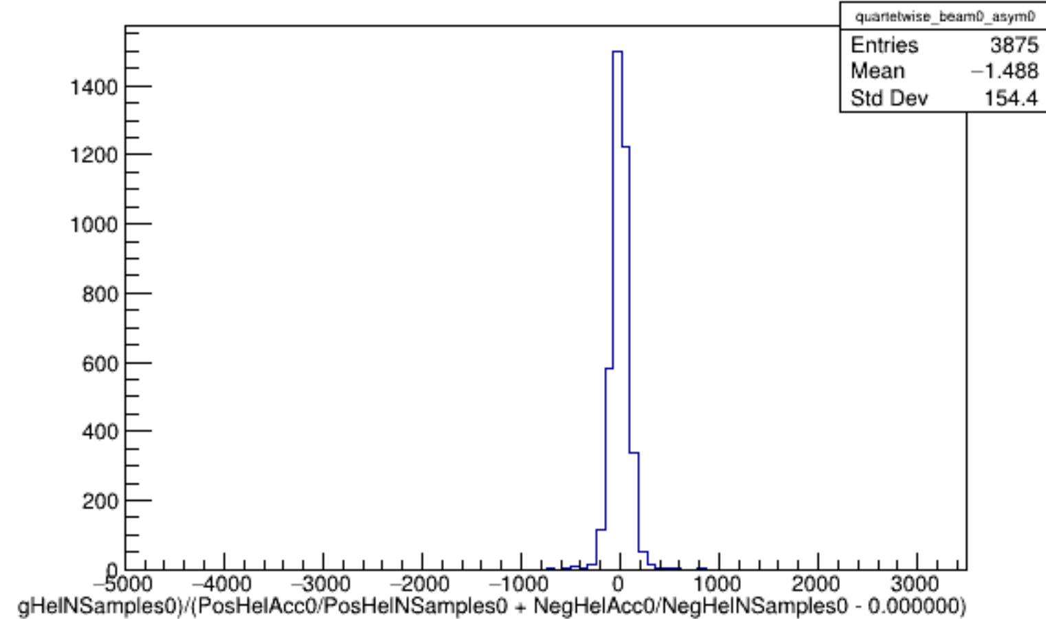
Run 5823 quartetwise, Asyms0 (Raw): Beam OFF
