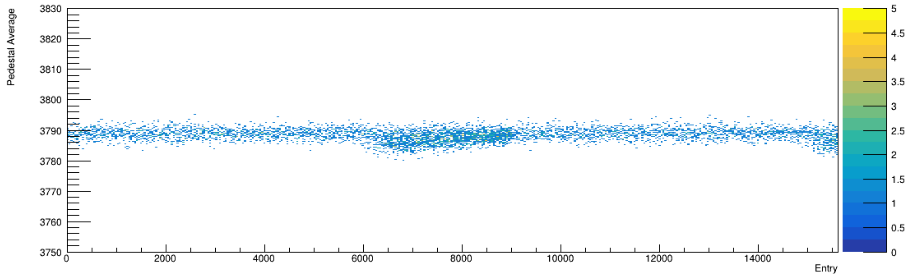
Run 5823, snapshots: Pedestal vs. Time
