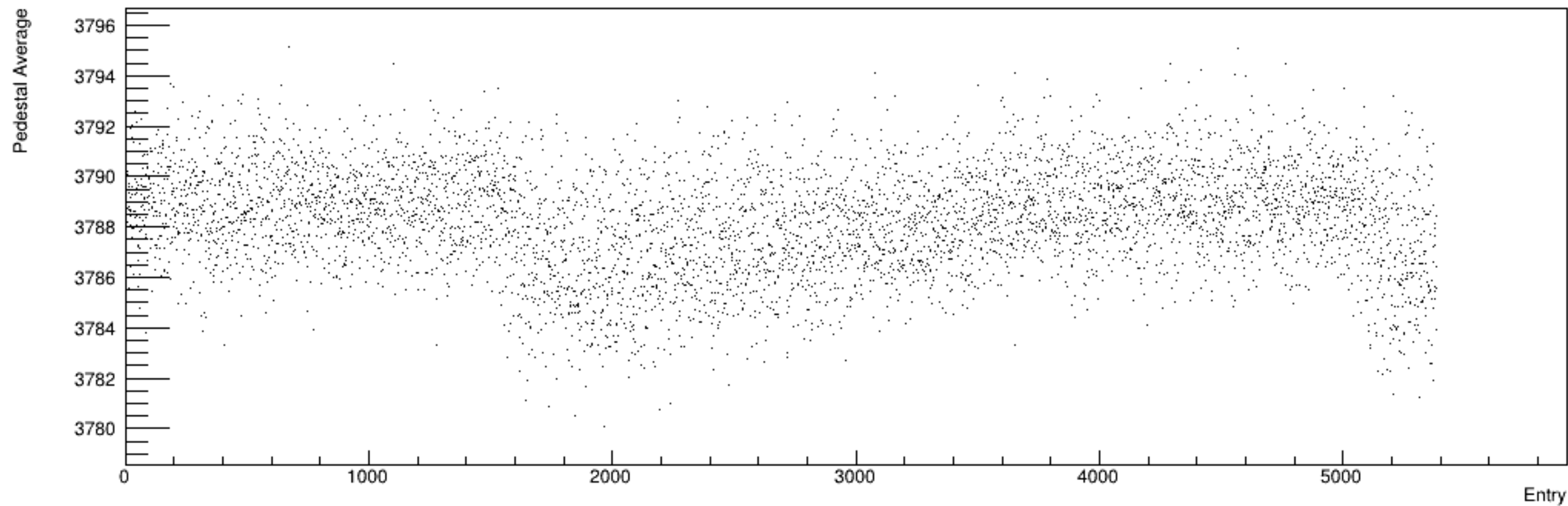
Run 5823, snapshots: Pedestal vs. Time
