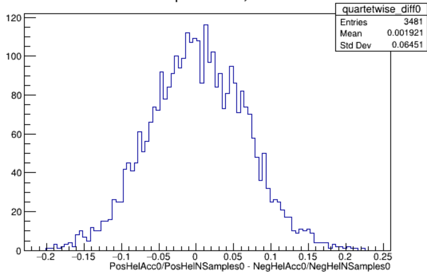
Run 5826 quartetwise, Diffs0: All
