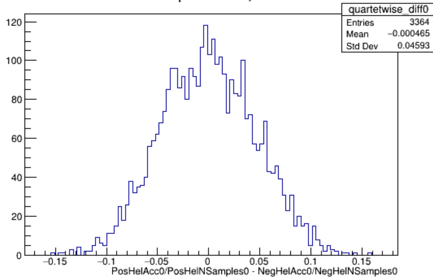
Run 5828 quartetwise, Diffs0: All
