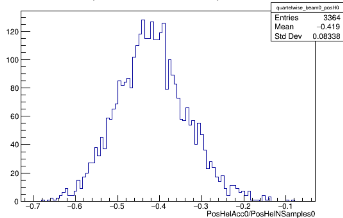
Run 5828 quartetwise, PosHelAcc0/NSamples0: Beam OFF
