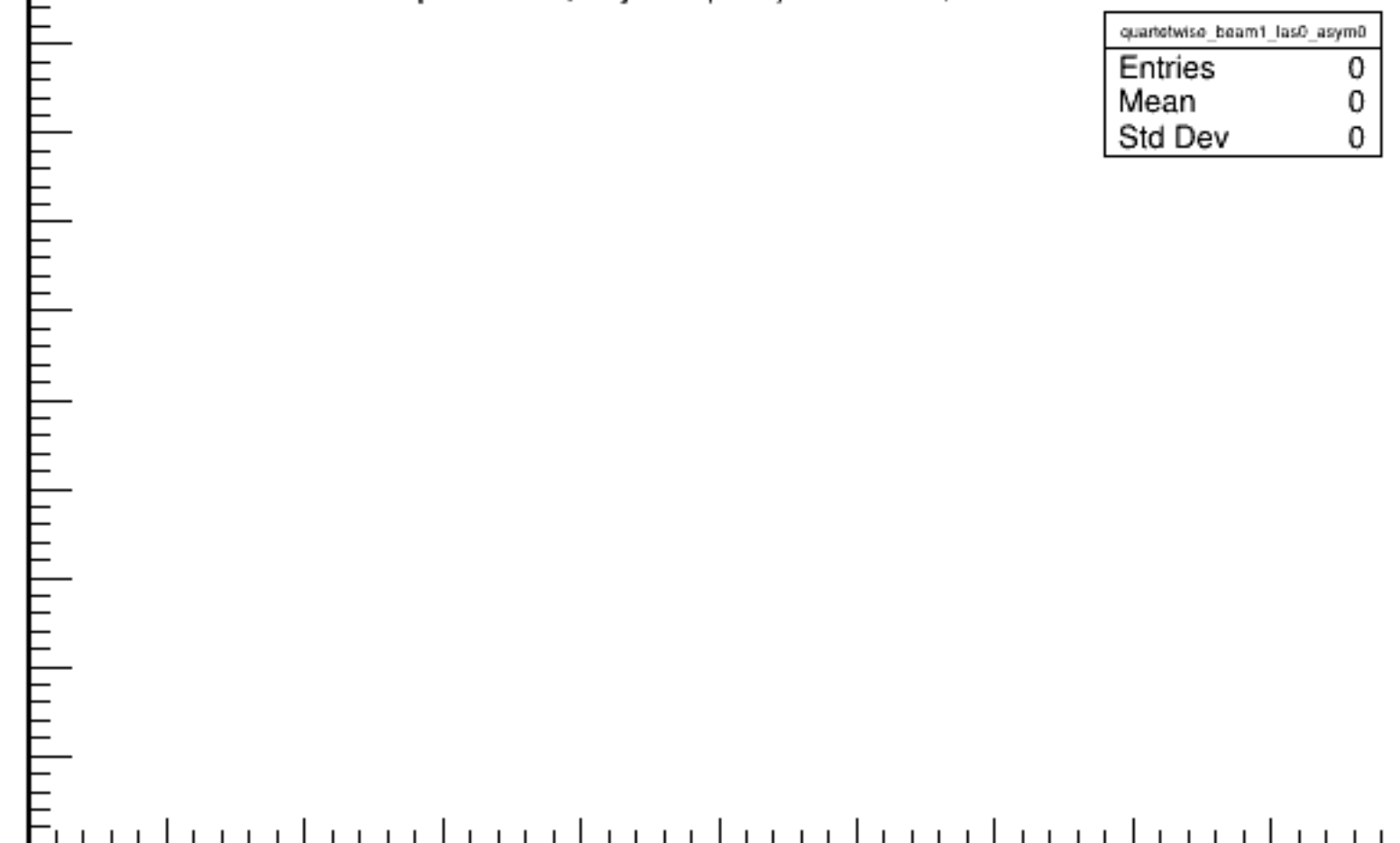
Run 5828 quartetwise, Asyms0 (Raw): Beam ON, Laser OFF
