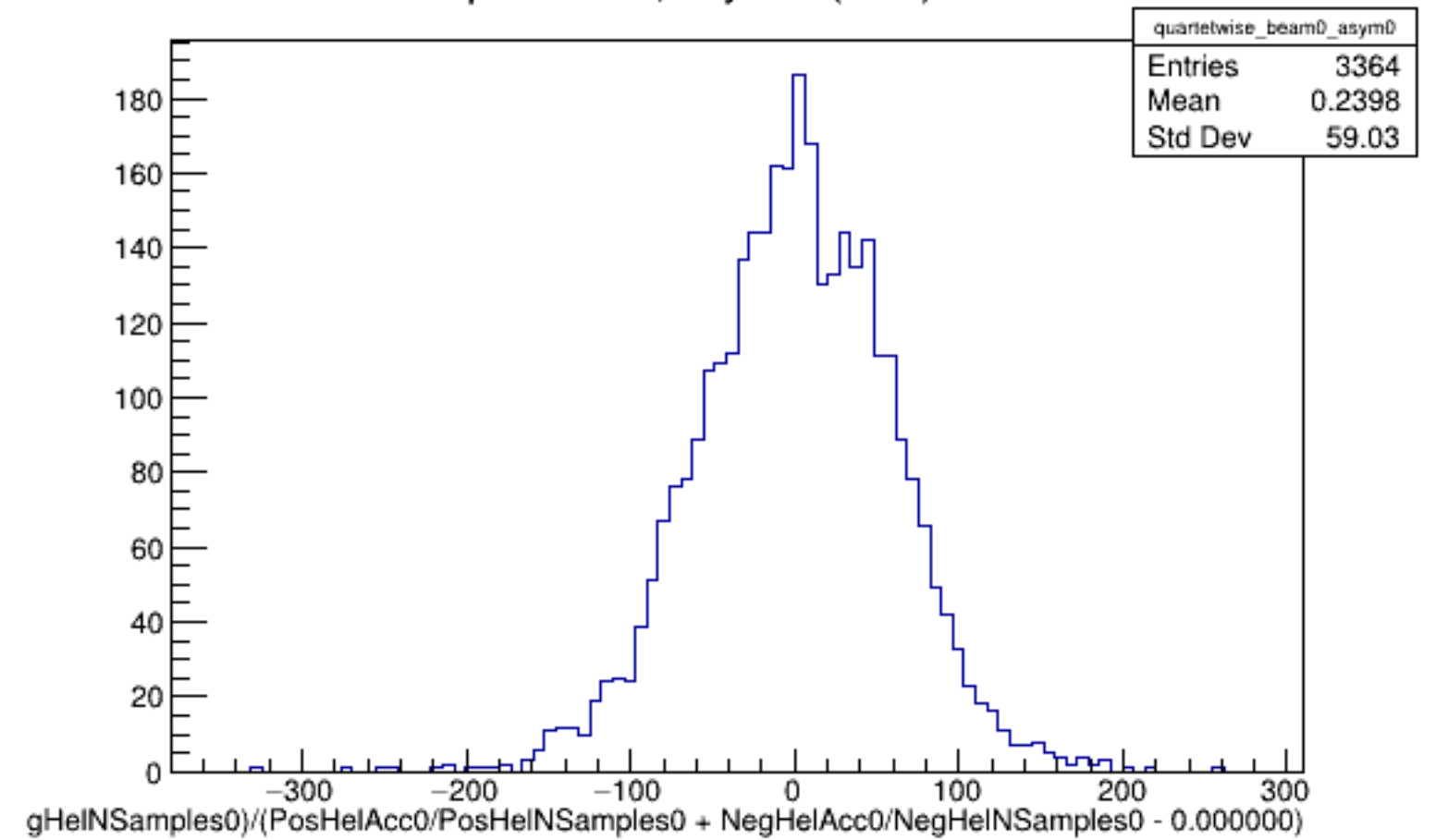
Run 5828 quartetwise, Asyms0 (Raw): Beam OFF
