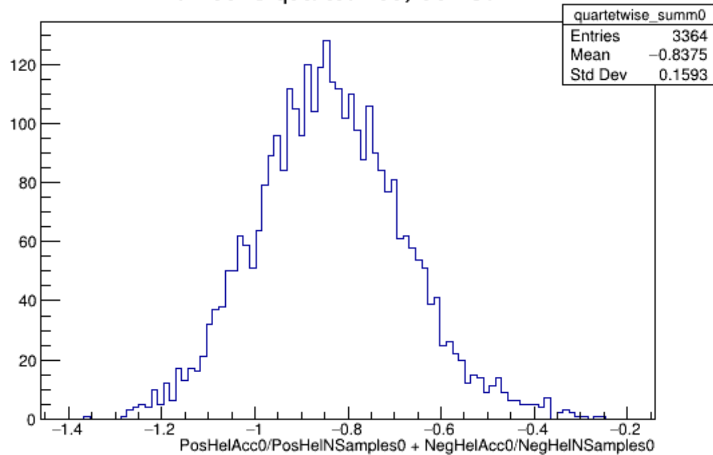
Run 5828 quartetwise, Sums0: All
