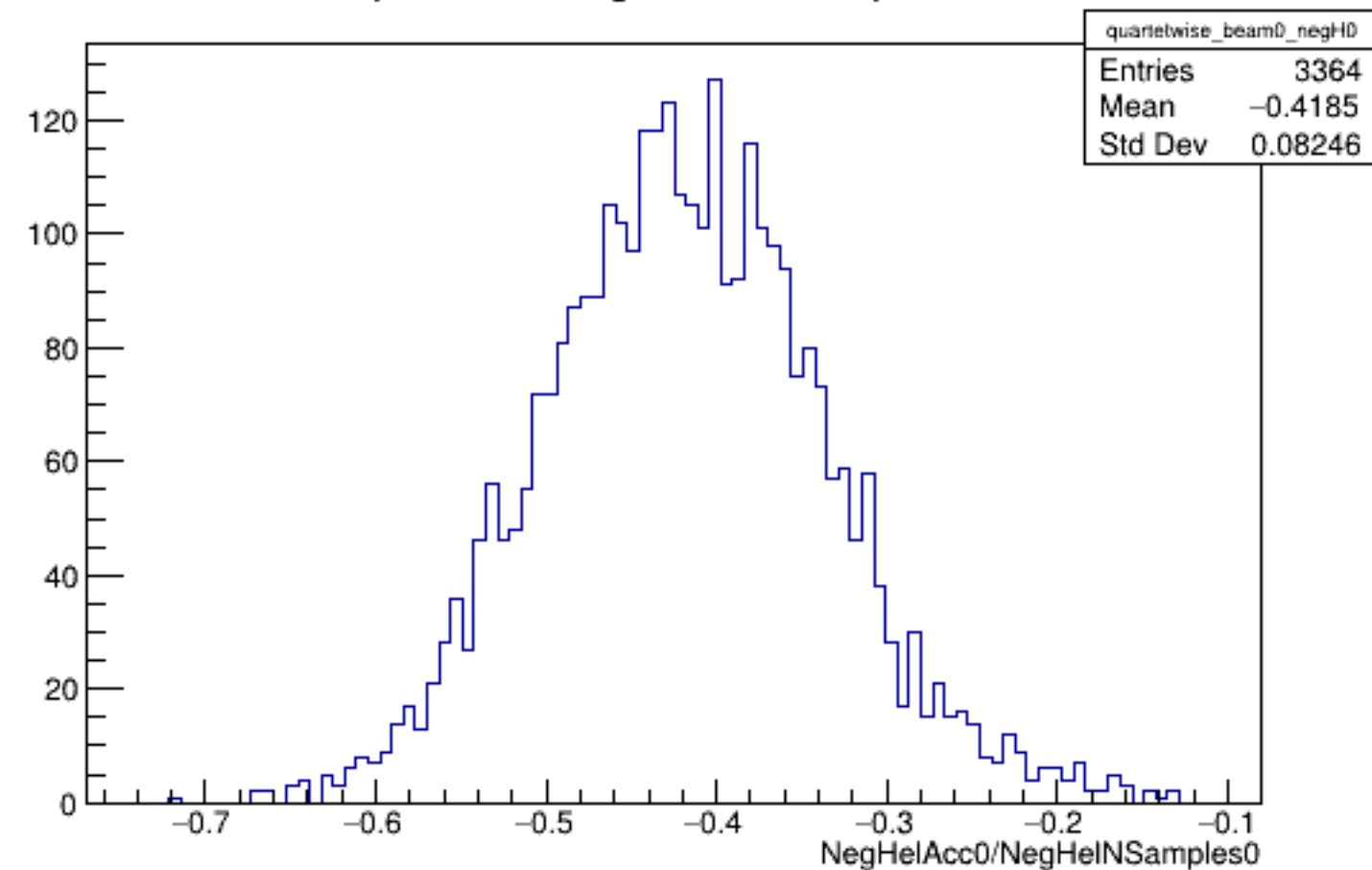
Run 5828 quartetwise, NegHelAcc0/NSamples0: Beam OFF
