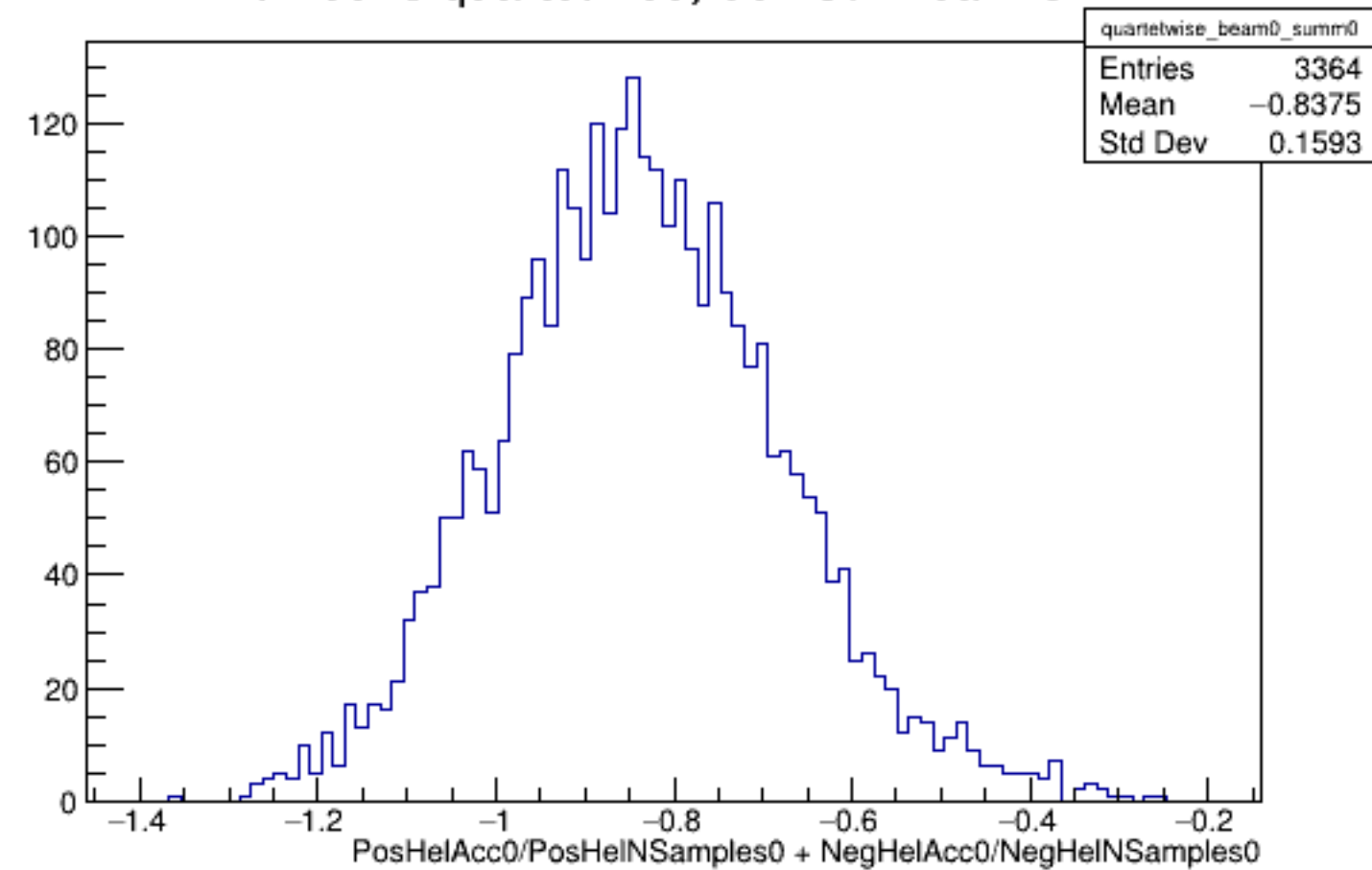
Run 5828 quartetwise, Sums0: Beam OFF
