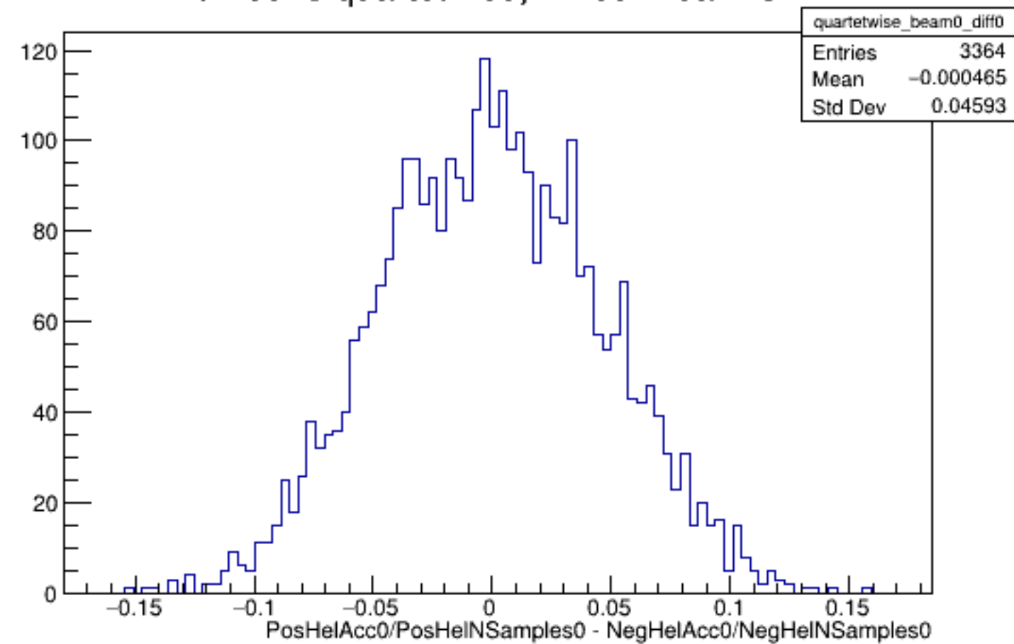
Run 5828 quartetwise, Diffs0: Beam OFF
