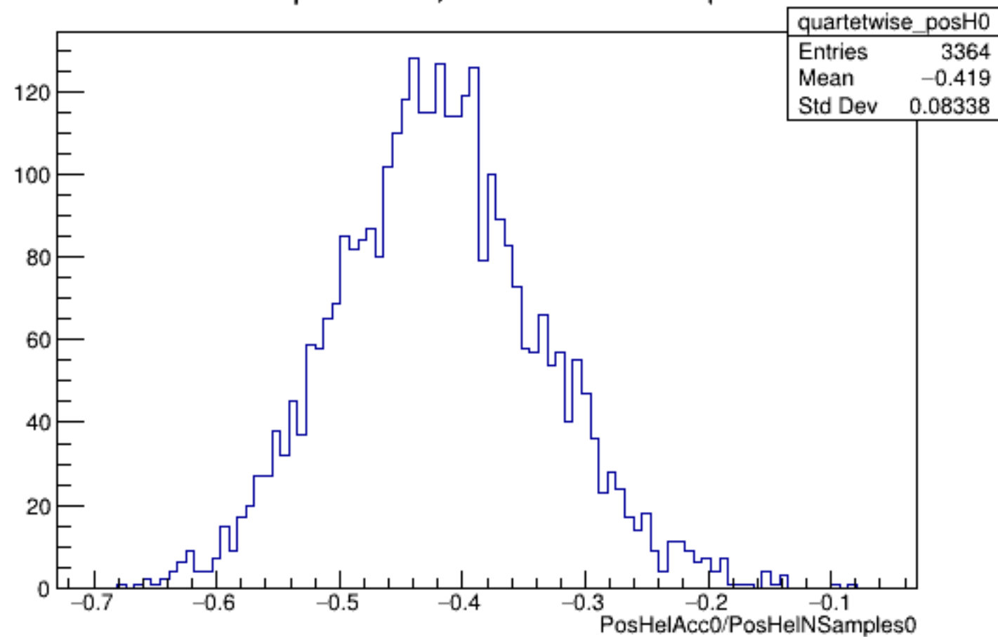
Run 5828 quartetwise, PosHelAcc0/NSamples0: All
