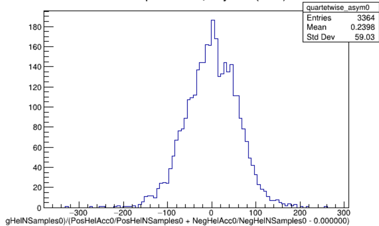
Run 5828 quartetwise, Asyms0 (Raw): All
