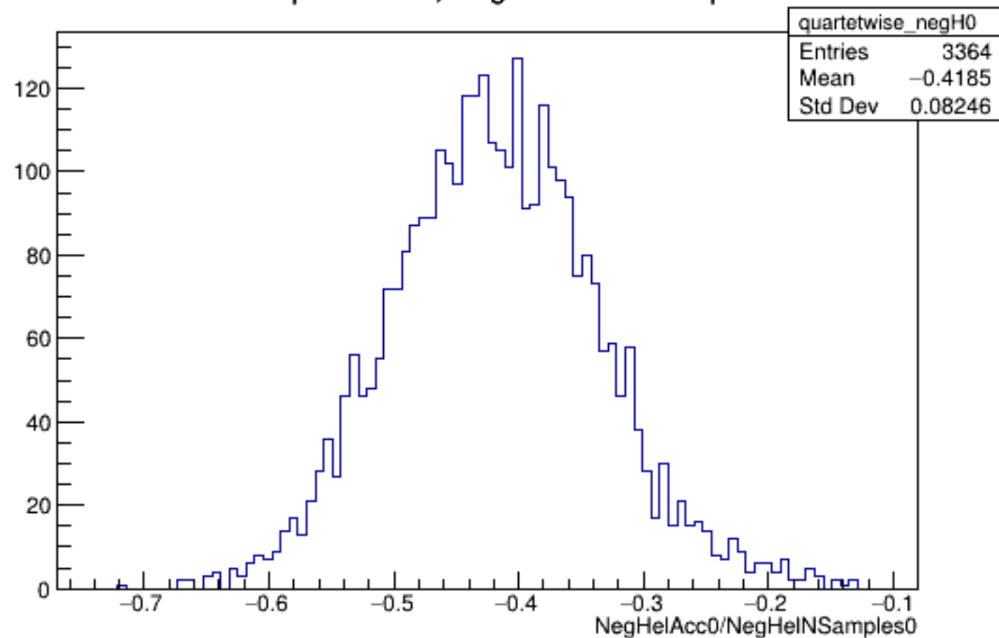
Run 5828 quartetwise, NegHelAcc0/NSamples0: All
