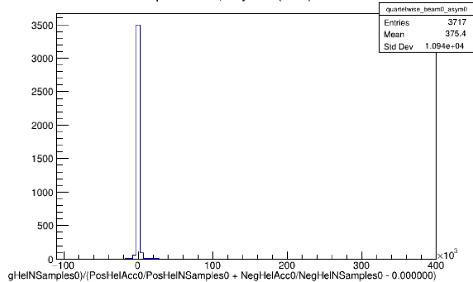
Run 5833 quartetwise, Asyms0 (Raw): Beam OFF
