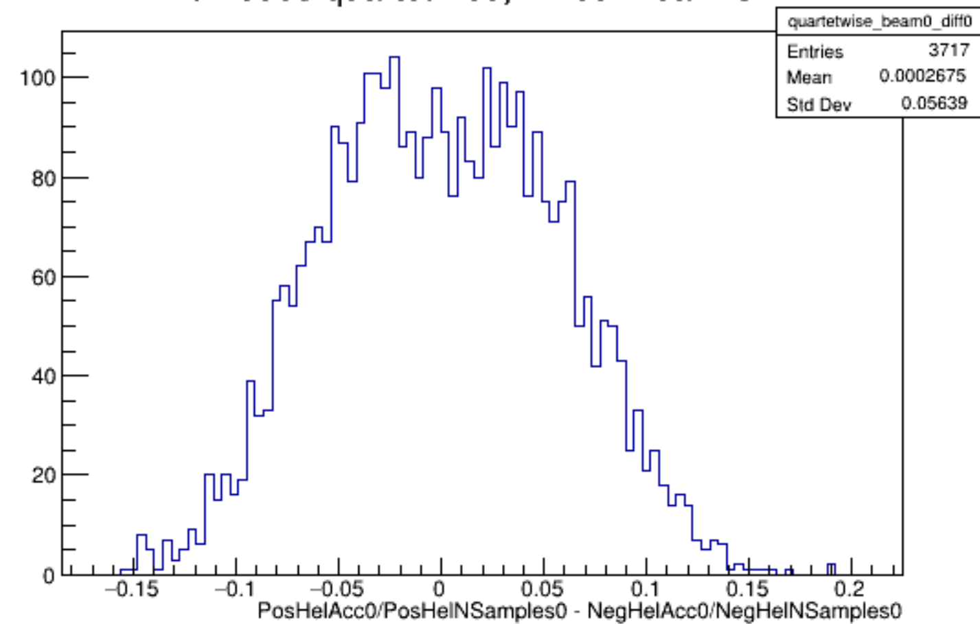
Run 5833 quartetwise, Diffs0: Beam OFF
