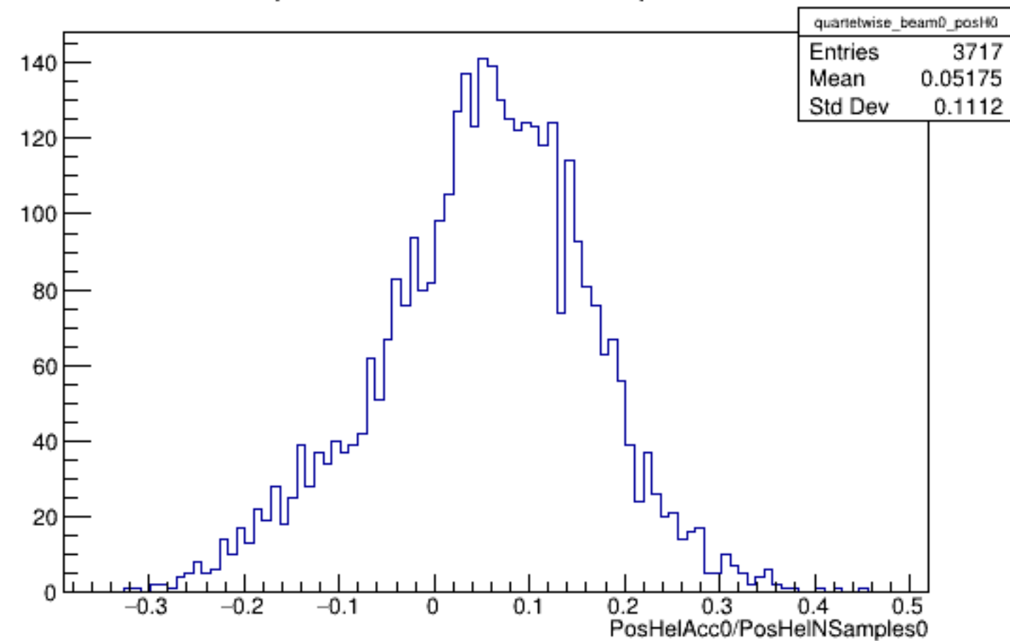
Run 5833 quartetwise, PosHelAcc0/NSamples0: Beam OFF
