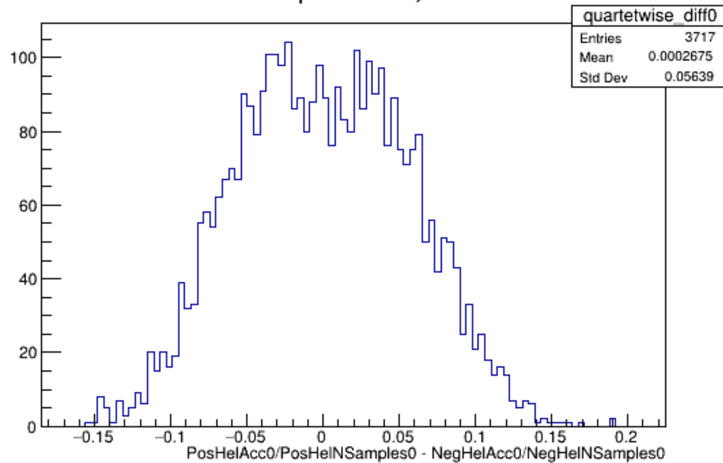
Run 5833 quartetwise, Diffs0: All
