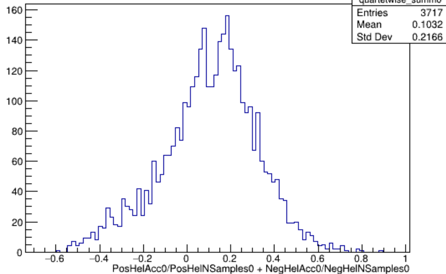
Run 5833 quartetwise, Sums0: All
