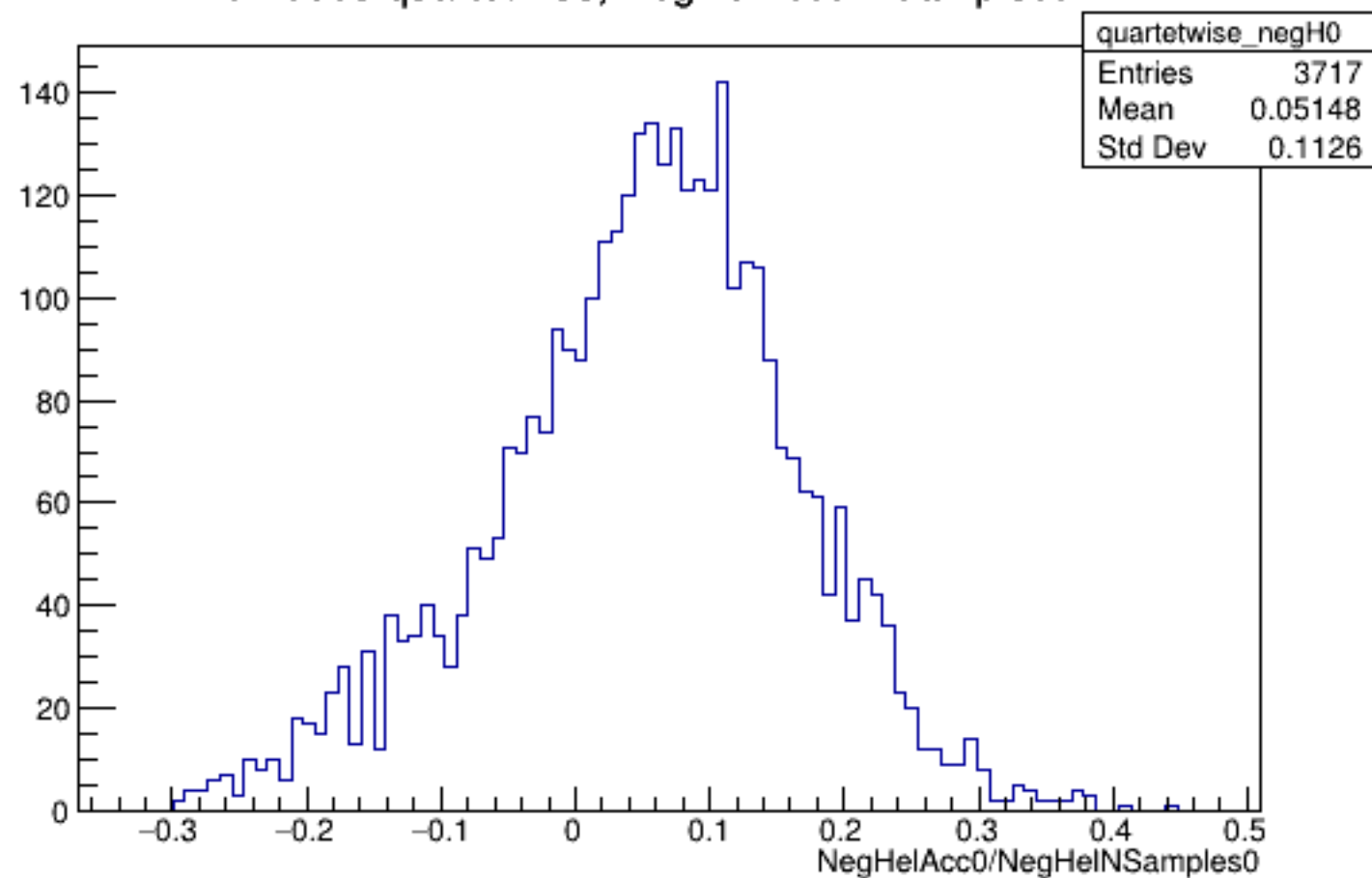
Run 5833 quartetwise, NegHelAcc0/NSamples0: All
