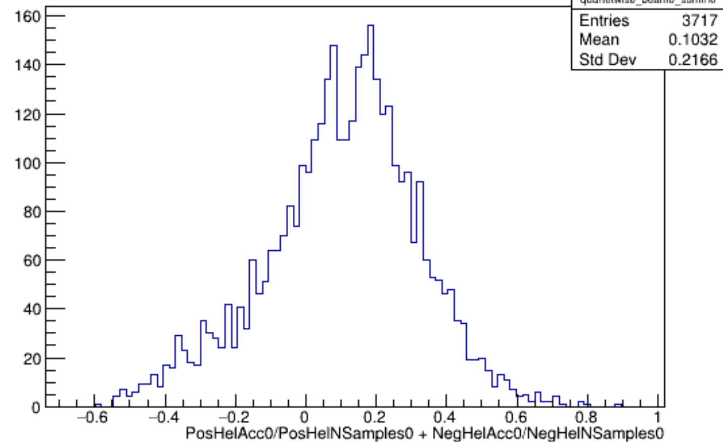
Run 5833 quartetwise, Sums0: Beam OFF
