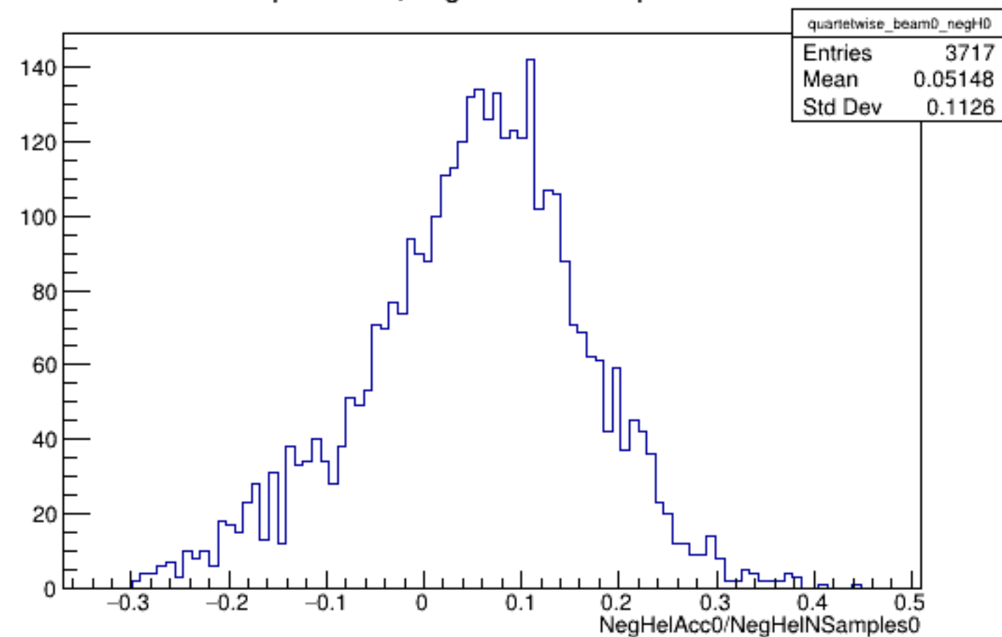
Run 5833 quartetwise, NegHelAcc0/NSamples0: Beam OFF
