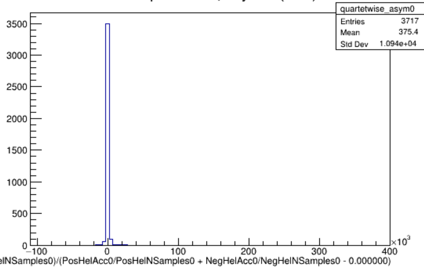
Run 5833 quartetwise, Asyms0 (Raw): All
