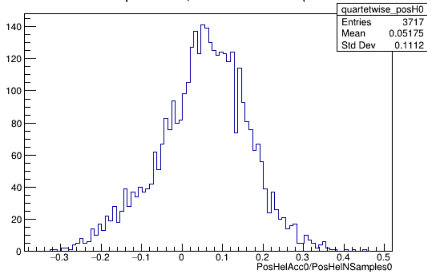
Run 5833 quartetwise, PosHelAcc0/NSamples0: All
