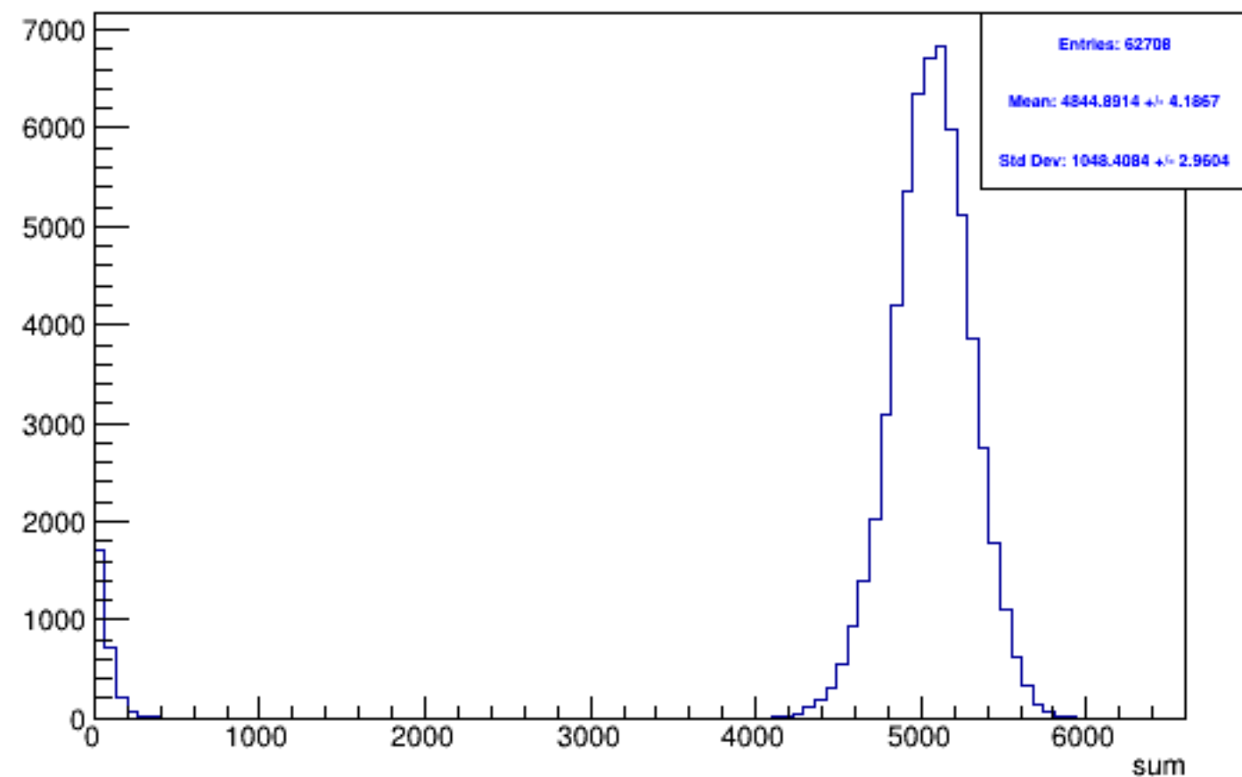
Run 5833 triggerwise, sums: Beam OFF
