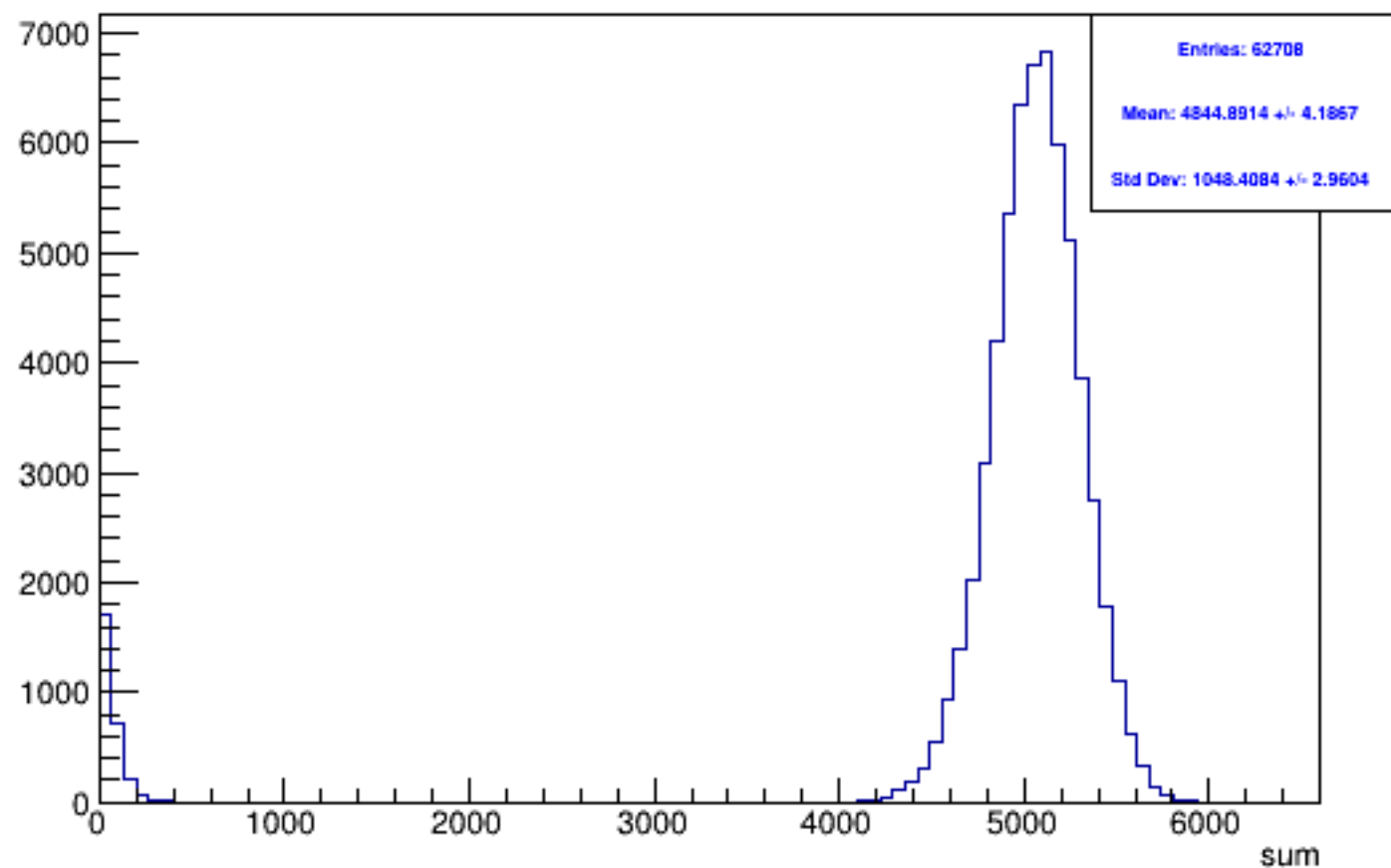
Run 5833 triggerwise, sums: All
