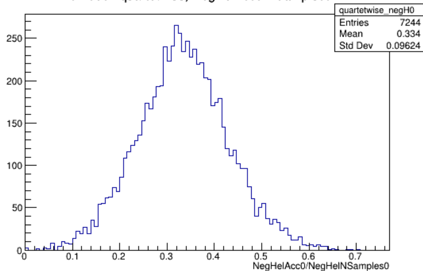
Run 5837 quartetwise, NegHelAcc0/NSamples0: All
