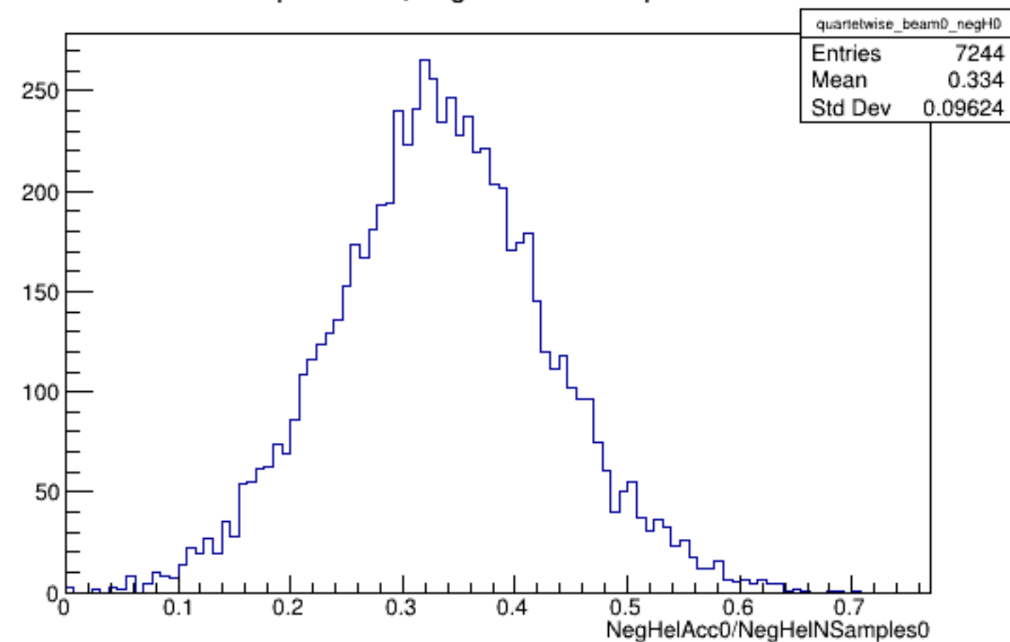
Run 5837 quartetwise, NegHelAcc0/NSamples0: Beam OFF
