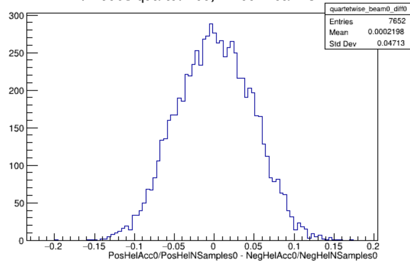
Run 5838 quartetwise, Diffs0: Beam OFF
