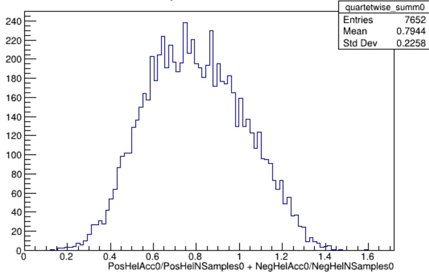
Run 5838 quartetwise, Sums0: All
