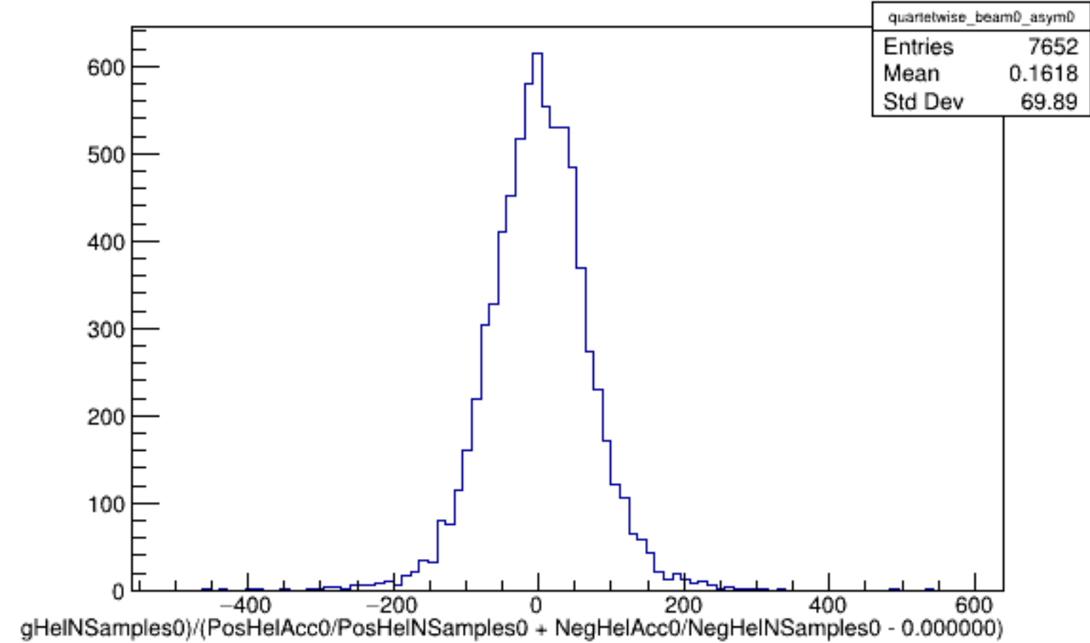
Run 5838 quartetwise, Asyms0 (Raw): Beam OFF
