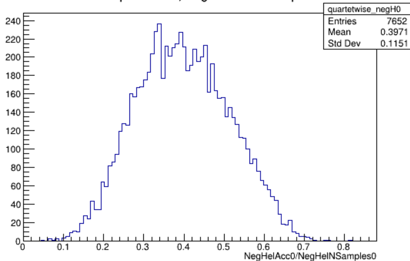
Run 5838 quartetwise, NegHelAcc0/NSamples0: All
