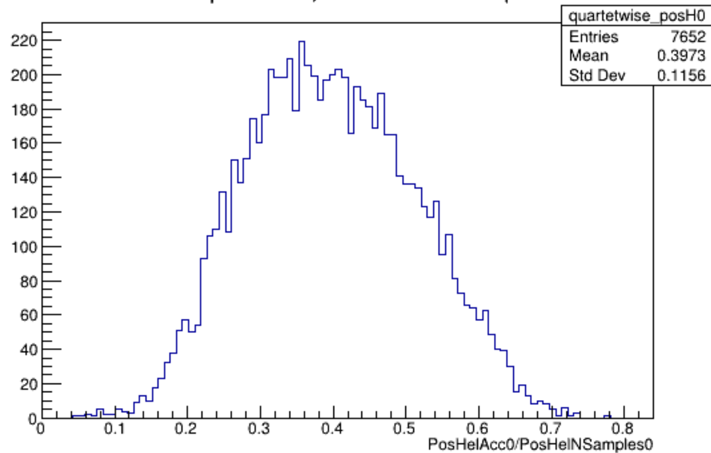
Run 5838 quartetwise, PosHelAcc0/NSamples0: All
