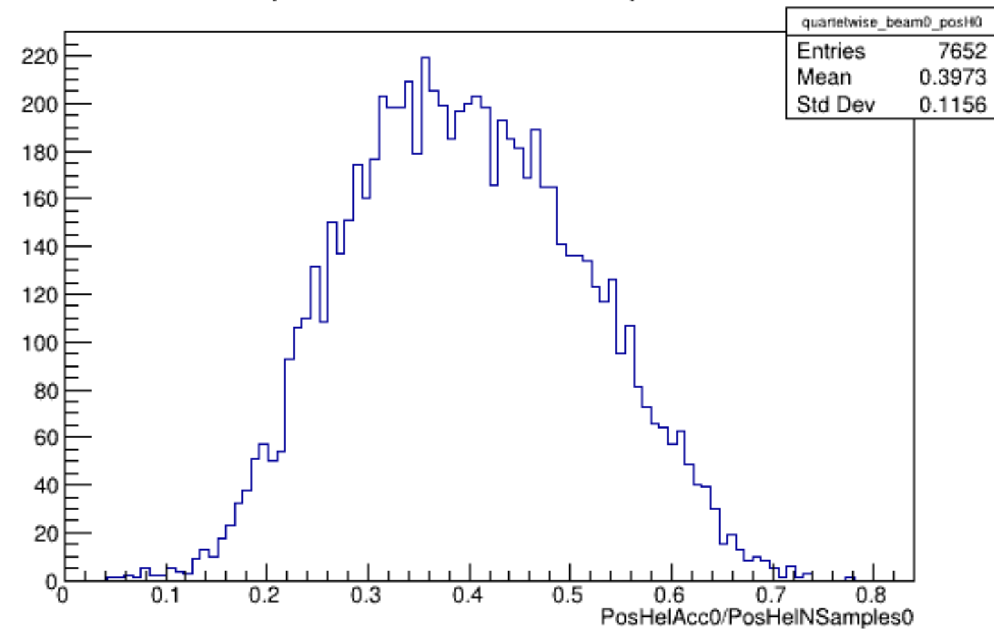
Run 5838 quartetwise, PosHelAcc0/NSamples0: Beam OFF
