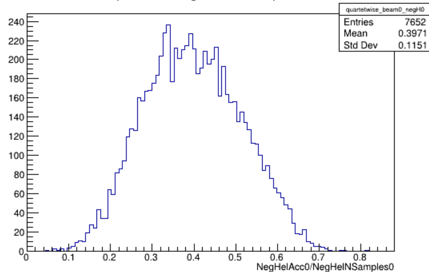
Run 5838 quartetwise, NegHelAcc0/NSamples0: Beam OFF
