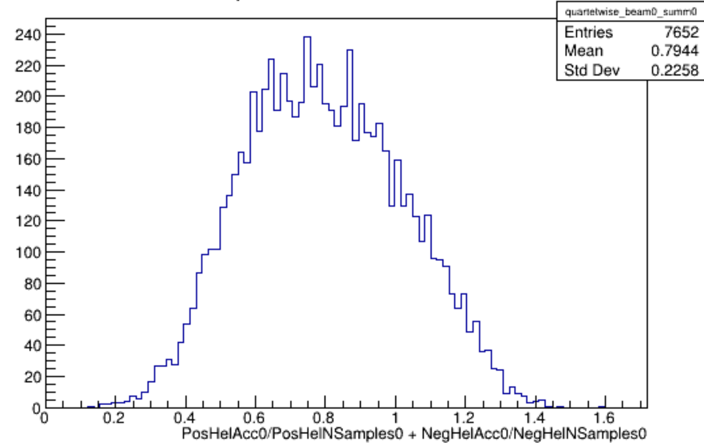
Run 5838 quartetwise, Sums0: Beam OFF
