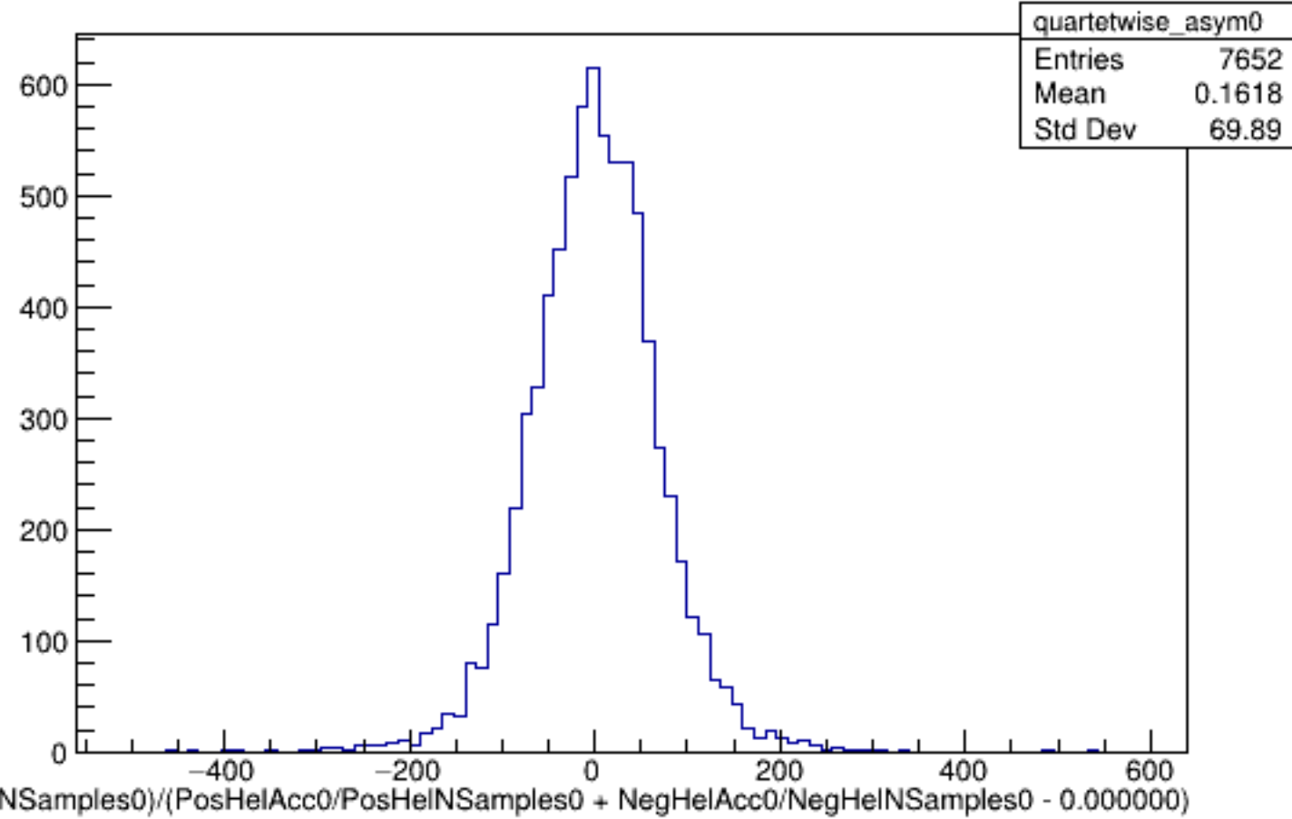
Run 5838 quartetwise, Asyms0 (Raw): All
