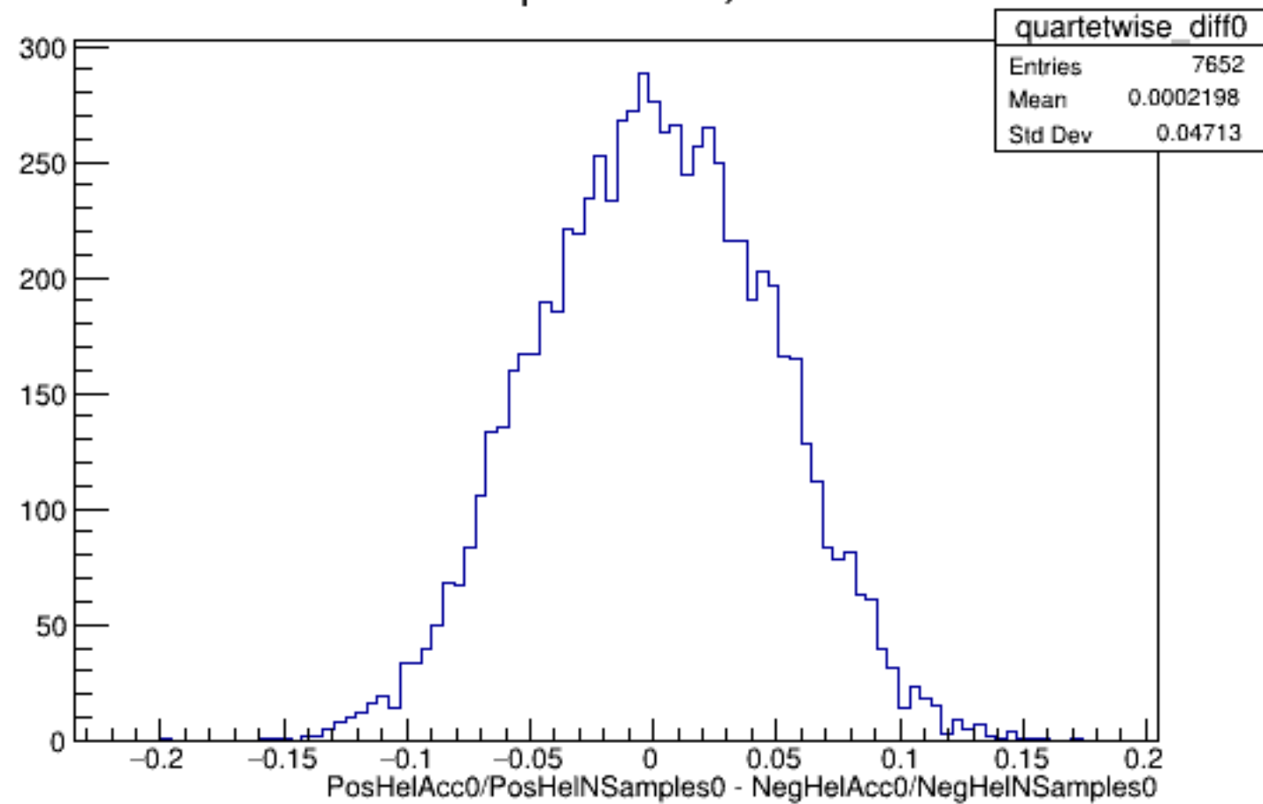
Run 5838 quartetwise, Diffs0: All
