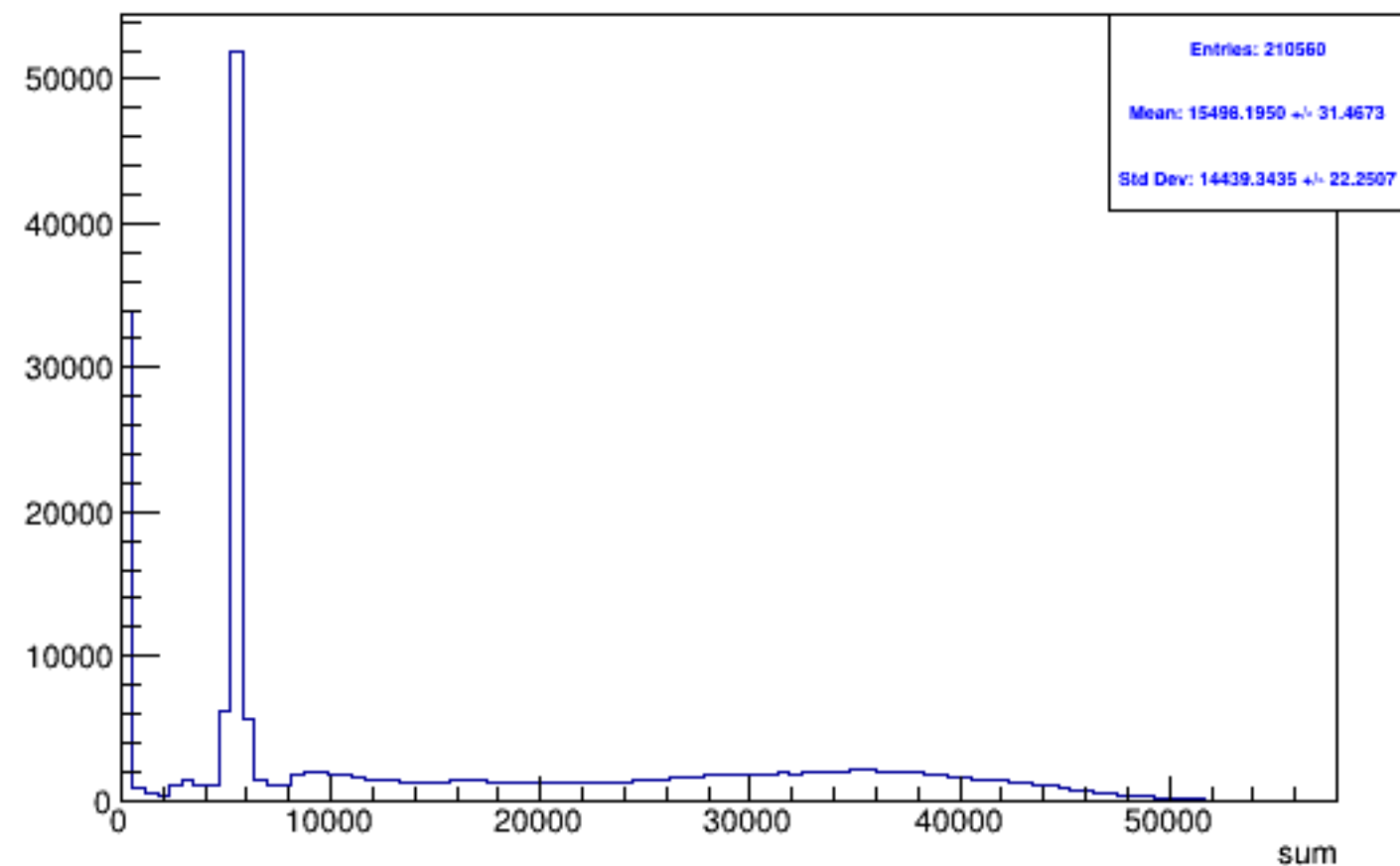
Run 5838 triggerwise, sums: Beam OFF
