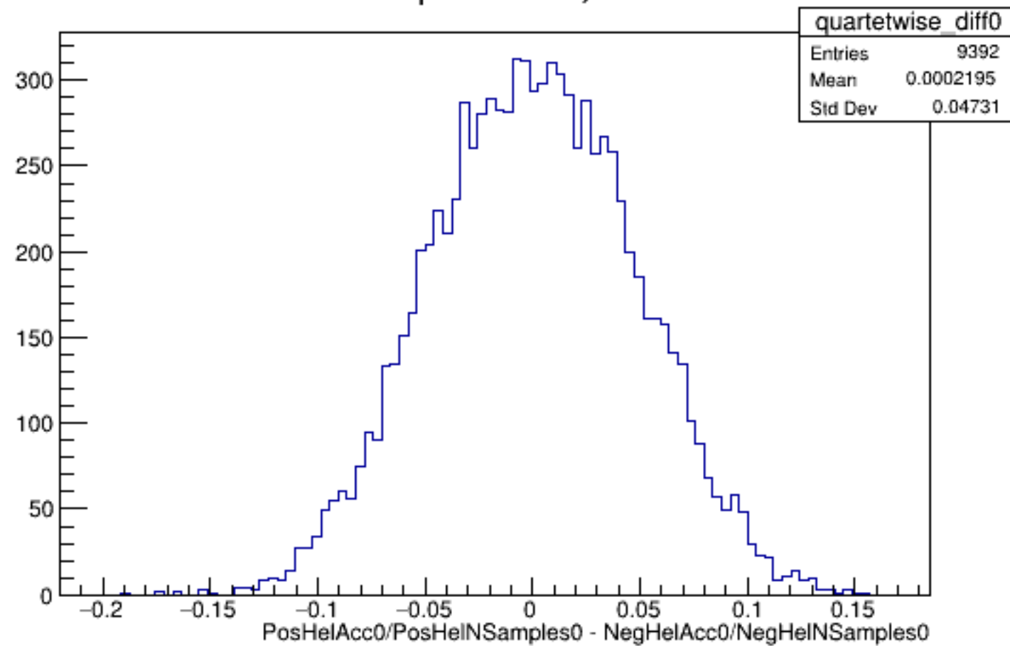
Run 5839 quartetwise, Diffs0: All
