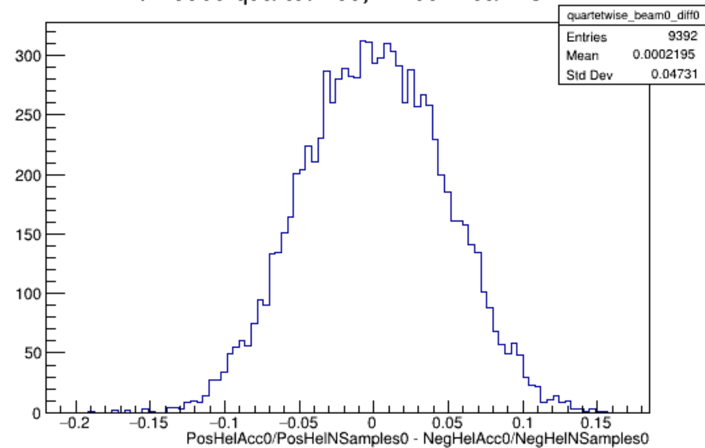
Run 5839 quartetwise, Diffs0: Beam OFF
