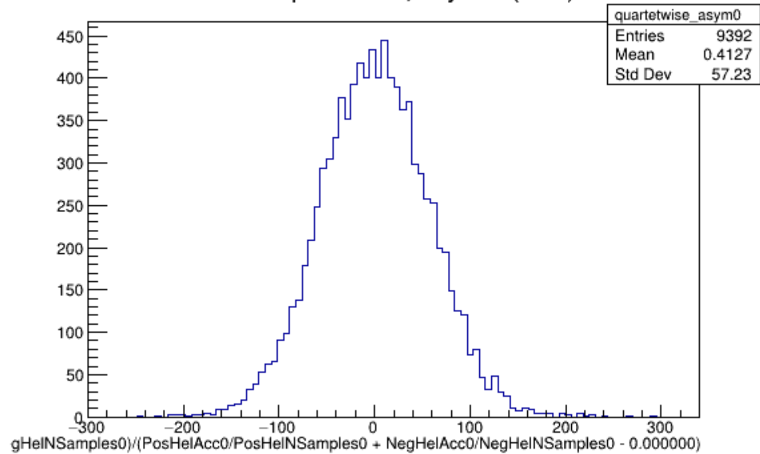
Run 5839 quartetwise, Asyms0 (Raw): All
