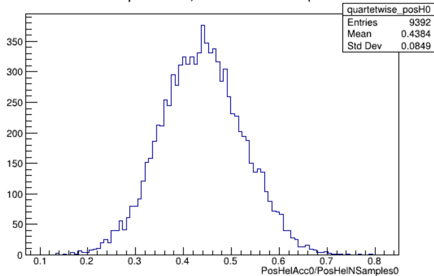
Run 5839 quartetwise, PosHelAcc0/NSamples0: All
