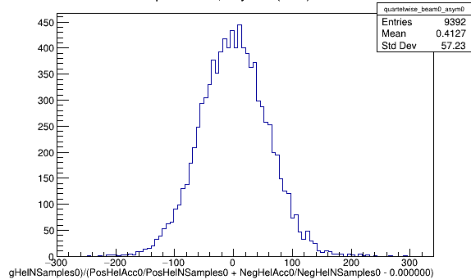
Run 5839 quartetwise, Asyms0 (Raw): Beam OFF
