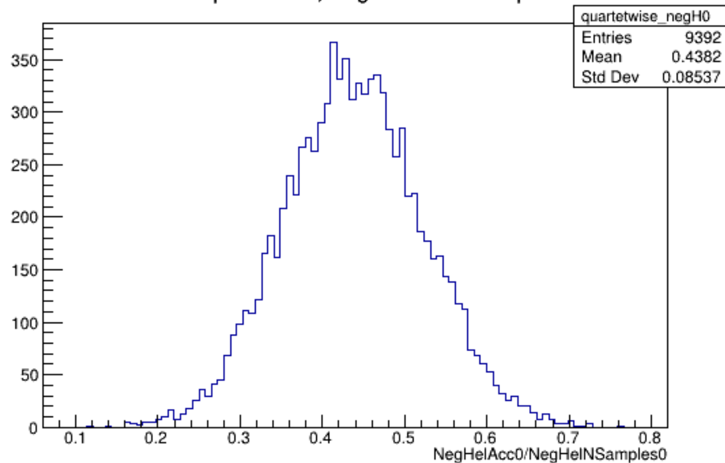
Run 5839 quartetwise, NegHelAcc0/NSamples0: All
