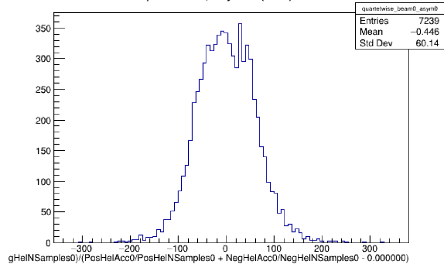
Run 5840 quartetwise, Asyms0 (Raw): Beam OFF
