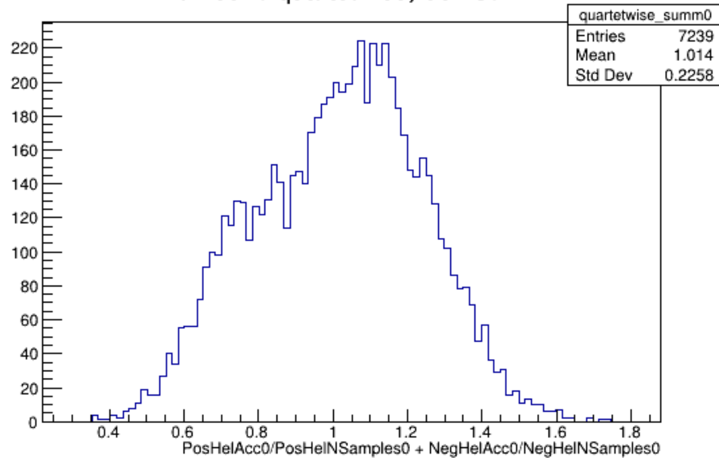
Run 5840 quartetwise, Sums0: All
