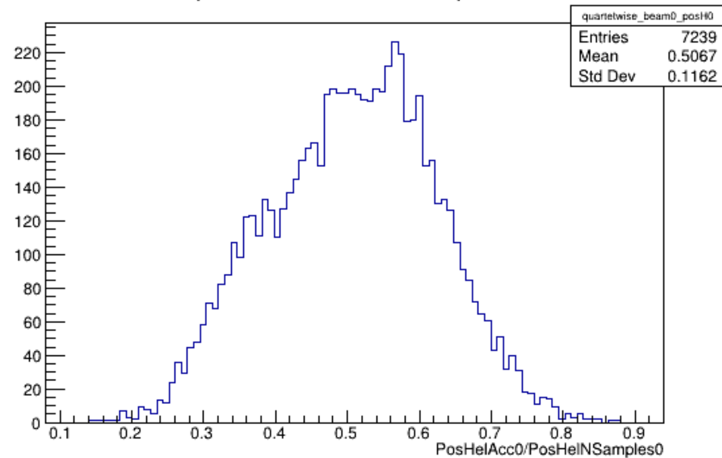
Run 5840 quartetwise, PosHelAcc0/NSamples0: Beam OFF
