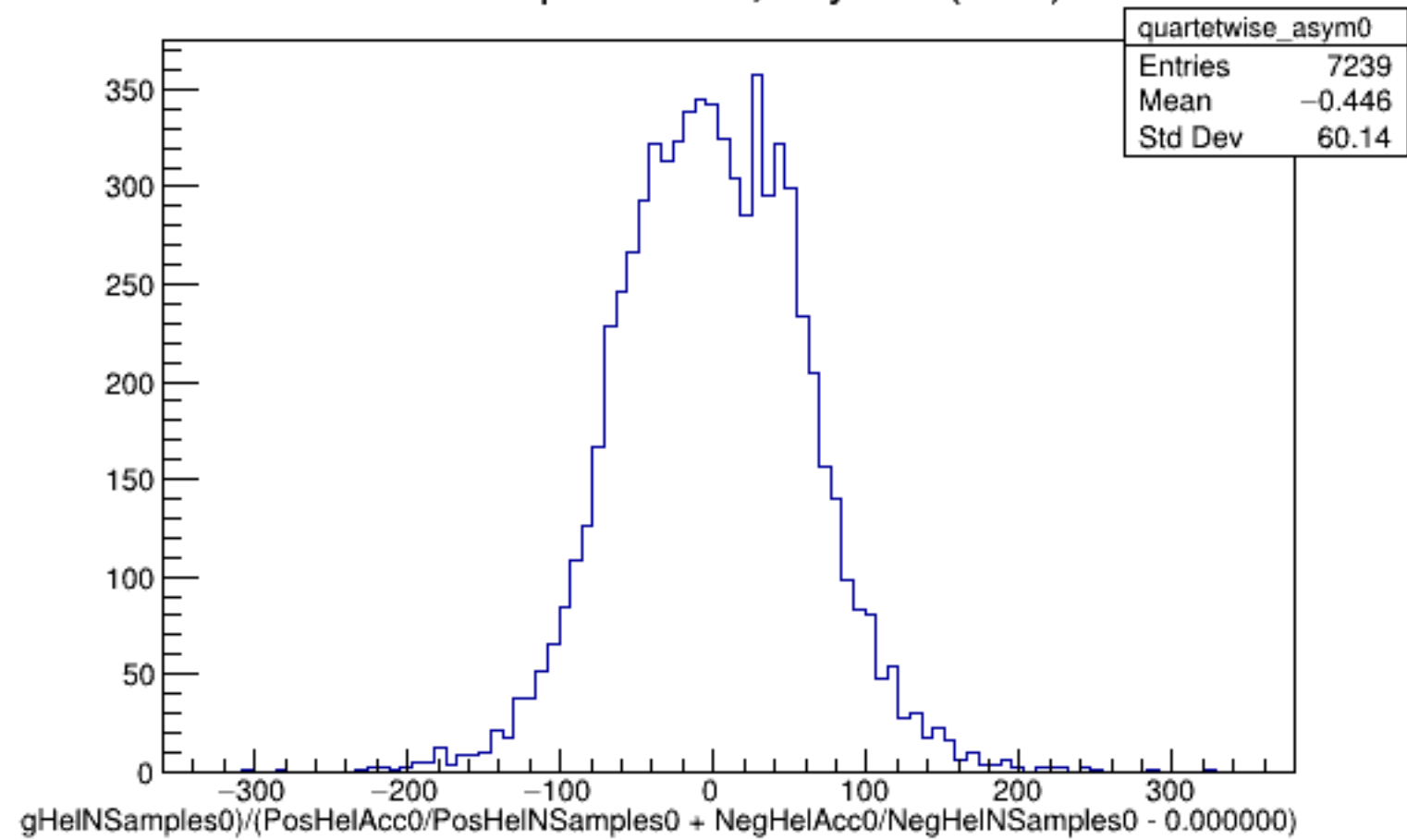
Run 5840 quartetwise, Asyms0 (Raw): All
