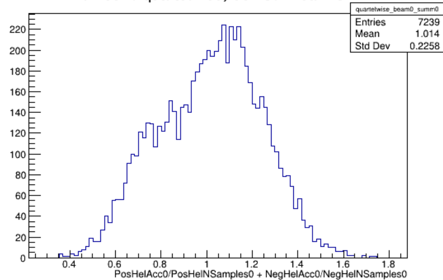
Run 5840 quartetwise, Sums0: Beam OFF
