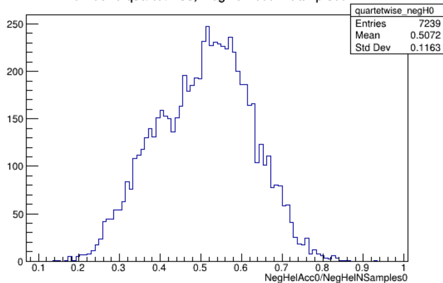
Run 5840 quartetwise, NegHelAcc0/NSamples0: All
