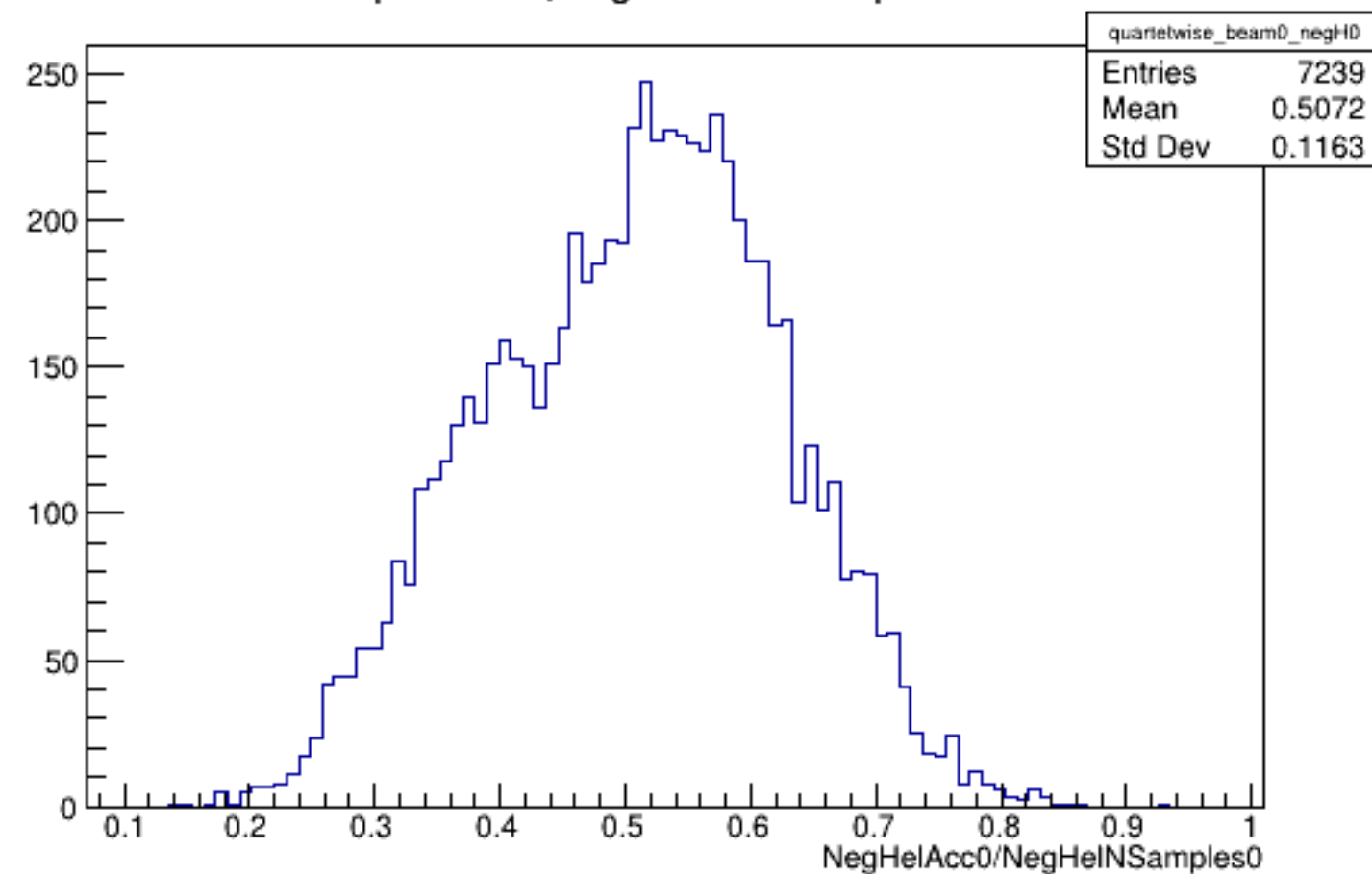
Run 5840 quartetwise, NegHelAcc0/NSamples0: Beam OFF
