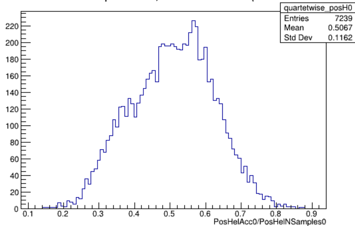
Run 5840 quartetwise, PosHelAcc0/NSamples0: All
