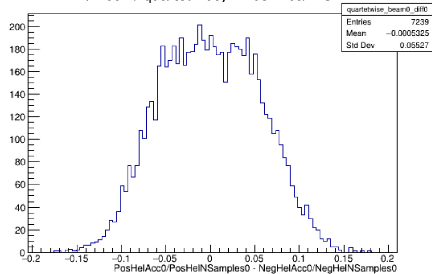
Run 5840 quartetwise, Diffs0: Beam OFF
