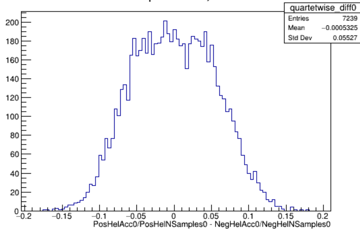
Run 5840 quartetwise, Diffs0: All
