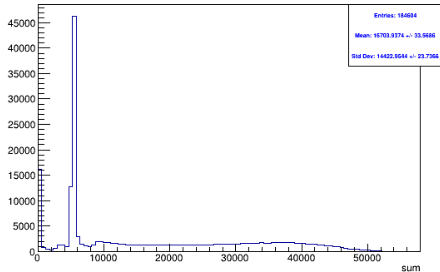
Run 5840 triggerwise, sums: Beam OFF
