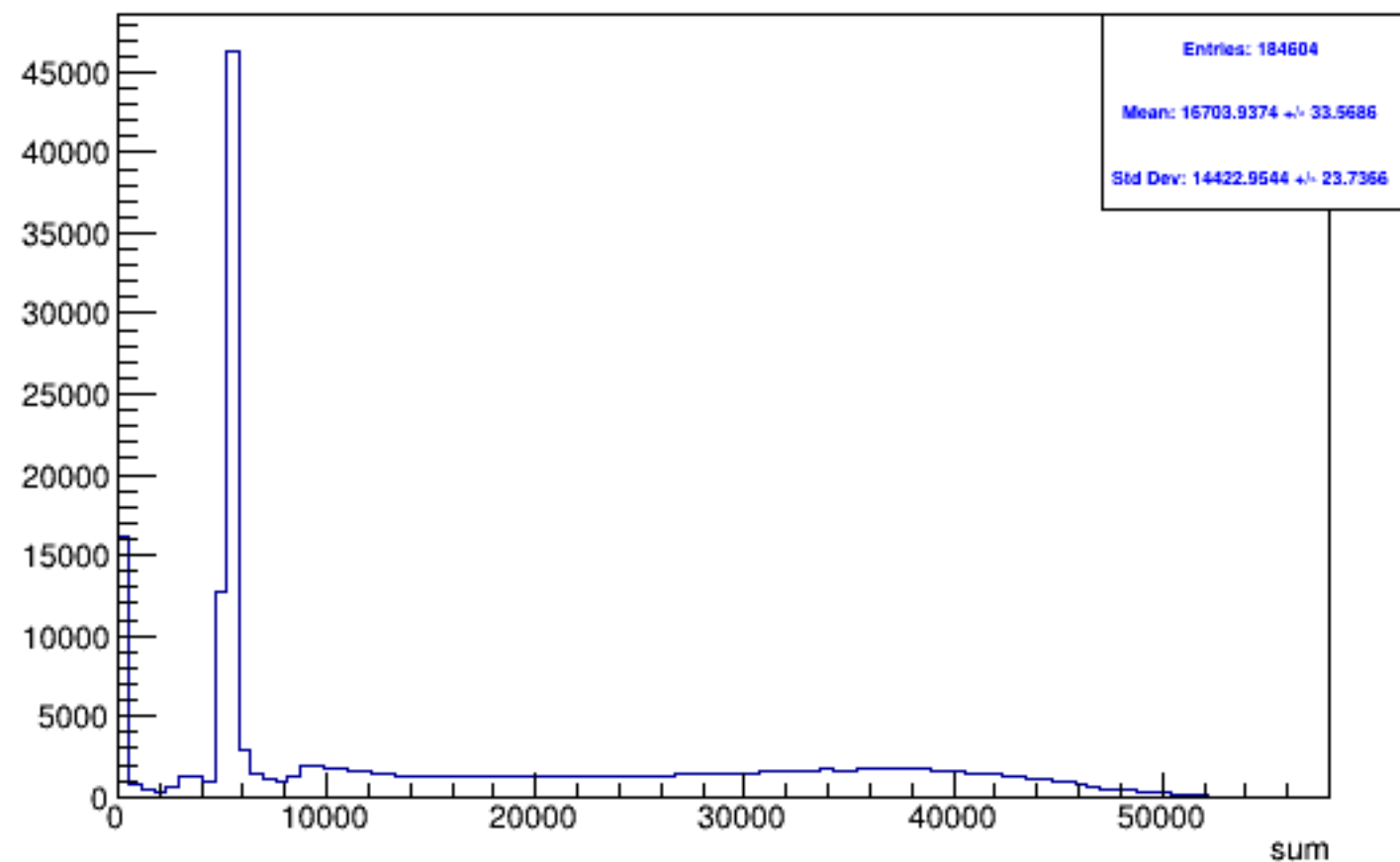
Run 5840 triggerwise, sums: All
