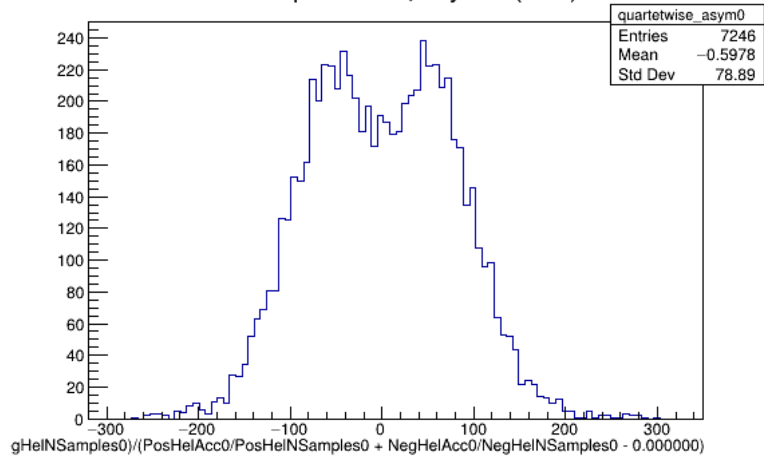
Run 5850 quartetwise, Asyms0 (Raw): All
