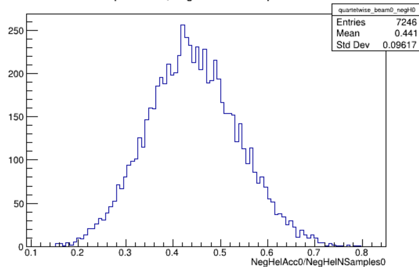
Run 5850 quartetwise, NegHelAcc0/NSamples0: Beam OFF
