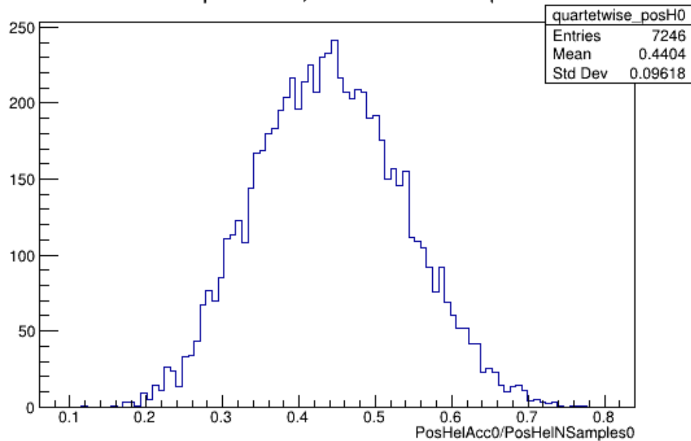
Run 5850 quartetwise, PosHelAcc0/NSamples0: All
