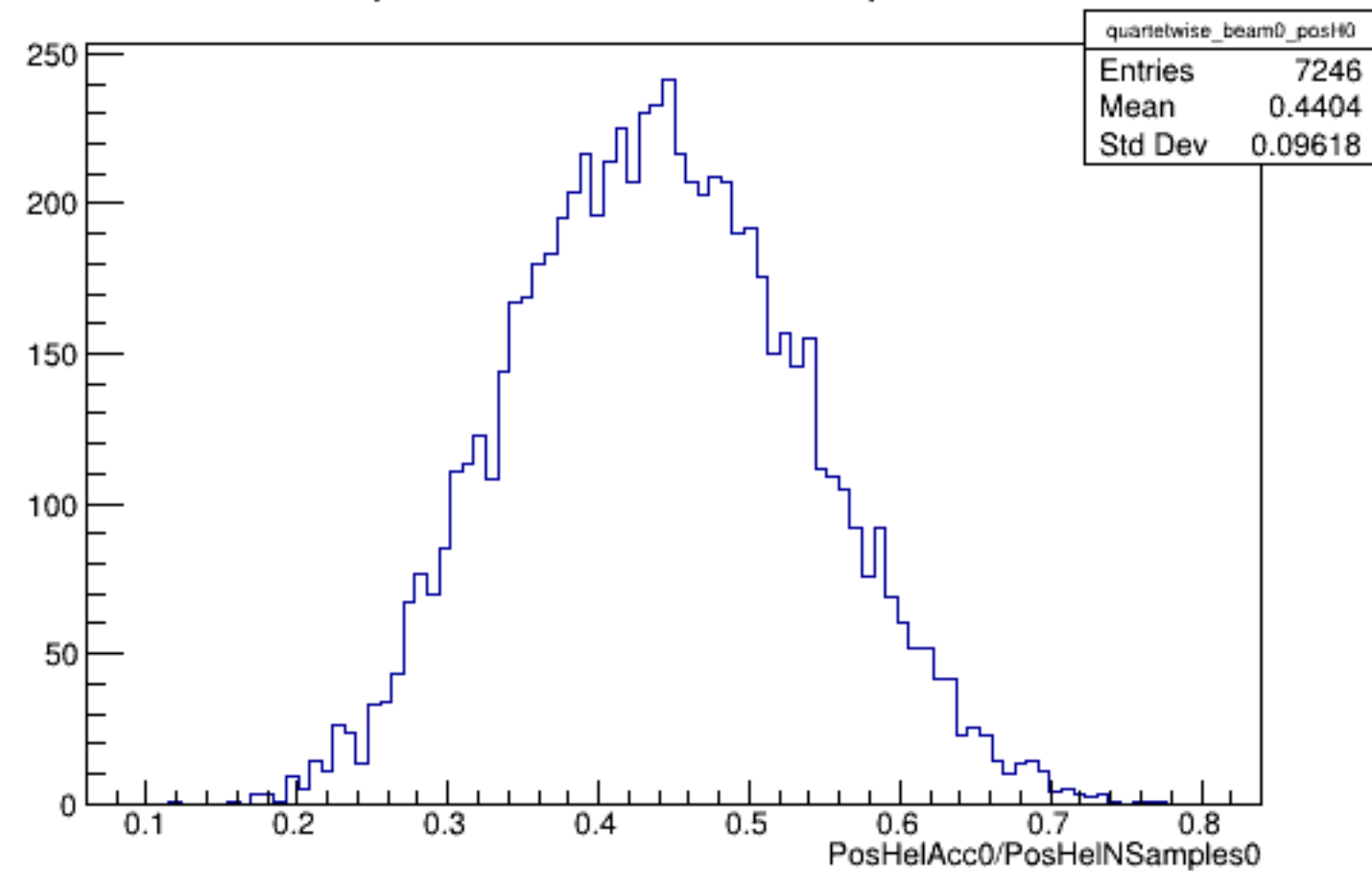
Run 5850 quartetwise, PosHelAcc0/NSamples0: Beam OFF
