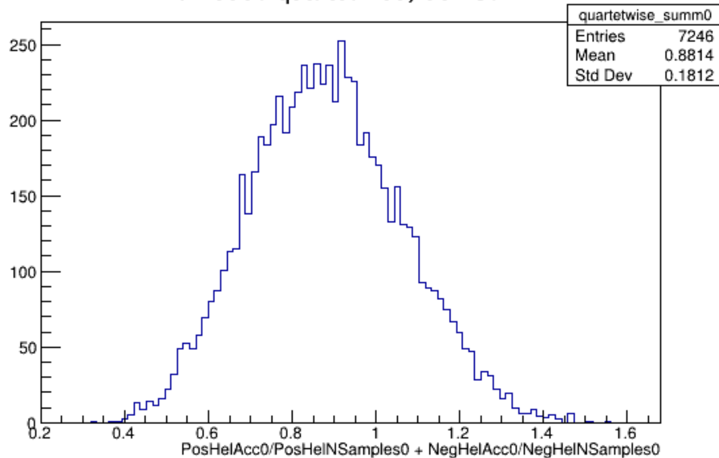
Run 5850 quartetwise, Sums0: All
