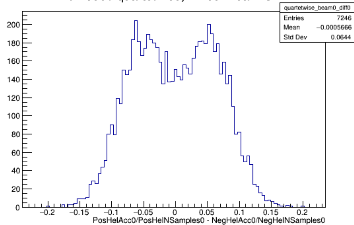
Run 5850 quartetwise, Diffs0: Beam OFF
