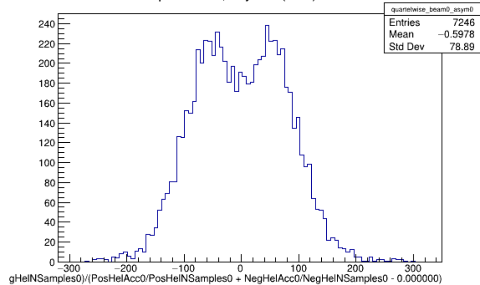
Run 5850 quartetwise, Asyms0 (Raw): Beam OFF
