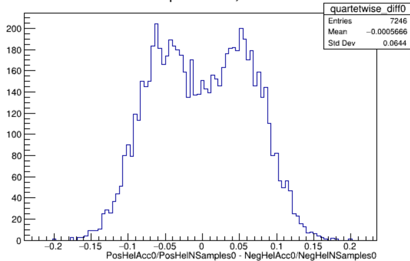
Run 5850 quartetwise, Diffs0: All
