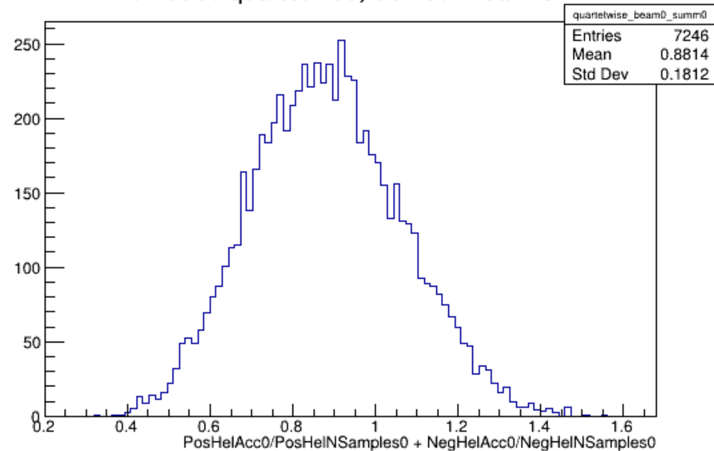
Run 5850 quartetwise, Sums0: Beam OFF
