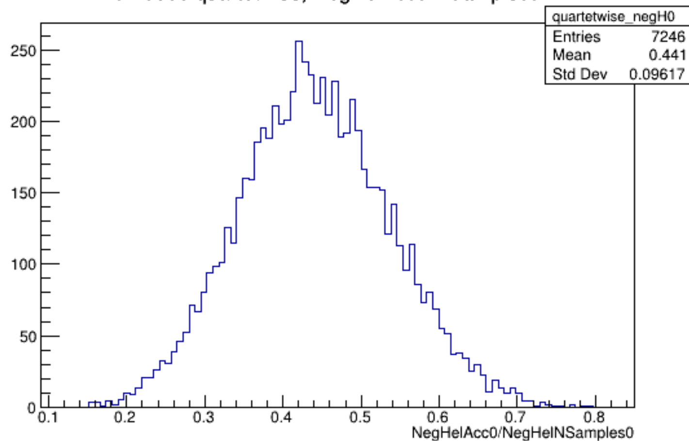
Run 5850 quartetwise, NegHelAcc0/NSamples0: All
