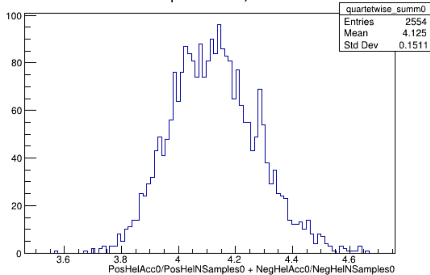
Run 5851 quartetwise, Sums0: All
