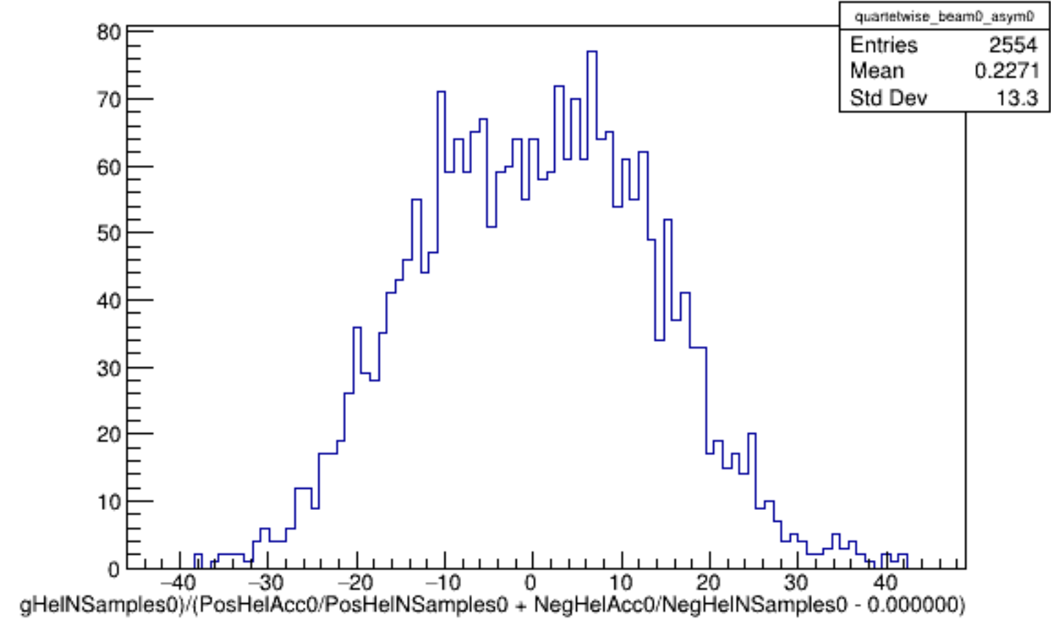
Run 5851 quartetwise, Asyms0 (Raw): Beam OFF
