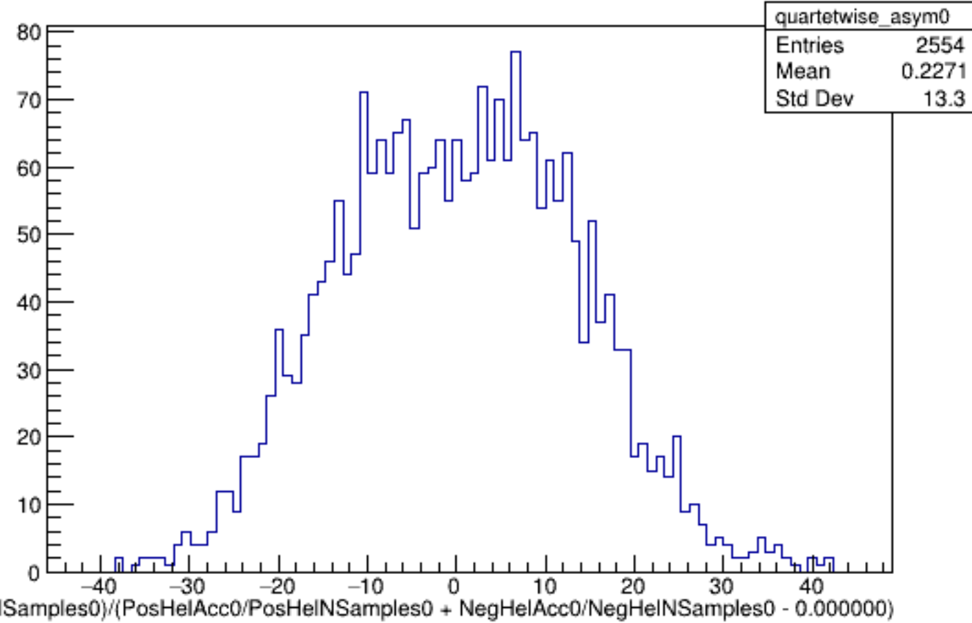
Run 5851 quartetwise, Asyms0 (Raw): All
