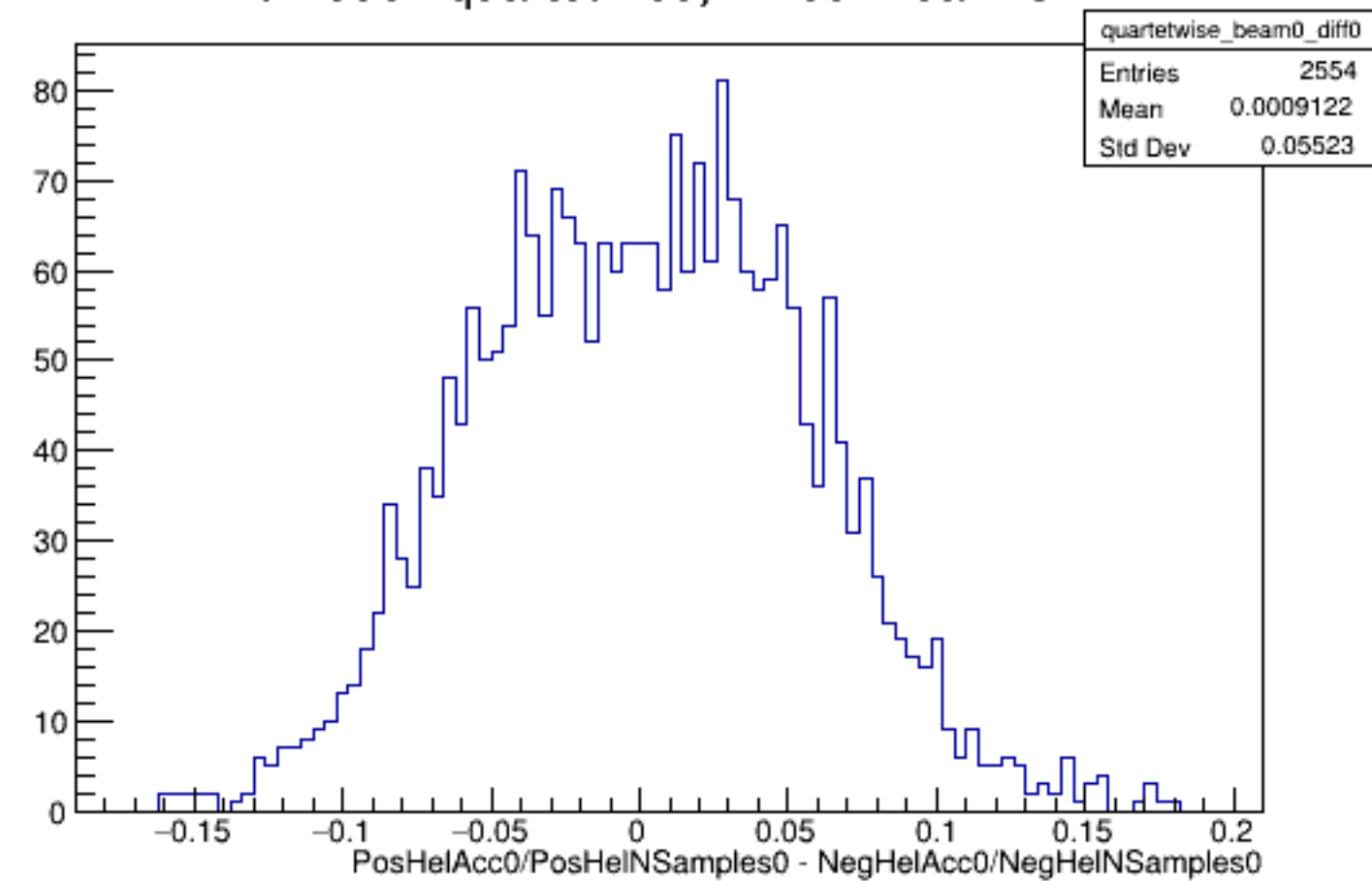
Run 5851 quartetwise, Diffs0: Beam OFF
