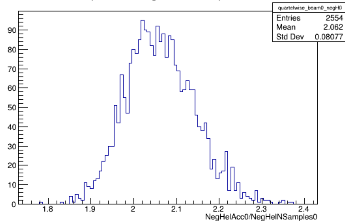
Run 5851 quartetwise, NegHelAcc0/NSamples0: Beam OFF
