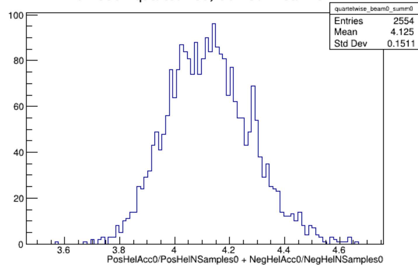
Run 5851 quartetwise, Sums0: Beam OFF
