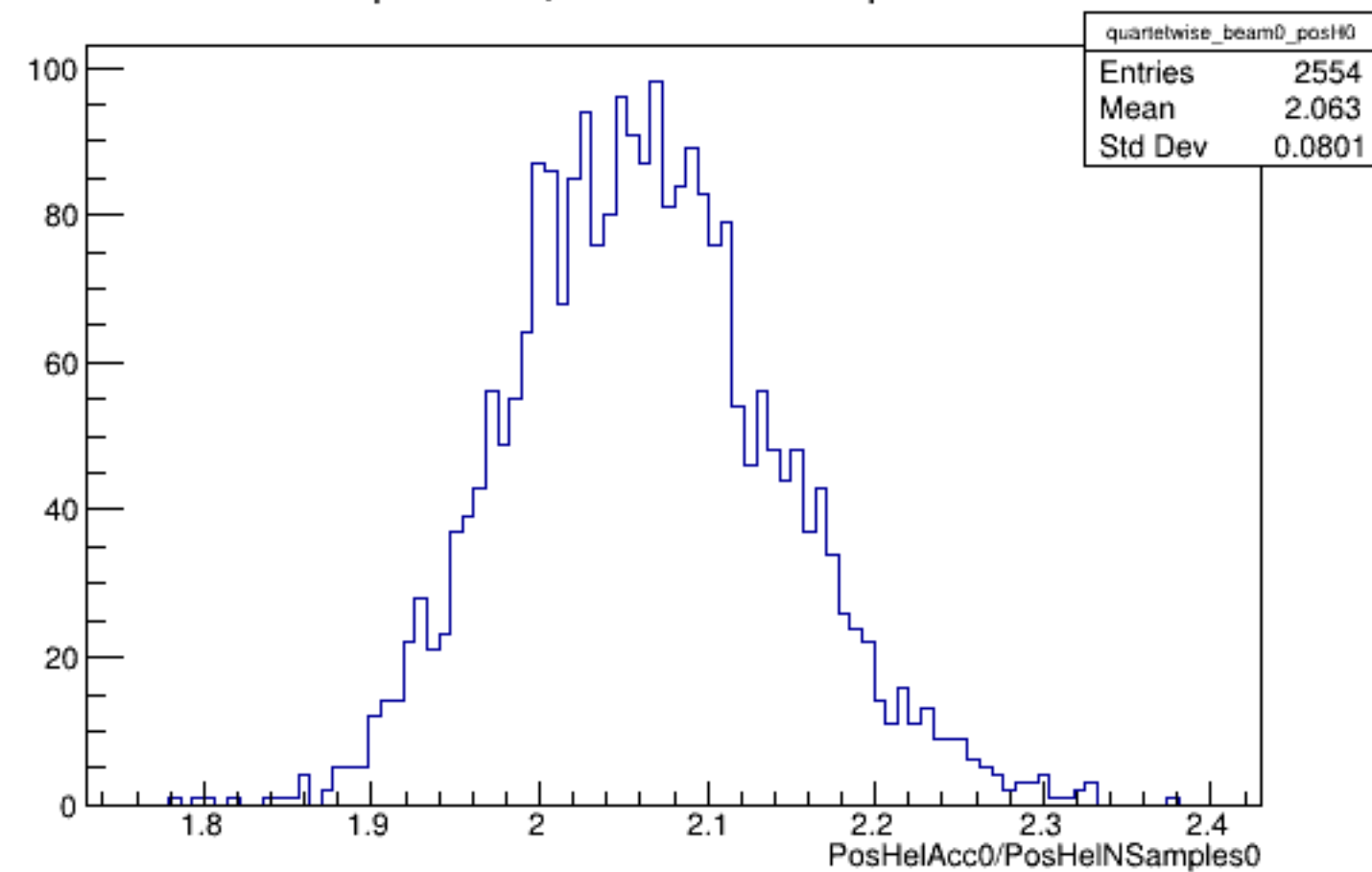
Run 5851 quartetwise, PosHelAcc0/NSamples0: Beam OFF
