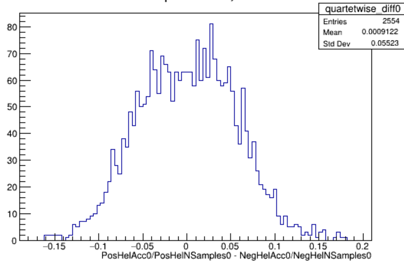
Run 5851 quartetwise, Diffs0: All
