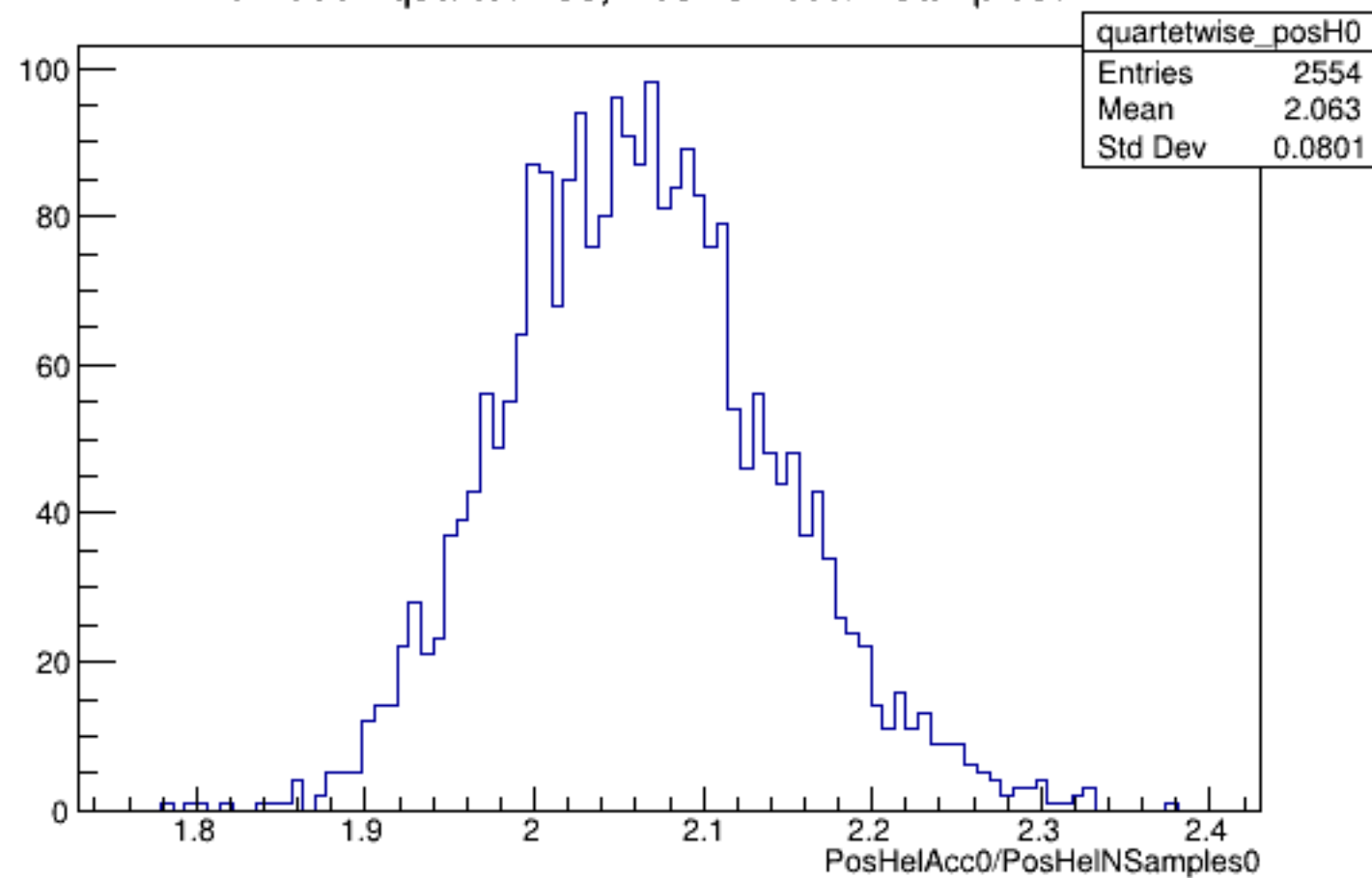
Run 5851 quartetwise, PosHelAcc0/NSamples0: All
