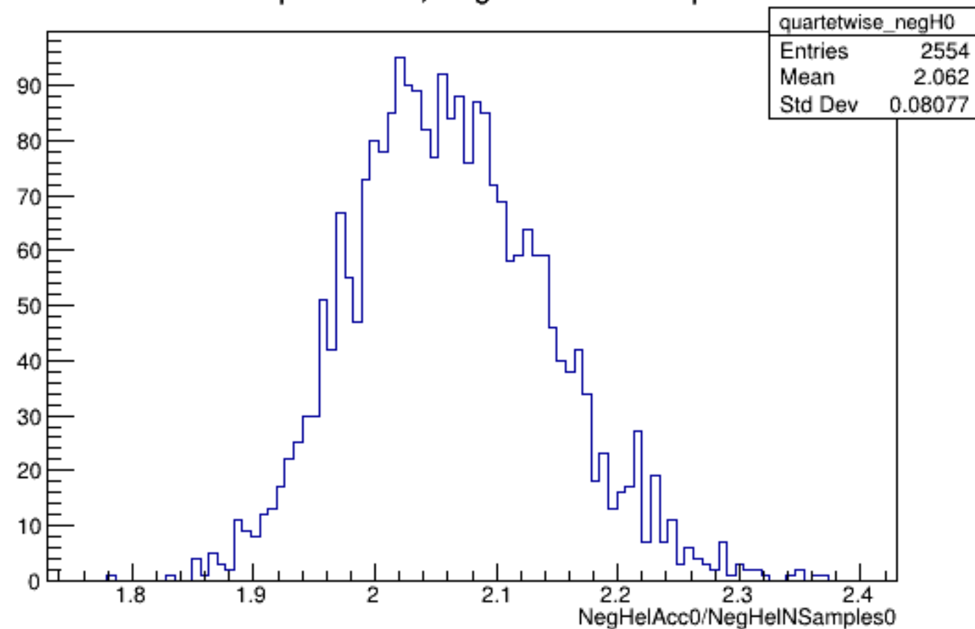
Run 5851 quartetwise, NegHelAcc0/NSamples0: All
